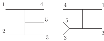
Figure 5.10: Interference of diagrams leading to factors of s_{35}s_{23} in the denominator.
