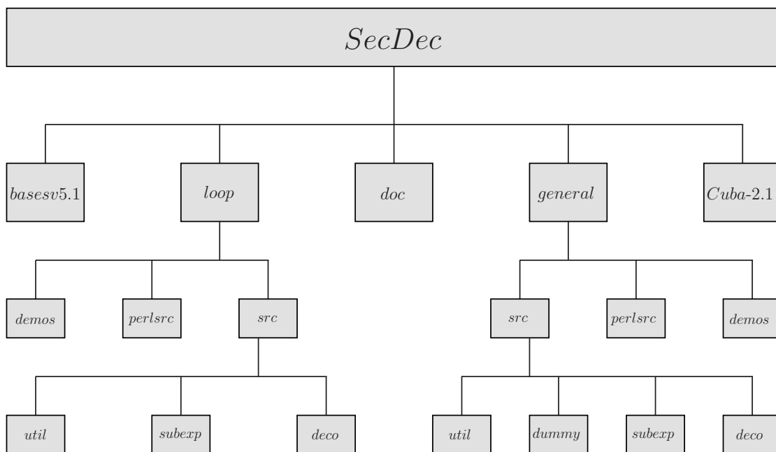
Figure 5.1: Directory structure of the SecDec program.
