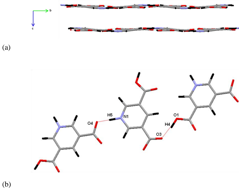
Figure 3.1: (a) The packing of 35PDCA as viewed down the a axis. (b) The structure of 35PDCA in the ab plane, highlighting the SSHB (N1–H5...O4), at 15 K.
