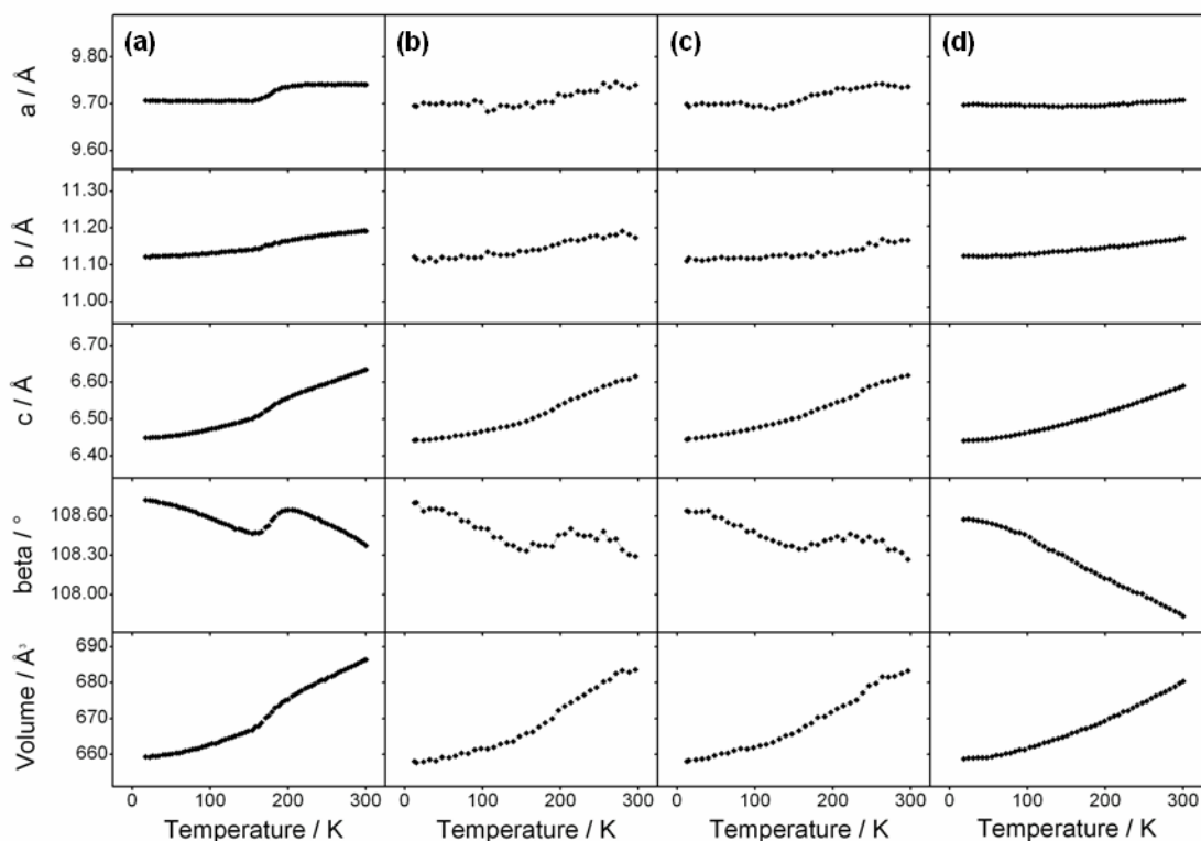
Figure 3.5: Temperature dependence of the unit cell parameters of the four ^{35}\text{PDCA} isotopologues obtained from variable temperature XRD data by sequential single-phase
