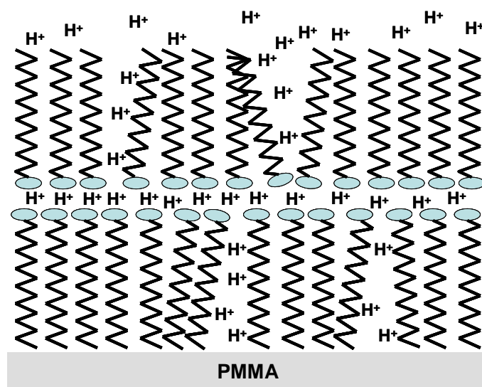
Figure 6.12 Schematic diagram of the 10-layer AA membrane when exposed to the acid solutions.
