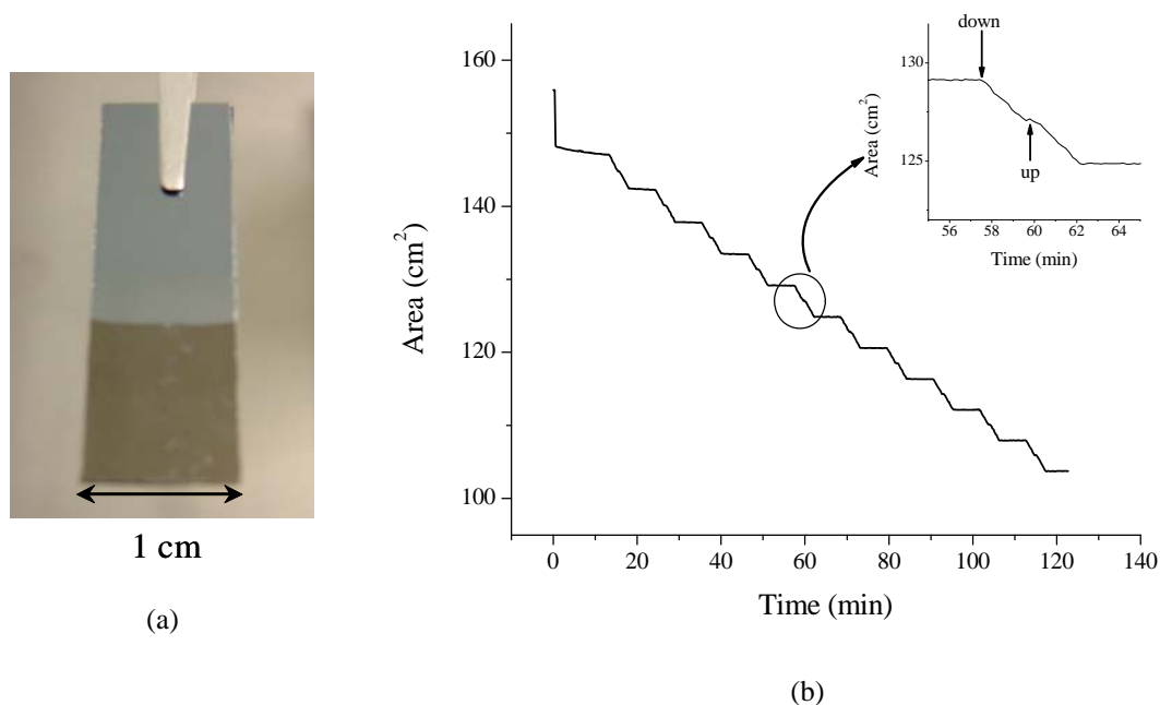
Figure 4.11 (a) Cadmium arachidate film on a Si wafer. (b) Dipping profile for depositing cadmium arachidate film onto a Si wafer
