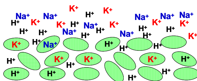
Figure 7.7 Schematic diagram of the ISOFETs coated by multimolecular layers of pure valinomycin.
