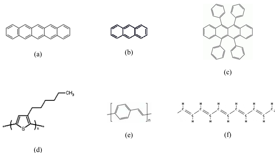
Figure 2.1 Chemical structure of some organic semiconductors. (a) Pentacene. (b) Anthracene. (c) Rubrene. (d) Poly (3-hexylthiophene). (e) Poly(p-phenylene vinylene). (f) Polyacetylene.
