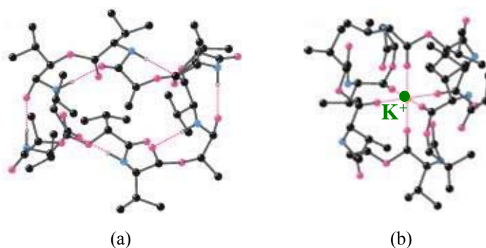
Figure 7.8 Schematic diagrams of molecular structures. (a) Uncomplexed valinomycin. (b) Valinomycin - K^+ complex.
