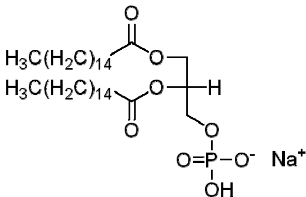
Figure 4.2 Chemical structure of 1,2-Dipalmitoyl- sn -glycero-3-phosphatidic acid.
