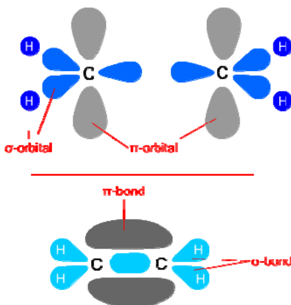
Figure 2.2 Schematic diagrams of \sigma and \pi bonds formed between carbon atoms.
