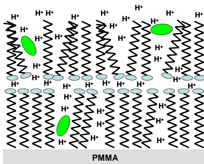
Figure 6.13 Schematic diagram of the 10-layer membrane of 95%AA + 5 %val when exposed to the acid solutions.
