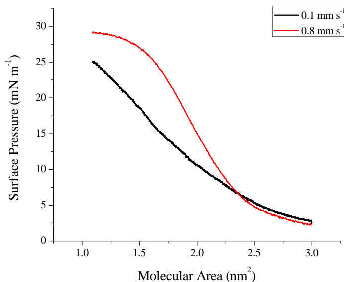
Figure 4.7 Isotherms of valinomycin at 293 K, pH 5.5, with compression speeds of 0.1 \text{ mm s}^{-1} (black) and 0.8 \text{ mm s}^{-1} (red).
