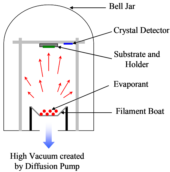
Figure 3.1 Schematic diagram of thermal vapour deposition.
