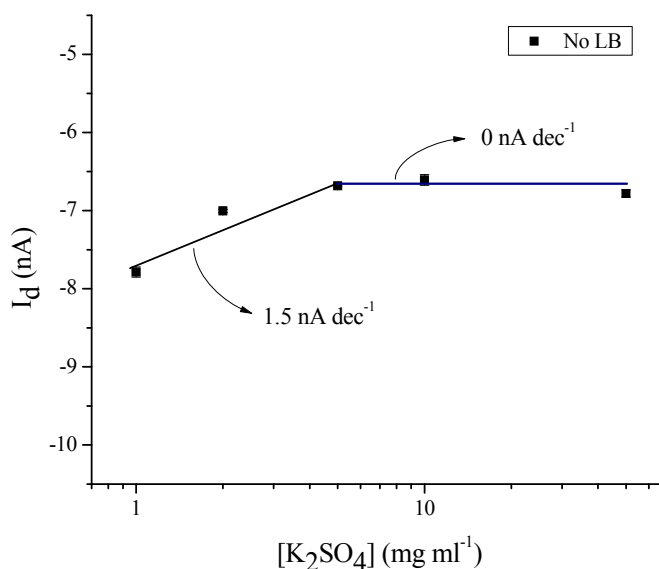
Figure 7.1 pK response of an uncoated interdigitated ISOFET.
