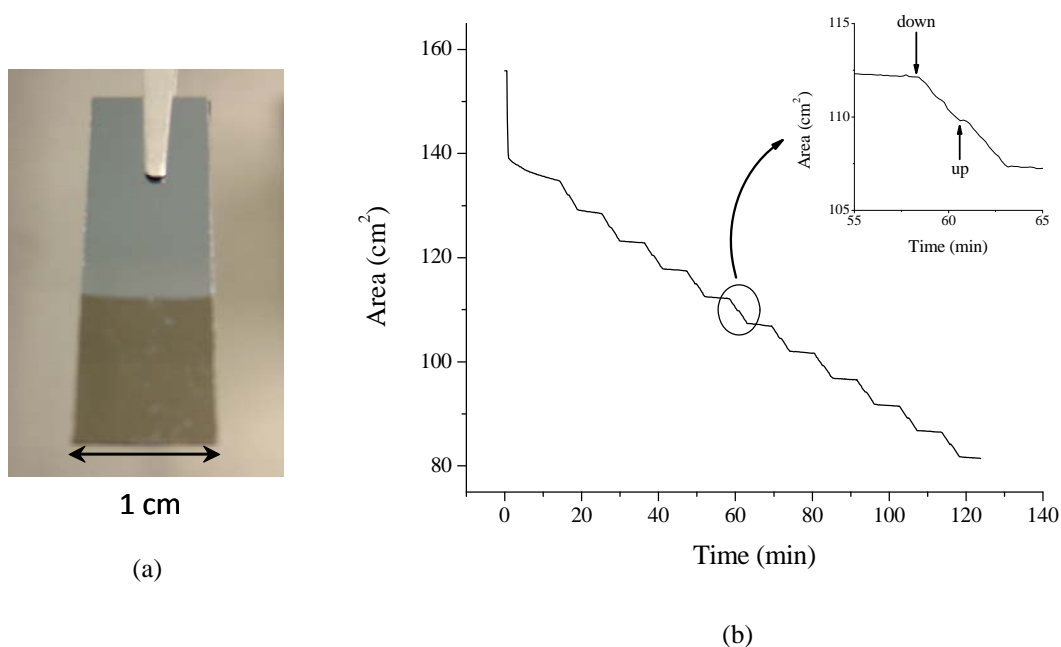
Figure 4.10 (a) Arachidic acid film on a Si wafer. (b) Dipping profile for depositing arachidic acid film onto a Si wafer.
