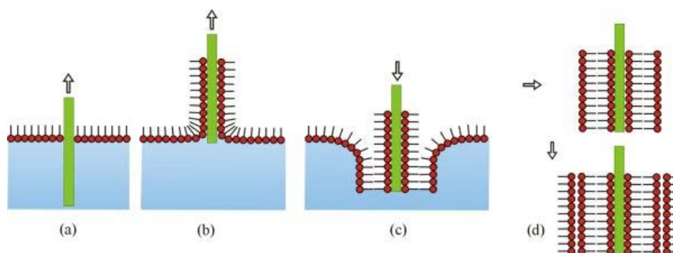
Figure 3.9 Y-type deposition of monomolecular film onto a substrate : (a) Moving the substrate out of the subphase. (b) Monomolecular layer attached onto the substrate while moving out the subphase. (c) A further monomolecular layer is deposited onto the substrate while moving the substrate down into the subphase. (d) A multilayer film is deposited on the substrate by repeatedly moving the substrate up and down.
