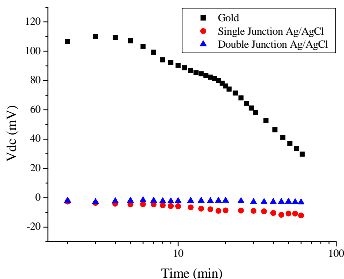
Figure 5.5 Potentials across the different gate electrodes, gold wires, single junction Ag/AgCl and double junction Ag/AgCl, in DI water.
