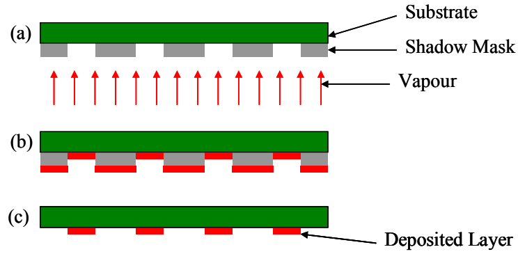
Figure 3.2 (a) Schematic diagram of the shadow mask deposition. (b) Thin film deposited on the masked substrate. (c) Thin film on the substrate after removing the mask.
