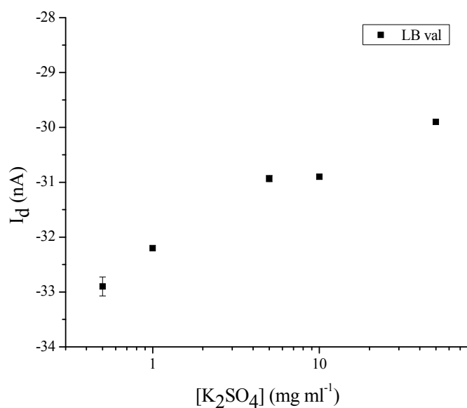
Figure 7.5 pK response of an interdigitated ISOFET with 10 LB monolayers of pure valinomycin.
