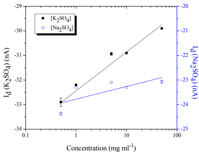
Figure 7.11 pK and pNa responses of an interdigitated ISOFET with 10 LB monolayers of pure val.
