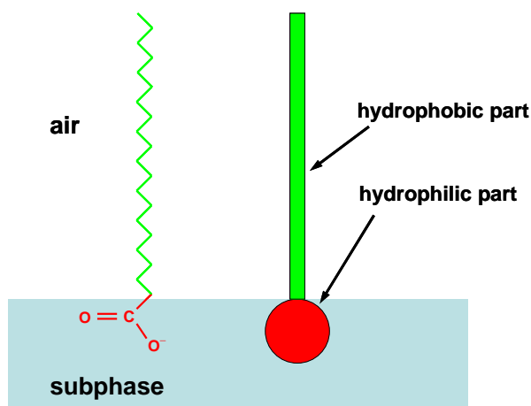
Figure 3.6 Amphiphilic molecule (fatty acid) on the surface of water (subphase).
