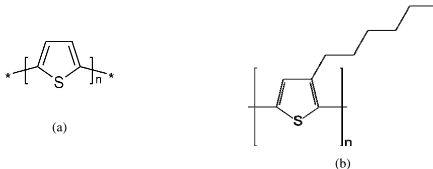
Figure 5.3 Structure formulas : (a) Unsubstituted polythiophenes. (b) Poly(3-hexylthiophene).
