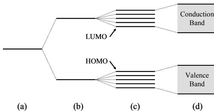
Figure 2.4 Energy diagram of carbon atoms: (a) A single carbon atom. (b) A molecule with two carbon atoms. (c) A large molecule of many carbon atoms. (d) Bulk material.
