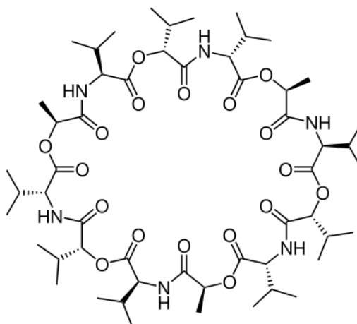
Figure 4.3 Chemical structure of valinomycin.
