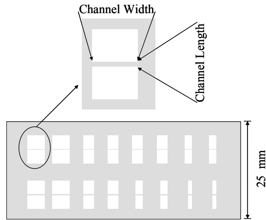
Figure 3.3 A diagram of the shadow mask used for depositing the source and drain electrodes in this research.
