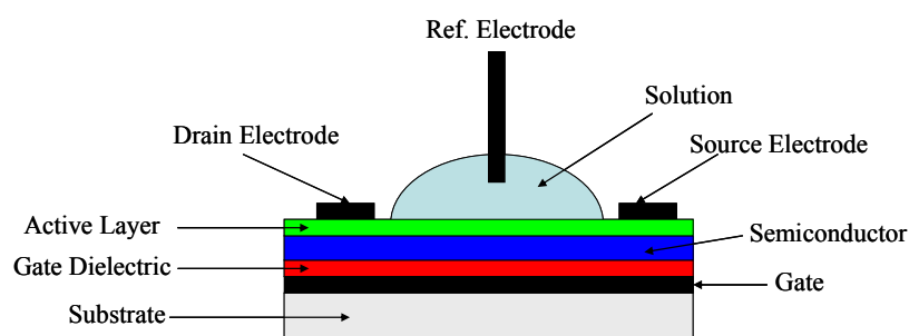
Figure 2.12 Schematic diagram of an ion sensitive organic field effect transistor with the bottom-gate structure.
