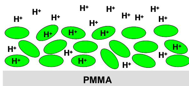
Figure 6.14 Schematic diagram of the multilayer valinomycin when exposed to the acid solutions.
