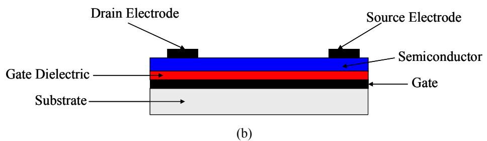
Figure 2.6 Schematic diagrams of thin-film transistors: (a) Top-gate structure. (b) Bottom-gate structure.
