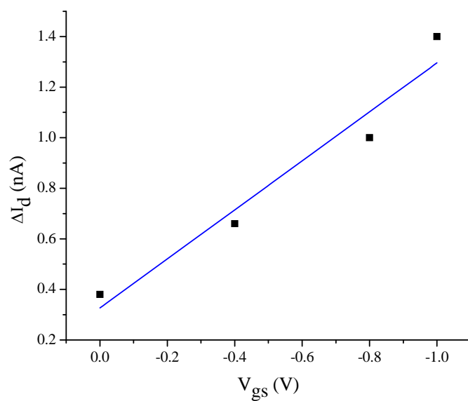
Figure 5.16 \Delta I_d versus V_{gs} , V_{ds} = -0.5 V, the interdigitated ISOFET, in DI water.
