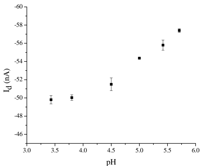
Figure 6.9 The pH response of the interdigitated ISOFET coated with 10 LB layers of pure AA, at room temperature, V_{ds} = -0.2 V and V_{gs} = -0.2 V.
