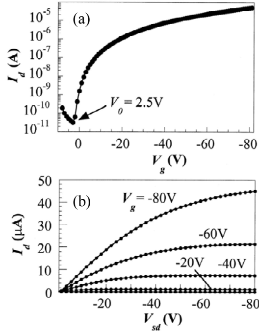
Figure 2.8 (a) Transfer characteristics in the saturation regime. (b) Output characteristics of a typical P3HT FET ( L = 75 \mu\text{m} , W = 1500 \mu\text{m} ) [17].
