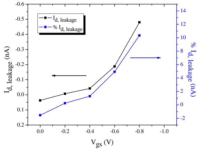
Figure 5.13 Leakage current, I_{d, \text{leakage}} , versus V_{gs} , V_{ds} = 0 V, the standard ISOFET, in DI water.
