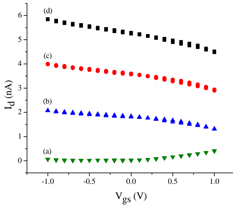
Figure 5.7 Transfer characteristics of the standard ISOFET (Cr/Au/P3HT/650 nm PMMA), varying V_{gs} between -1.0 and 1.0 V, W/L ratio = 40; using (a) V_{ds} 0. (b) V_{ds} -0.5. (c) V_{ds} -1.0. (d) V_{ds} -1.5 V.
