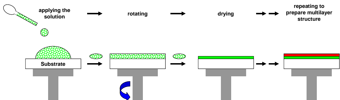
Figure 3.5 Schematic diagram of the spin-coating process.
