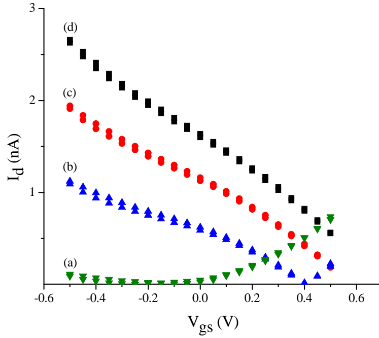
Figure 5.8 Transfer characteristics of the standard ISOFET (Cr/Au/P3HT/150 nm PMMA), varying V_{gs} between -0.5 and 0.5 V, W/L ratio = 40; using (a) V_{ds} 0. (b) V_{ds} -0.2. (c) V_{ds} -0.4. (d) V_{ds} -0.6 V.
