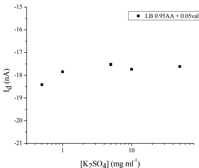
Figure 7.4 pK response of an interdigitated ISOFET with 10 LB monolayers of 95%AA + 5%val.
