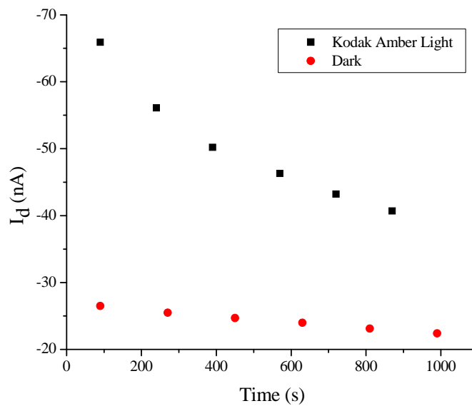
Figure 5.18 Typical responses of the interdigitated ISOFET under steady-state illumination, V_{gs} = 0 V, V_{ds} = -1 V, in DI water.
