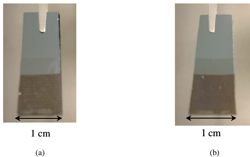
Figure 4.14 (a) DPPA film on arachidic acid/Si wafer, 5 dips of DPPA on 10 AA layers. (b) DPPA film on Cd arachidate/Si wafer, 5 dips of DPPA on 10 CdAA layers.
