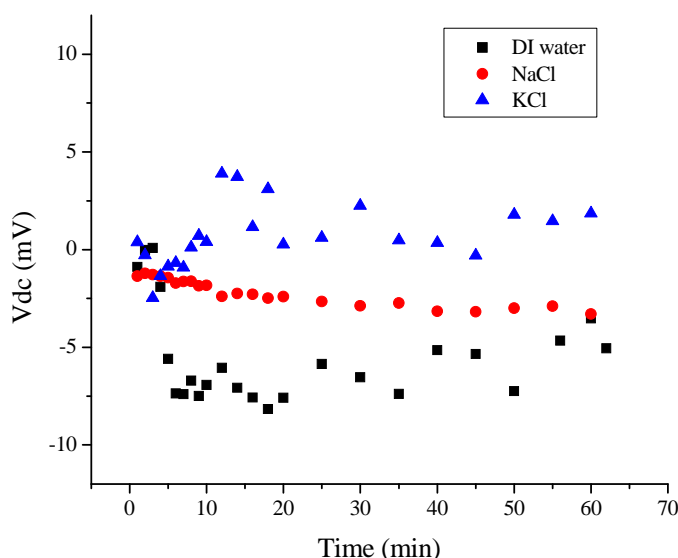
Figure 8.7 Potentials across 0.45 \mu\text{m} porous membrane; the same concentration in both compartments, DI water, KCl (0.01M) and NaCl (0.01M).
