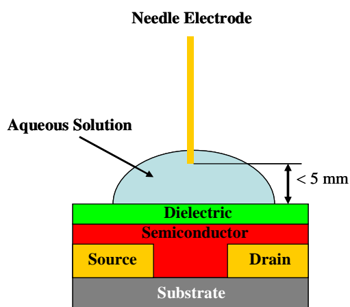
Figure 9.2 Schematic diagram of the measurement configuration using a needle electrode [5,6].
