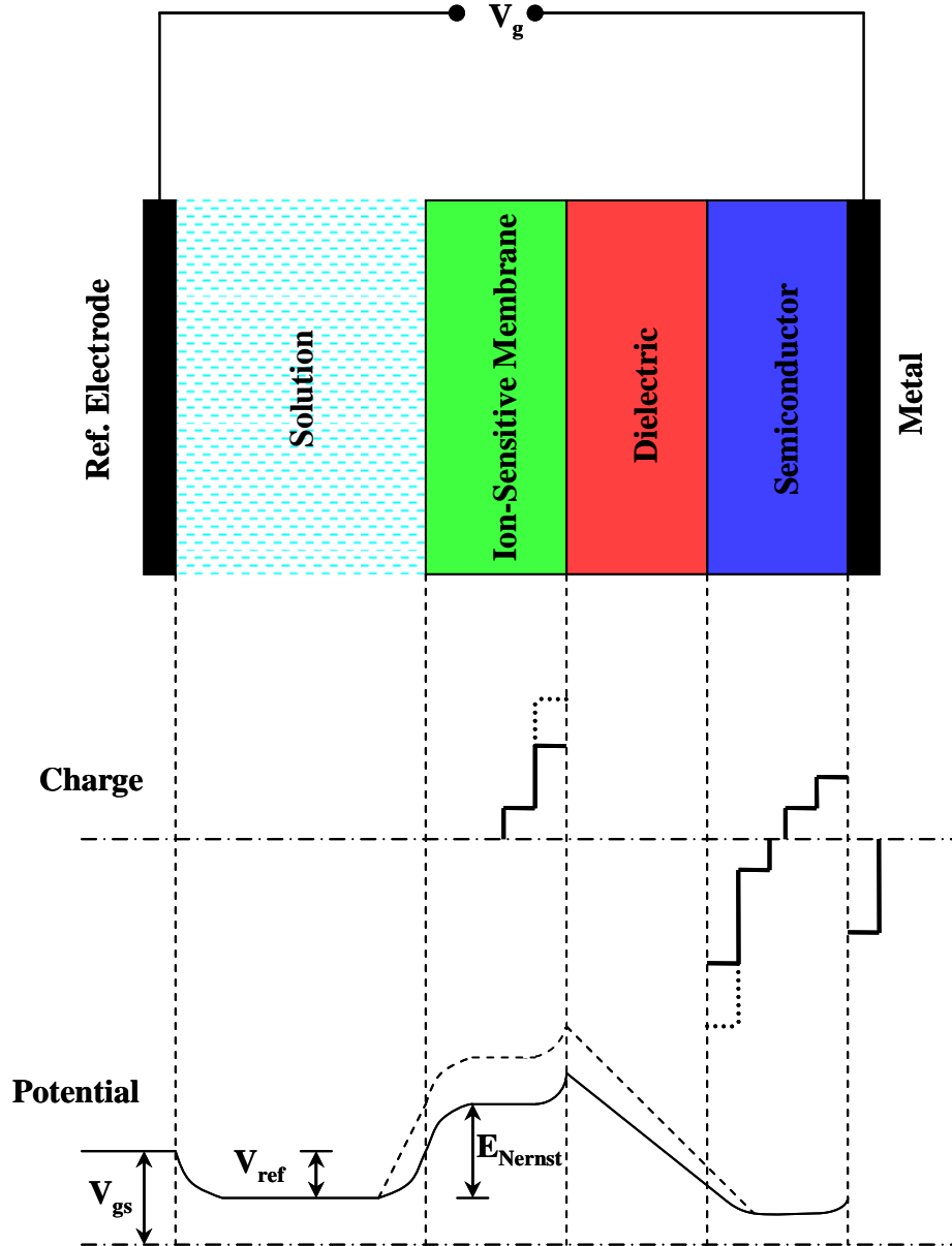
Figure 2.10 Charge and potential distributions across the ISO-FET structure; dashed line represents the distributions when the activity (concentration) of the solution changes [30].
