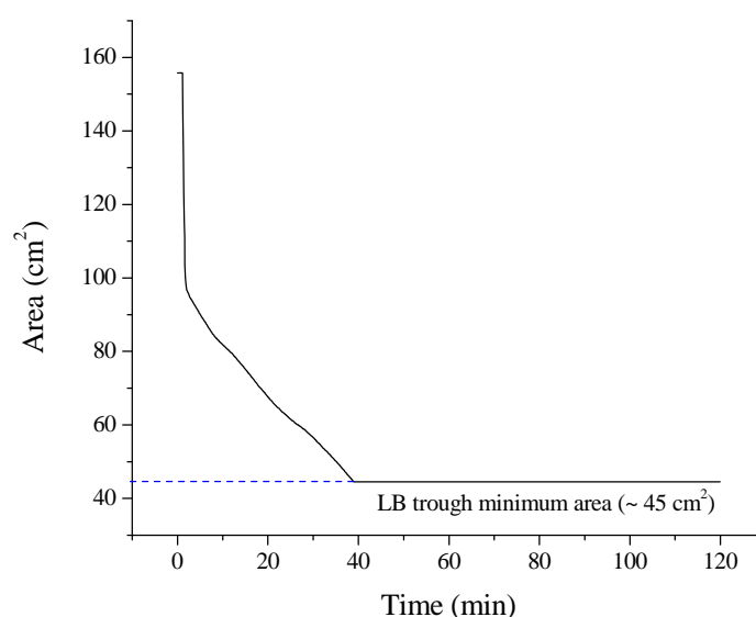
Figure 4.15 Pressure-control profiles of valinomycin; constant surface pressure of 15 \text{ mN m}^{-1}
