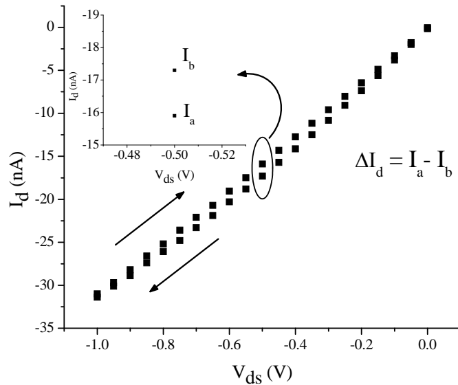
Figure 5.15 Output characteristics of the ISOFET with standard source-drain electrodes, scanning V_{ds} 0\text{ V} \rightarrow -1\text{ V} \rightarrow 0\text{ V} ; V_{gs} = -1.0\text{ V} , in DI water.
