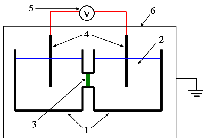
Figure 8.6 Schematic diagram of the measuring system. 1) PTFT compartments. 2) Solutions. 3) Membrane. 4) Electrodes. 5) Voltmeter. 6) Faraday cage.
