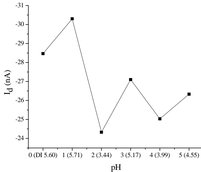
Figure 6.6 Typical sequential responses of the ISOFET in different pH solutions. The structure of the device : Cr/Au/P3HT/PMMA/10 monolayers of 95%AA + 5%val. Measurement in the dark at room temperature.
