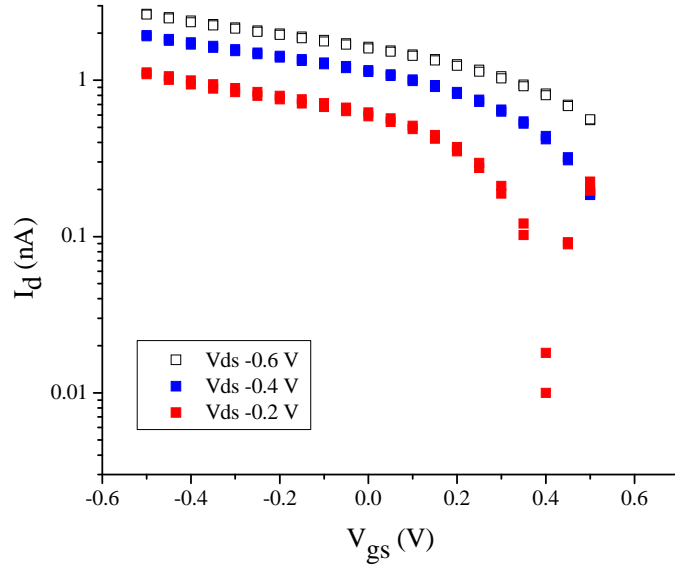
Figure 5.9 Semilogarithmic transfer graphs corresponding to the data in Figure 5.8b, 5.8c and 5.8d.
