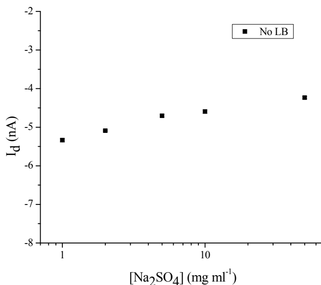
Figure 7.9 pNa response of an uncoated interdigitated ISOFET.
