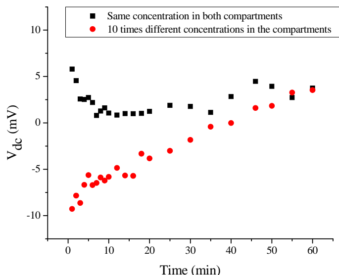
Figure 8.9 Potentials across the 0.45 \mu\text{m} porous membrane coated with 4 LB layers of 95% AA+5% valinomycin; KCl (0.01M) : KCl (0.01M) and KCl (0.01M) : KCl (0.001M).
