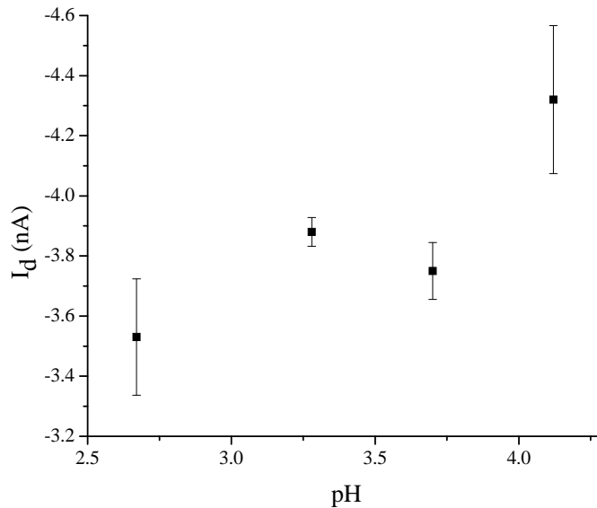
Figure 6.7 The pH response of an uncoated standard ISOFET (W/L ratio = 40) at room temperature. V_{ds} = -0.2 V and V_{gs} = -0.6 V.
