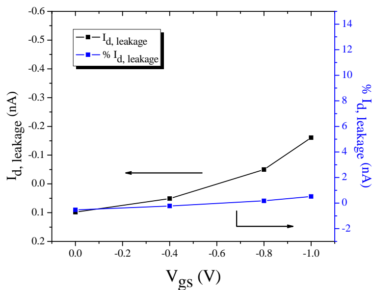
Figure 5.17 Leakage current, I_{d, leakage} versus V_{gs} , V_{ds} = 0 V, the interdigitated ISOFET, in DI water.
