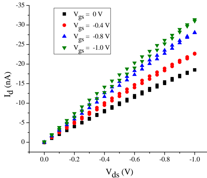
Figure 5.14 The output characteristics of the ISOFET with interdigitated source-drain electrodes; scanning V_{ds} 0 V \rightarrow -1 V \rightarrow 0 V, V_{gs} = 0, -0.4, -0.8, -1.0 V, in DI water, W/L ratio = 880.
