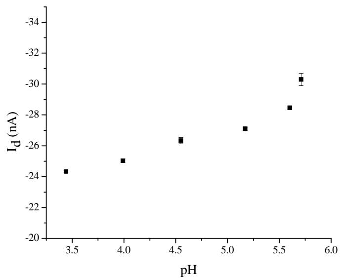
Figure 6.10 The pH response of the interdigitated ISOFET coated with 10 LB layers of 95%AA + 5 % val; at room temperature; V_{ds} = -0.2 V and V_{gs} = -0.2 V.
