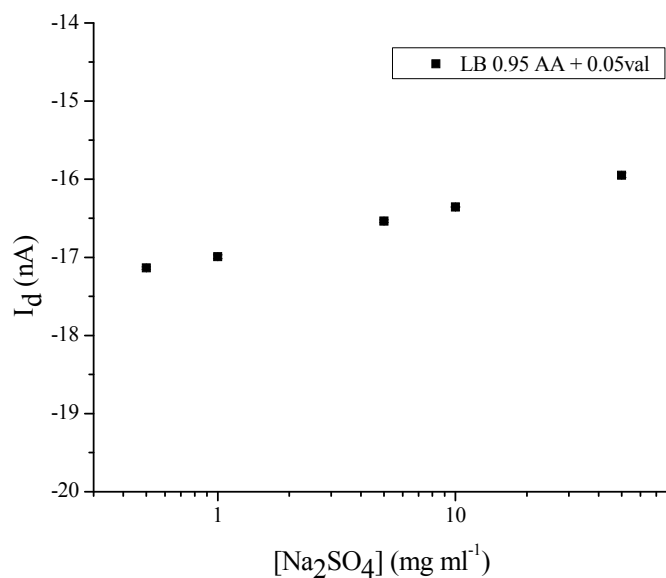
Figure 7.10 pNa response of an interdigitated ISOFET with 10 LB monolayers of 95%AA + 5%val.
