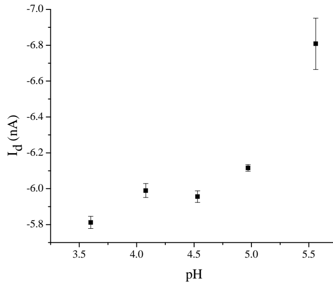
Figure 6.8 The pH response of the uncoated interdigitated ISOFET (W/L ratio = 880) at room temperature. V_{ds} = -0.2 \text{ V} and V_{gs} = -0.2 \text{ V} .
