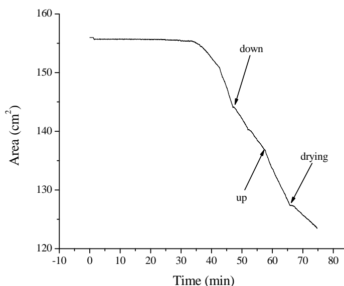
Figure 8.5 Dipping profile of valinomycin on the Millipore 0.45 \mu\text{m} porous membrane.
