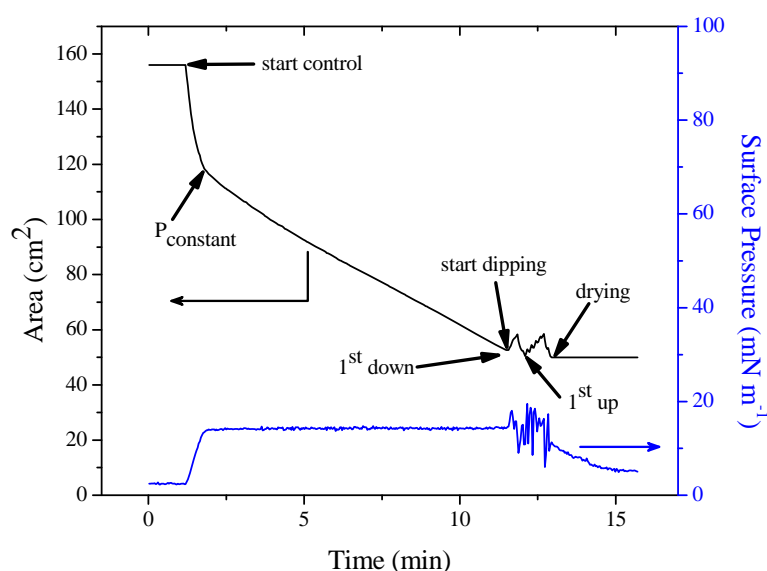
Figure 6.3 Dipping profile of pure valinomycin on an interdigitated ISOFET using DI water as the subphase; at the constant surface pressure of 15 \text{ mN m}^{-1} .
