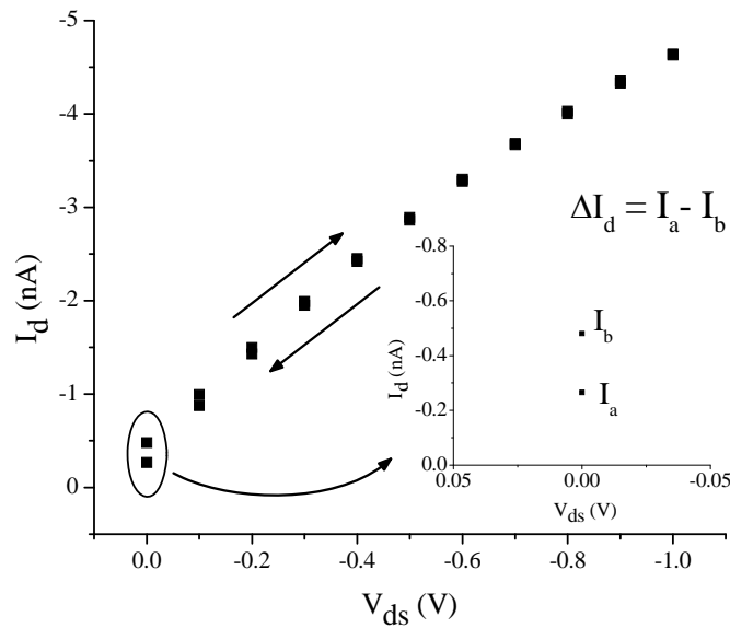
Figure 5.11 Output characteristics of the ISOFET with standard source-drain electrodes; scanning V_{ds} 0\text{ V} \rightarrow -1\text{ V} \rightarrow 0\text{ V} ; V_{gs} = -0.8\text{ V} , in DI water.
