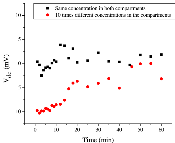
Figure 8.8 Potentials across the uncoated 0.45 \mu\text{m} porous membrane; the same concentration in both compartment (0.01M:0.01M) and 10 times different concentrations (0.01M:0.001M).
