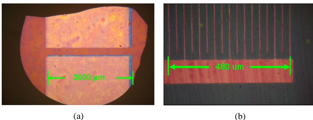
Figure 5.2 Patterns of source and drain electrodes. (a) Standard pattern. (b) Interdigitated pattern.
