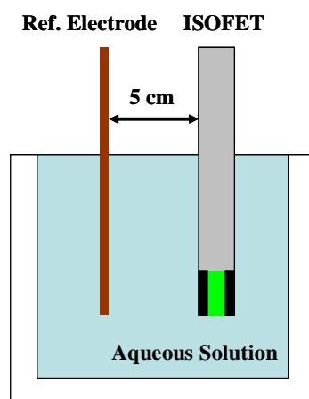
Figure 9.1 Schematic diagram of the measurement configuration using a reference electrode.
