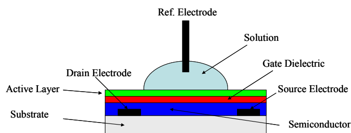
Figure 2.11 Schematic diagram of an ion sensitive organic field effect transistor with a top-gate configuration.
