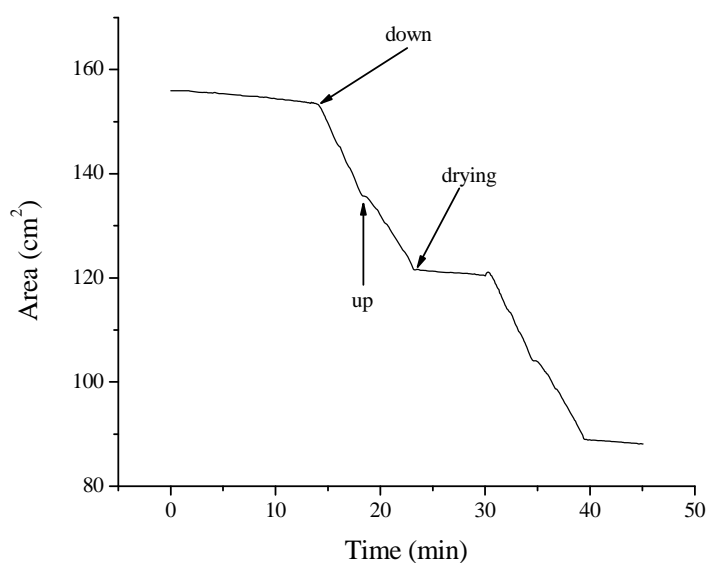
Figure 8.4 Dipping profile of the mixture of arachidic acid and valinomycin (9:1 weight ratio) on the Millipore 0.45 \mu m porous membrane.
