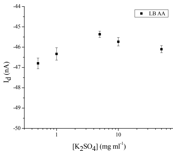
Figure 7.2 pK response of an interdigitated ISOFET with 10 LB monolayers of pure AA.
