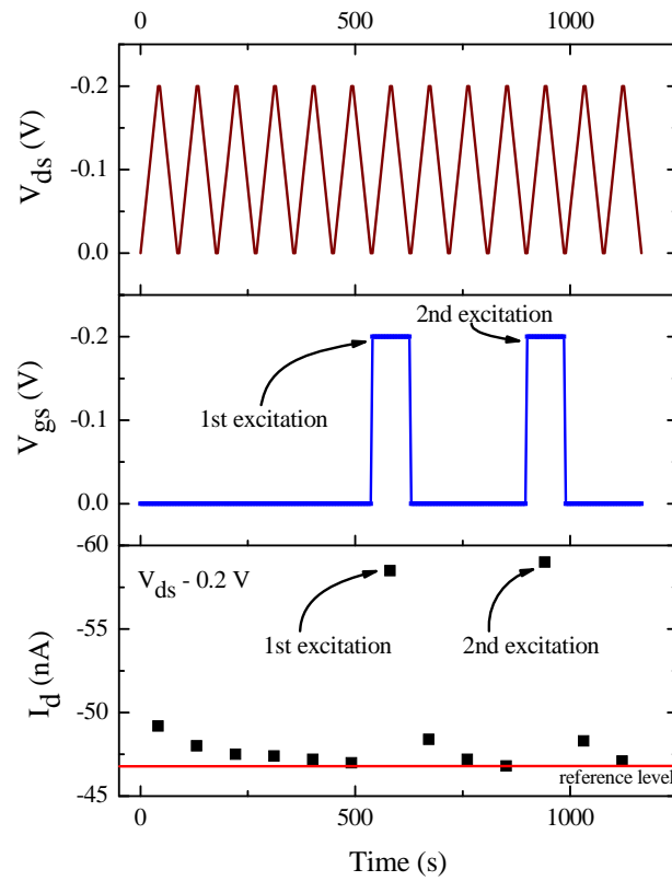
Figure 6.5 Typical responses of the ISOFET in DI water using sequence of the scan in V_{ds} over the range 0 V \rightarrow -0.2 V \rightarrow 0 V. The structure of the device: Cr/Au/P3HT/PMMA/10 AA. Measurement in the dark at room temperature.
