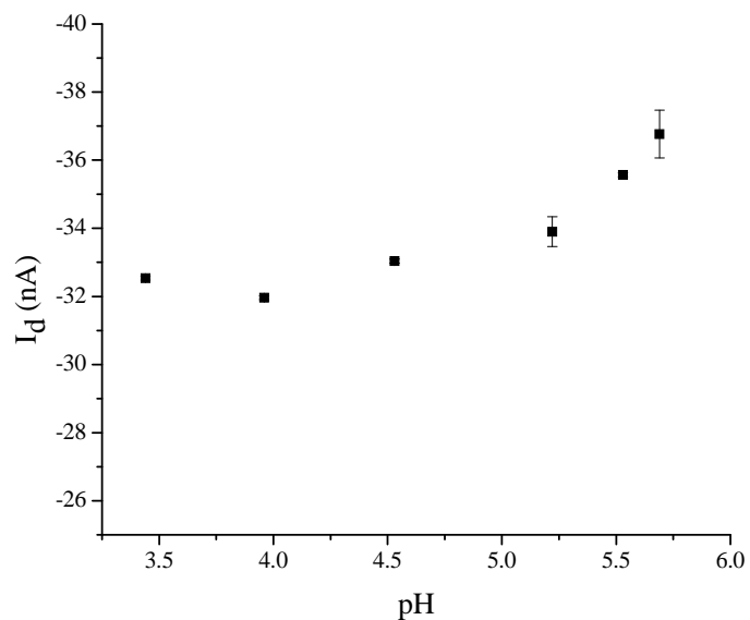
Figure 6.11 The pH response of the interdigitated ISOFET coated with multilayer valinomycin; at room temperature; V_{ds} = -0.2 V and V_{gs} = -0.2 V.
