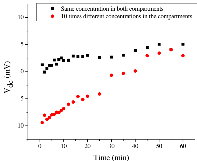
Figure 8.10 Potentials across the 0.45 \mu\text{m} porous membrane coated with 2 LB layers of pure valinomycin; KCl (0.01M) : KCl (0.01M) and (0.01M) : KCl (0.001M).
