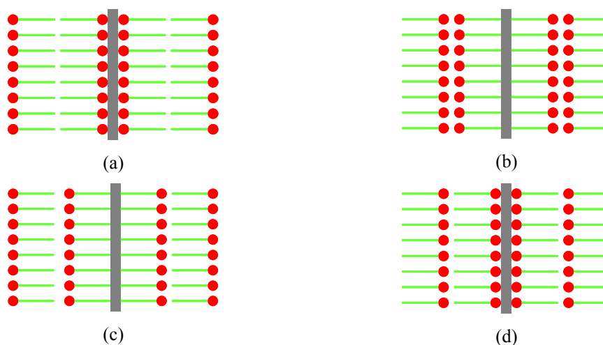
Figure 3.10 (a) Y-type deposition on hydrophilic surface. (b) Y-type deposition on hydrophobic surface. (c) X-type deposition. (d) Z-type deposition.
