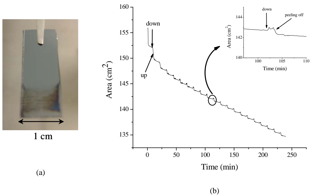
Figure 4.13 (a) DPPA film on Si wafer, 20 dips. (b) Dipping profile of a DPPA film onto Si wafer.
