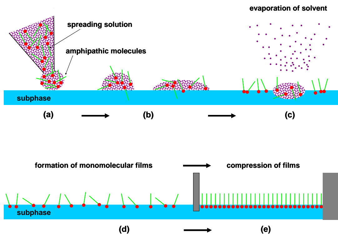
Figure 3.7 Formation of monomolecular film : (a) organic solution dropped onto the subphase, (b) organic molecules spread on the subphase, (c) solvent molecules evaporate, (d) expanded monomolecular films formed on the subphase, (e) condensed film on the subphase.
