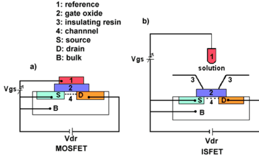
Figure 2.9 Schematic diagram of (a) a MOSFET. (b) An ISFET.
