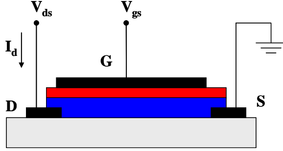
Figure 2.7 A circuit for biasing a thin – film transistor.
