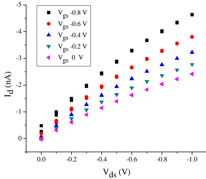
Figure 5.10 Output characteristics of the ISOFET with standard source-drain electrodes; scanning V_{ds} 0 V \rightarrow -1 V \rightarrow 0 V; V_{gs} = 0, -0.2, -0.4, -0.6, -0.8 V; W/L ratio = 40.
