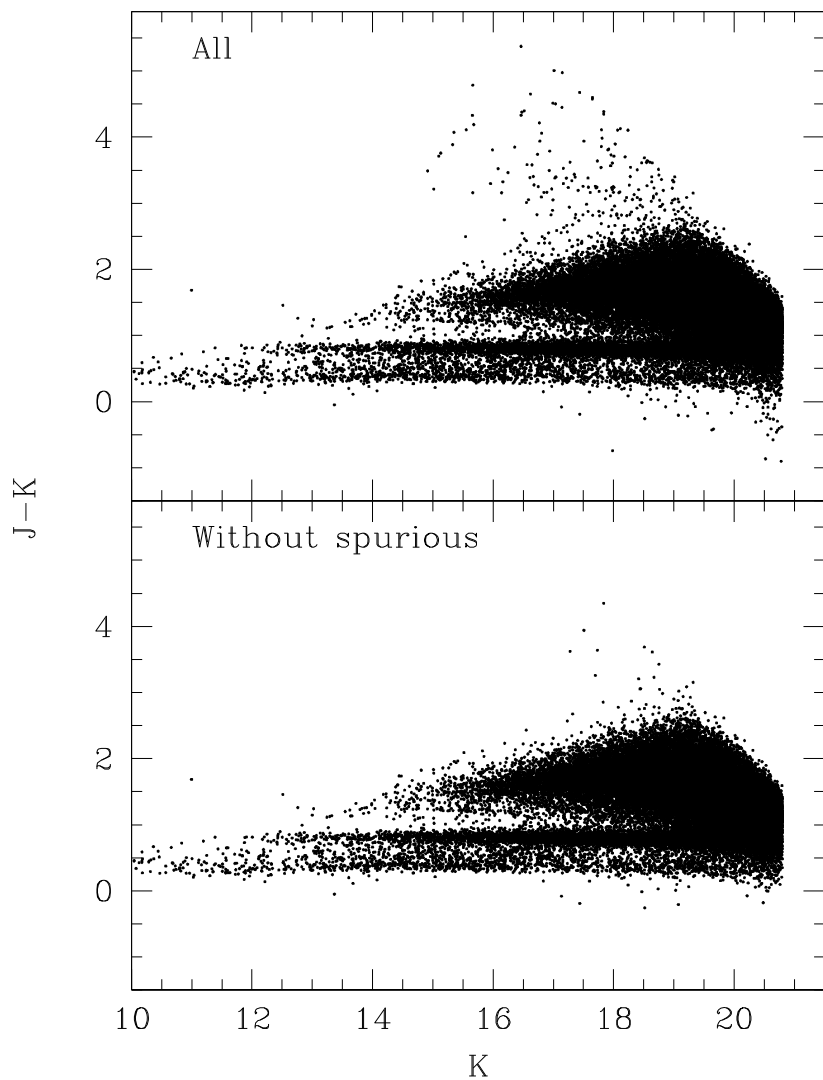
Figure 2.5: The colour-magnitude diagram for one of the SA22 fields before (top) and after (bottom) removing spurious objects.
