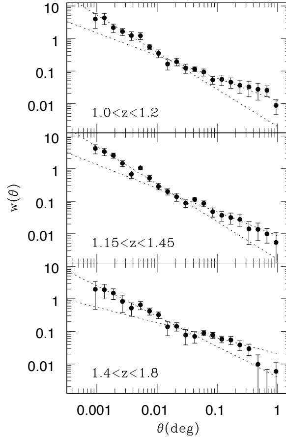
Figure 4.5: Angular two-point correlation functions of DXS/PS1 EROs at 1.0 < z < 1.2 (top), 1.15 < z < 1.45 (middle) and 1.4 < z < 1.8 (bottom). Dotted lines indicate the power-law fits on small and large scales separately.
