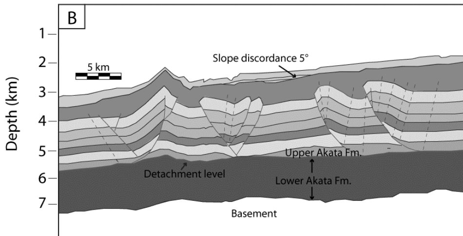
Water column decompacted and youngest thrust restored
