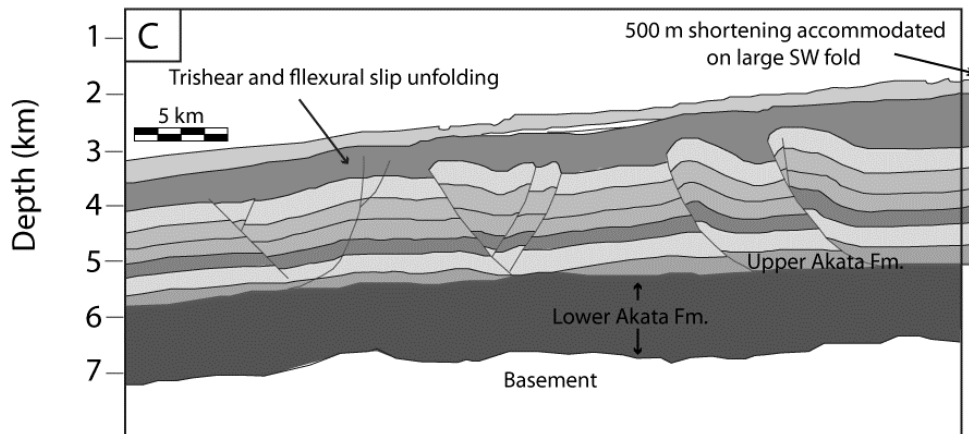
Water column decompacted and youngest thrust restored
