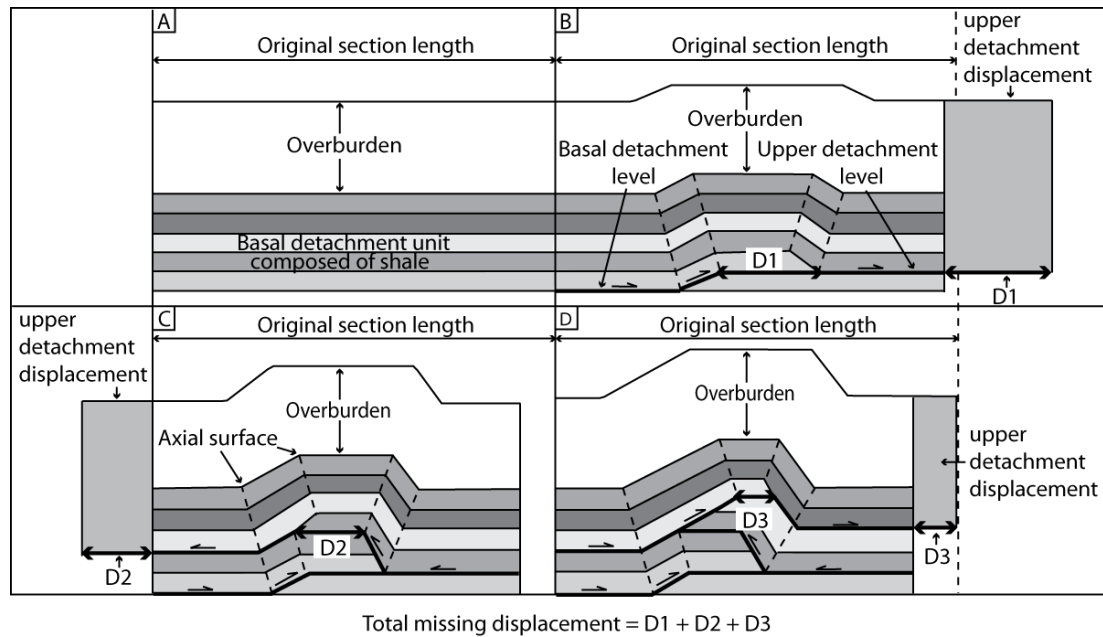
Fig. 4.13. Model showing how thickening of the incompetent unit may occur within the detachment fold core. Thickening in the detachment unit occurs via a series of stacked imbricates thrusts causing fold amplification within the overburden.
