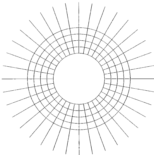
Figure 6.12: Finite/inifnite element mesh model for scattering problem. Inner radius 1, radius of finite/inifnite element interface 2.
