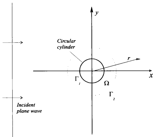
Figure 6.11: Geometry of scattering problem in two dimensions.
