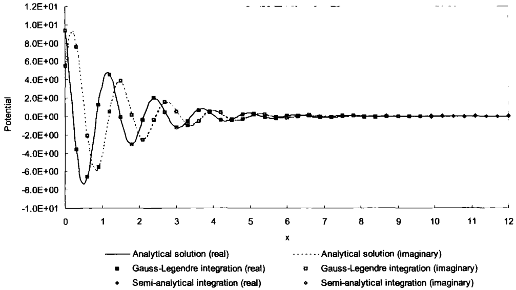
Figure 4.7: Real and imaginary parts of potentials for the rotated evanescent mode, for k = 3 , \alpha = 5 and \beta = 10^\circ , along the centre-line of the domain, y = 0.6 .
