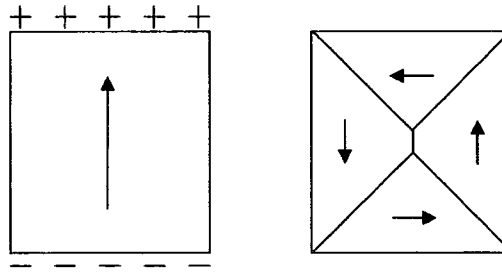
Figure 1-1. Domain formation reduces demagnetisation energy
