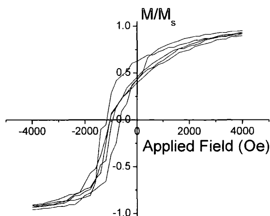
Figure 4-12. Hysteresis loops obtained for different cylindrical clusters of 15 particles
