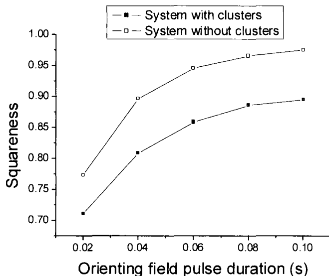
Figure 4-17. Squareness variation with duration of the orienting field pulse
