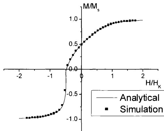
Figure 3-4. Analytical and simulated hysteresis loops of non-interacting Stoner-Wohlfarth particle systems
