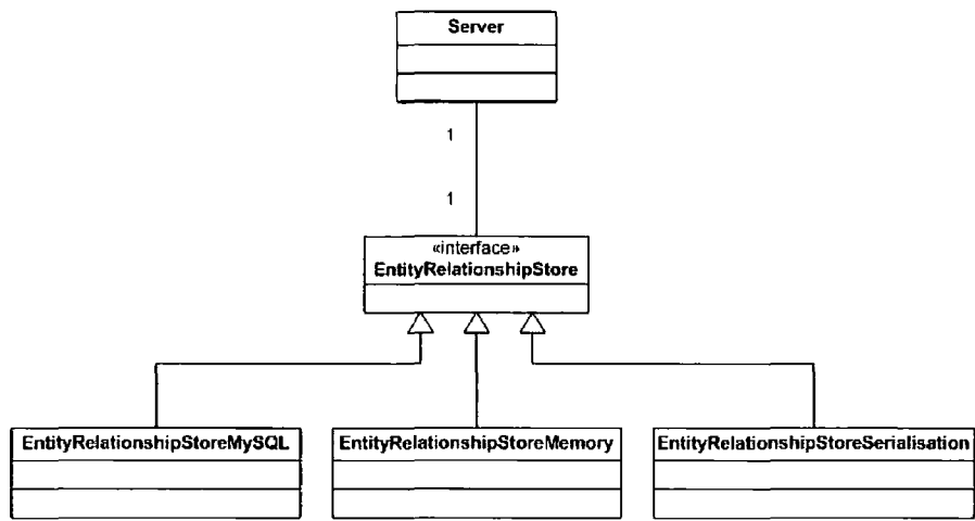
Figure 5-5 EntityRelationshipStore static UML diagram
