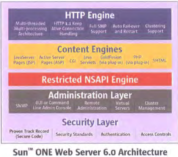
Figure 2-2 Sun™ ONE web server architecture
