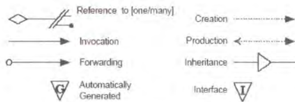
Figure 4-9 Additional LePUS symbols
