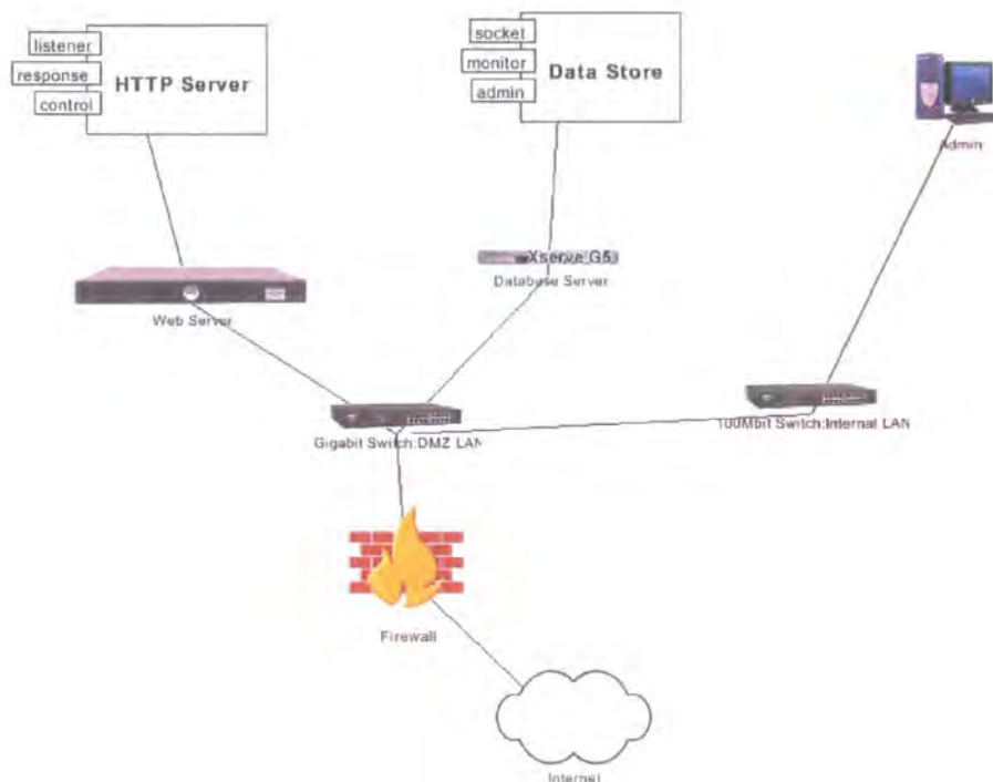
Figure 8-9 Deployment View
