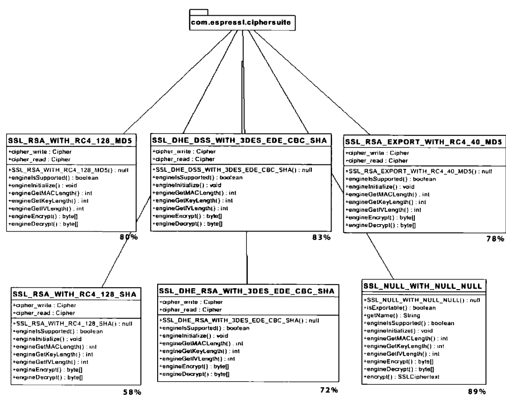
Figure 8-4 Package view
