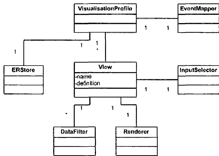
Figure 8-1 ArchVis view model
