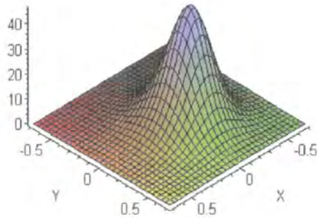
Figure 4.3: Example 4.4 — \|\Phi\|^2 for various values of s .
