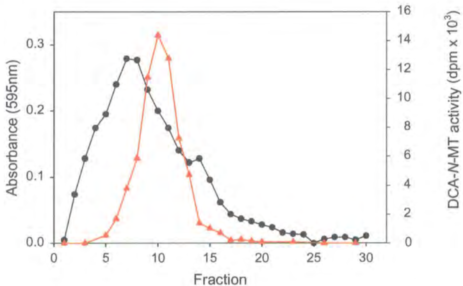
Figure 4.16: Elution profile of DCA-N-MT from a Sephacryl S-100 column.
