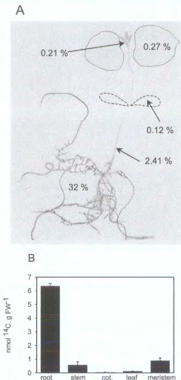
Fig. 2. Distribution of radiolabel in soybean plant fed [ 14 C]-DCA through the root medium. Hydroponically-grown, 10 day-old soybean seedlings were treated with 45.2 nmol (37 kBq) [UL- 14 C]-3,4-dichloroaniline. After 3.5 days, plants were analysed by phosphorimaging (A). Radioactivity in the dissected plant parts was quantified by LSC and the results expressed as % of the original dose (A) and nmol of [ 14 C]-DCA equivalents g -1 FW (B), with results showing the means of duplicated experiments ± S.E.
