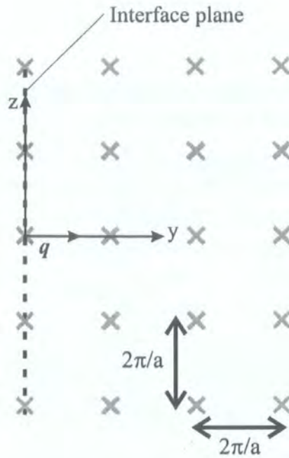
Figure A-2: Square lattice in reciprocal space.
