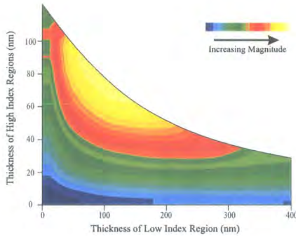
Figure 3.7: Plot of the change in the difference between the upper and lower guided mode propagation constants due to a 1 nm wavelength increase. The upper guide configuration is given by the two axes. The lower guide thickness is the required value for an athermal structure when combined with the specified upper guide configuration.
