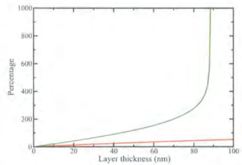
Figure 2.12: Effect of layer 4 manufacturing tolerances on a low refractive index ( n = 1.34 ) film with a variety of thicknesses (actual). The graphs show the resolved (calculated) thicknesses with red lines indicating the upper limit, green lines the lower limit and black lines the original structure. The left-hand column shows actual values and the right-hand column percentage discrepancies. The top figures (a) are for the thickness tolerance, the middle (b) for the refractive index tolerance and the lower (c) for a combined refractive index and thickness tolerance.
