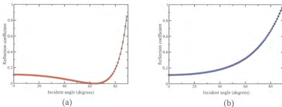
Figure 7.6: Fresnel Equations plotted for the TM (a) and TE (b) polarisations. The black curve represents values calculated from the Fresnel equations and the circles, red for TM and blue for TE, the results generated by the interface matching calculations. Exact agreement may be seen for the reflection at the interface with uniform block ( n = 2 ).
