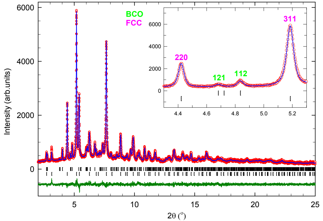
Fig 3.7: Observed (open red circles) and calculated (blue line) data of the room temperature synchrotron powder X-ray diffraction pattern for the sample with nominal composition Rb 0.50 Cs 2.50 C 60 . The upper bars represent the positions of the Bragg reflections of the BCO phase and the lower ones of the FCC phase. The wavelength was \lambda = 0.39988(4) Å.
