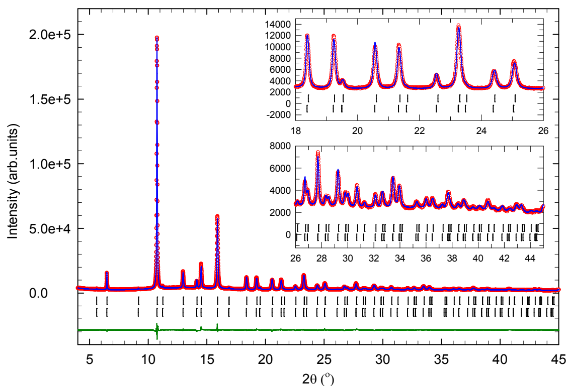
Fig 5.30: Observed (open red circles) and calculated (blue line) data of the 20 K synchrotron powder X-ray diffraction pattern for \text{NaKCsC}_{60} . The upper bars represent the positions of the Bragg reflections for the spherically disordered Fm\bar{3}m phase, and the lower bars represent the merohedral Fm\bar{3}m phase. The wavelength is \lambda = 0.80007(6) \text{ \AA} .
