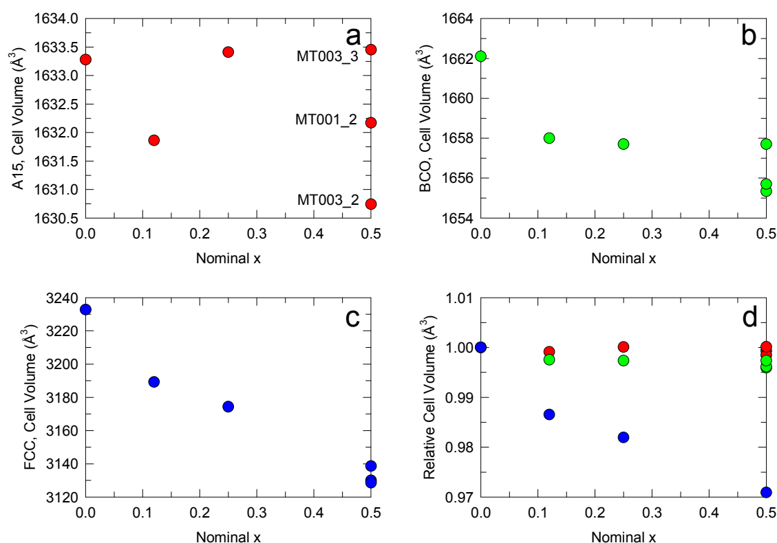
Fig 4.12: Changes in unit cell volume with nominal Rb content, x in the \text{Rb}_x\text{Cs}_{3-x}\text{C}_{60} series. Panels a, b, c show the corresponding evolution for the A15, BCO, and FCC phase, respectively. Panel d depicts the
