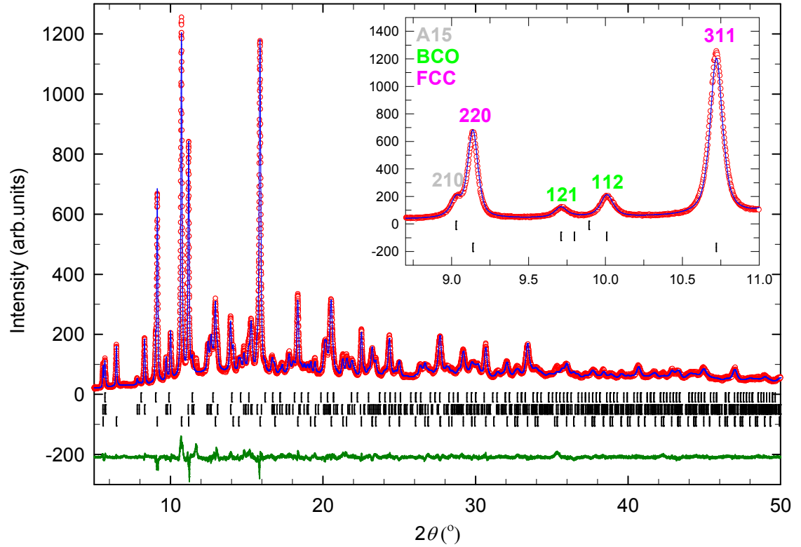
Fig 3.16: Observed (open red circles) and calculated (blue line) data of the 12 K synchrotron powder X-ray diffraction pattern for the sample with nominal composition \text{Rb}_{0.12}\text{Cs}_{2.88}\text{C}_{60} . The upper bars represent the positions of the Bragg reflections of the A15 phase, the middle ones of the BCO phase and the lower ones of the FCC phase. The wavelength is \lambda = 0.826028(1) \text{ \AA} .
