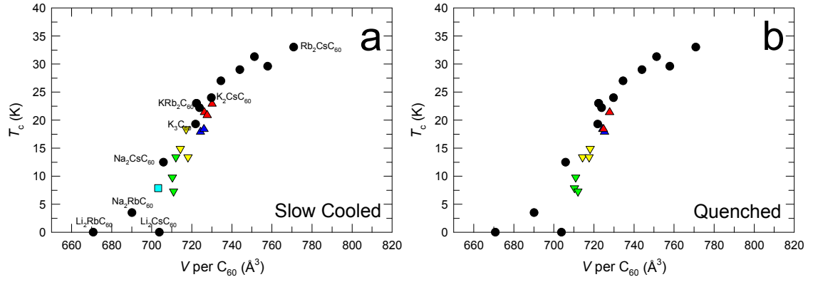
Fig 5.59: Change in T_c with V per C_{60} at room temperature for both (a) slow cooled and (b) quenched samples. (a+b) Down (Up) triangles represent the disordered (merohedral) Fm\bar{3}m model, squares Pa\bar{3} . Red accounts for the single phase merohedral Fm\bar{3}m model. Yellow (Blue) accounts for the disordered (merohedral) Fm\bar{3}m phase of the two-phase materials. The black markers represent a silhouette of literature values for the T_c vs V per C_{60} of other Fm\bar{3}m materials. The T_c 's of the two-phase materials are attributed to whichever is the majority phase.
