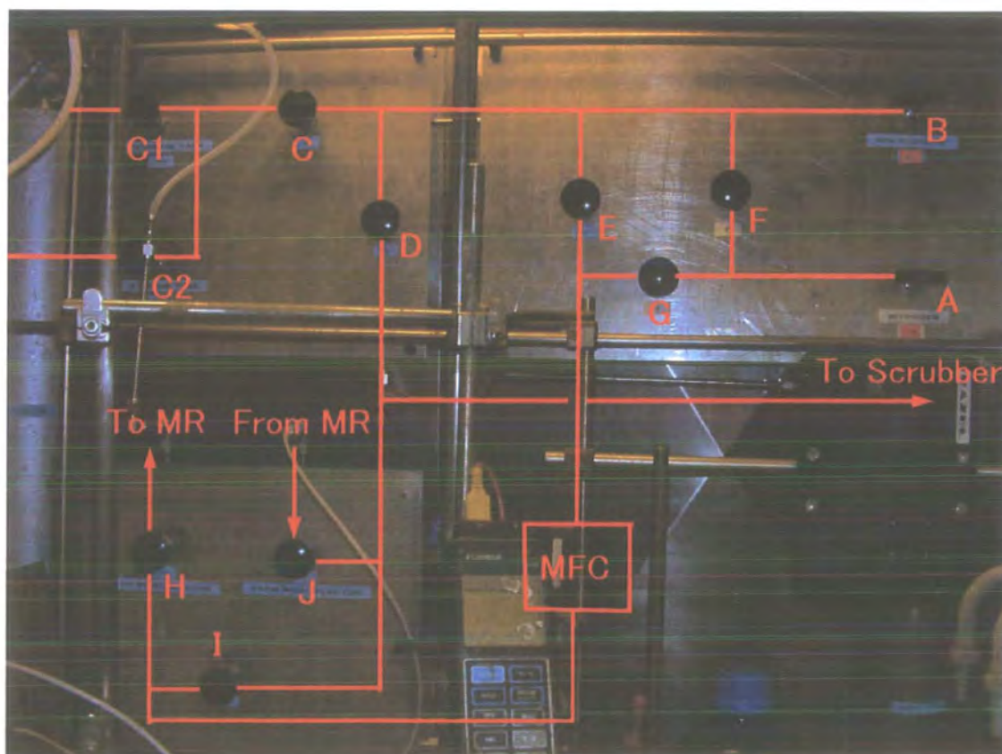
Fig 31 (valves)
