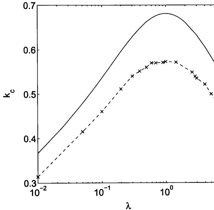
Figure C.5: Comparison of the critical parameter k_c defined in Eq. (C.16) as a function of the asymmetry parameter \lambda obtained by the variational method (solid line) presented in subsection C.2.2 and by numerical solution of the GPE (2.27) (dashed line) presented in Chapter 7.
