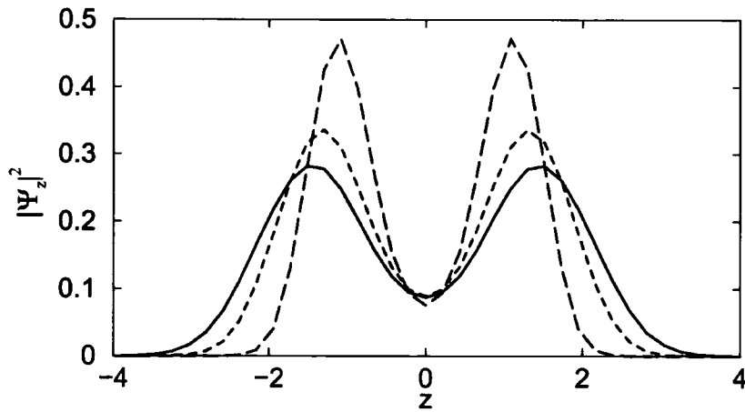
Figure 6.7: Density distributions |\Psi_z|^2 along the z -axis for the \Psi_g for fixed g_{3D} = 10\pi and different geometries: solid corresponds to the geometry shown in Fig. 6.6(a), dashed to the one in Fig. 6.6(b) and finally long dashed to the one in Fig. 6.6(c).
