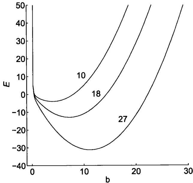
Figure C.1: Energy for bosons interacting with attractive forces, as a function of the condensate size b for different values of |g_{1D}| = 10, 18, 27 . The energy functional has always minima and the condensate is always stable in one dimension.
