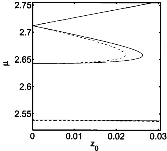
Figure 3.8: Comparison between the exact (solid) and the two-state model (dashed) eigenenergies, \mu , as a function of the barrier displacement, z_0 , for h = 4 \hbar \omega_{\perp} and g_{1D} = 0.5 .
