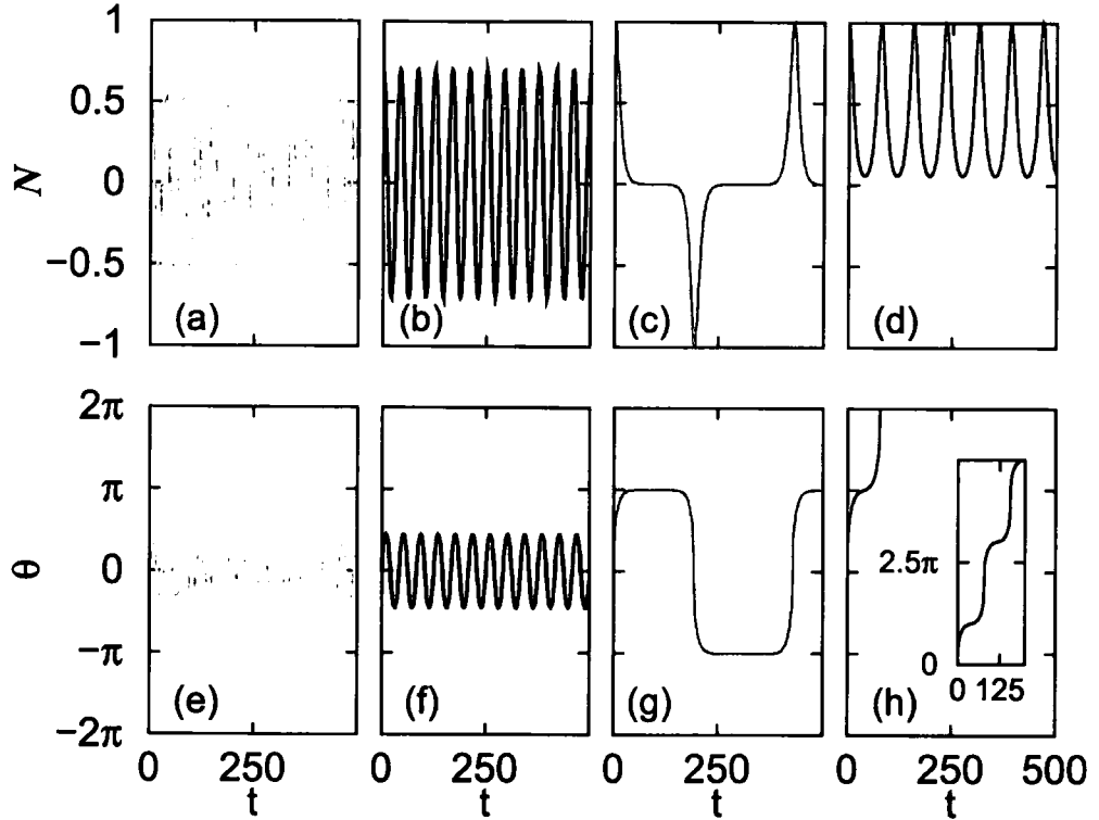
Figure 4.3: (a)-(d) The fractional population difference, N , and (e)-(h) the corresponding phase difference, \theta , as a function of time ( \omega_{\perp}^{-1} ) for E_J = 0.1\hbar\omega_{\perp} , E_C = 0.22\hbar\omega_{\perp} and \theta(0) = 0 in a symmetric trap ( \Delta = 0 ). In (a) and (e) N(0) = 0.5 , (b) and (f) N(0) = 0.7 , (c) and (g) N(0) = N_c = 0.99585919488 and finally (d) and (h) N(0) = 0.996 . The phase difference \theta as a function of time is plotted inset in (h).
