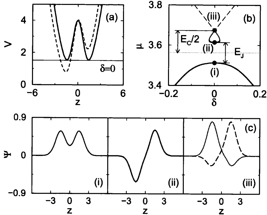
Figure 3.9: Double well potential with corresponding eigenenergies and eigenstates. (a) Schematic geometry of the total confining potential in the axial direction for a Gaussian barrier (height h = 4 \hbar\omega_{\perp} , waist w = a_{\perp} ) located at the centre of the trap. Plotted are the symmetric ( \delta = 0 , solid line) and asymmetric ( \delta = 0.5 \hbar\omega_{\perp}/a_{\perp} , dashed line) cases. (b) Eigenenergies for the double-well as a function of the potential gradient \delta indicating the self-interaction energy, E_C , and the Josephson coupling energy, E_J . The horizontal dotted grey line corresponds to the zero energy of the two-state model. The parameters used here are g_{3D} = \pi and spherical trap geometry ( \lambda = 1 ) corresponding to E_C = 0.220 \hbar\omega_{\perp} and E_J = 0.102 \hbar\omega_{\perp} . (c) Eigenstates at the centre of the trap: (i) ground state (lower solid line), (ii) anti-symmetric first-excited state with equal population in both wells (thick solid line), (iii) first excited state with unequal populations, having more population in left well (dotted), or in right well (dashed).
