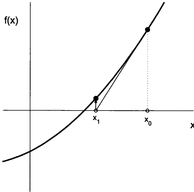
Figure A.1: Newton's method for finding root of an one dimensional function: start with an initial guess for the root at x_0 calculate the derivative at that point to find the next guess of the root.
