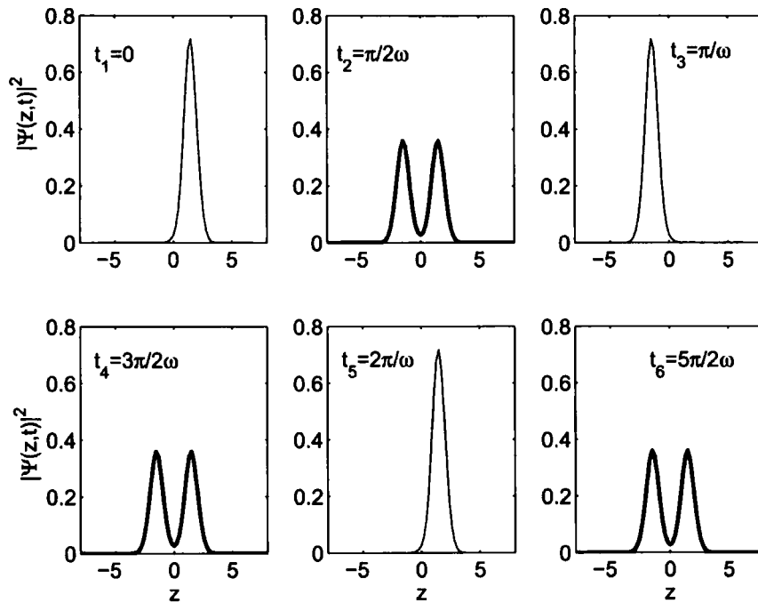
Figure 4.2: Coherent density oscillations of a wavefunction obtained by interference of the ground and first excited states in a double-well potential. The period of the motion is 2\pi/\omega .
