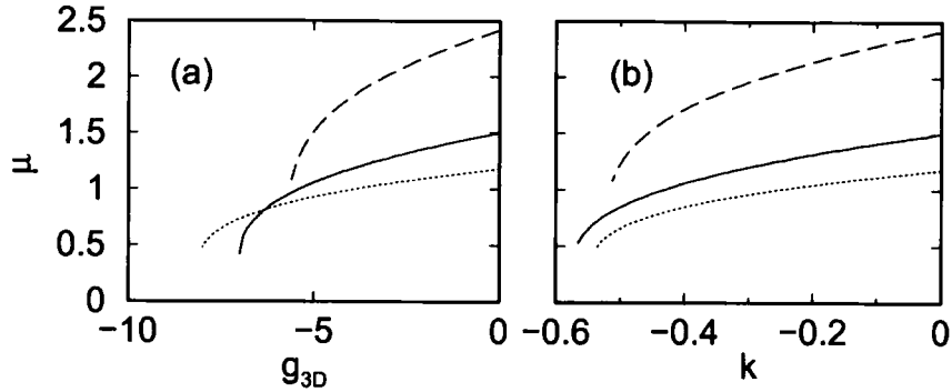
Figure 7.2: Eigenenergy value \mu , for the ground state for a spherical, \lambda = 1 (solid), a “pancake”, \lambda^2 = 8 (dashed) and “cigar” trap, \lambda^2 = 1/8 (dotted line) as a function of: (a) the nonlinear parameter g_{3D} and (b) the parameter k = \mathcal{N}|a|/a_0 .
