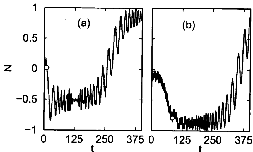
Figure 6.12: Evolution of fractional population difference N as a function of time for initial states prepared by phase imprinting ( |\alpha| = \hbar\omega_{\perp} , \tau_0 = 3 \omega_{\perp}^{-1} ). The grey and black curves correspond respectively to the absence of a potential gradient (i.e. symmetric double well), and the addition of a potential gradient \delta = R(t - \tau_1) increased linearly at rate R = 2 \times 10^{-3} (\hbar\omega_{\perp}^2/a_{\perp}) from time \tau_1 , with this time indicated by the open circles. (a) \alpha = \hbar\omega_{\perp} , \tau_1 = 10 \omega_{\perp}^{-1} and (b) \alpha = -\hbar\omega_{\perp} , \tau_1 = 85\omega_{\perp}^{-1} . Other parameters as in Fig. 6.1.
