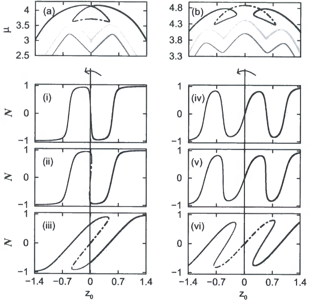
Figure 5.2: The eigenenergies \mu for (a) the first and (b) the second excited states for large (black) and low interactions (grey) lines as a function of the barrier displacement z_0 for g_{1D} := 0 , (dark grey), 0.5, (light grey) and 5 (black). The eigenenergies for g_{1D} = 0 and 0.5 have been shifted along the \mu -axis by +0.1 \hbar\omega_{\perp} and +0.3 \hbar\omega_{\perp} respectively. The fractional population difference N for the first (i)-(iii) and (iv)-(vi) the second excited state respectively as a function of z_0 for h = 4 \hbar\omega_{\perp} . In (i) and (iv) g_{1D} = 0 , (ii) and (v) g_{1D} = 0.5 and finally (iii) and (vi) g_{1D} = 5 . Bold lines correspond to stationary solutions of Eq. (3.1) and black lines are the symmetric projections in the -z_0 -axis.
