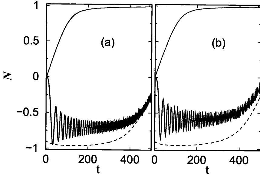
Figure 6.9: Comparison between the evolution of fractional population difference N (a) in three and (b) one dimension as a function of time ( \omega_{\perp}^{-1} ). In g_{3D} = \pi and \lambda = 1 whereas in (b) g_{1D} = 0.5 . Solid bold (dashed) lines indicate corresponding eigenstate populations for the ground (first excited) state. Other parameters same as in Fig. 6.1.
