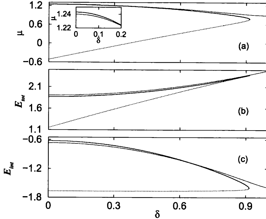
Figure 7.9: (a) The eigenstates \mu , (b) the total energy E_{tot} and (c) the interaction energy E_{int} as a function of the potential gradient \delta for the \Psi_g (solid black), the \Psi_e (grey) and the “self-trapped” ground (dotted lines) states. Inset in (a) we plot the eigenstates \mu for small \delta . Other parameters: g_{1D} = -4 and h = 4 \hbar\omega_{\perp} .
