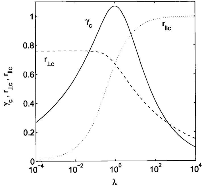
Figure C.4: Critical values of the nonlinear parameter \gamma_c (solid) and the lengths r_{\parallel c} (dotted) and r_{\perp c} (dashed lines) as a function of the asymmetry parameter \lambda (in units \hbar\omega ) for bosons interacting with attractive forces in units defined by the two harmonic oscillator lengths b_{\parallel 0} and b_{\perp 0} . Those results are also presented in [76].
