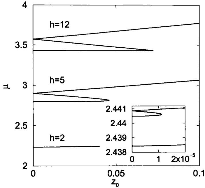
Figure 3.6: The energy eigenvalue, \mu , as a function of the barrier displacement, z_0 , for e_1 with g_{1D} = 0.5 and barrier heights h = 2, 5 , and 12 \hbar\omega_{\perp} . The energy curves for h = 2.91 \hbar\omega_{\perp} and h = 2.92 \hbar\omega_{\perp} are shown inset. The loop structure appears at h = 2.916 \hbar\omega_{\perp} .
