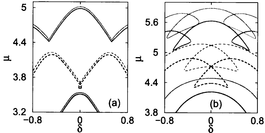
Figure 3.11: The energy eigenvalue, \mu , as a function of the potential gradient \delta , for the ground state g and the first two excited states, e_1 (dashed) and e_2 (dotted) lines in one (light grey) and three dimensions (black) lines, with h = 4 \hbar \omega_{\perp} and (a) g_{1D} = 0.5 and g_{3D} = \pi and (b) g_{1D} = 5 and g_{3D} = 10\pi . In both cases in three dimensions, we assume a spherical trap, \lambda = 1 .
