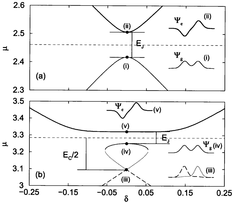
Figure 7.6: Eigenenergies for the double-well for (a) a noninteracting and (b) attractive Bose gas as a function of the potential gradient \delta indicating the self-interaction energy, E_C , and the Josephson coupling energy, E_J in each case. The horizontal dotted grey line corresponds to the zero energy of the two-state model. The values of the nonlinearity used here are (a) g_{3D} = 0 and (b) g_{3D} = -\pi corresponding to (a) E_J = 0.089 \hbar\omega_\perp and E_C = 0 and (b) E_J = 0.071 \hbar\omega_\perp and E_C = -0.379 \hbar\omega_\perp . The eigenstates at the centre of the trap are also shown in each case. We assume a spherical trap geometry ( \lambda = 1 ), and a Gaussian barrier of height h = 4 \hbar\omega_\perp located at the centre of the trap.
