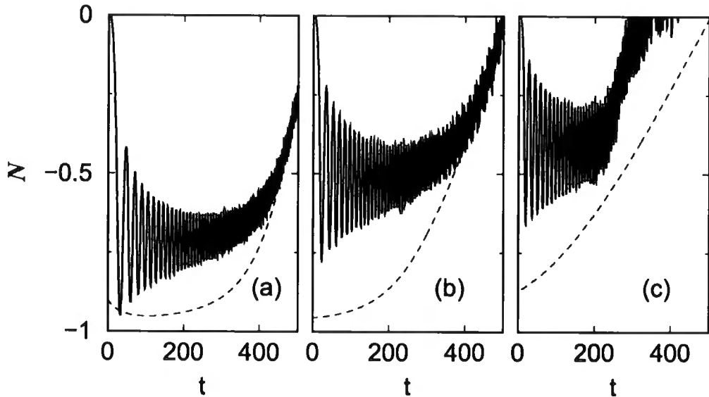
Figure 6.5: Evolution of fractional population difference N as a function of time ( \omega_{\perp}^{-1} ) for identical trap configurations ( \lambda = 1 , h = 4 \hbar \omega_{\perp} and R = 10^{-3} (\hbar \omega_{\perp}^2 / a_{\perp}) ) and increasing nonlinearity (a) g_{3D} = \pi , (b) 4\pi and (c) 10\pi . Dashed lines indicate corresponding eigenstate populations for the first excited state.
