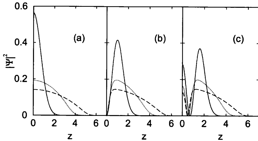
Figure 2.1: Condensate density |\Psi|^2 , against the position z , for (a) the ground, (b) first and (c) second excited states for positive values of the nonlinear constant g_{1D} = : 0, (solid), 40, (dotted) and 100 (dashed) lines.
