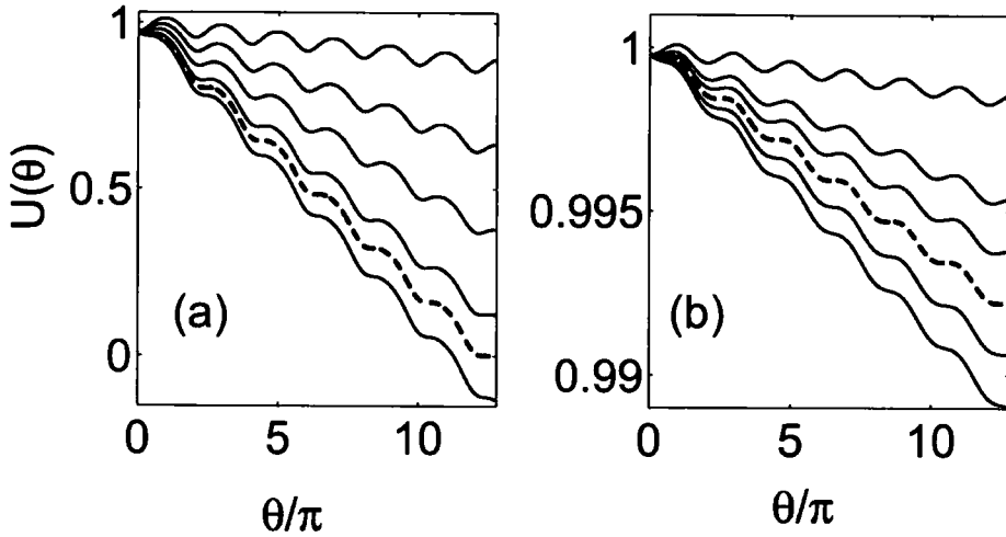
Figure 5.6: Plots of the washboard potential as a function of \theta/\pi for different velocities v , for g_{1D} = 0.5 and (a) h = 4 \hbar\omega_{\perp} and (b) h = 12 \hbar\omega_{\perp} . For v = v_c the washboard potential has no bound states (dashed lines). For the parameters used here, Eq. (5.4) gives v_c = 0.008 a_{\perp}\omega_{\perp} in (a) and 5 \times 10^{-5} a_{\perp}\omega_{\perp} in (b). In (a) v(\times 10^{-3} a_{\perp}\omega_{\perp}) := 1, 3, 5, 7, 8, 9 whereas in (b) v(\times 10^{-5} a_{\perp}\omega_{\perp}) := 1, 3, 4, 5, 7, 9 .
