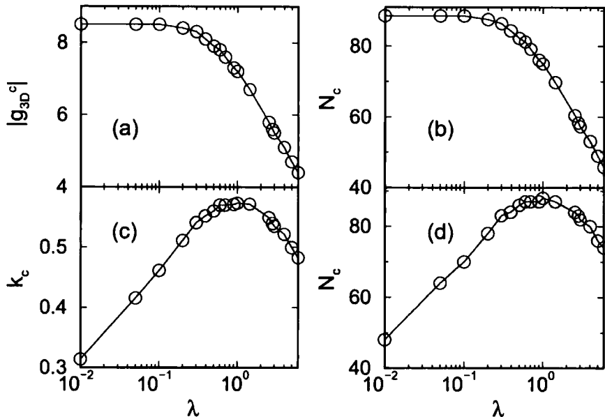
Figure 7.3: Plots of the critical parameters, (a) nonlinear constant g_{3D}^c and (c) k_c , Eq. (7.1) and the corresponding \mathcal{N}_c in (b) and (d) as a function of \lambda .
