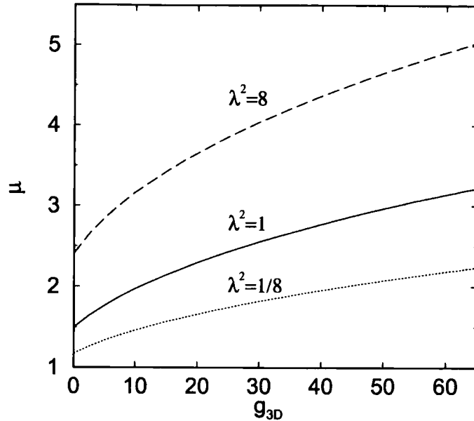
Figure 2.5: Chemical potential \mu , for the ground state for positive values of the nonlinear constant g_{3D} for \lambda^2 = 8 (dashed), 1, (solid) and 1/8 (dotted) lines.
