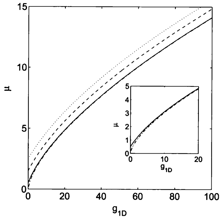
Figure 2.2: Chemical potential \mu , for the ground state, (solid), the first, (dashed) and the second (dotted lines) excited states for positive values of the nonlinear constant g_{1D} . The chemical potential for the TF-limit, Eq. (2.24), is also plotted as dashed-dotted line. Inset the chemical potential for the ground (solid) and the TF-limit (dashed-dotted) lines.
