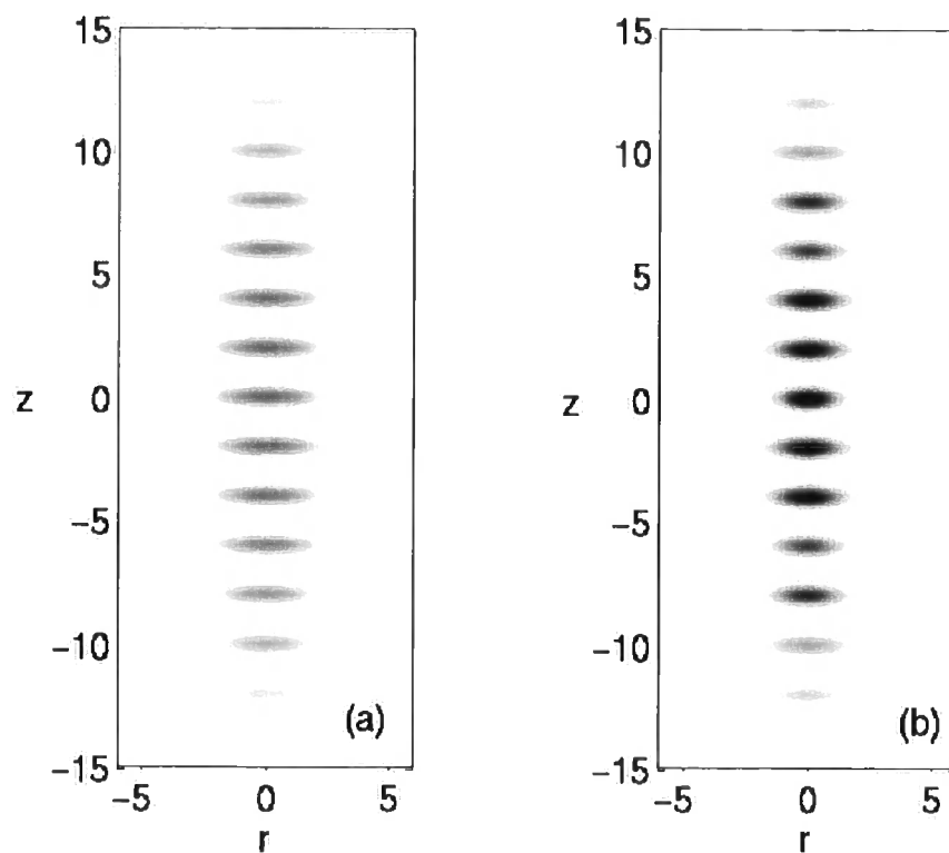
Figure 8.7: Images showing a cross-section of the condensate density at (a) t = 175 \omega_{\perp}^{-1} and (b) t = 625 \omega_{\perp}^{-1} . (a) shows that the potential (Eq. (8.2)) creates lattice along the axial direction. (b) shows the response of the condensate to the sudden change to attractive interactions, g_{3D} = -18 .
