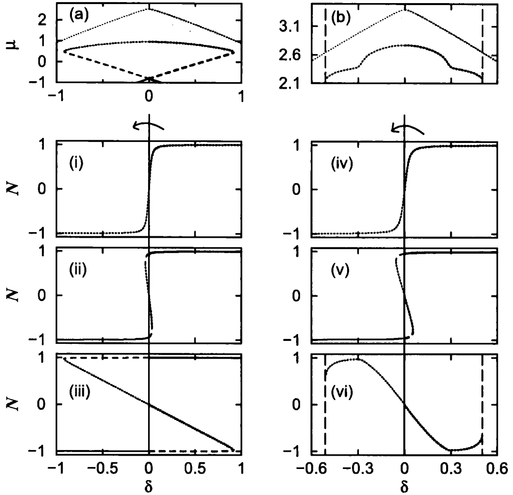
Figure 8.1: The eigenenergies \mu for the ground state in (a) one and (b) three dimensional double-well potential as a function of the potential gradient \delta for g_{1D} := 0 , (dark grey), -0.5 , (light grey) and -4 (black lines) and g_{3D} := 0 , (dark grey), -\pi , (light grey) and -6 (black lines) (from top to bottom). The eigenenergies for g_{1D} = 0, -4 and g_{3D} = -6 have been shifted along the \mu -axis by (\hbar\omega_{\perp}) : +0.1, -0.3 and -0.4 respectively. The fractional population difference N in a one (i)-(iii) and three dimensional double-well (iv)-(vi) respectively as a function of \delta . The values of the nonlinearities used here are: g_{1D} = 0, -0.5, -4 from (i)-(iii) and g_{3D} = 0, -\pi, -6 . Bold lines correspond to stationary solutions of the GPE and black lines are the symmetric projections in the -\delta -axis. In all cases we consider \hbar = 4 \hbar\omega_{\perp} .
