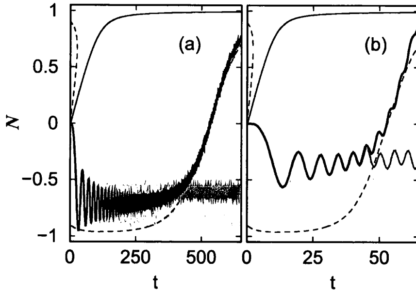
Figure 6.8: Evolution of fractional population difference N as a function of time (thick black lines) for different rates R of increase of the potential gradient: (a) R = 10^{-3} (\hbar\omega_{\perp}^2/a_{\perp}) and (b) R = 10^{-2} (\hbar\omega_{\perp}^2/a_{\perp}) . Grey (brown) lines plot corresponding evolution of the population difference for the case when the potential gradient is held constant after a time t = (a) 100 \omega_{\perp}^{-1} ( 400 \omega_{\perp}^{-1} ) and (b) 10 \omega_{\perp}^{-1} ( 40 \omega_{\perp}^{-1} ). Other parameters used, as in Fig. 6.1.
