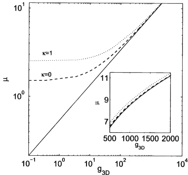
Figure 2.9: Chemical potential for the ground, \kappa = 0 , (dot-dashed) and the first excited, \kappa = 1 , state (dotted) line. The TF limit, \mu_{TF}^{3D} , (Eq. (2.37)) is also plotted as solid line. Inset we plot the chemical potential for large g_{3D} .
