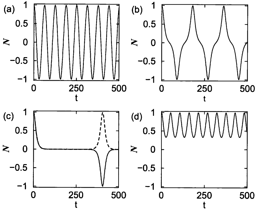
Figure 6.3: Evolution of fractional population difference N as a function of time, calculated using the two-state coupled Eqs. (4.18) and (4.19), with initial conditions N(0) = 0.994 and \phi(0) = \pi in a symmetric double-well trap ( \delta = 0 ). \Lambda takes the values: (a) 0, (b) 1.8, (c) 1.80407218718131001 (dashed) with N > 0 and 1.8080407218718131010 (dotted) with N < 0 and finally (d) 1.9.
