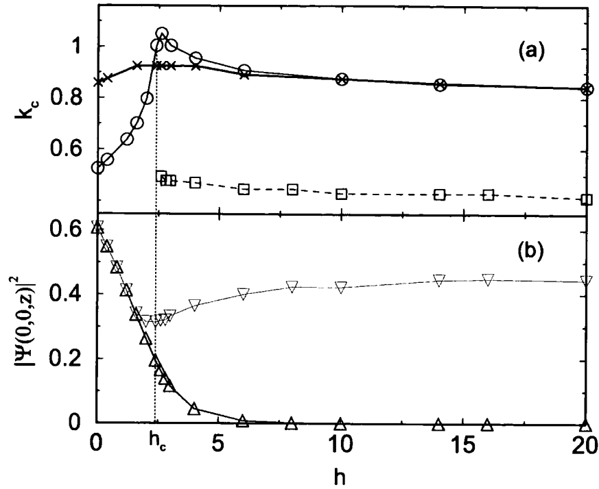
Figure 7.12: (a) Critical parameter k_c as a function of h for a spherical geometry ( \lambda = 1 ). Stability curves of the symmetric \Psi_g , (curve (iv) in Fig. 7.6(b)), first excited \Psi_e (curve (v)) and asymmetric ground states (curve (iii)) are shown as circles, crosses and squares respectively. (b) Condensate density |\Psi(0,0,z)|^2 along the z axis as a function of h for the state \Psi_g . Shown are the central |\Psi(0,0,0)|^2 (black) and peak |\Psi(0,0,z_m)|^2 (grey lines) densities, where z_m is the longitudinal position of maximum density in the double-well configuration (i.e. centre of each well). Vertical dotted line highlights the critical value h_c , above which the stability curve consists of two branches.
