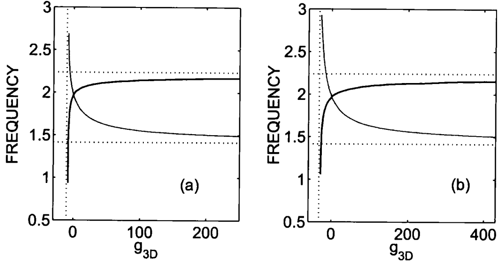
Figure 2.10: Monopole (grey) and quadrupole (black line) frequencies obtained from the numerical solution of the GPE (2.27) for an isotropic trap, \lambda = 1 . (a) shows the case with no vortex \kappa = 0 and (b) shows the two modes in the case of a vortex line along the z -axis, \kappa = 1 .
