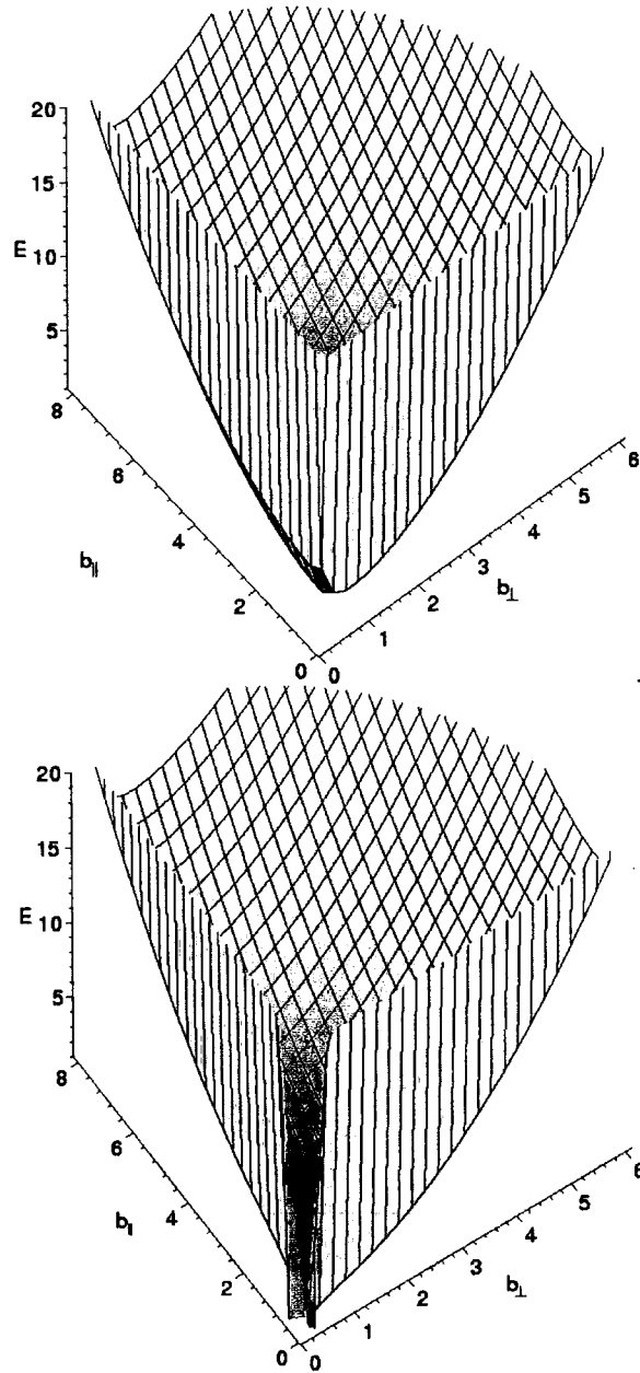
Figure C.3: Ground state energy E as a function of the variational parameters b_{\perp} and b_{\parallel} for two values of the nonlinearity |g_{3D}| = 4 (top) and 8.5 (bottom). We note that there is a critical value |g_{3D}^c| for which the energy has no longer minima and the condensate collapses.
