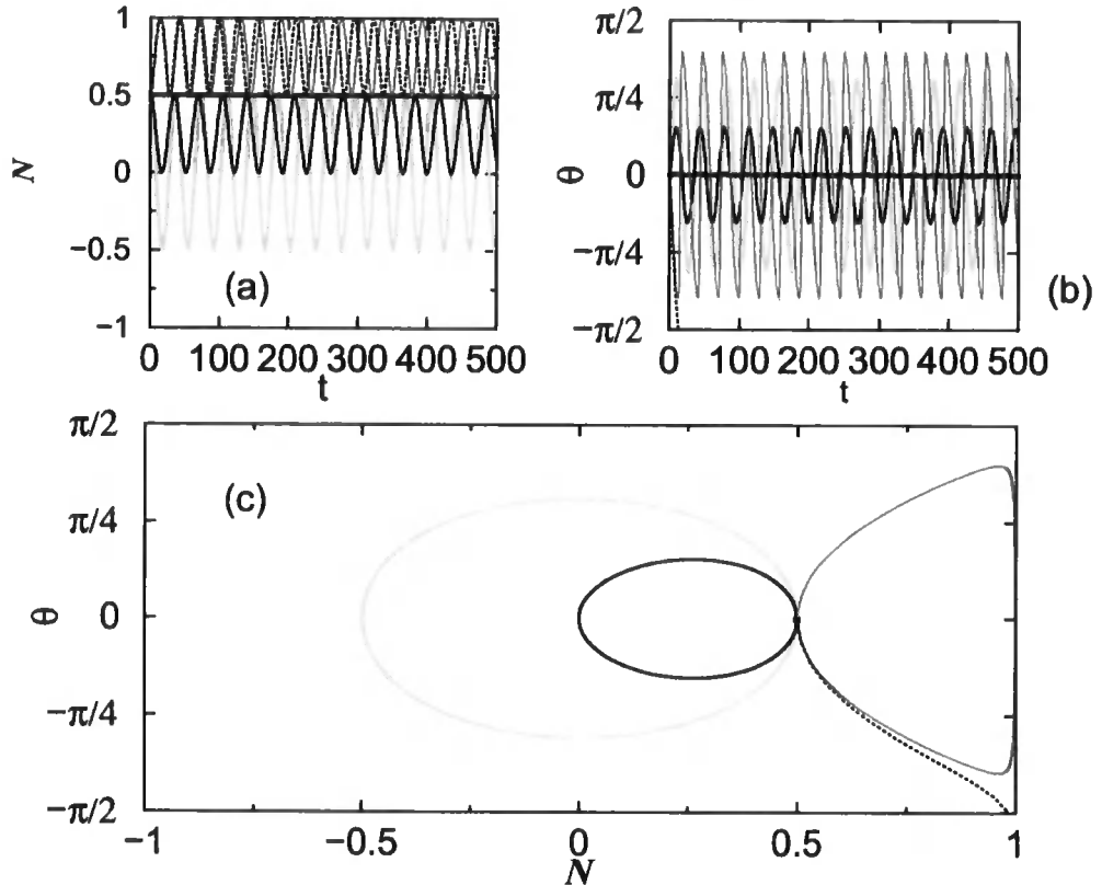
Figure 4.8: Evolution of (a) the population imbalance N and (b) the phase difference across the junction \theta for different values of the potential gradient \Delta . (c) Corresponding phase portrait (\theta, N) for a system with \theta(0) = 0 and N(0) = 0.5 . The values of the potential gradient are \Delta(\hbar\omega_{\perp}) =: 0 (light grey), 0.0867 (black), 0.177 (bold black), 0.344 (dark grey) and 0.357 (dotted black) lines. Other parameters for the two-state model are E_J = 0.1\hbar\omega_{\perp} and E_C = 0.24\hbar\omega_{\perp} .
