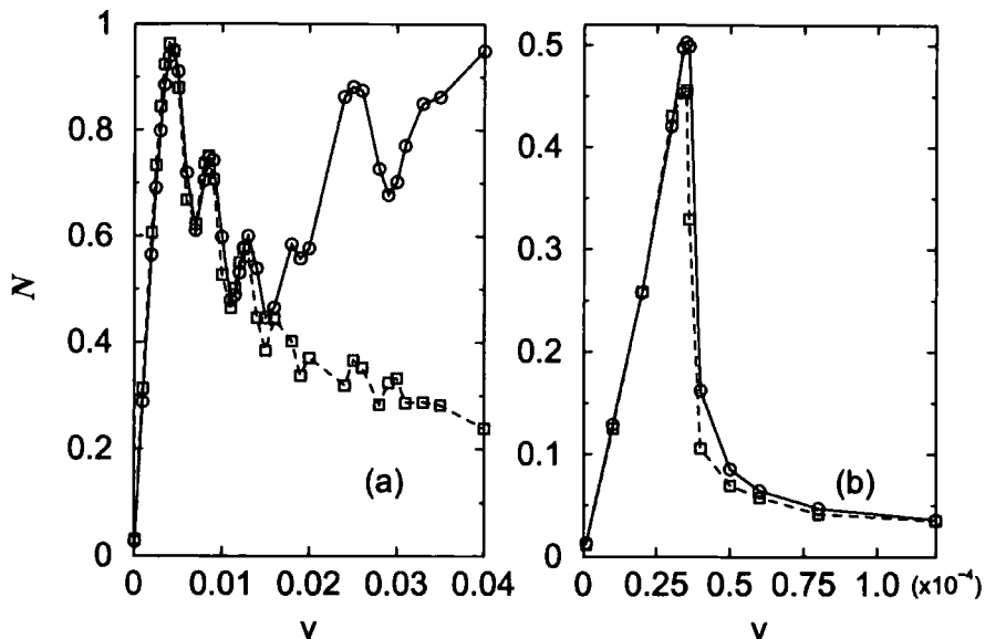
Figure 5.5: The fractional population difference as a function of the barrier speed v obtained from the GPE (solid line) and the two-state model (dashed line) for g_{1D} = 0.5 and (a) h = 4 \hbar \omega_{\perp} and (b) h = 12 \hbar \omega_{\perp} . The barrier is moved from the centre outwards for a time (a) t = 30 \omega_{\perp}^{-1} and (b) t = 1000 \omega_{\perp}^{-1} . For v = v_c there is a large step in the fractional population difference which corresponds to the critical velocity for the transition from a dc to an ac-current. In (a) v_c = 0.005 a_{\perp} \omega_{\perp} and (b) v_c = 0.000035 a_{\perp} \omega_{\perp} which are in good agreement with previous calculations. In (a) for v > 0.017 a_{\perp} \omega_{\perp} the second level crossing is reached leading to a departure between the GP simulation and the prediction of the two-state model whereas in (b) we are below the second level crossing for the range of velocities chosen. Other parameters as in Fig. 4.7.
