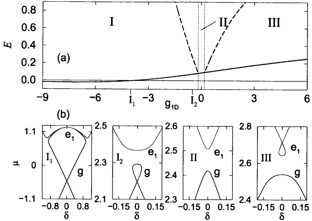
Figure 7.8: (a) The self-interaction energy |E_C| (dashed) and the Josephson energy E_J (solid) lines at \delta = 0 as a function of the nonlinearity g_{1D} for the one dimensional confining trap (Eq. 7.6), with h = 4 \hbar \omega_{\perp} . (b) Typical eigenenergies \mu as a function of the potential gradient \delta for various nonlinearities (from left to right) g_{1D} = -4, -0.5, 0 and 0.5 . The horizontal solid line corresponds to E = 0 .
