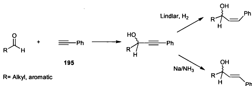
Scheme 33
