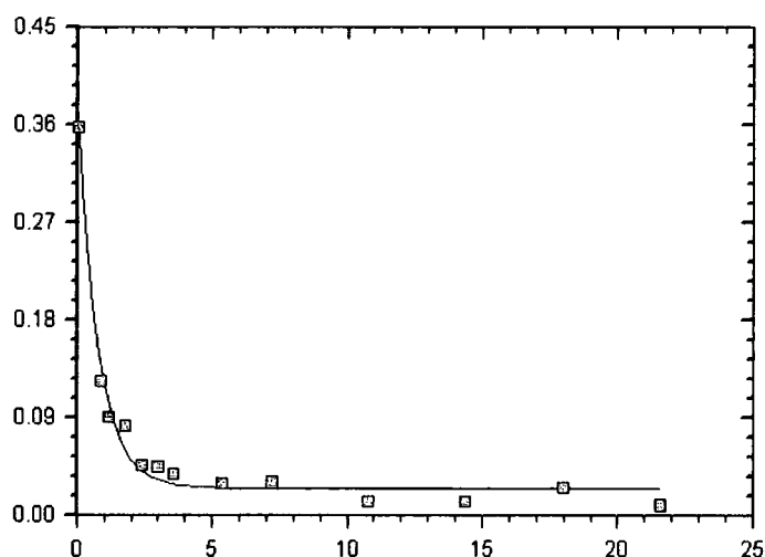
Graph 2: Average concentration of 156b (M, error 0.0017 M) against time ( 10^3 \text{ s} ).
