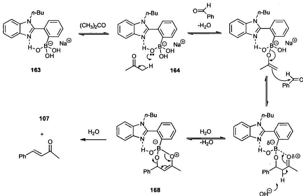
Scheme 31
