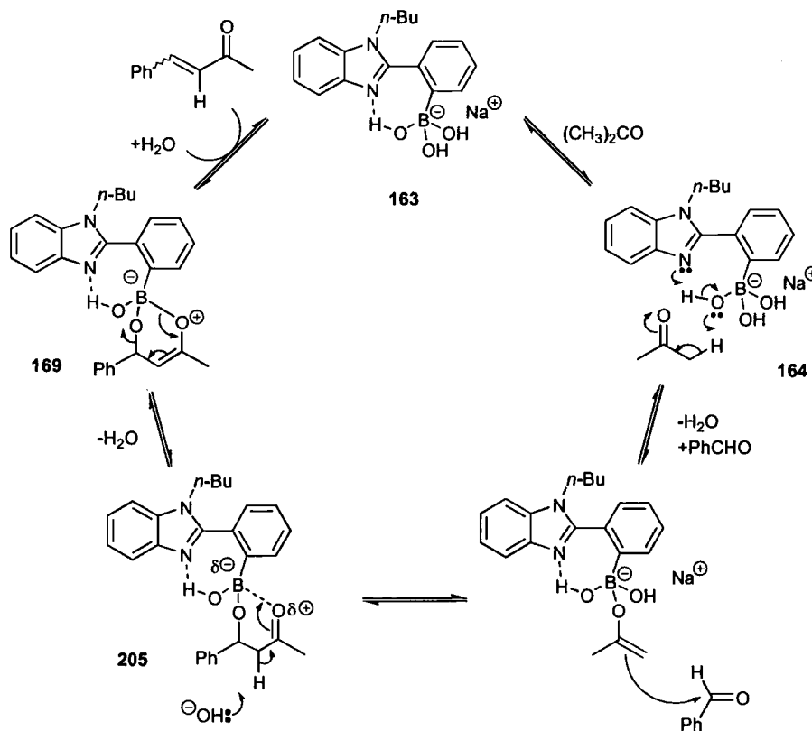
Scheme 39
