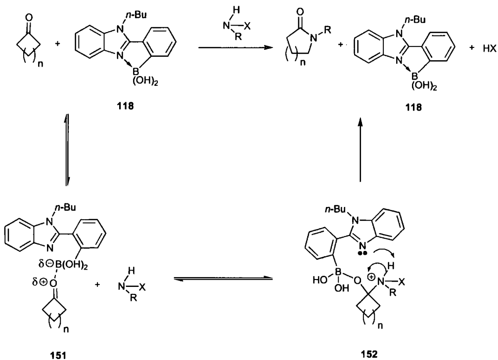
Scheme 25
