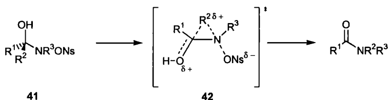
Scheme 6 17
