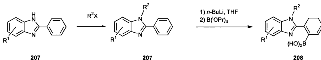
Scheme 42
