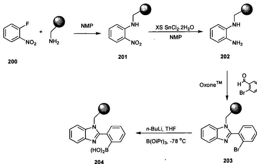
Scheme 34
