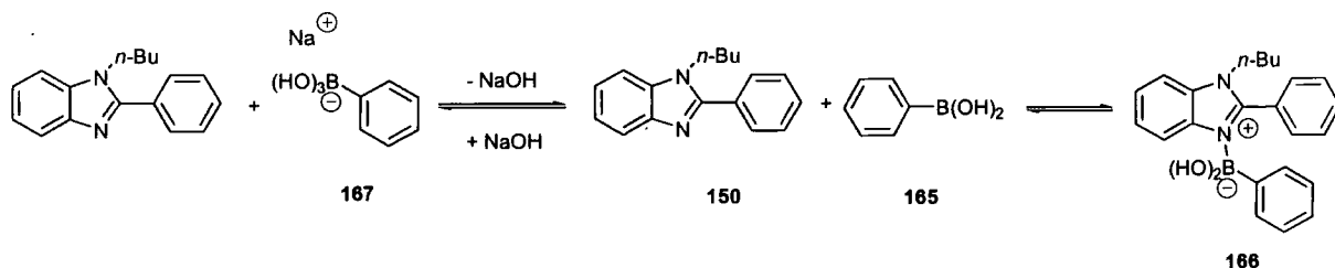
Scheme 30
