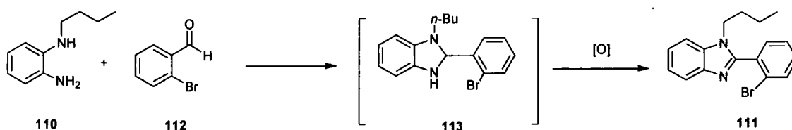
Scheme 18
