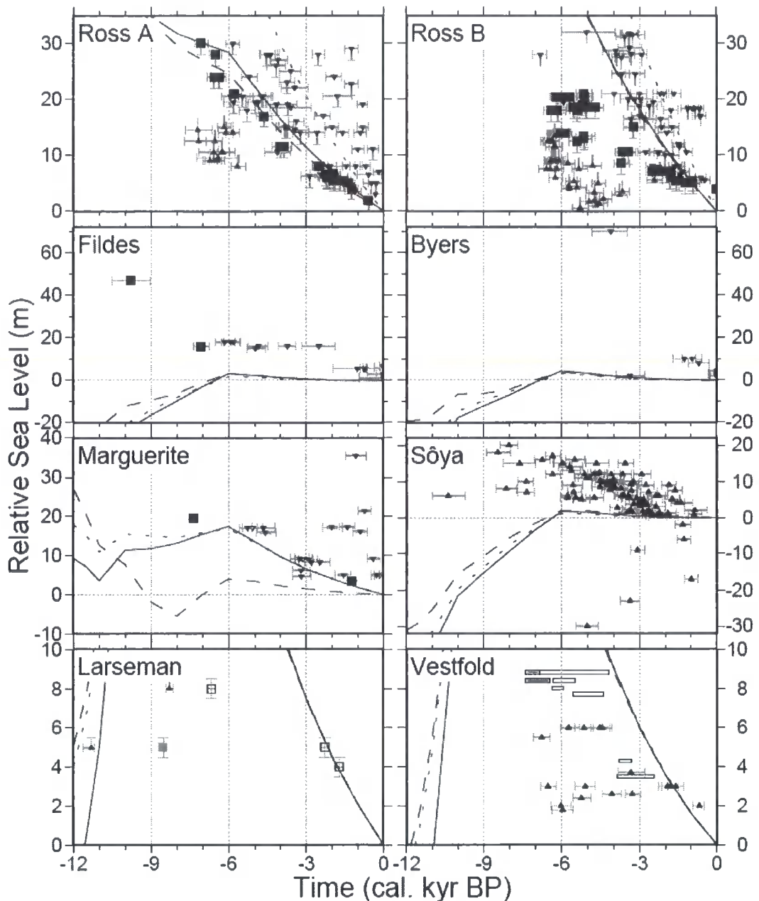
Figure 4.7: Sea-level predictions based on the reference earth model and three different models of Antarctic mwp-IA melt scenarios: Ross Sea source (dashed line), Weddell Sea source (dotted line), combination of Weddell Sea and Ross Sea (solid line). See main text for more details.
