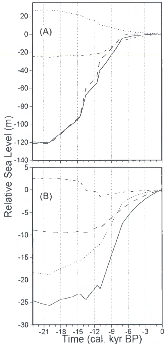
Figure 2.7: (A) The total sea-level prediction at Barbados for a model run in which a 0 m contribution to mwp-IA from Antarctica (solid line) is assumed. The dashed, dotted and dashed-dotted lines show the contributions from, respectively, the eustatic and non-eustatic spatially uniform and the spatially varying sea-level signal (see text for details). (B) The spatially varying signal at Barbados (solid line) split into components associated with ice-(dotted), ocean-(dashed) and rotation-induced (dot-dashed) perturbations to sea level.
