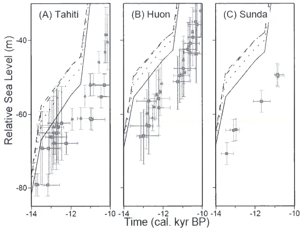
Figure 2.6: Sea-level predictions for Tahiti, Huon Peninsula and Sunda Shelf within the Lateglacial time window for four different source scenarios for the mwp-IA event. The solid and dashed lines represent the 0 m and 15 m contributions from the Antarctic ice complex (in units of equivalent eustatic sea-level rise) considered in Figure 2.3 and Figure 2.5. The dotted line shows the prediction for a global melt source distribution based on the All-ICE3G model of Clark et al. [28]; in this case the relative contributions to mwp-IA from North American, Antarctic and European ice sheets are 16, 5 and 5 m (eustatic). The dashed-dotted line shows the prediction for a northern hemisphere source distribution based on the model proposed by Peltier [69]; in this case the relative contributions from North American and European ice sheets are 22 and 5 m (eustatic), respectively.
