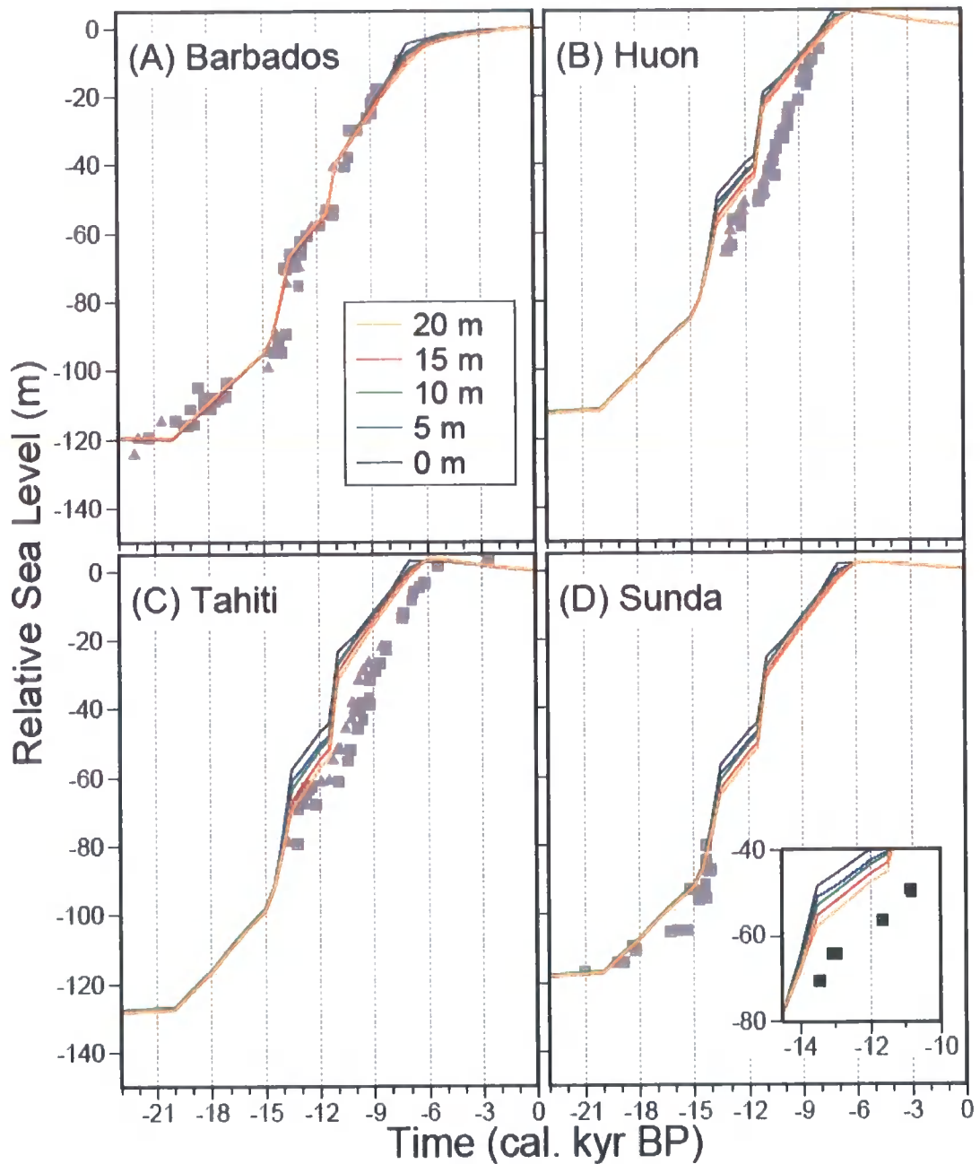
Figure 2.3: Sea-level predictions based on the reference earth model and a range of melt scenarios to illustrate the sensitivity to changes in the relative contributions of the Laurentide and Antarctic ice sheets to mwp-IA. The key in Frame A identifies the contribution, in eustatic sea level, from the Antarctic ice sheet for each model run. Each model was tuned to fit the Barbados record and so the success of each melt scenario can be gauged by the quality of the fit at the three southern hemisphere sites (Frames B to D). The inset in Frame D shows the fit of the model predictions to the data from location B shown in Figure 2.2. The triangles and squares indicate the sea-level observations described in the text and shown in Figure 2.1. Note that data error bars are not shown to improve the clarity of the figure.
