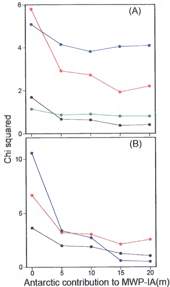
Figure 3.5: (A) Normalised \chi^2 misfit between predictions and post-LGM observations at four locations: Huon (black line), Tahiti (red line), Sunda (blue line) and Bonaparte Gulf (green line). Model predictions were generated using a GIA model tuned to the Barbados sea-level record for an earth model with a lower mantle viscosity of 4 \times 10^{22} Pa s and a range of Antarctic contributions to mwp-IA (in units of equivalent eustatic sea-level change; see x-axis). (B) Same as (A) but \chi^2 is calculated over the Lateglacial period only ( \sim 14 -9 cal. kyr BP).
