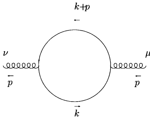
Figure 4.2: Fermion loop correction to the gluon propagator
