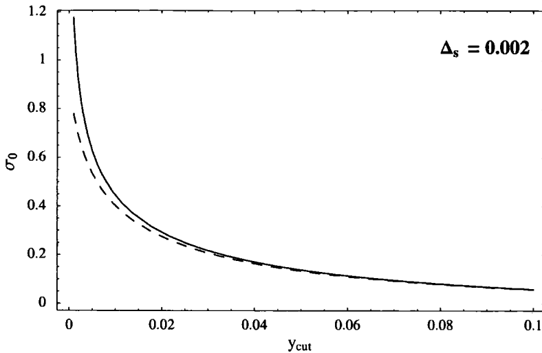
Figure 5.3: A comparison between the results for cross sections formed using the final states |q_{p_1} \bar{q}_{p_2} g_{p_3}\rangle (solid line) and |\{q_{p_1} \bar{q}_{p_2} g_{p_3}\}\rangle (dashed line) for \Delta_s = 0.002 .
