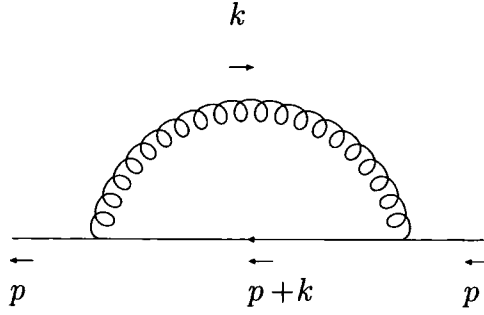
Figure 4.1: Correction to the fermion propagator
