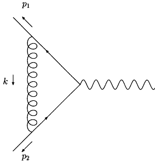
Figure 2.5: The vertex correction diagram
