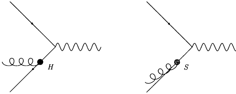
Figure 3.3: The emission of a hard gluon contributes to a three jet final state; the emission of a soft gluon contributes to a two jet final state.
