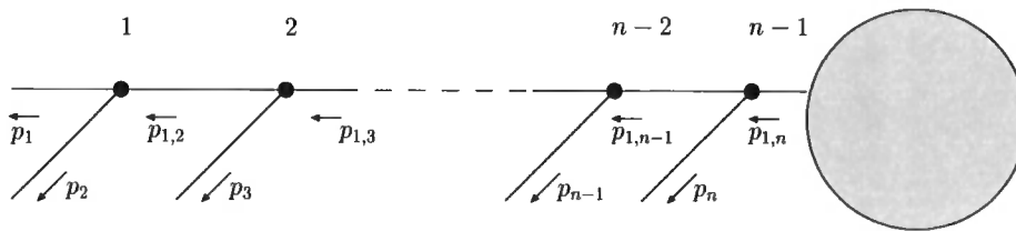
Figure 5.5: Some diagrams which will be zero under the new splitting functions.
