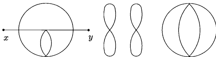
Figure 2.3: A typical Feynman diagram in \phi^4 theory including both connected and disconnected pieces.
