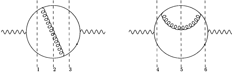
Figure 5.1: Some of the cut diagrams for the vertex correction calculation.
