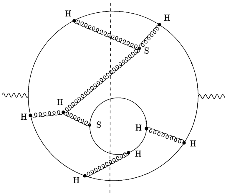
Figure 5.8: Cut diagram with apparently mismatched external states.
