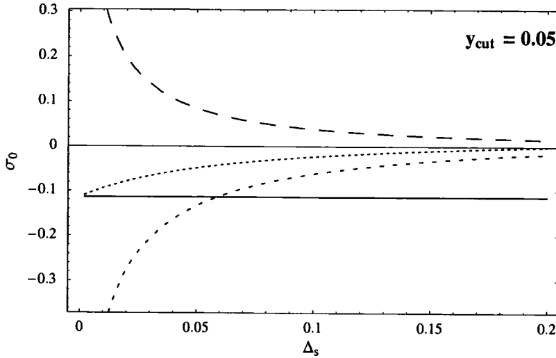
Figure 5.4: A comparison between the results for the |\{q_{p_1}\bar{q}_{p_2}\}\rangle cross section (long dashed line), the two jet part of the |\{q_{p_1}\bar{q}_{p_2}g_{p_3}\}\rangle cross section (short dashed line), their sum (dotted line) and the two jet result obtained from |q_{p_1}\bar{q}_{p_2}\rangle and |q_{p_1}\bar{q}_{p_2}g_{p_3}\rangle (solid line) for y_{cut} = 0.05 .
