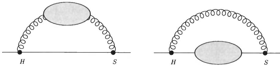
Figure 5.5: Some diagrams which will be zero under the new splitting functions.
