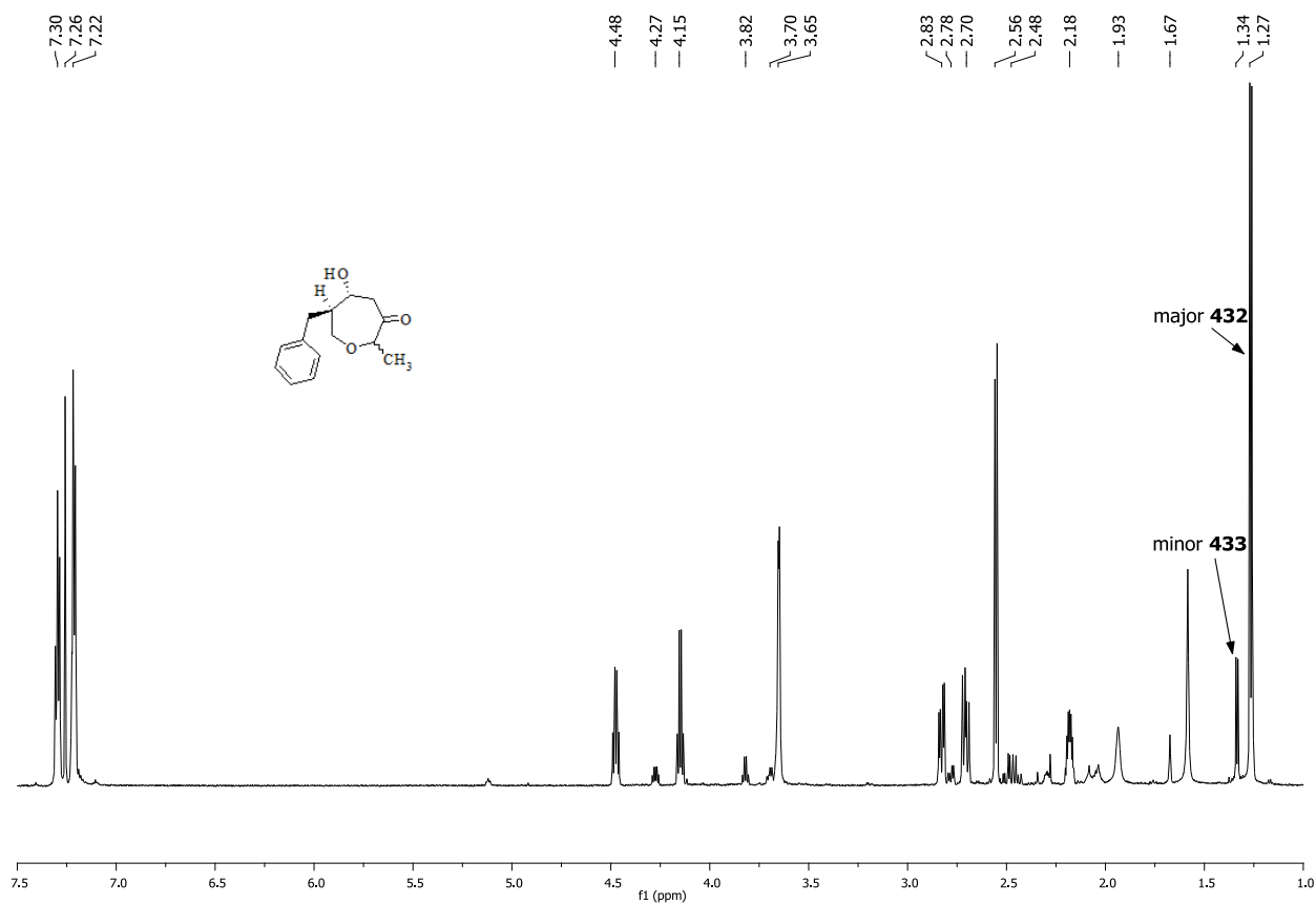
Figure 7.6
