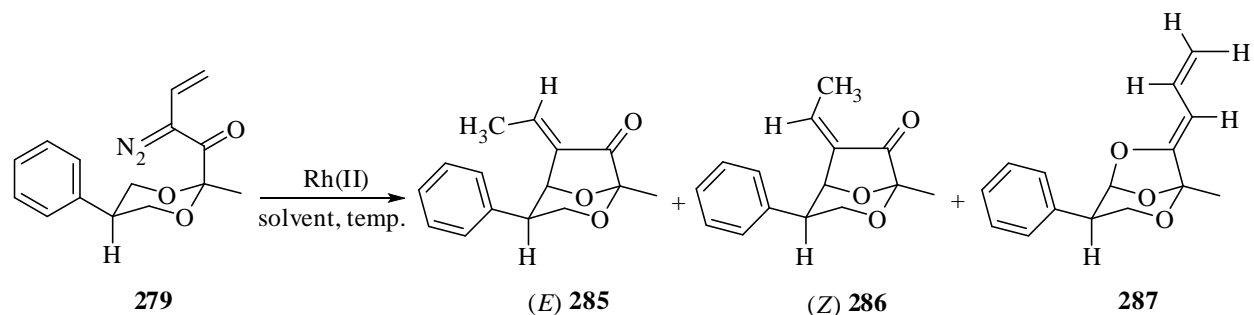
Scheme 5.13
