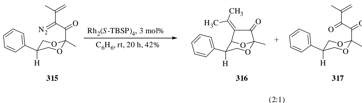
Scheme 5.29
