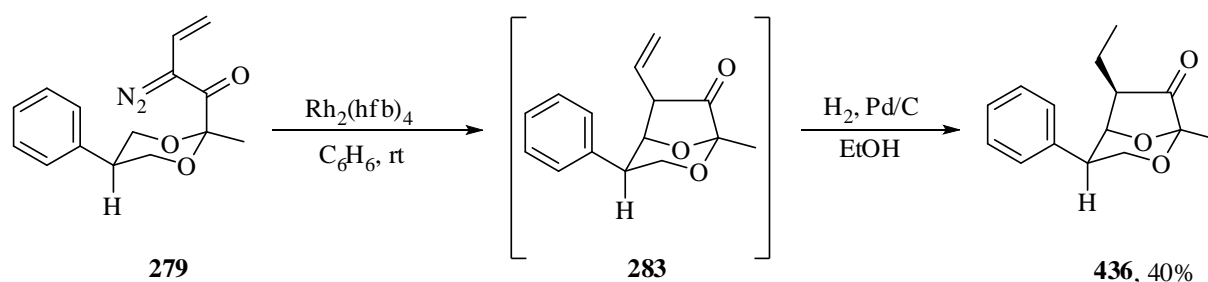
Scheme 7.27
