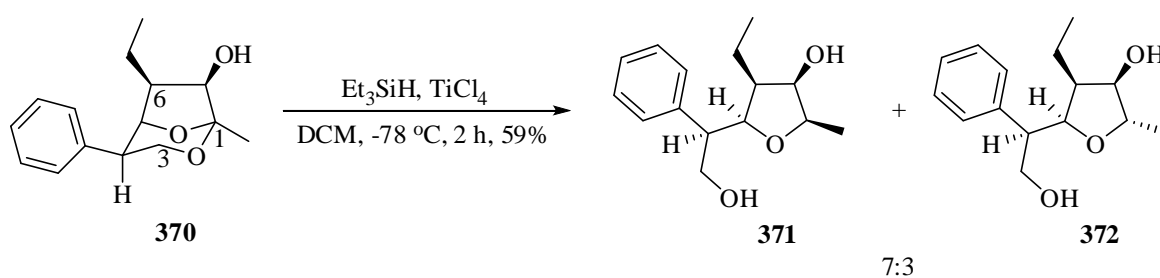
Scheme 6.18
