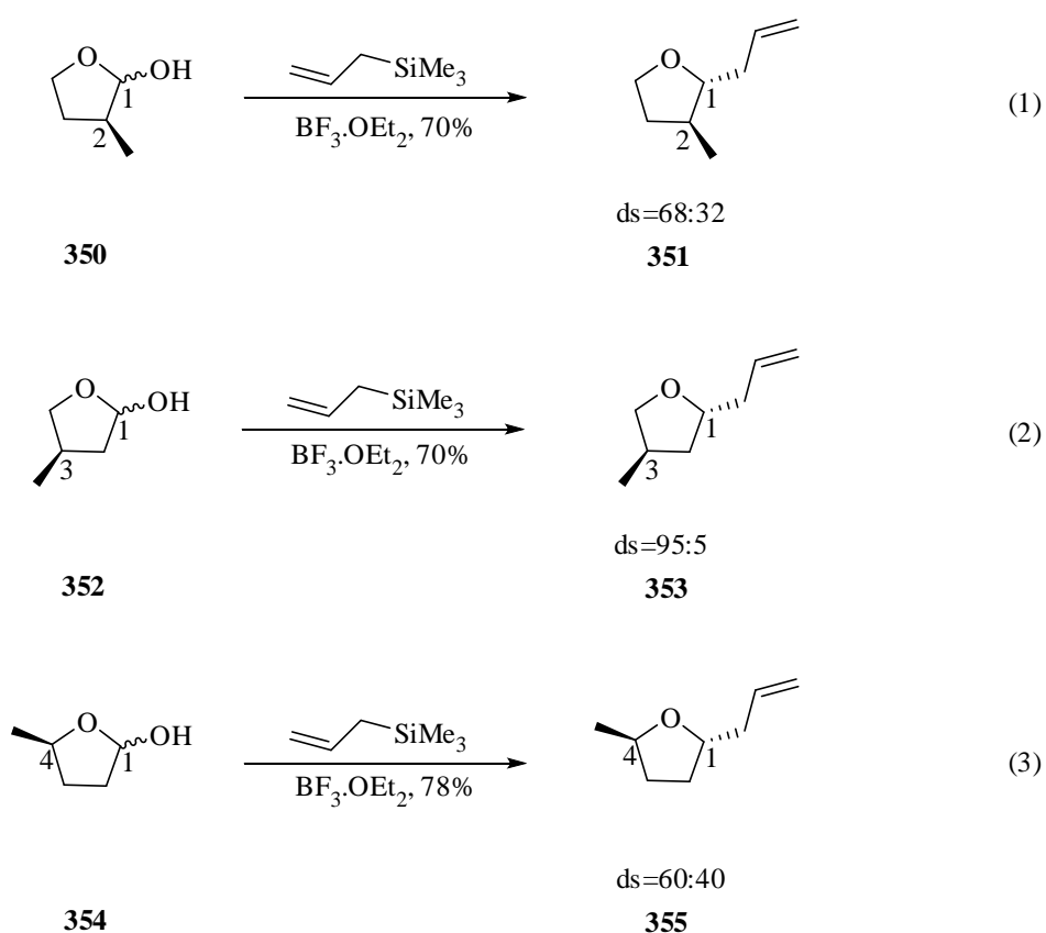
Scheme 6.8
