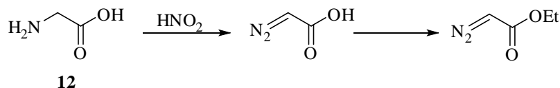
Scheme 1.6
