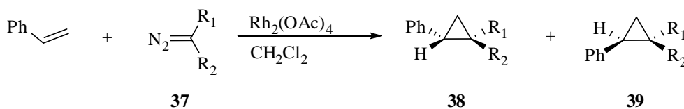
Scheme 1.20
