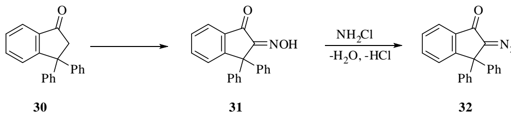
Scheme 1.12
