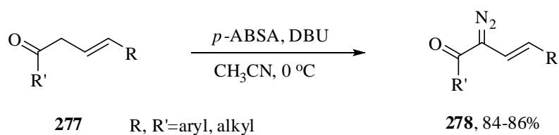
Scheme 5.8
