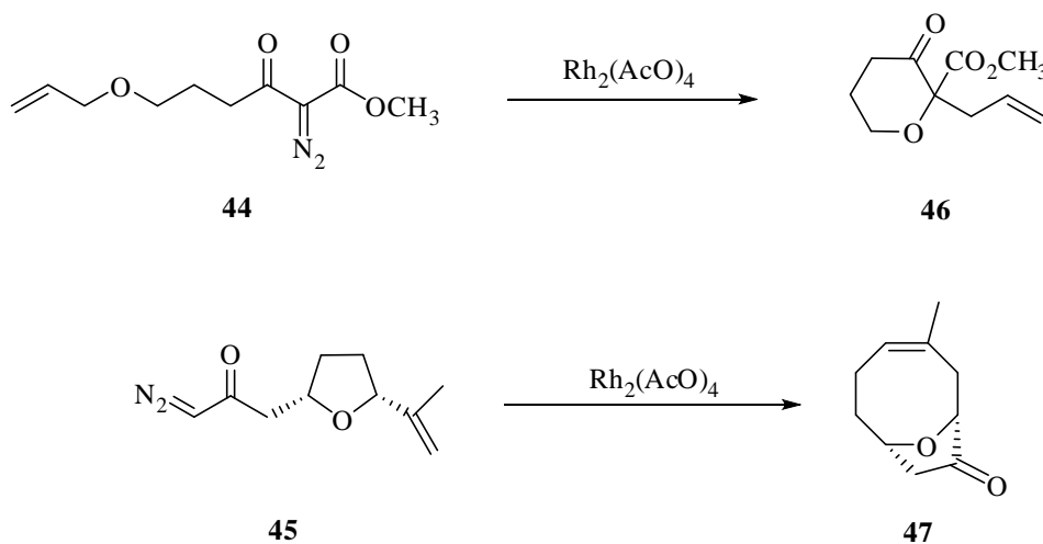
Scheme 1.25
