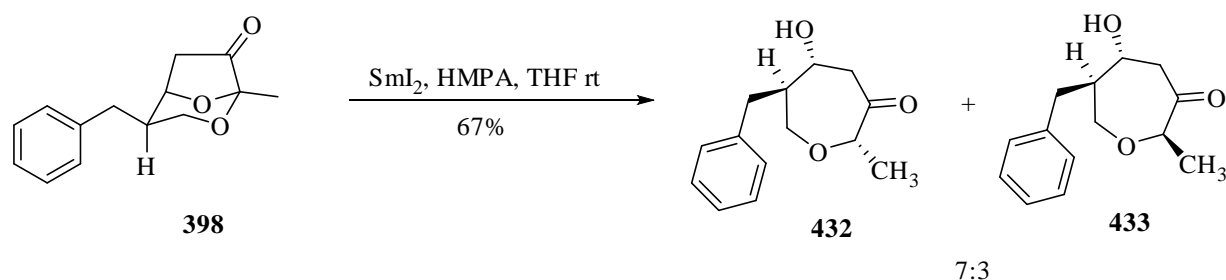
Scheme 7.25
