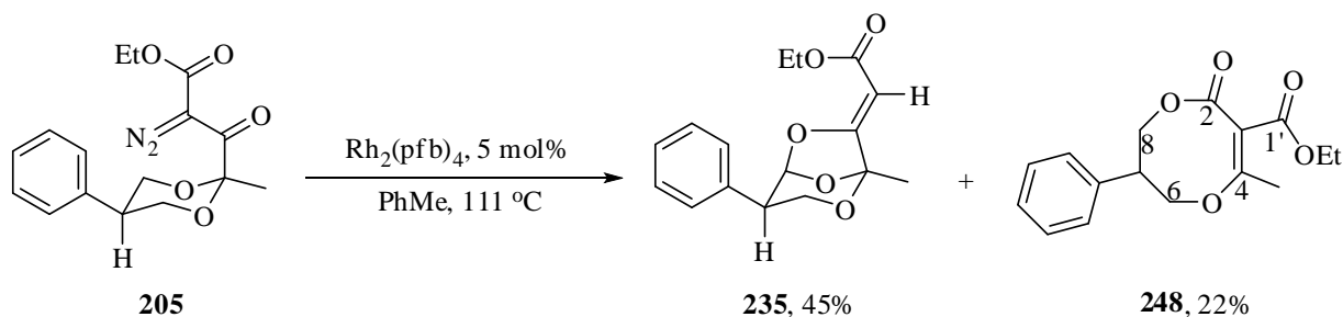
Scheme 4.12
