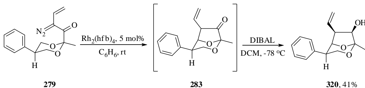
Scheme 5.32
