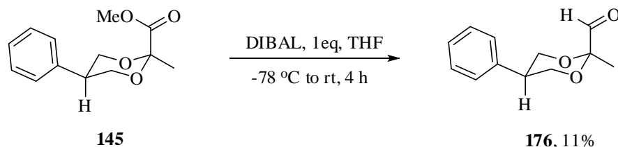
Scheme 2.10
