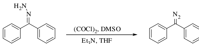
Scheme 1.14
