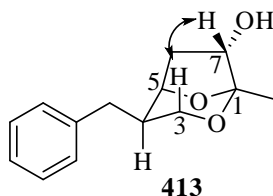
Figure 7.2
