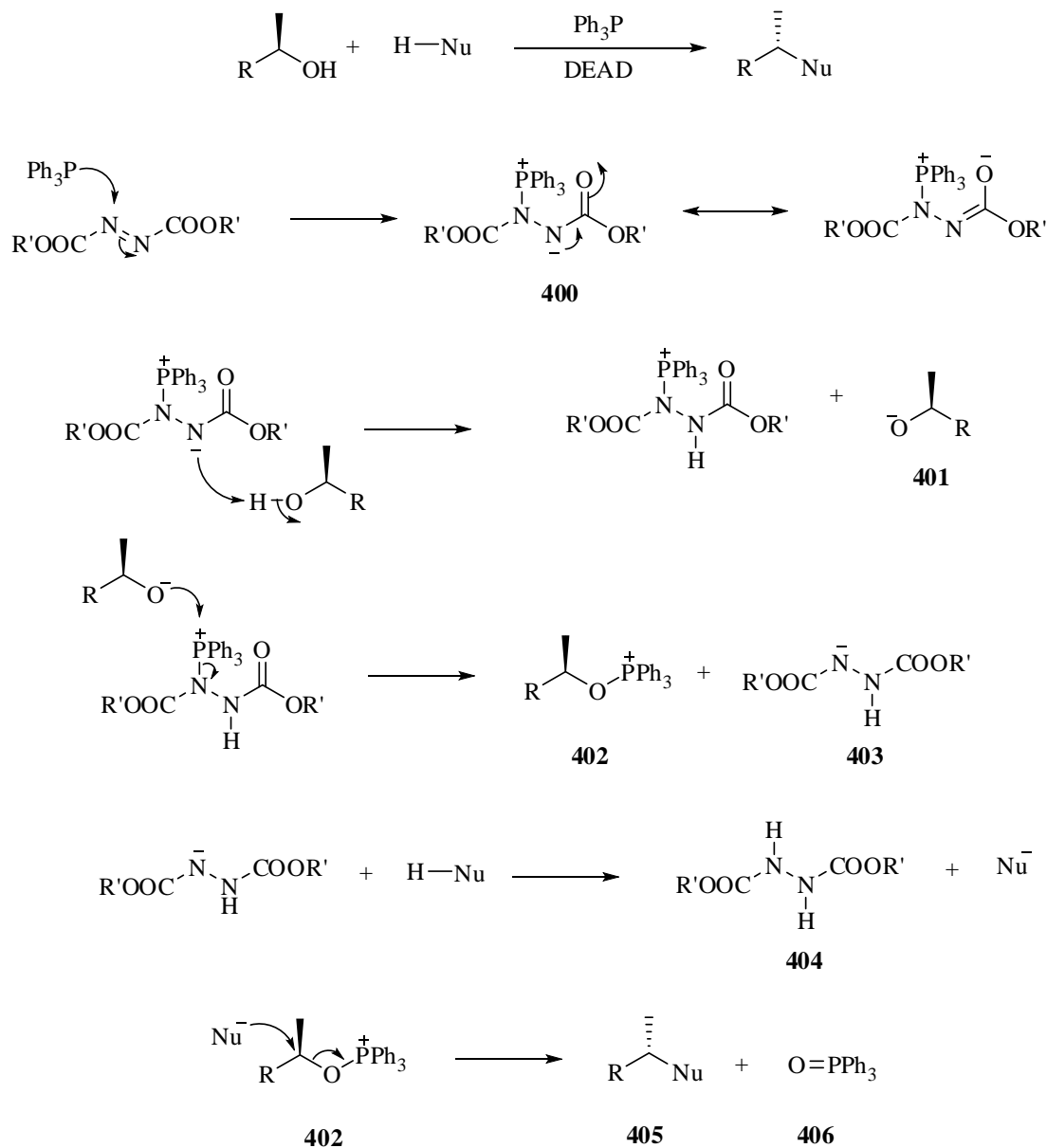
Scheme 7.10
