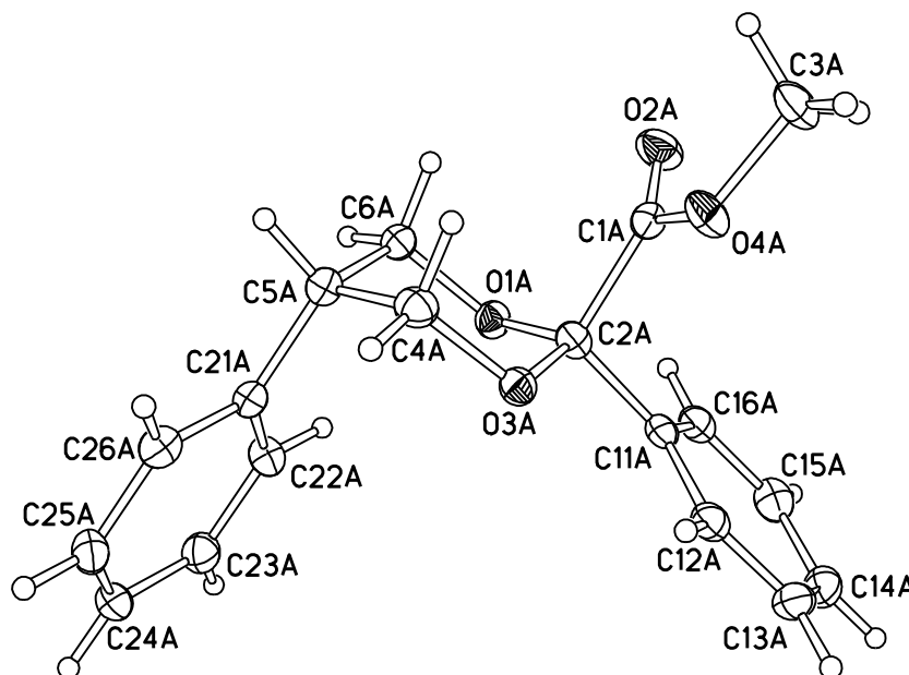
Figure 2.4
