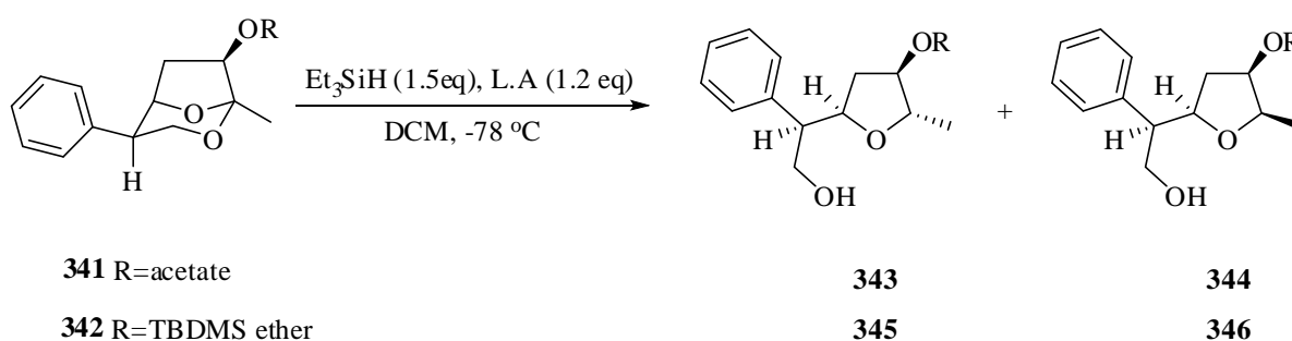
Scheme 6.5
