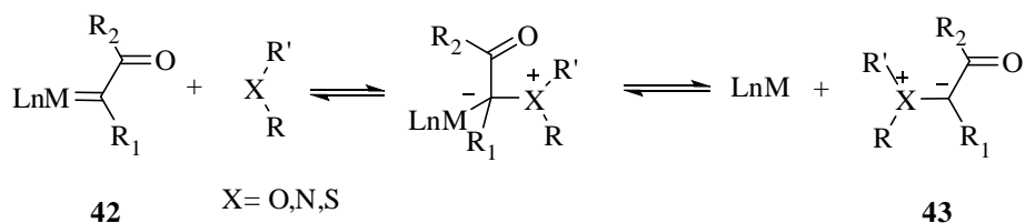
Scheme 1.23
