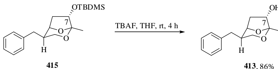
Scheme 7.17
