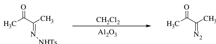
Scheme 1.13
