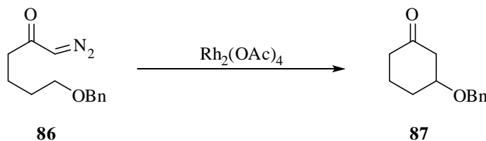
Scheme 1.47
