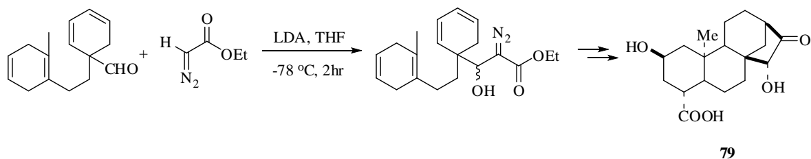
Scheme 1.40
