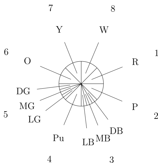
Figure 5.11: Configuration \sigma for Example 5.2.3
