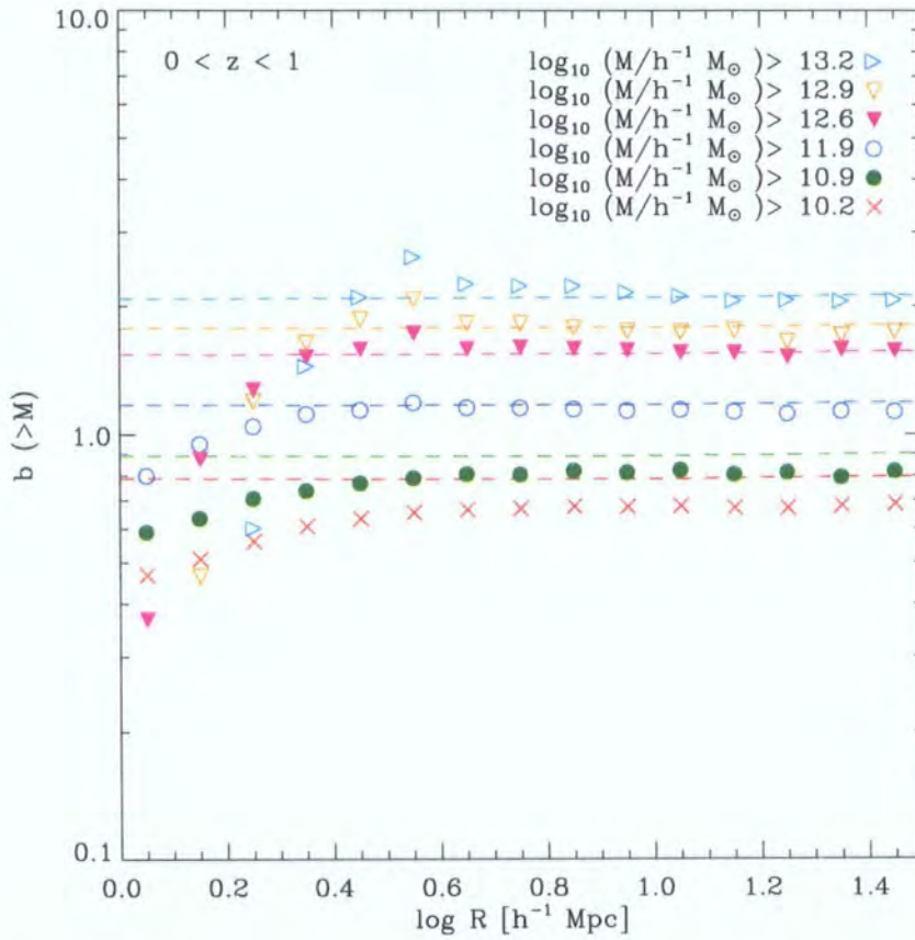
Figure 7.4: The linear bias parameter as a function of scale for haloes in the light-cone. The bias is defined as b^2 = \xi_{LC}^{hh} / \xi_{LC}^{mm} , where \xi_{LC}^{hh} and \xi_{LC}^{mm} are, respectively, the two-point correlation function for haloes and for dark matter in the light-cone. The symbols indicate our measurements while the dashed lines indicate the analytical prediction given by the square root of the ratio between Eq. 7.4 and Eq. 7.5.
