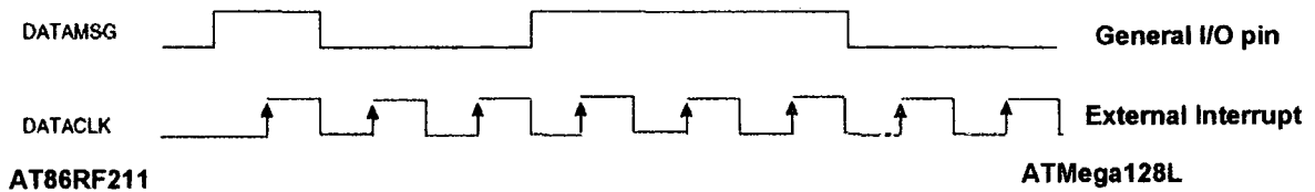
Figure 48 – Dataclk recovery
