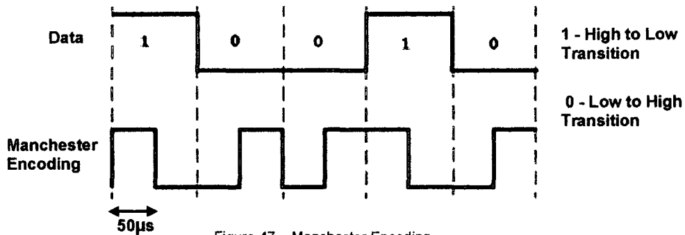
Figure 47 – Manchester Encoding
