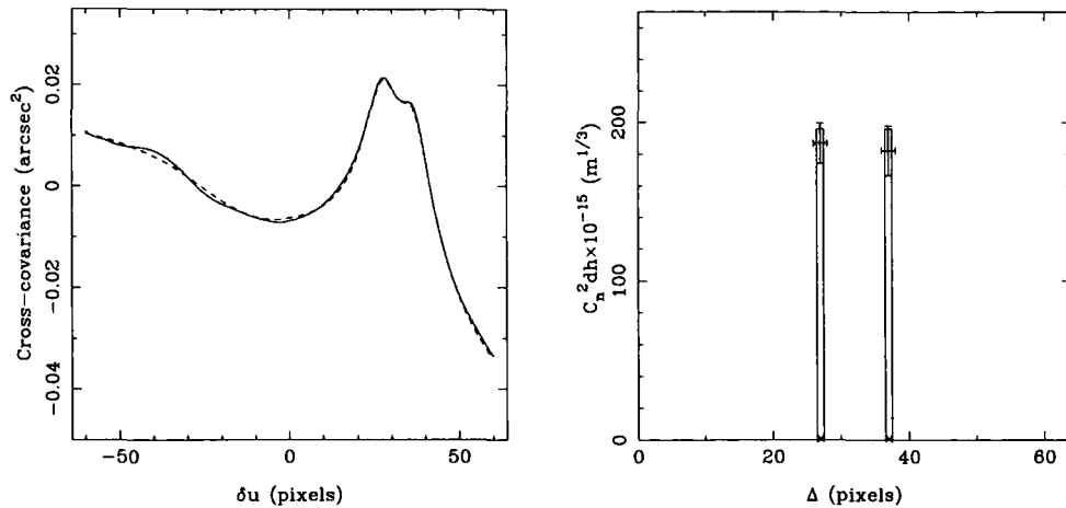
Figure 6.8: SLOTDAR in the high light level case. w = d/2 , no photon noise. Left : measured cross-covariance (solid line) and fit (broken line). Right : fitted profile. The error bars on the fitted C_n^2 show the change in the fitted parameters needed to increase the least squares difference by a factor of 2.
