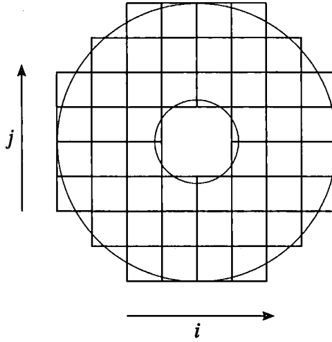
Figure 5.3: Pupil geometry for the 8 \times 8 subaperture ESO portable SLODAR system, showing the mapping of the square wavefront sensor subapertures on to the annular aperture function of the Meade LX200 telescope.
