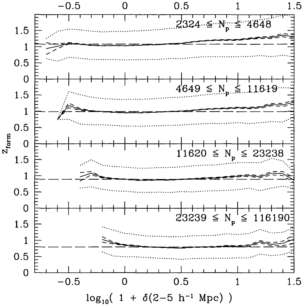
Figure 2.10: The formation redshift of haloes as a function of overdensity in a spherical shell of inner radius 2 h^{-1} \text{ Mpc} and outer radius 5 h^{-1} \text{ Mpc} centred on the halo (solid lines). The range of particle numbers for the haloes in each panel is shown; these are chosen so that haloes have the same mass as those in the corresponding panel of fig. 3 of Lemson & Kauffmann (1999). Note the difference in the scale of the horizontal axis between the linear scale of fig. 3 of Lemson & Kauffmann (1999) and the logarithmic scale of this figure which extends to higher densities. Short-dashed lines show the error on the determination of the mean formation redshift in each bin in overdensity. Dotted lines show the 1\text{-}\sigma dispersion in halo formation times. The flat, long-dashed line is at the mean formation redshift for all haloes in that bin in mass, and is shown only to guide the eye.
