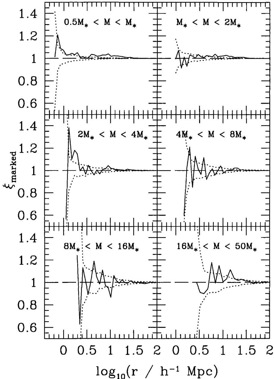
Figure 2.6: The marked correlation function of haloes with mass in the ranges shown (solid lines), with \bar{\omega}_f as the mark. Dotted lines are calculated as in Fig. 2.5a. The top four panels may be compared with fig. 4 of Sheth & Tormen (2004b) since the value of M_* in their simulation is approximately twice ours. Note, though, the difference in axis scale, and the fact that in their figure formation redshift is used for the mark, whereas here \bar{\omega}_f is used (see Fig. 2.7 which shows this does not affect our conclusions). The lower four panels cover the same mass range as Fig. 2.5a.
