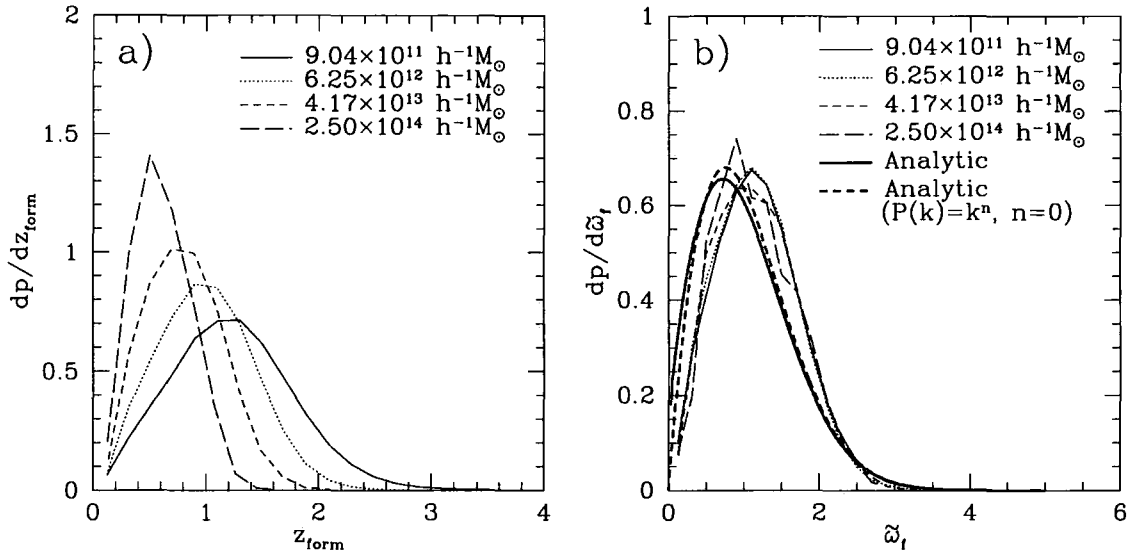
Figure 2.4: The distribution of halo formation redshift (left-hand panel) and of scaled formation redshift \tilde{\omega}_f (right-hand panel). The distribution is shown for haloes in four different mass bins spaced equally in \log(\text{halo mass}) and centred on the mass given in the legend. The trend in the left-hand panel is such that haloes of larger mass have a more strongly peaked distribution, with the peak at smaller redshift. In the right-hand panel, we show in addition the analytic prediction for the distribution of \tilde{\omega}_f (which is very nearly independent of mass) with thicker, smoother lines. The thick, solid line shows the prediction using the input power spectrum for the Millennium Simulation, while the thick, dashed line shows the prediction using a power-law initial power spectrum with index n = 0 .
