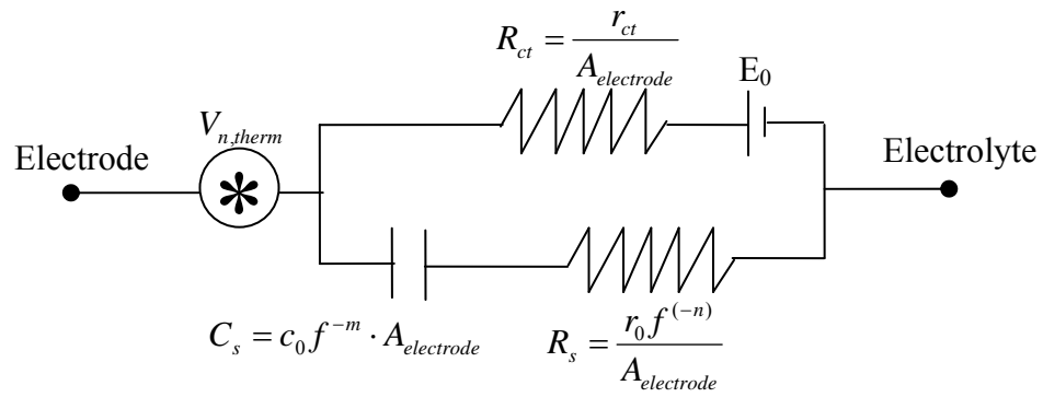
Figure 7.10 Electrode Model for Pt and Au electrodes
