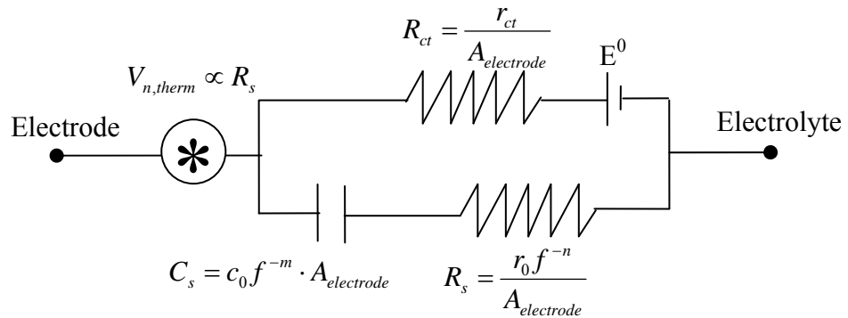
Figure 6.6 Electrical model of the electrode-electrolyte interface
