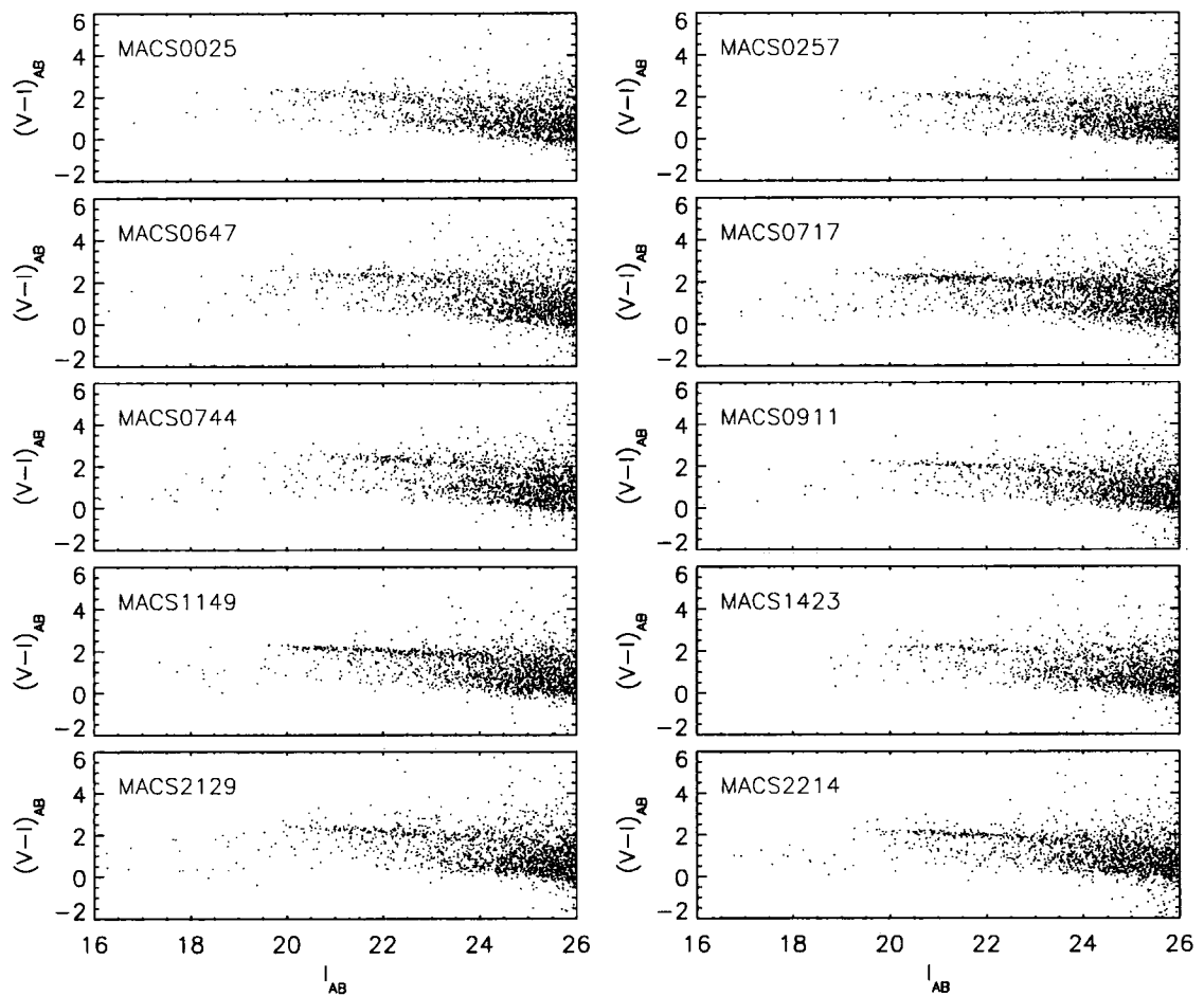
Figure 3.1: The individual (V_{555} - I_{814}) colour-magnitude diagrams for the MACS clusters. Colour-magnitude plots for individual clusters in the LARCS survey can be found in Pimbblet et al. (2002).
