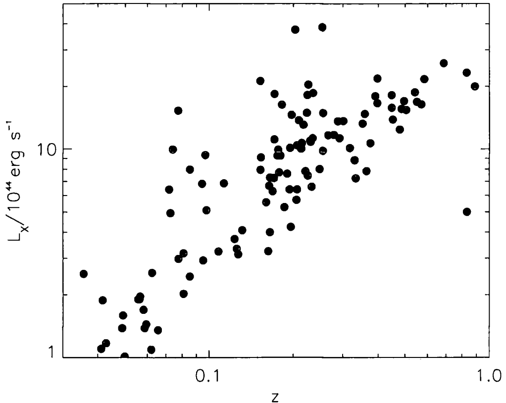
Figure 2.1: The X-ray luminosity vs z for our sample.
