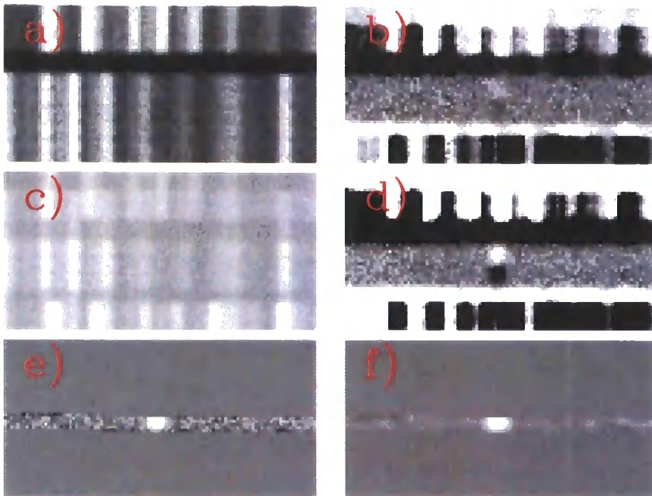
Figure 5.3: Examples of the various steps in the data reduction, showing a region centred on a bright emission line. The six panels each show a region of \sim 135 \text{ \AA} in the spectral (horizontal) direction by 25 pixels in the spatial (vertical) direction. Panel (a): the initial individual frame. Panel (b): the same frame after sky-subtraction (by shifting a copy of the image by 16 pixels and subtracting). The dipole signature of an emission line is now visible. Panel (c): the initial frame after adding instead of subtracting the two shuffled regions to produce an image of the sky. Panel (d): frames from step (b) after median combination of several exposures. Panel (e): co-addition of the positive and negative components of the dipole by 'nod-folding' and masking (see text for details). Panel (f): after convolution with the 2D Gaussian kernel.
