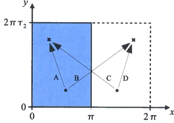
Figure 3.6: The annulus as obtained from the torus by setting \tau_1 = 1 and identifying under x = -x ( z = -\bar{z} ). A fundamental region is shown shaded. The propagator is obtained by supplementing each transition (marked A,D) by an image charge piece (marked B,C).
