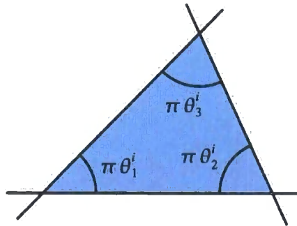
Figure 4.3: We work with internal angles, and always stick to the notation where subscripts on angles label intersections, and superscripts label tori.
