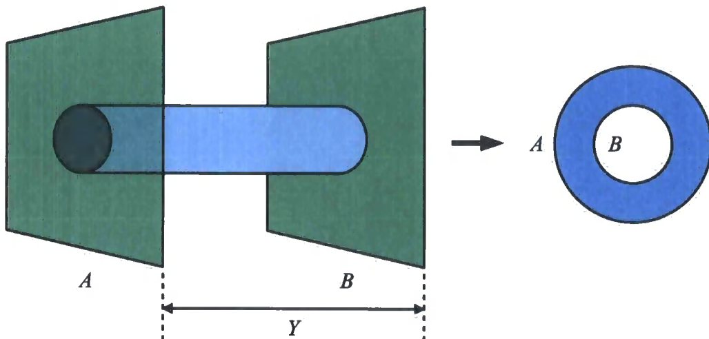
Figure 2.3: The one-loop partition function between parallel branes A and B, separated by a distance Y , is an annulus diagram with one edge of the annulus on each brane.
