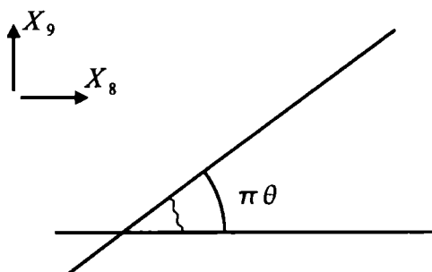
Figure 2.4: Two branes at a relative angle \pi\theta .
