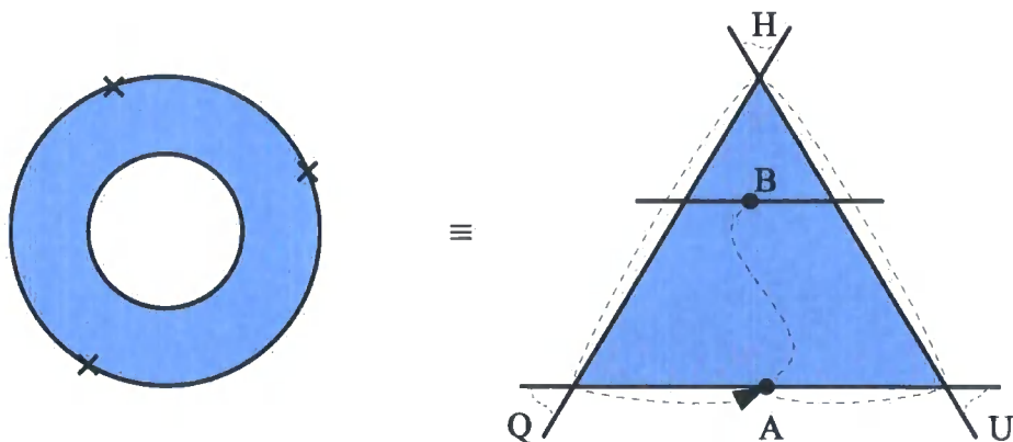
Figure 4.1: The annulus diagram corresponds to taking an open string stretched between two branes as shown, and moving one end around the Yukawa triangle.
