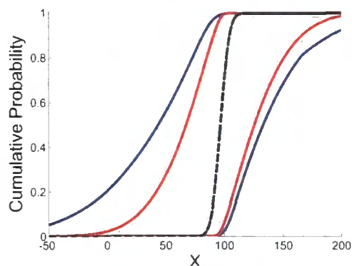
Figure 3.6: Robust Normal Bayesian p-boxes
