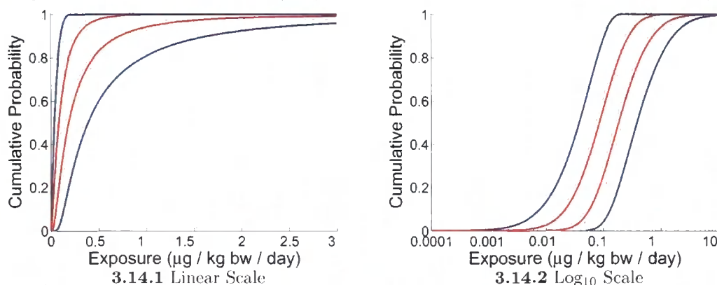
Figure 3.14: 95% B_I p-box (red) and between 94.91 and 98.3% B_F p-box (blue)
