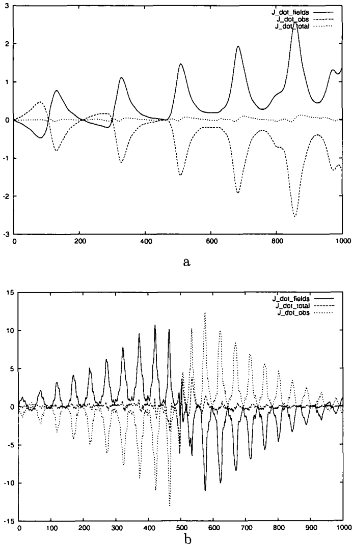
Figure 5.14: Plots of the time derivative of the total angular momentum, \dot{J}_{tot} and its components \dot{l}_{fields} and \dot{l}_{obs} as a function of time for a two different systems: a) d = 6 skyrmion configuration with b = 2 for \Gamma = 0.25 and b) d = 5 skyrmion configuration with b = 2 for \Gamma = -0.5
