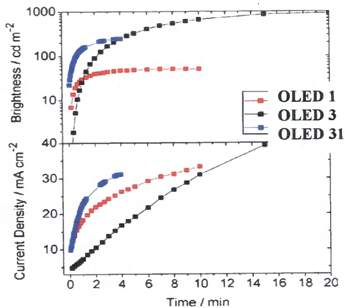
Figure 78. Linear logarithmical presentation of the brightness and current density as a function of time for LECs of OLEDs 1, 3 and 31 driven at an applied bias of 3 V: device architecture ITO/PEDOT:PSS/complex/Al.
