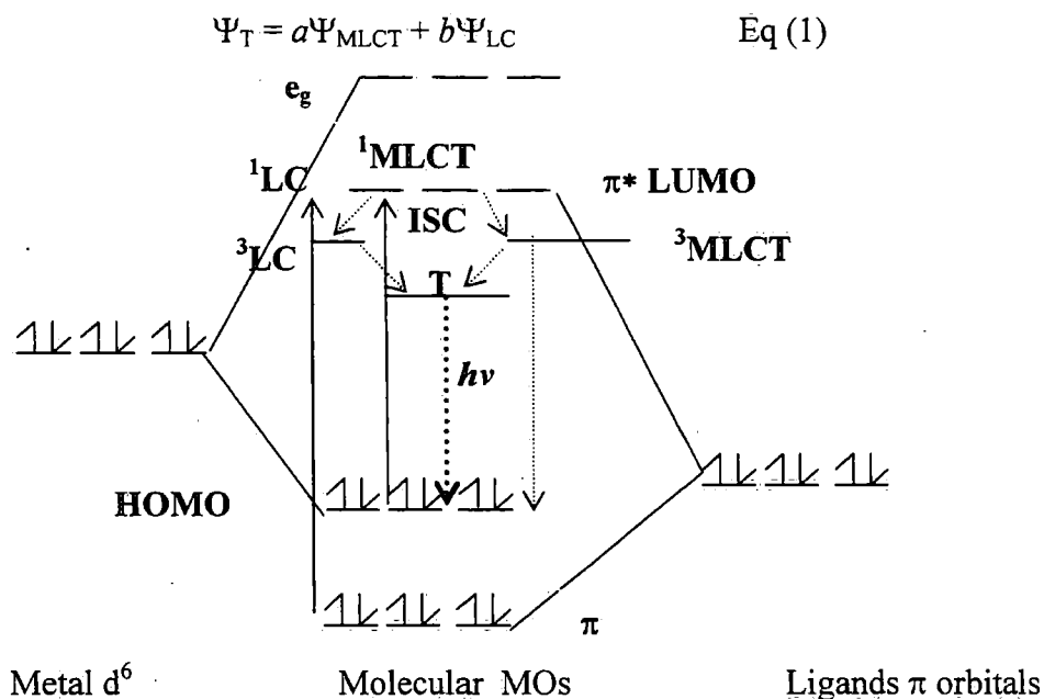
Figure 50. Schematic and simplified molecular orbital diagram for an octahedral d^6 metal complex involving 2-phenylpyridine ( C_3 symmetry) type ligands in which various possible transitions are indicated.
