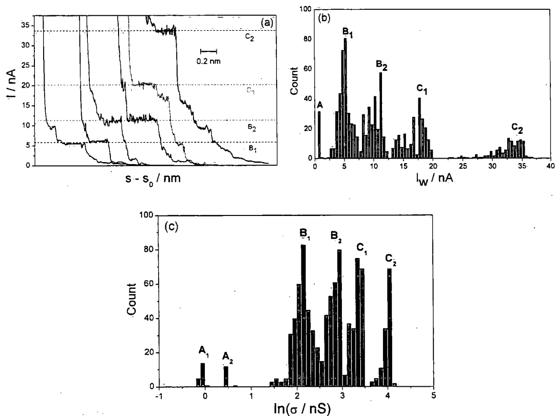
Figure 31. (a) Typical scans recorded during the tip withdrawal when compound RJ 32 molecular junctions are formed and then broken at a bias voltage of 600 mV using the BJ method. (b) Histogram of current values constructed from 52 individual BJ scans for RJ 32 . (c) A log scale conductance histogram using the data shown in b.
