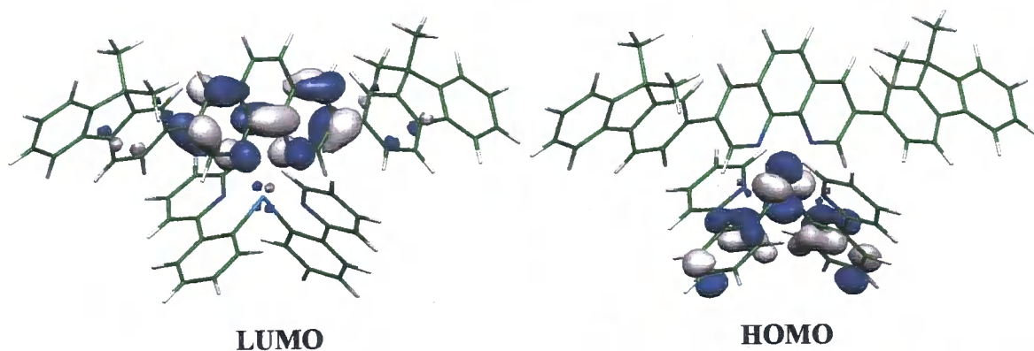
Figure 74. Isocontour plots (0.04 e bohr -3 ) calculated for the HOMO and the LUMO orbitals of 96 (OLED 3') (from reference 153).
