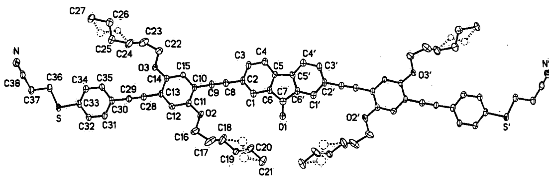
Figure 11. The X-ray crystal structure of the ca. 4 nm molecule CSW-11 (calculated from intramolecular S---S distance) synthesised in our group (from reference 23).
