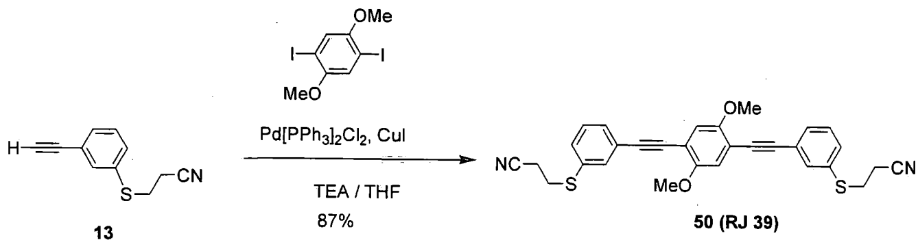
Scheme 8. The synthesis of meta linked OPE; 50 (RJ 39) .
