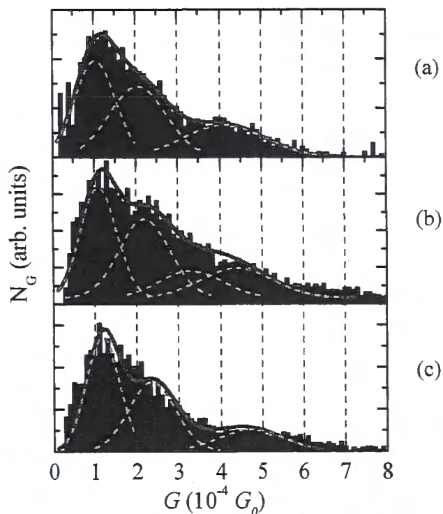
Figure 39. Histogram plot of conductance data during the breaking process of OPE derivatives (a) no side chain ( RJ 16Ac ) (b) methoxy side chains ( CSW 558 ) and (c) hexyloxy side chains ( 35 (RJ 8Ac) ).
