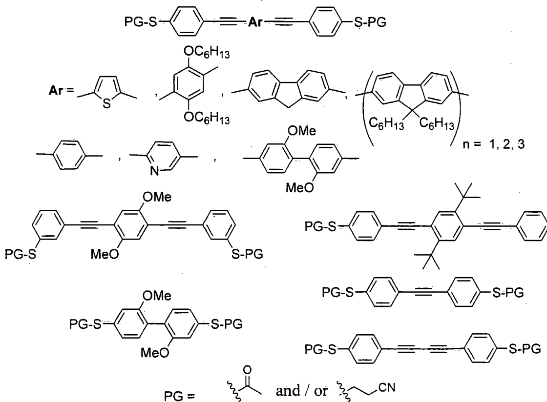
Figure 15. The structures of our targets.
