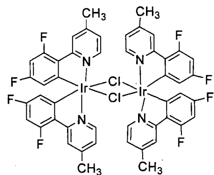
87 [(4\text{Meppy})_2\text{IrCl}]_2
