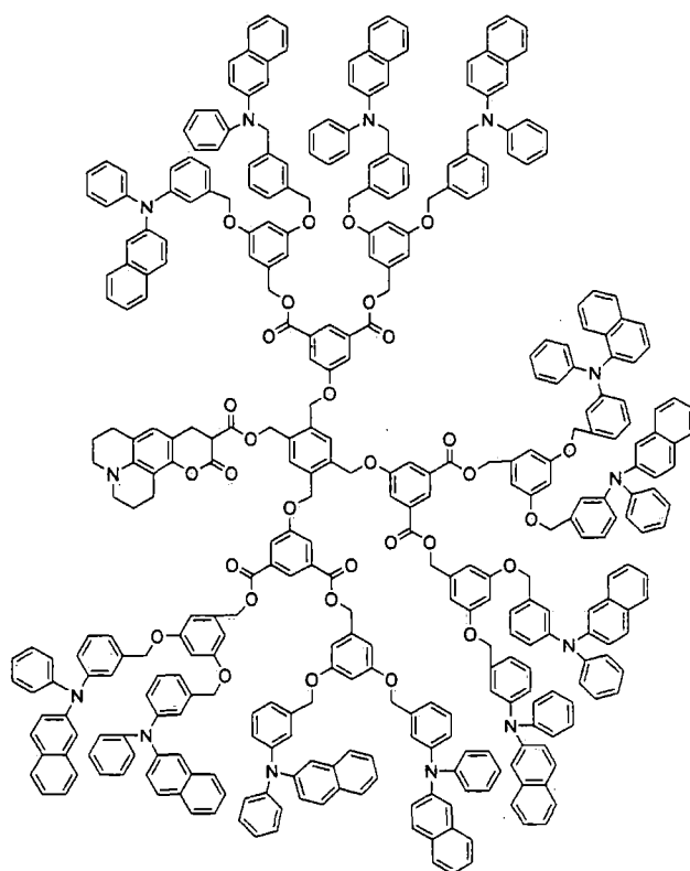
Figure 44. Example of a dendrimeric molecule used in OLEDs.
