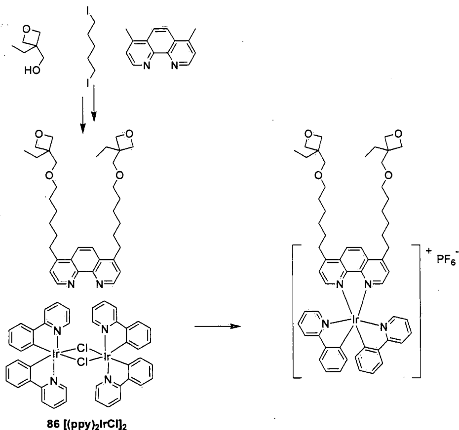
Scheme 29. The synthetic pathway to future target complex
