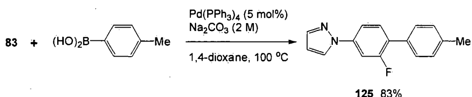
Scheme 30. Suzuki-Miyaura reaction of 83 .
