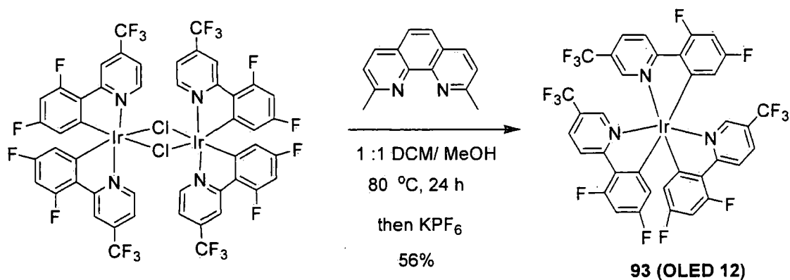
Scheme 28. Unexpected synthesis of 93 (OLED 12).
