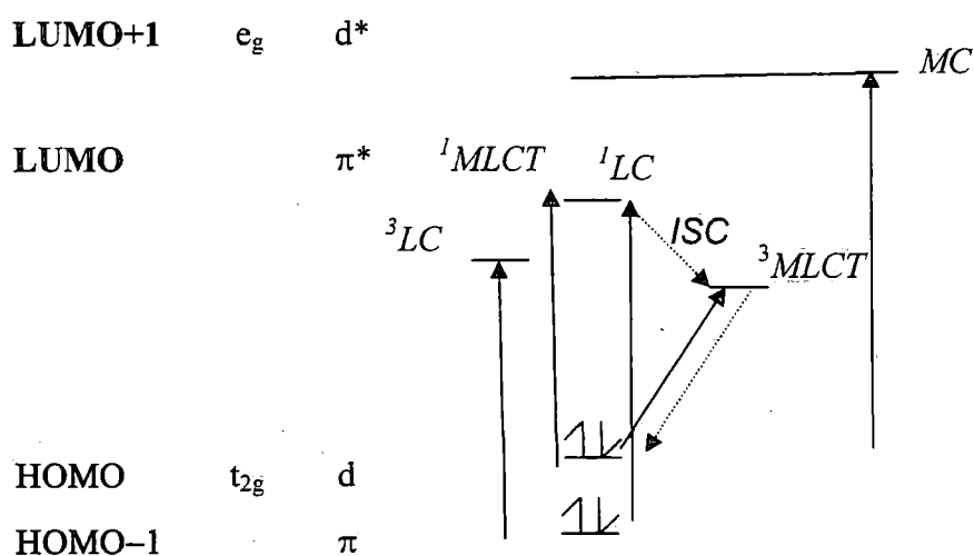
Figure 49. Introductory MO model for a compound with single \pi , d , and \pi^* orbitals and the respective MLCT, LC and MC transitions.
