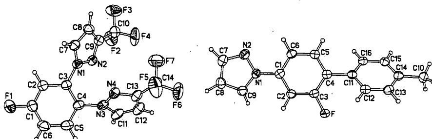
Figure 82. X-ray molecular structures of compounds 122 at room temperature (left) and 125 at 120 K (right). Thermal ellipsoids are drawn at the 30% ( 122 ) and 50% ( 125 ) probability levels; rotational disorder of CF 3 groups is not shown.
