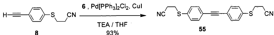
Scheme 10. The synthesis of mono-alkyne 55 .
