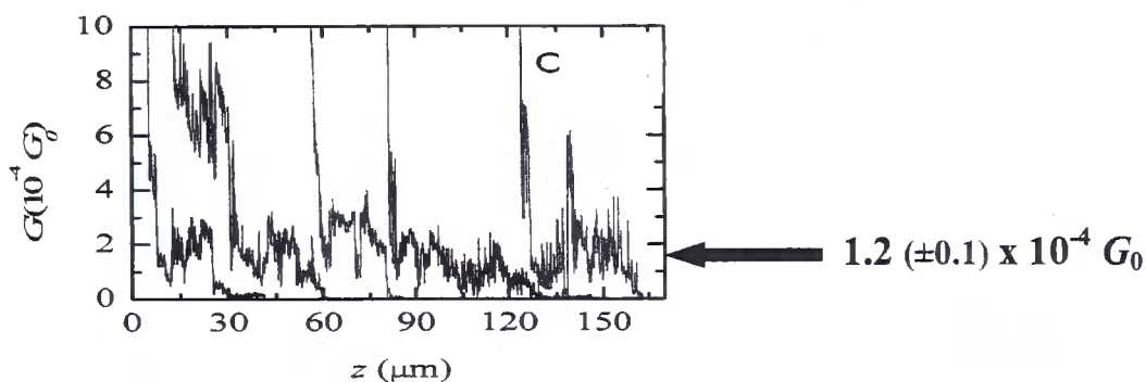
Figure 38. Variation of conductance during the breaking process of a junction of deprotected 57 (RJ 8Ac) . The results of 5 different experiments are shown with the traces shifted horizontally for clarity.
