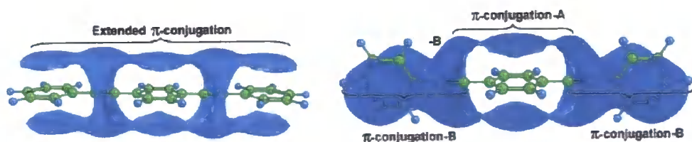
Figure 10. \pi -Conjugation features for OPE in different conformations (from reference 100).
