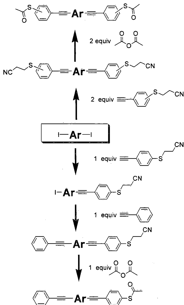
Figure 16. The general synthesis of oligo(1,4-aryleneethynylene)s terminated with either one or two thioacetate groups.
