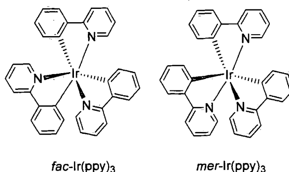
Figure 45. Facial and meridional isomers of Ir(ppy) 3 .
