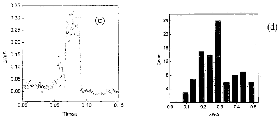
Figure 29. (a) Variation of the mean molecular area with the combined period of self-assembly of 35 ( RJ 8 ). (b) Symmetrical I - V characteristics of the Au- 35 ( RJ 8 ) structure contacted by a Au probe. (c) The SAMs of 35 ( RJ 8 ) show current jumps of ca. 0.2-0.3 nA. (d) Histogram of the observed current jumps with a notable grouping at 0.2-0.3 nA. Data obtained at a set point current of 300 mV.
