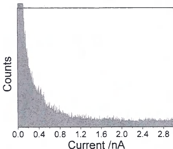
Figure 36. Conductance histograms for 59 (RJ 40Ac) .
