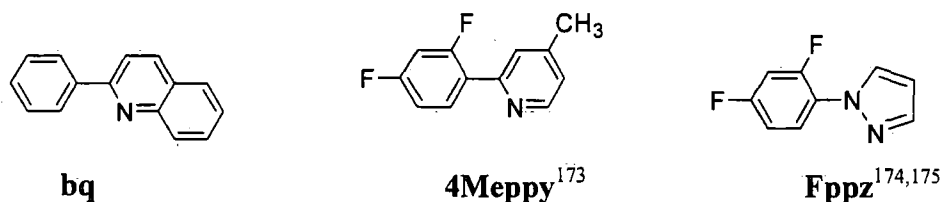
Figure 67. The structures of the C N ligands for cyclometalation.
