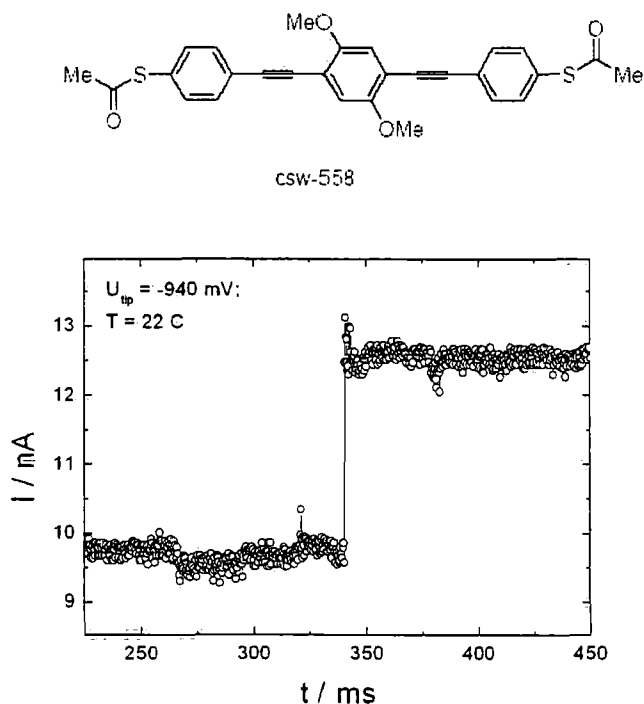
Figure 5. Typical current jump of ca. 3 nA recorded using the molecular wire of CSW-558 to bridge the gap by the I(t) method (from reference 78).
