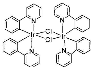
86 [(\text{ppy})_2\text{IrCl}]_2
