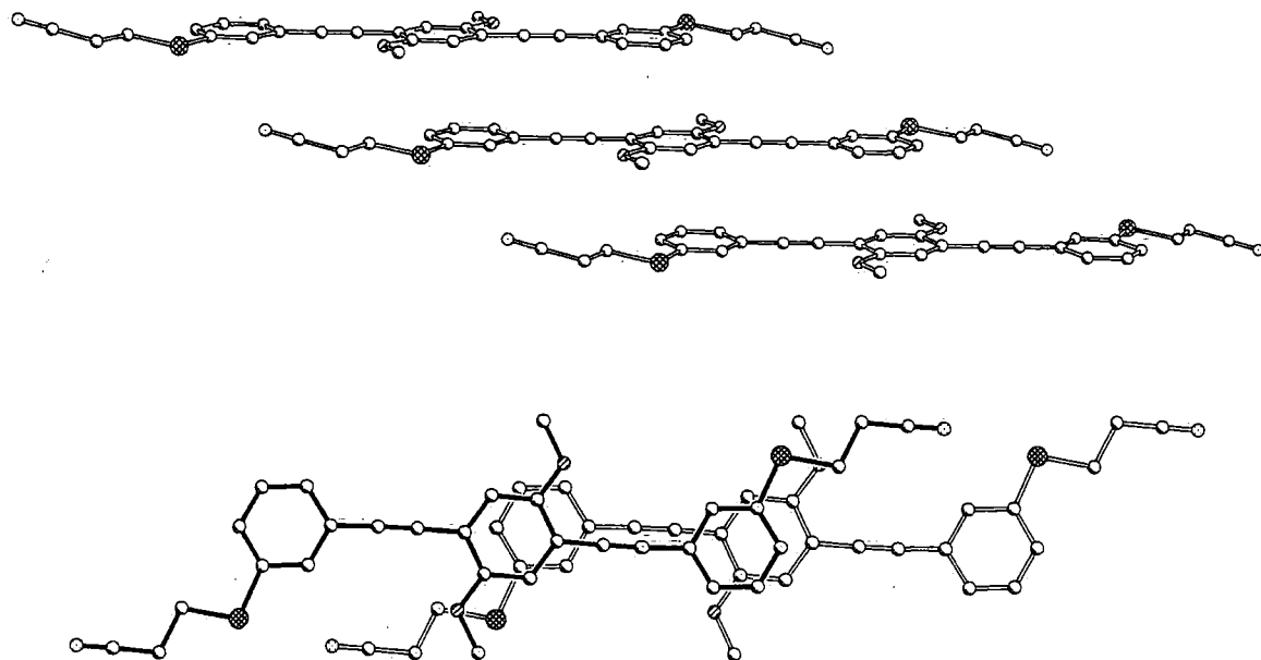
Figure 19. Crystal packing of 50 (RJ 39) , plane-centroid distance 3.57 and 3.60 Å, centroid-centroid distance 3.74 Å.
