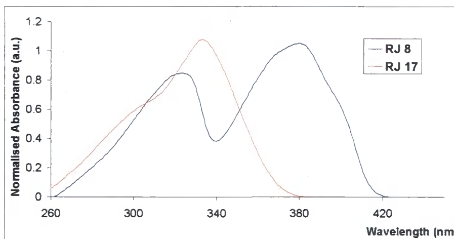
Figure 26. The UV-Vis absorption spectra of 35 (RJ 8) and 49 (RJ 17) in DCM solution.
