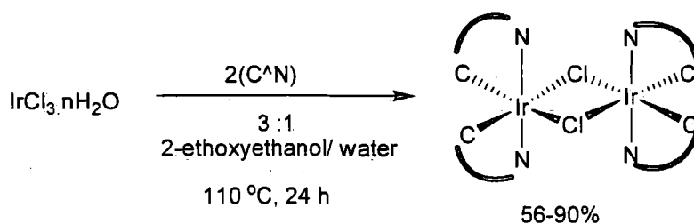
Scheme 26. The general synthesis of iridium(III) dimer complexes
