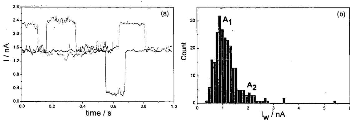
Figure 33. (a) I(t) method for compound RJ 32 showing typical current jumps. The corresponding histogram constructed from 250 jumps with I_0 = 1.5 to 5 nA and U_t = 600 mV is shown in (b).
