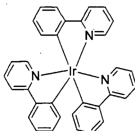
tris(2-phenylpyridine)iridium ( \text{Ir(ppy)}_3 )
