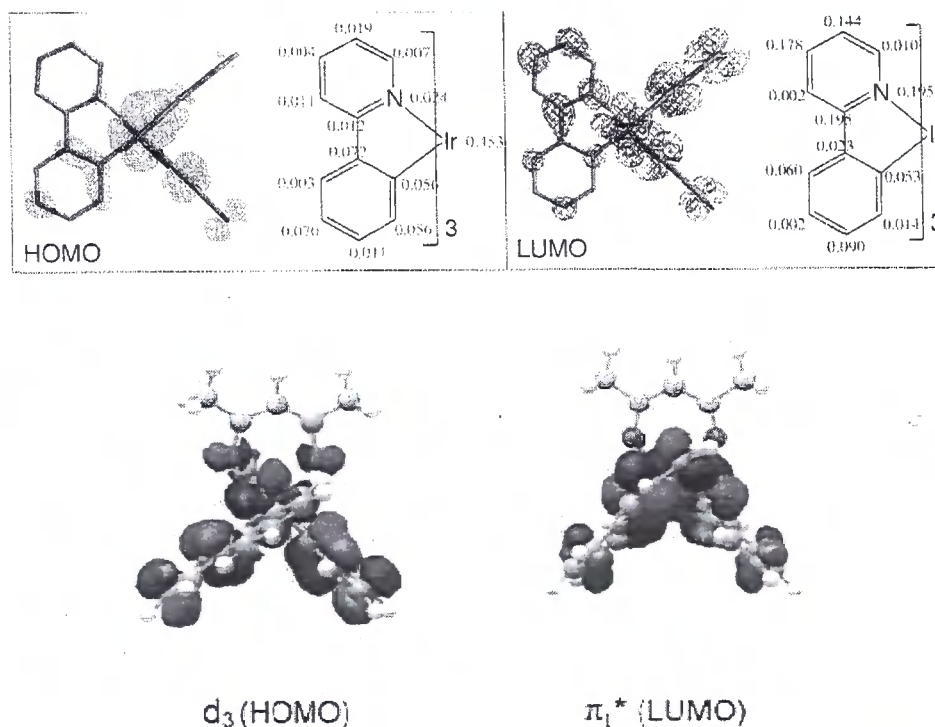
Figure 56. DFT derived orbitals of fac -Ir(ppy) 3 (top) and (ppy) 2 Ir(acac) (bottom). (from reference 160)
