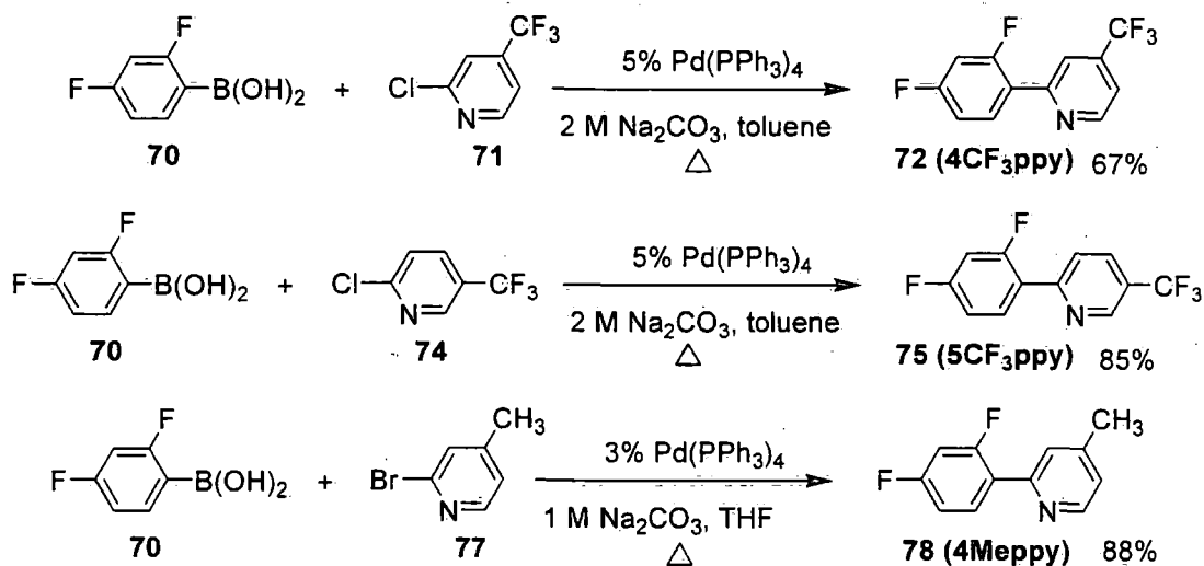
Scheme 23. The synthesis of 72 ( 4CF 3 ppy ), 75 ( 5CF 3 ppy ) and 78 ( 4Meppy )
