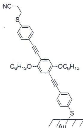
Figure 28. Molecular wire structure of 35 (RJ 8) with the terminal sulfur retaining the cyanoethyl group intact when assembled without the deprotecting agent.
