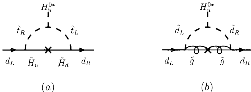
Figure 3.3: One-loop contributions to the \tilde{H}_u coupling with down quarks (a) via Higgsinos and (b) via gluinos which can lead to FCNCs. Flavour indices are suppressed.
