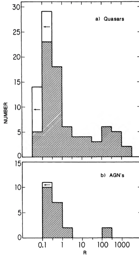
Figure 1.4: Distribution of the radio-loudness parameter, R , for quasars (top) and AGN (bottom). These distributions demonstrate a bimodality in R , with radio-loud AGN lying above R = 10 . Credit: Kellermann et al. (1989)
