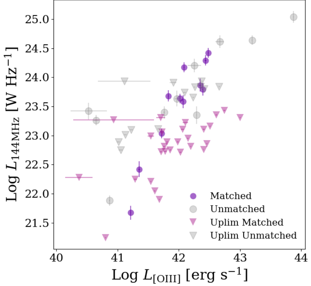
Figure 5.2: L_{144\text{MHz}} as a function of L_{[\text{OIII}]} , the coloured markers are from the L_{6\mu\text{m}} and redshift matched population I use in this analysis, and the grey are unmatched. L_{144\text{MHz}} in this figure is calculated at 0.3'' . Circles represent the detected AGN and downward triangles are the upper radio luminosity limits.
