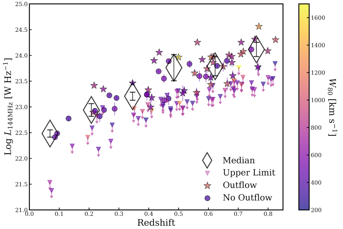
Figure 3.10: Relationship between L_{144\text{MHz}} and redshift with the W_{80} of [O III] traced with a colour map. Radio detected AGN are shown with either an outflow (small stars) or AGN with no outflow (circles). The median for five redshift bins are shown by large black hollow diamonds, with errors as the median absolute deviation. The upper limits for the radio non-detected AGN are shown by downward triangles.
