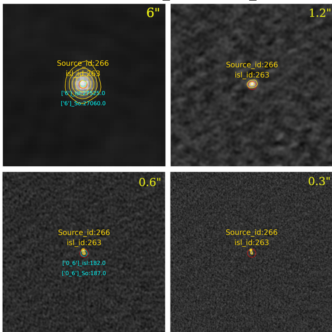
Figure 4.6: A montage of 60'' \times 60'' cutouts of the second component associated with the same source shown in Figure 4.5. See the caption of Figure 4.5 for more details on the cutouts.
