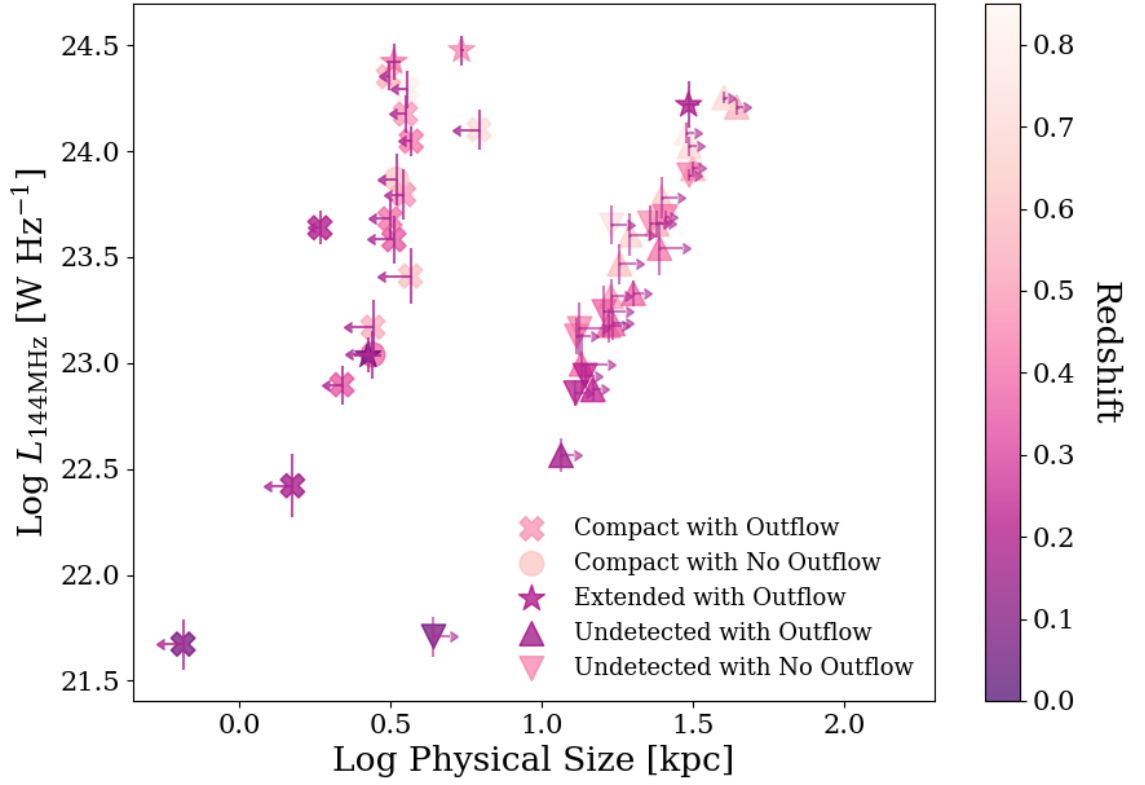
Figure 5.6: The relationship between the logarithm of the physical size, \log L_{144\text{MHz}} and redshift (as traced by a colour bar). I show compact sources with an outflow as crosses, compact source without an outflow as circles, extended AGN with outflows as stars, undetected AGN with an outflow as upward-pointing triangles, and undetected AGN without an outflow as downward-pointing triangles. The sizes of compact sources are upper limits, while the sizes for undetected AGN are lower limits.
