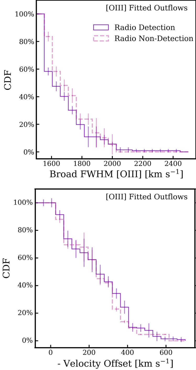
Figure 3.6: Further average cumulative distribution functions of [O III] properties. The solid purple step function shows the distribution for the radio detected AGN and the dashed pink line shows the information from the radio non-detected sources. Both panels have AGN with a second component fitted to [O III] and thus are in the [O III] fitted outflow category. Top : CDF of the broad component of [O III] FWHM. Bottom : Negative velocity offset of the broad component relative to the narrow component. Uncertainties are constructed using bootstrapping.
