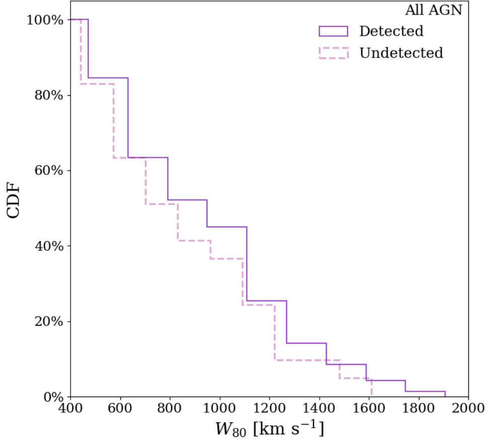
Figure C.2: Cumulative Distribution Function all AGN, regardless of outflow type comparing the W_{80} of detected and undetected AGN at 0.3''. The solid purple histograms show the results for the detected AGN and the dashed pink histogram portrays the undetected AGN.
