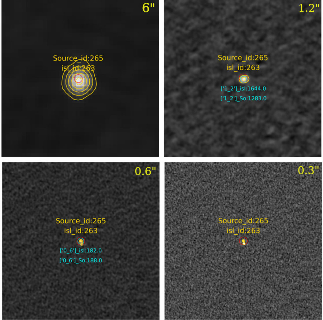
Figure 4.5: Example of a montage of 60'' \times 60'' cutouts used to associate components into a common source. For this case, two components detected at 0.3'' and 0.6'' are associated together. Top left: 6'' resolution image (see Figure 4.6 for source details). Top right: 1.2'' cutout. Bottom left: 0.6'' resolution cutout. Bottom right: 0.3'' resolution cutout. For the second component, information is provided in Figure 4.6. Contours are shown at the 5\sigma level. The source ID and island (isl) ID common across all resolutions are assigned to the 0.3'' component. Additional component information (in turquoise and smaller font) is shown on the respective resolution image. The red circle is centred on the component position at 0.3'' in each cutout, and the turquoise circle is the component location for the relevant resolution image
