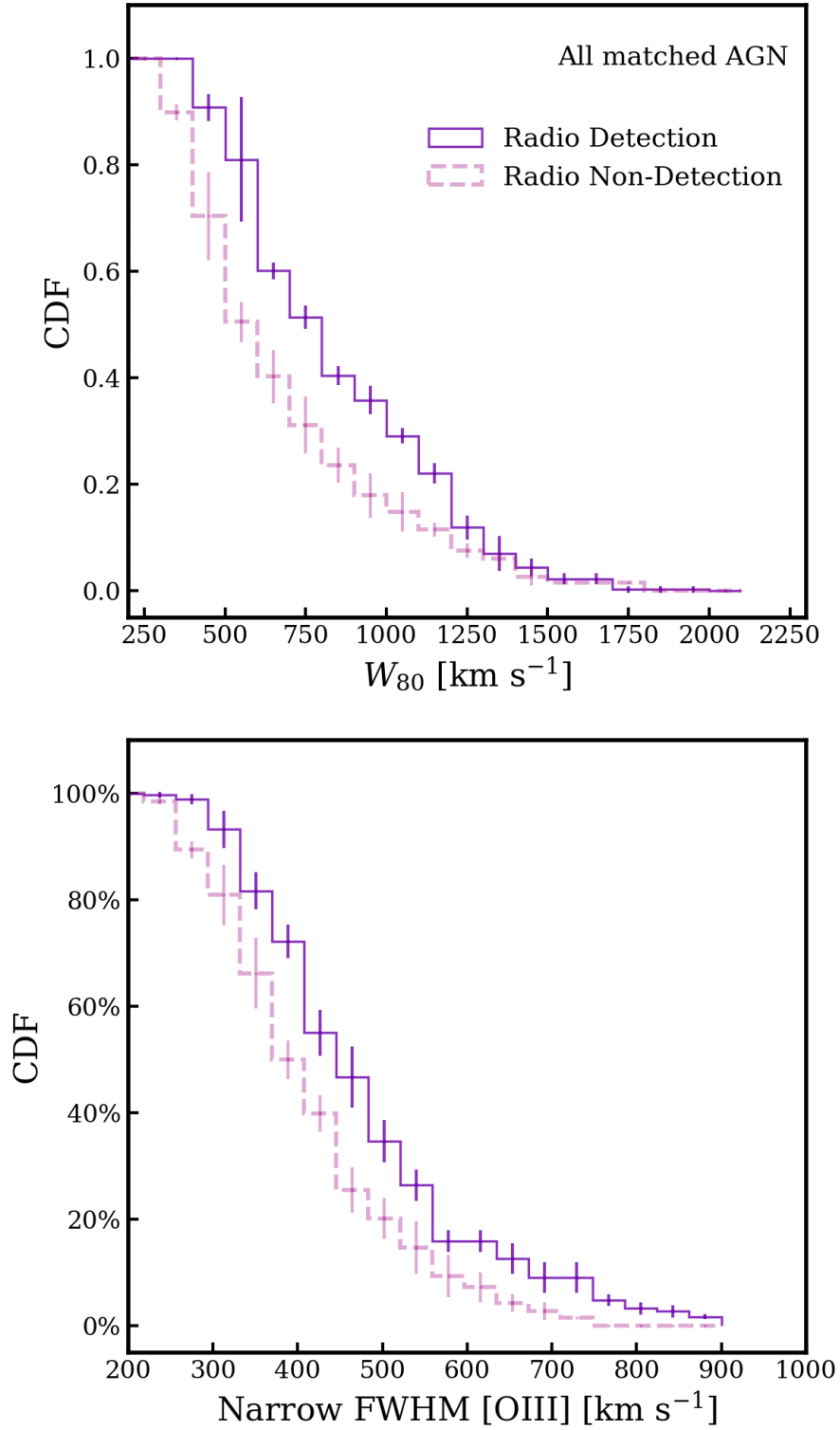
Figure 3.5: Average cumulative distribution functions of [O III] properties. The solid purple step function shows the distribution for the radio detected AGN and the dashed pink line shows the information from the radio non-detected sources. Top : Average CDFs of W_{80} [O III] showing the results from all 1000 matching iterations. Bottom : Average CDFs of the FWHM of the narrow component of [O III] with the all matching iterations. Uncertainties are constructed using bootstrapping.
