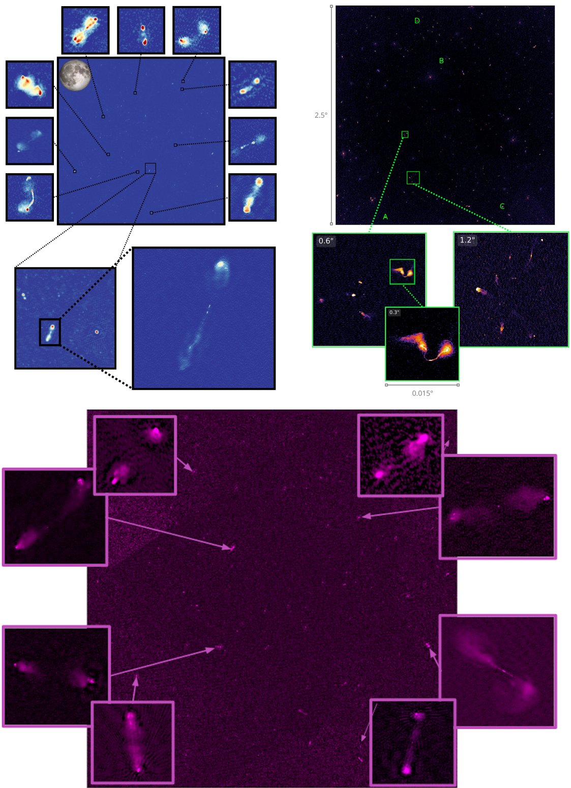
Figure 4.7: Here I show the three, wide-field sub-arcsecond resolution images of the LoTSS Deep Fields released in DR1. Top left : Lockman Hole (Sweijen et al., 2022). Top right : ELAIS-N1 (de Jong et al., 2024). Bottom : Boötes.
