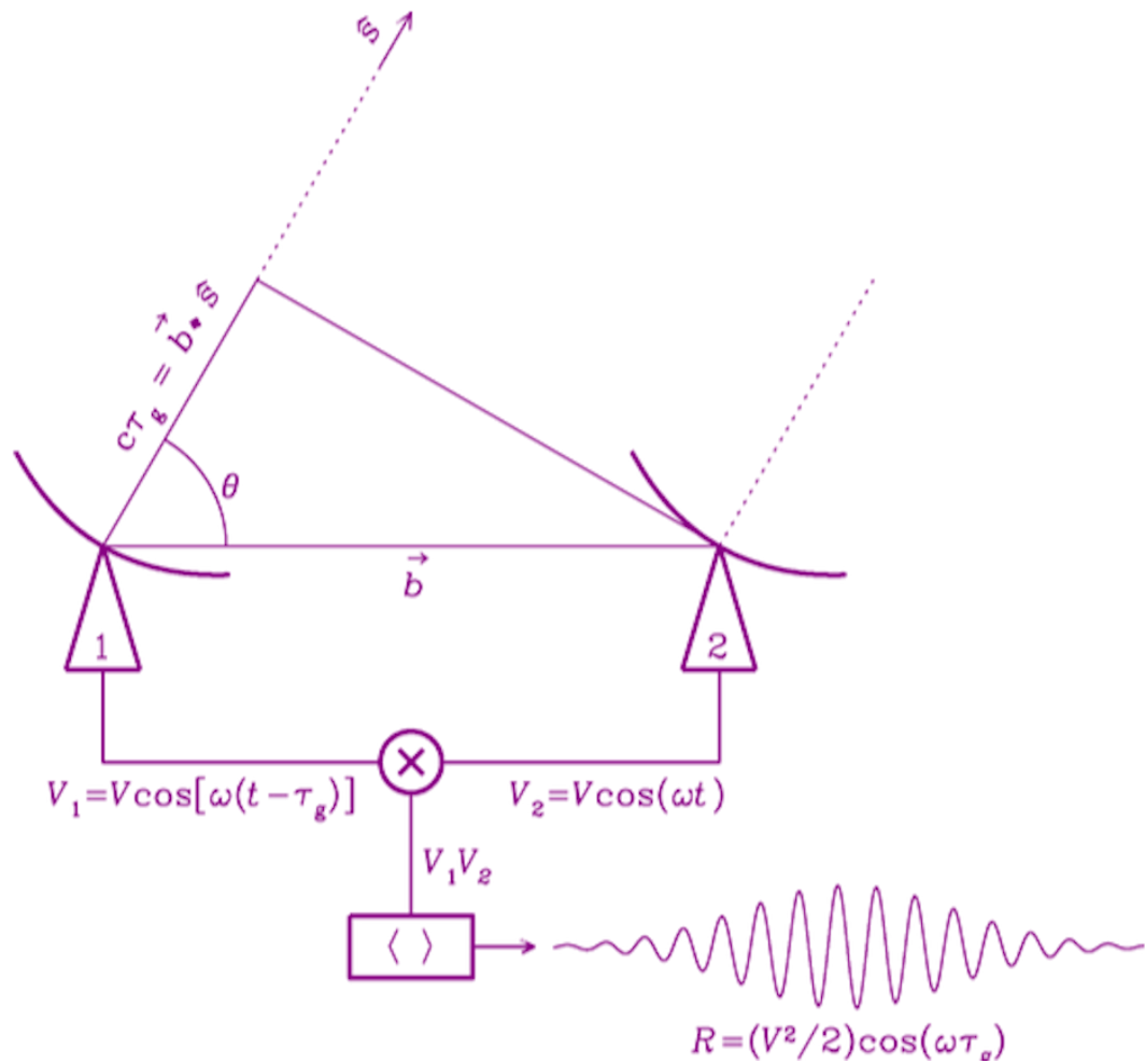
Figure 2.2: Diagram demonstrating the components of a two telescope interferometer, with baseline b . Credit: Adapted from NRAO.
