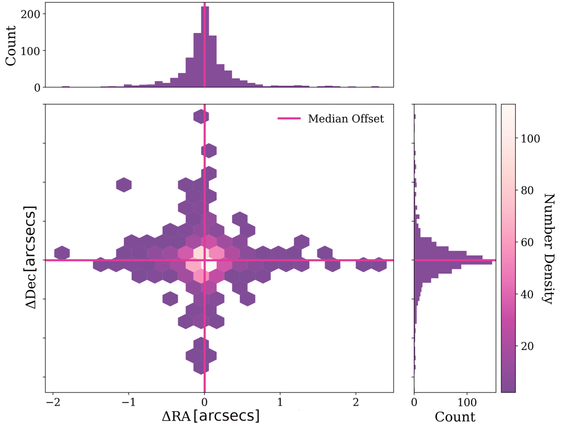
Figure 4.4: The relationship between \Delta RA and \Delta Dec after applying the astrometry correction. I calculate the offset by subtracting the 0.3'' positions from the 6'' LoTSS positions. The sources shown are high-SNR, compact objects I select to measure the astrometric correction for each facets. Each hexbin contains at least two sources, with the colour scale tracing the number density. The pink lines indicate the median values of \Delta RA and \Delta Dec , which cross near zero for both axes, as expected.
