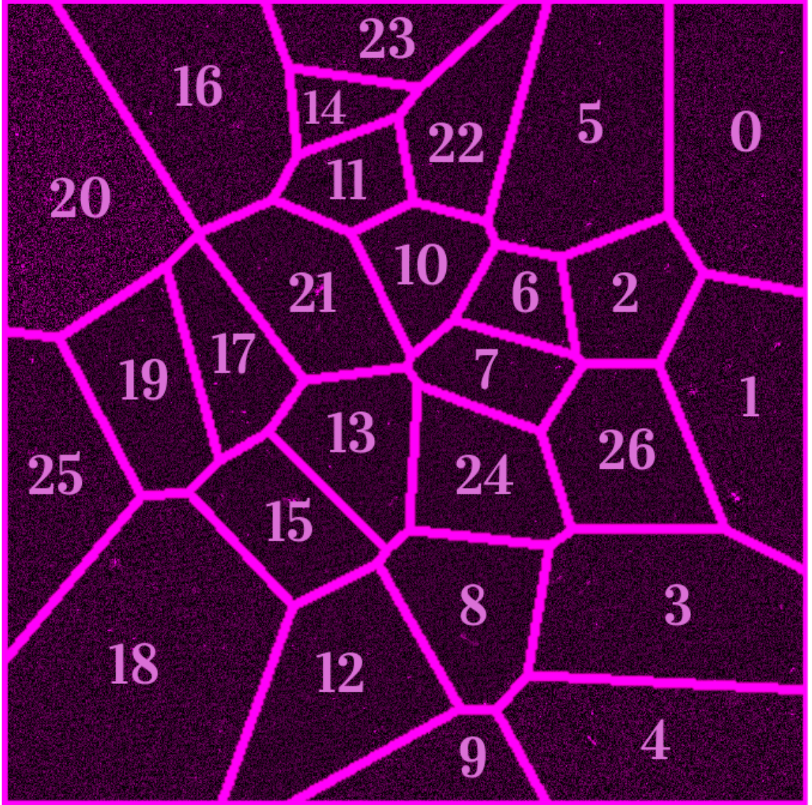
Figure 4.2: The layout of the 27 facets I use to produce the sub-arcsecond resolution, wide-field, images of the Boötes Deep Field. The background is the \sim 0.3'' image and facet 20 has a higher level of noise due to an extra flux scale correction required for this facet.
