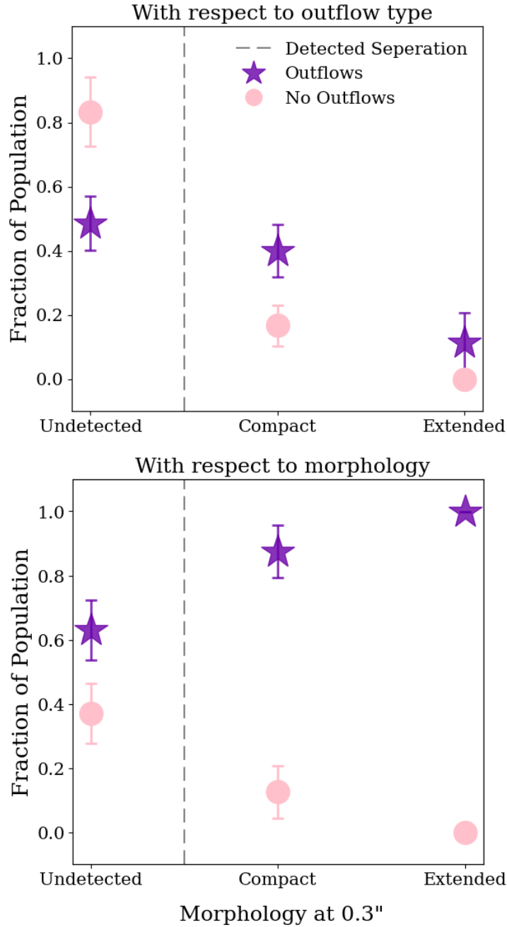
Figure 5.5: Fraction of population in relation to sub-arcsecond low-frequency radio morphologies, where a radio source is classified as either undetected, compact, or extended. Top: Distribution of morphology with respects to outflow population, i.e. for each outflow population, the fractions of different morphology categories add up unity. Bottom: Distribution of outflow population with respects to the morphology category, i.e. for each morphology class, the fractions of the outflow population adds to unity. The pink circle markers demonstrate the no outflow population and the purple stars represent the outflowing population. In cases where the fraction of the population is either zero or one, the uncertainty is omitted. The grey dashed line separates the undetected AGN from the detected AGN.
