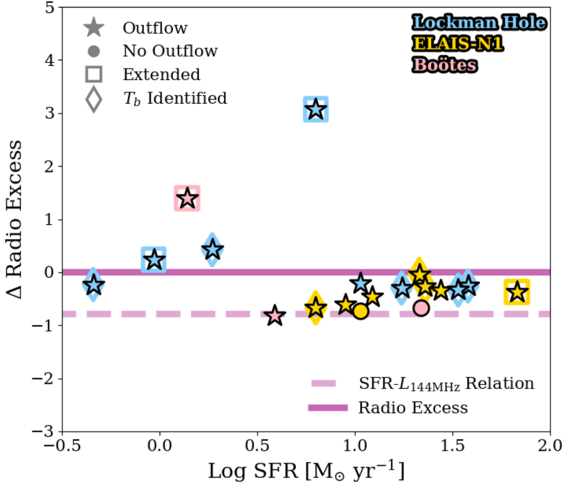
Figure 5.7: The relationship between \Delta radio excess and \log \text{SFR} . Only sources with a detection at 0.3'' contribute to this figure. The pink solid line is the radio excess divide which is centred at y = 0 , with the \text{SFR} and L_{144\text{MHz}} relation as the dashed pink line. I define these relations using the Boötes field (pink), and hence I scale sources within Lockman Hole (blue) and ELAIS-N1 (yellow), which have a different radio excess definition, to match the Boötes definition. Star markers represent AGN with outflows and circular markers show AGN without outflows. Markers surrounded by a square have an extended morphology and sources with a diamond around them are confirmed AGN cores using brightness temperature measurements.
