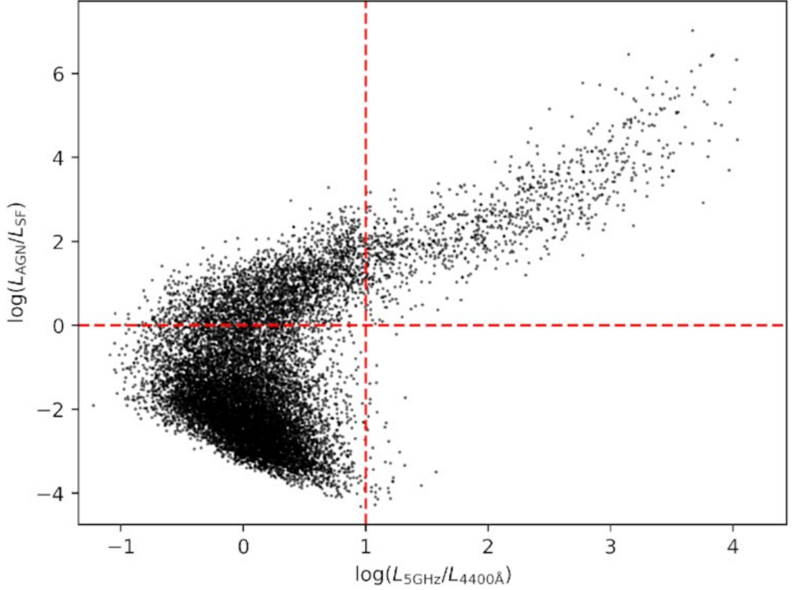
Figure 1.5: The logarithmic relationship between radio-loudness ( L_{5\text{GHz}}/L_{4400\text{\AA}} ) and jet dominance ( L_{\text{AGN}}/L_{\text{SF}} ). The traditional radio-loudness divide is marked at \log R = 1 , while the horizontal divide at \log(L_{\text{AGN}}/L_{\text{SF}}) = 0 indicates the transition to AGN-dominated jets. This illustrates that, for this population of modelled data points, radio-quiet AGN can, in fact, be jet dominated. Credit: Macfarlane et al. (2021).
