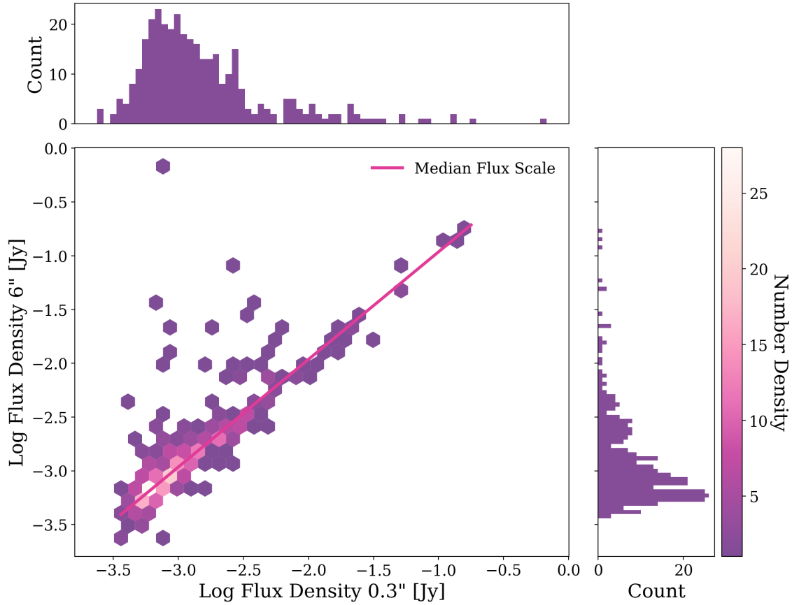
Figure 4.3: The relationship between the log flux density at 0.3'' and 6'' from LoTSS. The 0.3'' flux densities have been scaled by the final correction of 1.02. The sources contributing to this figure are high SNR, compact sources I select to measure the universal flux density scale required for Boötes. The top histogram shows the distribution of log flux densities at 0.3'', while the right histogram shows the distribution at 6''. The pink link indicates the median flux scale between these flux densities. Each hexbin contains at least one source, with the number density represented by the colour scale.
