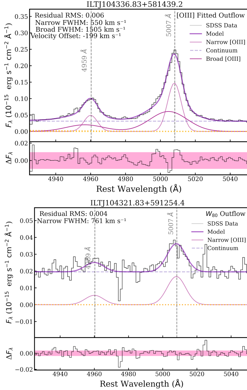
Figure 3.2: Example spectra for two categories of the [O III] SDSS spectral fitting results. The top panel of each subplot represents the SDSS spectral data in black, alongside the MCMC fitting results. The dark purple solid lines shows the final MCMC fitting result. The pink Gaussians represent the narrow component to [O III] and the Gaussians in magenta, if plotted, is the broad component of [O III] which implies an outflow is occurring. The light pink dashed lines, where present, shows the Fe II template used when modelling the data and finally the grey or yellow dashed lines shows the continuum. The lower panel of each subplot shows the residuals of the fit of the model to the SDSS data. The pink shaded region corresponds to rms 1\sigma region, calculated over the full spectral range of the model. This figure contains AGN from the radio detected population so the titles are the LoTSS source names. The top spectra shows an example of an AGN within the [O III] fitted outflow population and the bottom spectra shows an AGN undergoing a W_{80} outflow.
