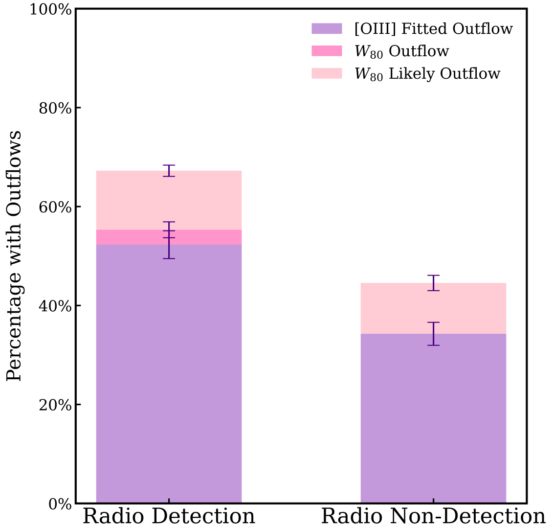
Figure 3.4: The stacked bar chart represents the average outflow detection rates from all 1000 iterations of randomly matching the radio detected AGN to the radio non-detected AGN. The light pink bar showing the W_{80} likely outflows, the darker pink is the W_{80} outflows, and the purple is the [O III] fitted outflows. For the radio detected AGN, 52.3 \pm 2.8\% have an [O III] fitted outflow, 3.0 \pm 1.6\% have W_{80} outflows, 11.9 \pm 1.1\% W_{80} likely outflow, and 32.8 \pm 2.5\% showing no signs of an outflow. In the same order the results for the radio non-detected AGN is, 34.3 \pm 2.3\% , 0.0 \pm 0.0\% , 10.3 \pm 1.5\% and 55.4 \pm 2.4\% .
