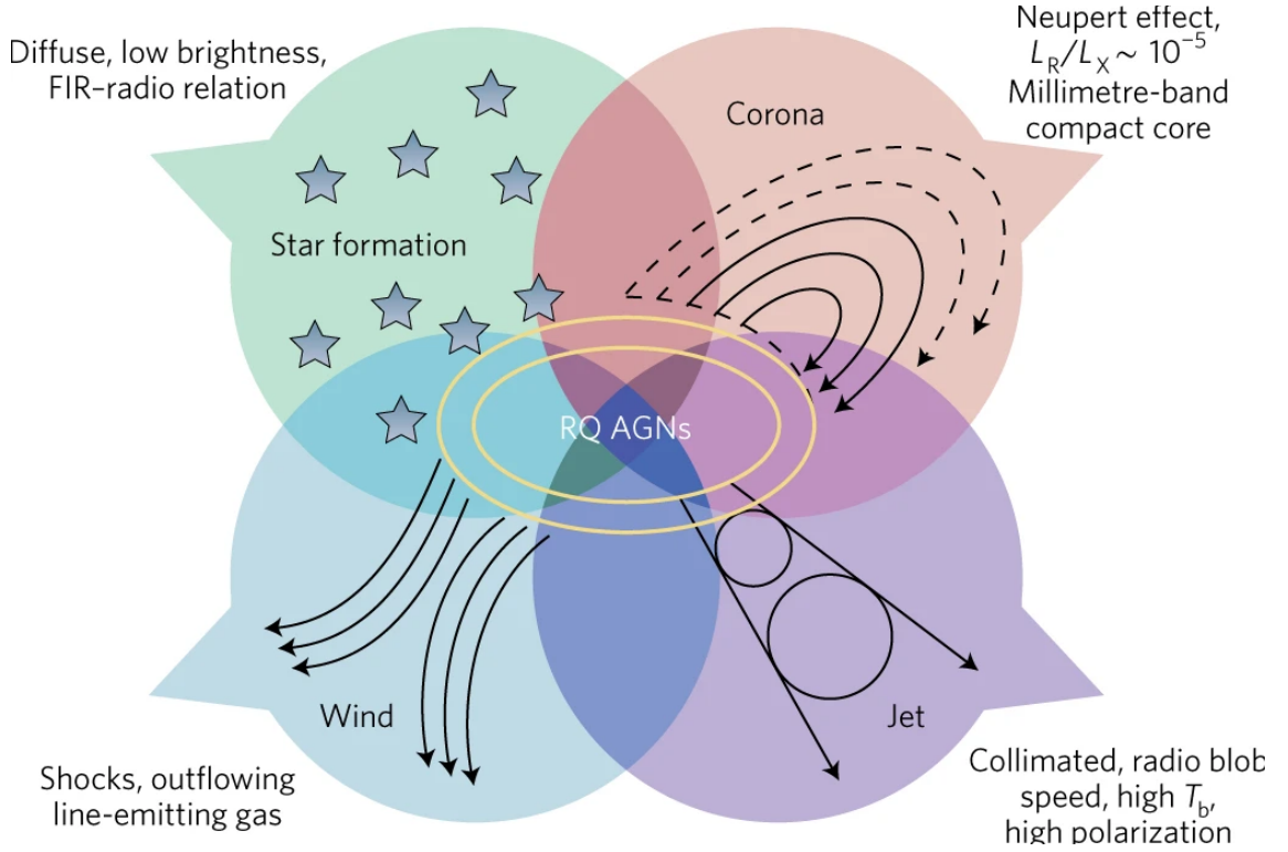
Figure 1.7: Schematic demonstrating the possible main physical mechanisms driving the radio emission from radio-quiet AGN. Credit: Panessa et al. (2019).
