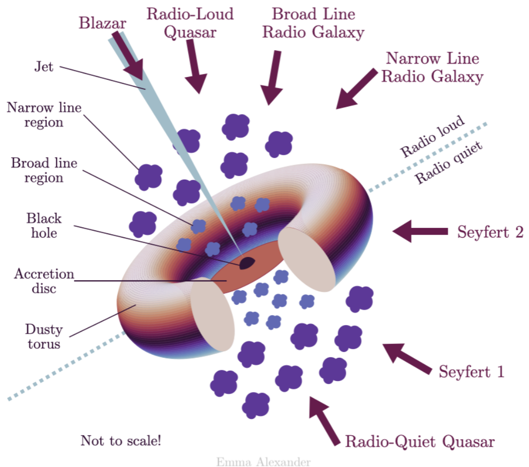
Figure 1.2: Schematic of the AGN unification model, illustrating the key components of an AGN. The central region contains the SMBH, accretion disk, and broad-line region, all surrounded by a dusty torus. Further from the centre are the narrow-line region and a radio jet originating from the central SMBH. The diagram also highlights that the observed type of AGN depends on the observer's viewing angle, e.g., Seyfert 1, Seyfert 2, and blazar. Credit: Emma Alexander.
