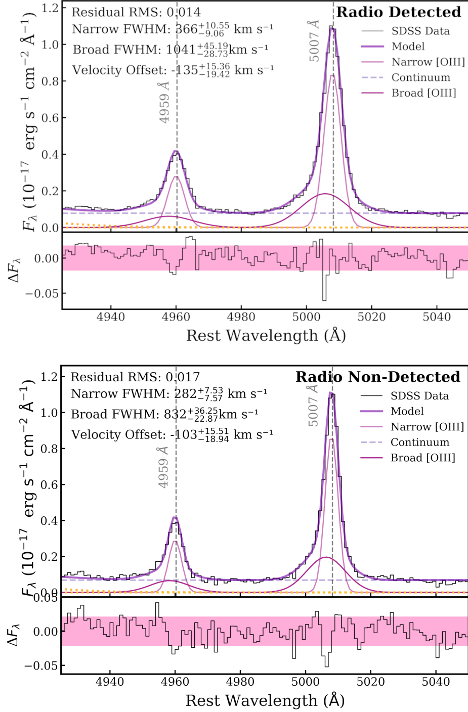
Figure 3.8: Composite spectra which are normalised by the peak of the narrow [O III] component and are produced from the closest matched L_{6\mu\text{m}} and z run, containing 59 AGN in each population with the MCMC fitting tool results applied. Top : Radio detected AGN. Bottom : Radio non-detected AGN. The bottom panel shows the residuals of the fits with 1\sigma of the residuals highlighted in the pink region. In the upper panel, the purple solid line shows the fit from the MCMC code to the SDSS data which is shown in back. The magenta line shows the broad component of [O III] with the pink Gaussians representing the narrow component of [O III].
