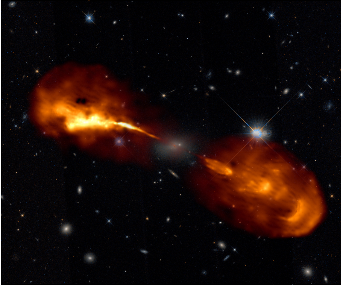
Figure 1.6: Sub-arcsecond resolution radio image of Hercules A at 144 MHz obtained with the ILT, overlaid on optical counterparts from the Hubble Telescope. This radio galaxy hosts one of the most powerful radio jets in the sky and is a poster child of radio-loud AGN. Credit: R. Timmerman.
