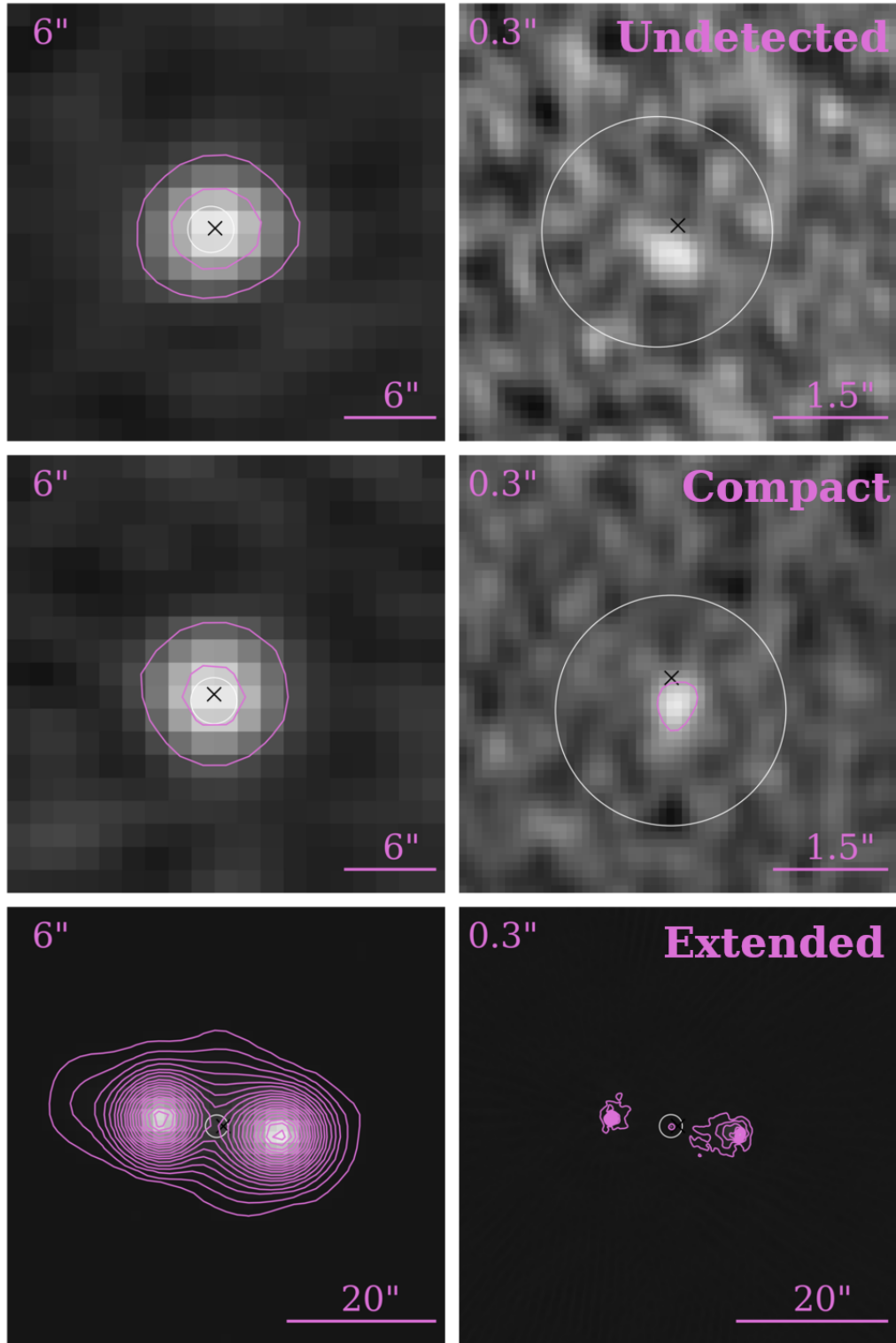
Figure 5.3: Demonstration of the morphology definitions in this work. Left: 6'' resolution, right: 0.3'' resolution. Top: Example of an “undetected” source, which does not have a 5\sigma detected at 0.3'' but is detected at 6''. Middle: A “compact” morphology. Bottom: “Extended” source. The black cross represents the LoTSS position, the white circle is the SDSS fibre and the contours are at a 5\sigma level.
