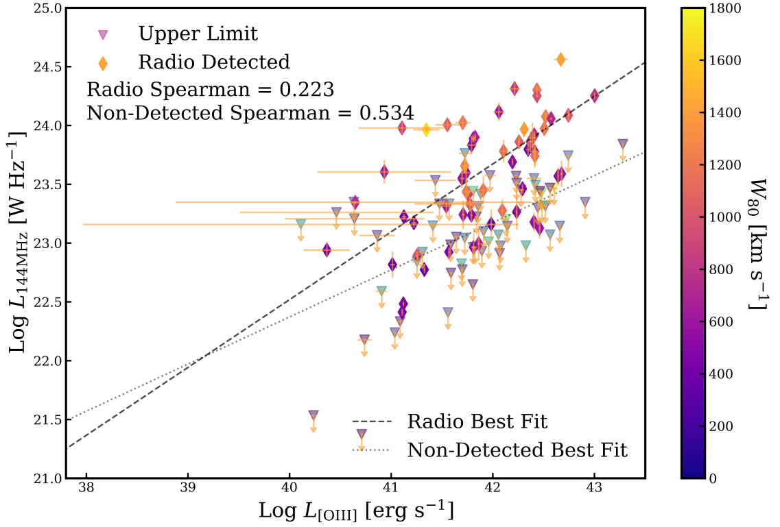
Figure 3.11: L_{144\text{MHz}} as a function of total L_{[\text{OIII}]} with the W_{80} traced by a colour scale. Radio detected AGN are plotted with diamonds and the upper limits for the radio non-detected AGN are shown by the downward triangles. The dashed black line show the best fit relationship for the radio detected AGN and the grey dotted line shows the best fit to the upper limits of the radio non-detected population.
