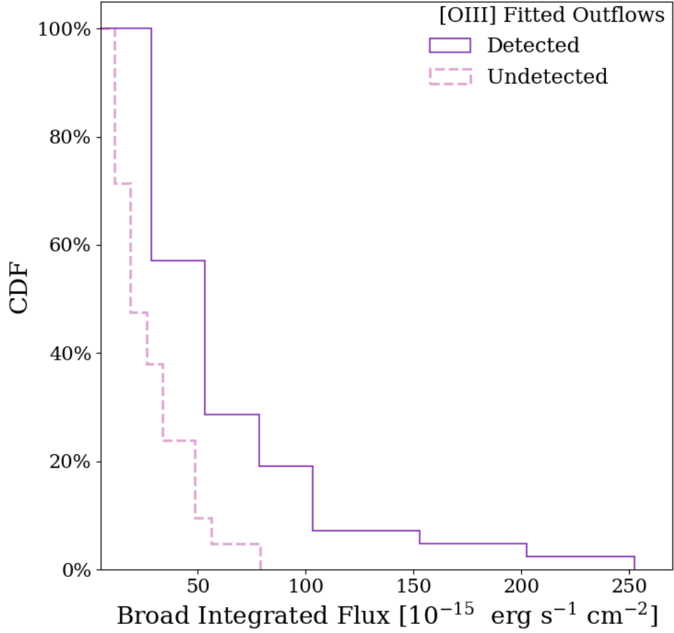
Figure C.1: Cumulative Distribution Function AGN with an [O III] fitted outflow comparing the integrated flux of the broad component fitted to [O III] of detected and undetected AGN at 0.3". The solid purple histograms show the results for the detected AGN and the dashed pink histogram portrays the undetected AGN.
