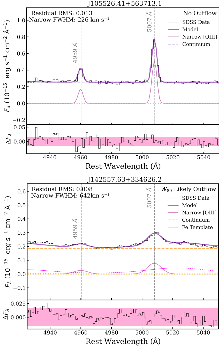
Figure 3.3: Example spectra for the other two categories of the [O III] SDSS spectral fitting results. See the caption for Figure 3.2 for details. The AGN in this figure are from the radio non-detected population so the titles are the SDSS names. The top spectra shows the spectra of an AGN within our no outflow category and the bottom spectra shows an example of an AGN which hosts a W_{80} likely outflow.
