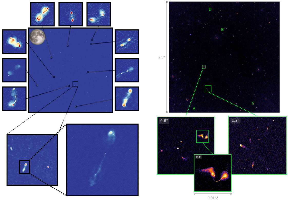
Figure 2.4: The two previously published wide-field 144 MHz sub-arcsecond resolution images of Lockman Hole (left credit: Sweijen et al., 2022) and ELAIS-N1 (right credit: de Jong et al., 2024).
