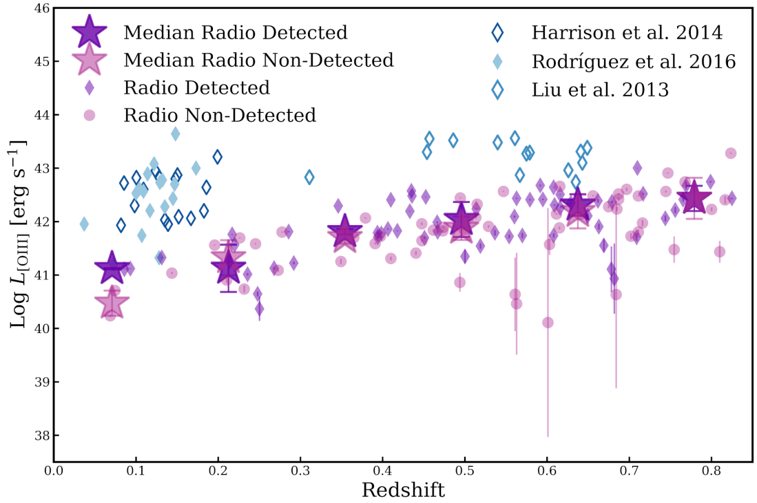
Figure 3.9: Total \lambda 5007 \text{ \AA} L_{\text{OIII}} as a function of redshift. The star markers show the median values for six redshift bins, with purple indicating the median for the radio detected AGN, and pink for the radio non-detected AGN. The errors are the median absolute deviation. For the background sources, the purple diamonds show the radio detected population and the pink circles show the radio non-detected AGN. Similar studies are presented with various blue diamond markers.
