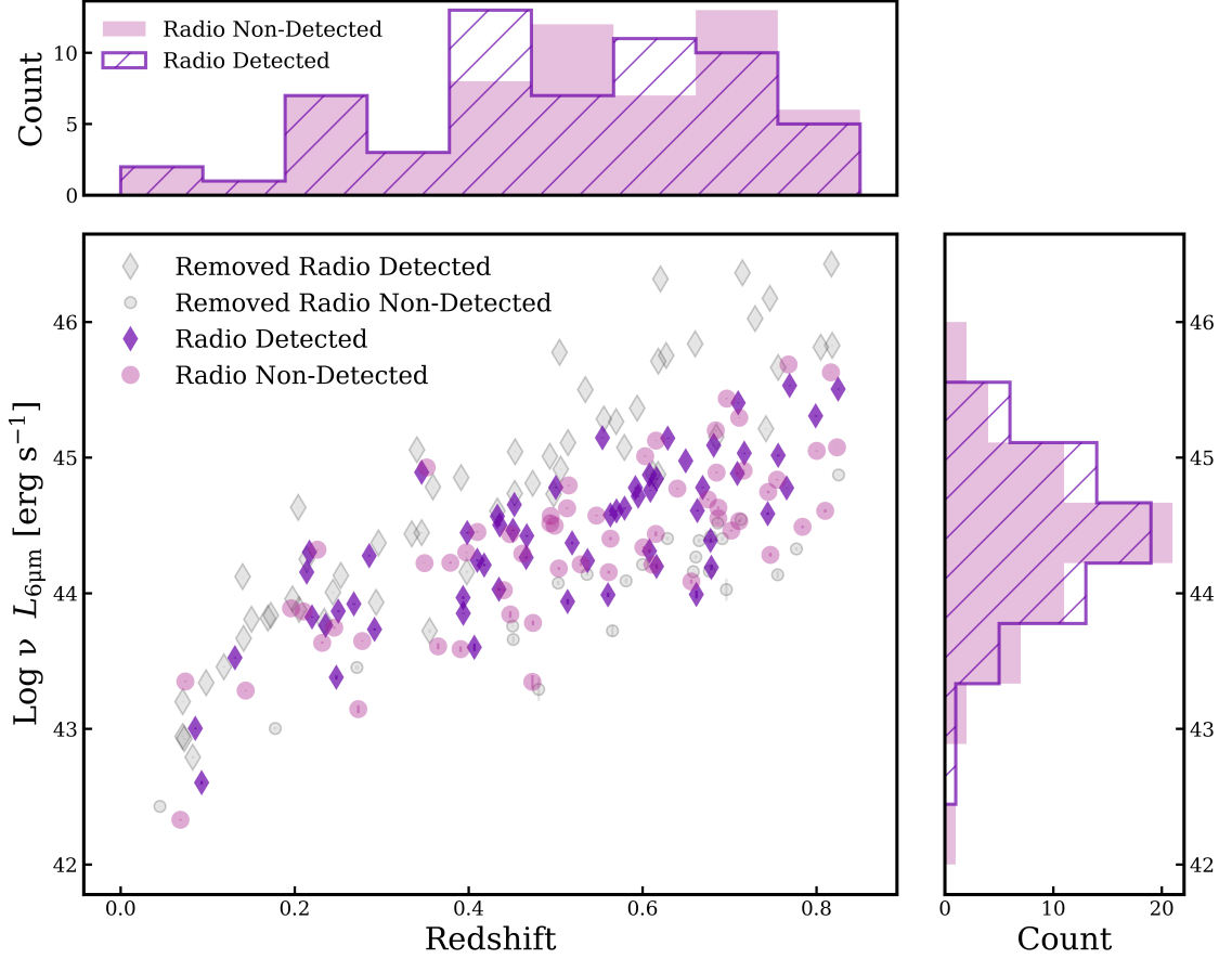
Figure 3.1: The L_{6\mu\text{m}} and redshift relation of our radio and radio non-detected populations. The coloured markers show one iteration from the 1000 trials to match a radio detected AGN (purple diamonds) in L_{6\mu\text{m}} and redshift to a radio non-detected AGN (pink circles). The grey points represent the AGN which, in this iteration, are removed as these are unmatched, with diamonds portraying the radio detected AGN, and circles for the radio non-detected AGN. The top histogram conveys the redshift distribution and the right histogram is the distribution of L_{6\mu\text{m}} . The hashed purple histogram is the radio detected AGN and the pink solid histogram are the radio non-detected AGN, showing they present similar distributions.
