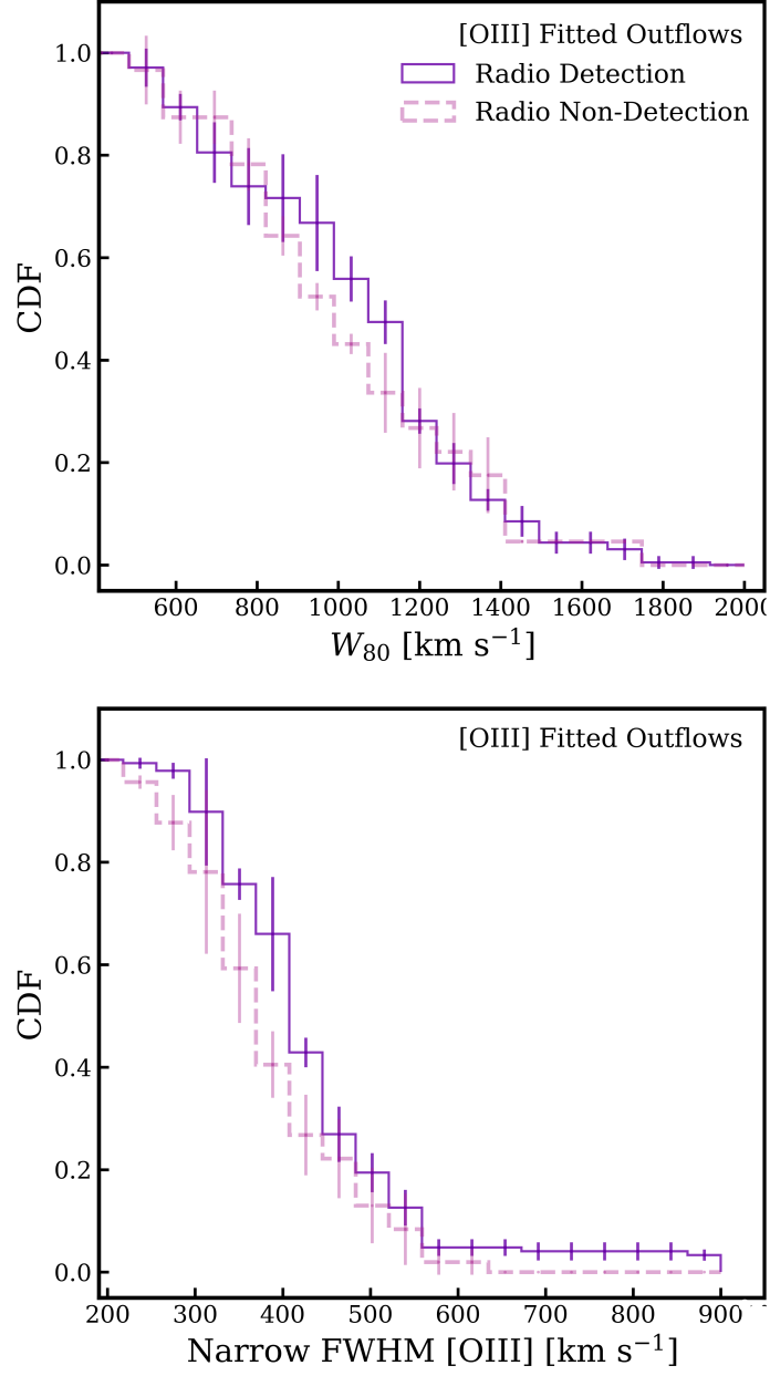
Figure A.1: Further average cumulative distribution functions of [O III] properties. The solid purple step function shows the distribution for the radio detected AGN and the dashed pink line shows the information from the radio non-detected sources. Top: CDFs of W_{80} [O III] showing the results only AGN which are fitted with a second component. Bottom: CDFs of the FWHM of the narrow component of [O III] with only AGN which are fitted with a second component. The uncertainties presented are as a result of bootstrapping.
