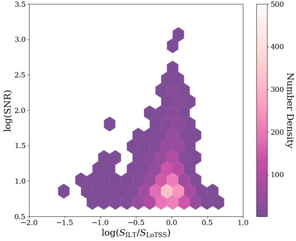
Figure B.1: The SNR of the \sim 0.3'' resolution image as a function of the ratio between the flux density at 0.3'' ( S_{\text{ILT}} ) and flux density at 6'' ( S_{\text{LoTSS}} ), where we trace the number density with the colour bar. For a hexagon to be plotted, at least 2 sources must lie within the bin.
