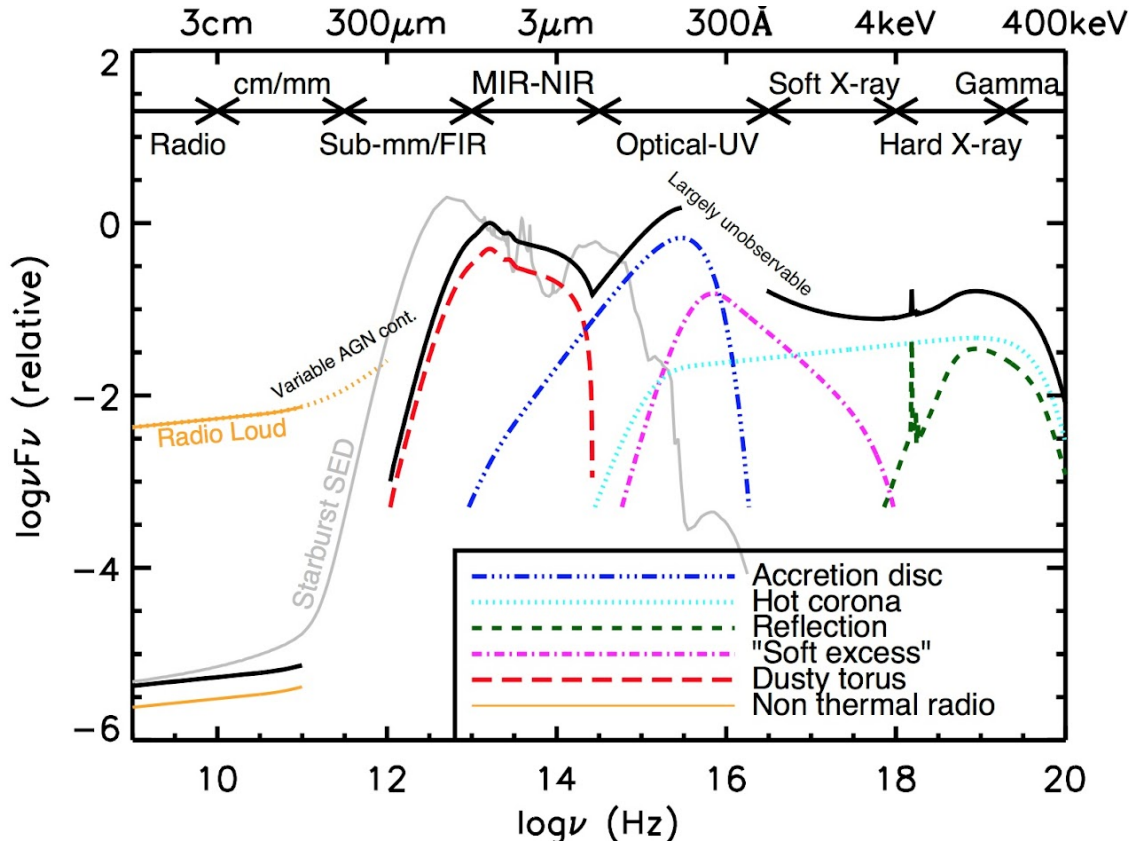
Figure 1.3: Schematic SED of a typical unobscured AGN. The black solid line represents the overall SED, while the coloured line with different styles shows the contributions of individual AGN components, such as the accretion disc and dusty torus, to the total emission. Credit: Harrison (2014).
