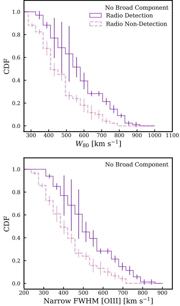
Figure A.2: Further average cumulative distribution functions of [O III] properties. The solid purple step function shows the distribution for the radio detected AGN and the dashed pink line shows the information from the radio non-detected sources. Top : CDFs of W_{80} [O III], all AGN which are fitted with a single Gaussian. Bottom : CDFs of the FWHM of the narrow component of [O III] with only AGN which are fitted with a second component. The uncertainties presented are as a result of bootstrapping.
