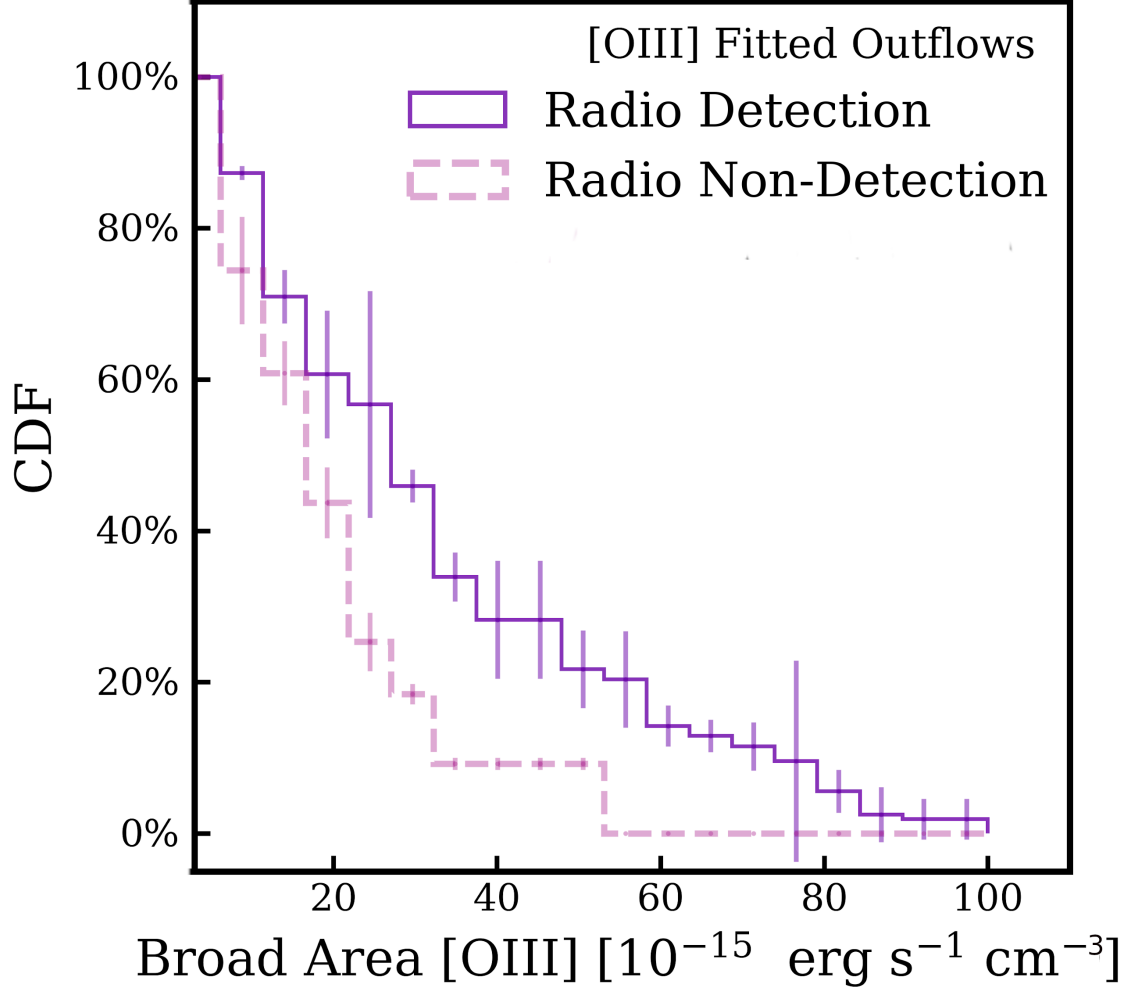
Figure 3.7: Average cumulative distribution function of the area of the broad component fitted to [O III], calculated using the peak and FWHM of the broad component. The solid purple step function shows the distribution for the radio detected AGN and the dashed pink line shows the information from the radio non-detected sources. AGN contributing to this figure have a second component fitted to [O III] and uncertainties are constructed using bootstrapping.
