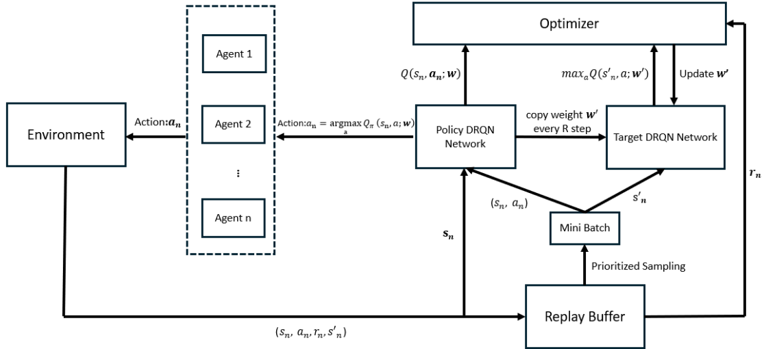
Figure 4: Reinforcement Learning Overview Diagram (DRQN)
