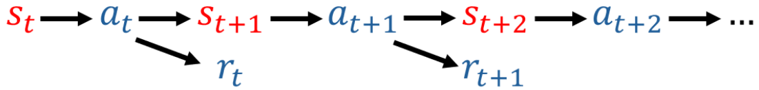
Figure 5: Interaction Process Between Agent and Environment
