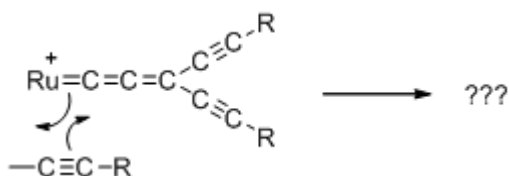
Scheme 31 Possible intermolecular alkyne attack
