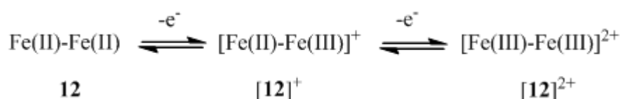
Figure 20 Equilibria between 12 , [\mathbf{12}]^+ and [\mathbf{12}]^{2+} .
