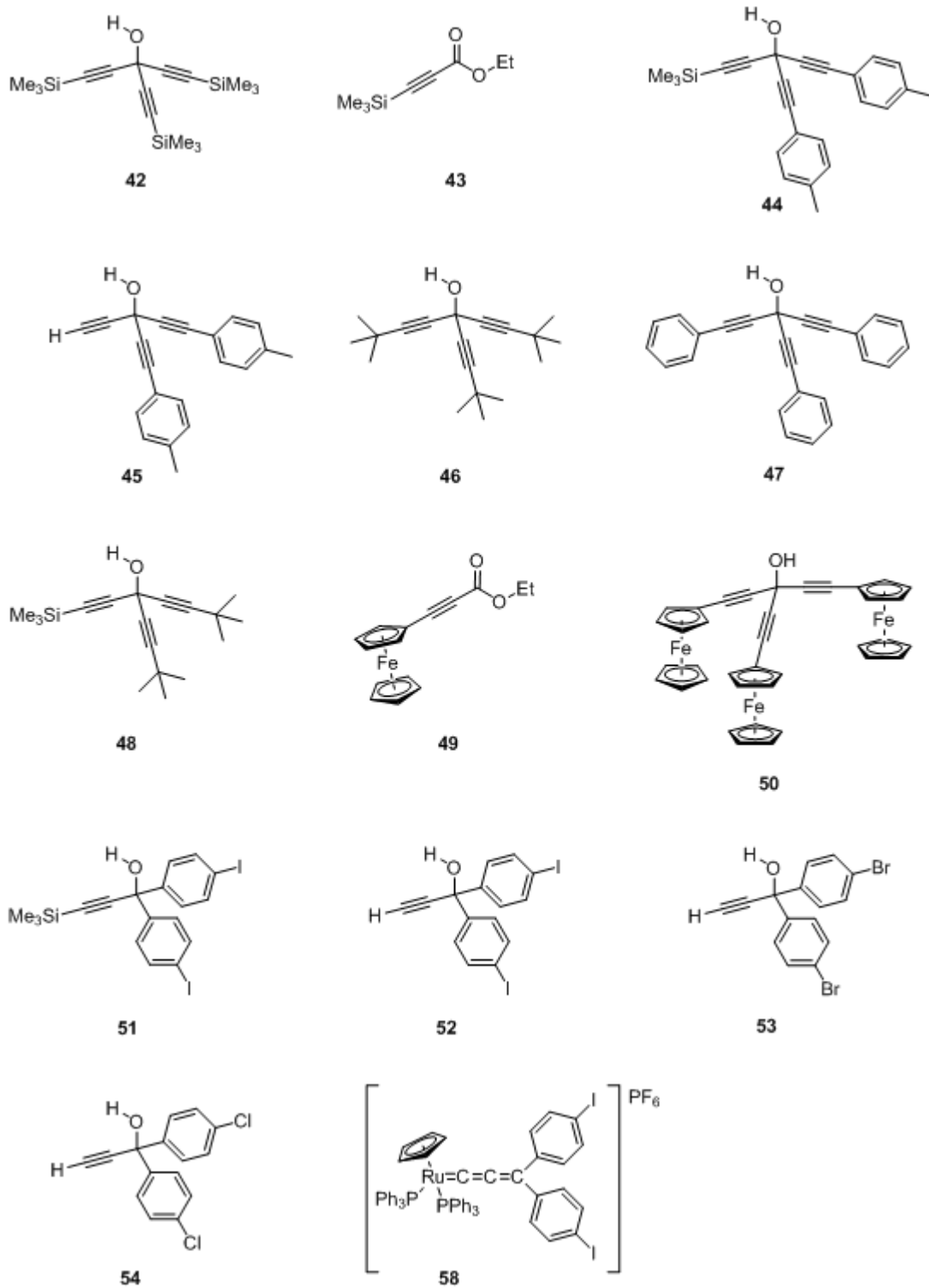
Chart 11 The acetylenic esters and triethynyl methanols prepared or discussed in this Chapter.
