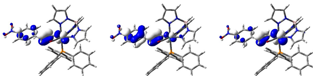
Figure 46 Contour plots: left; HOMO of 25-H , centre; \alpha -HOSO, right; \beta -LUSO of [25-H]^+ .
