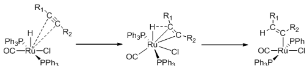
Scheme 9 Alkyne attack to the metal centre in the H-M-Cl quadrant. 272
