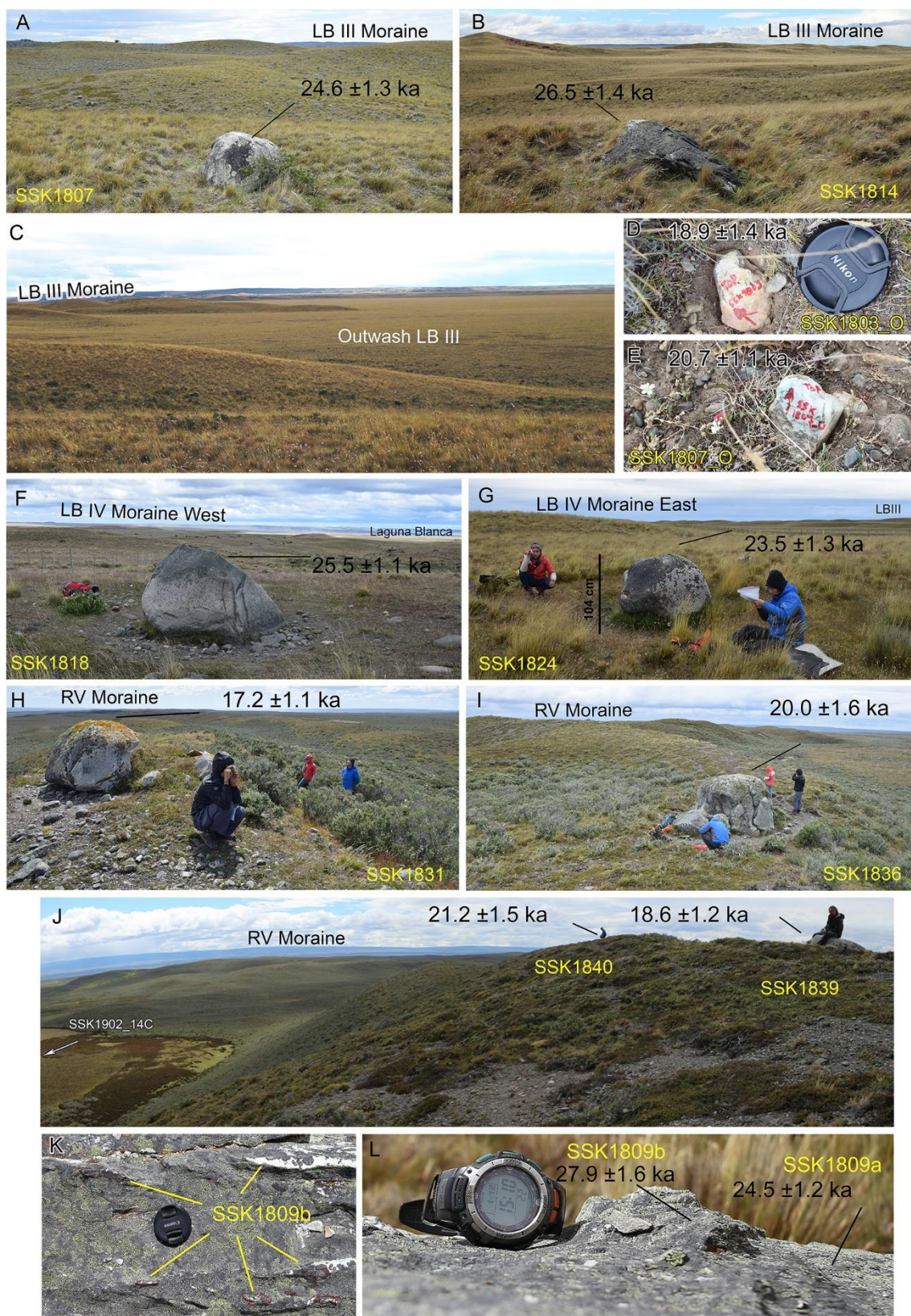
Figure 2.4. Examples of moraine boulder samples and outwash cobbles collected. A,B) Moraine boulders from LB III. C) LB III outwash. D,E) Cobbles collected from LB III outwash. F,G) Laguna Blanca IV. H–J) RV moraine. K,L) Sample SSK1809 showing the sampled quartz vein and sampled boulder surface.
