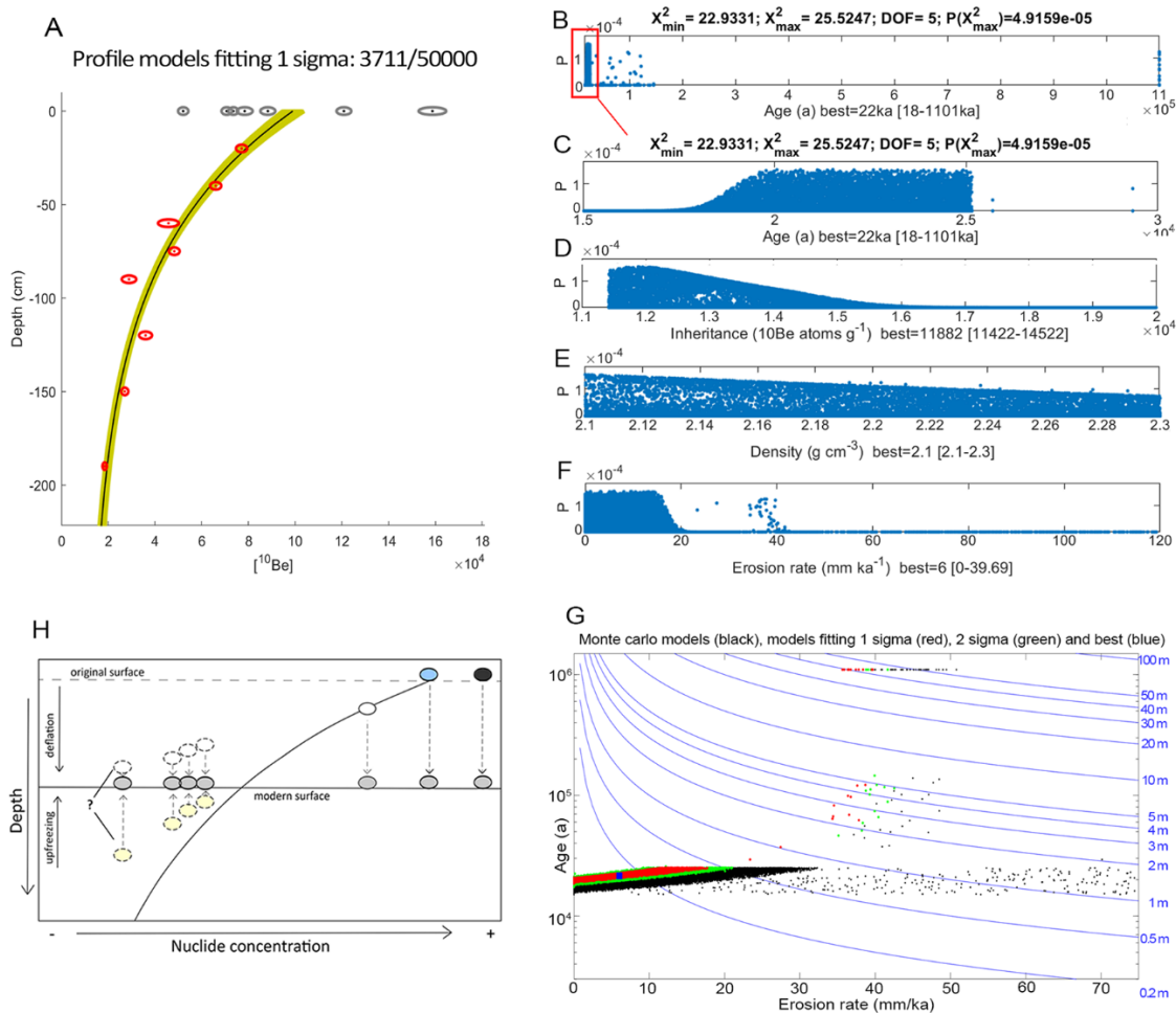
Figure 2.9. Depth profile model results from outwash deposit located in Otway ice lobe, associated with the southeastern Laguna Blanca spillway. A) Plot of ^{10}\text{Be} concentration of samples from the surface (grey circles) and depth profile (red circles), with their uncertainties as a function of depth. Green lines indicate the model results that fit within 1 sigma, the black line corresponds to the best fit model. B–F) Probability density distributions of the different outputs of the model: age, inheritance, density, and erosion rate. B) Shows the modelled ages plotted between 0–1,101 ka, whereas C) shows the ages plotted between 15–30 ka. G) Graphic showing relationship between age, erosion rate, and surface lowering. Red dots are model runs lying within 1-sigma of the data, green are those within 2-sigma, and black dots are other model runs. Model output shows 99.5% of data within 1-sigma lie within an age range of 18.6–25.1 ka, with a small component of well-fitting model runs that would require implausible (40–50 m) amounts of surface lowering. H) Schematic cartoon to explain scattered age of the surface samples and reasons for their difference in age from the depth profile modelling. The older samples could have been exposed to the cosmogenic radiation from the outwash terrace formation (blue sample). If the samples have a component of inheritance from earlier exposure, then the age will be older than the terrace (black sample). A deflation of the outwash will expose samples that were initially buried, resulting in younger than the outwash age (white). Younger samples could also be raised to the surface due to inflation processes, such as upfreezing (see Hein et al. (2009), and Darvill et al. (2015) for further discussion).
