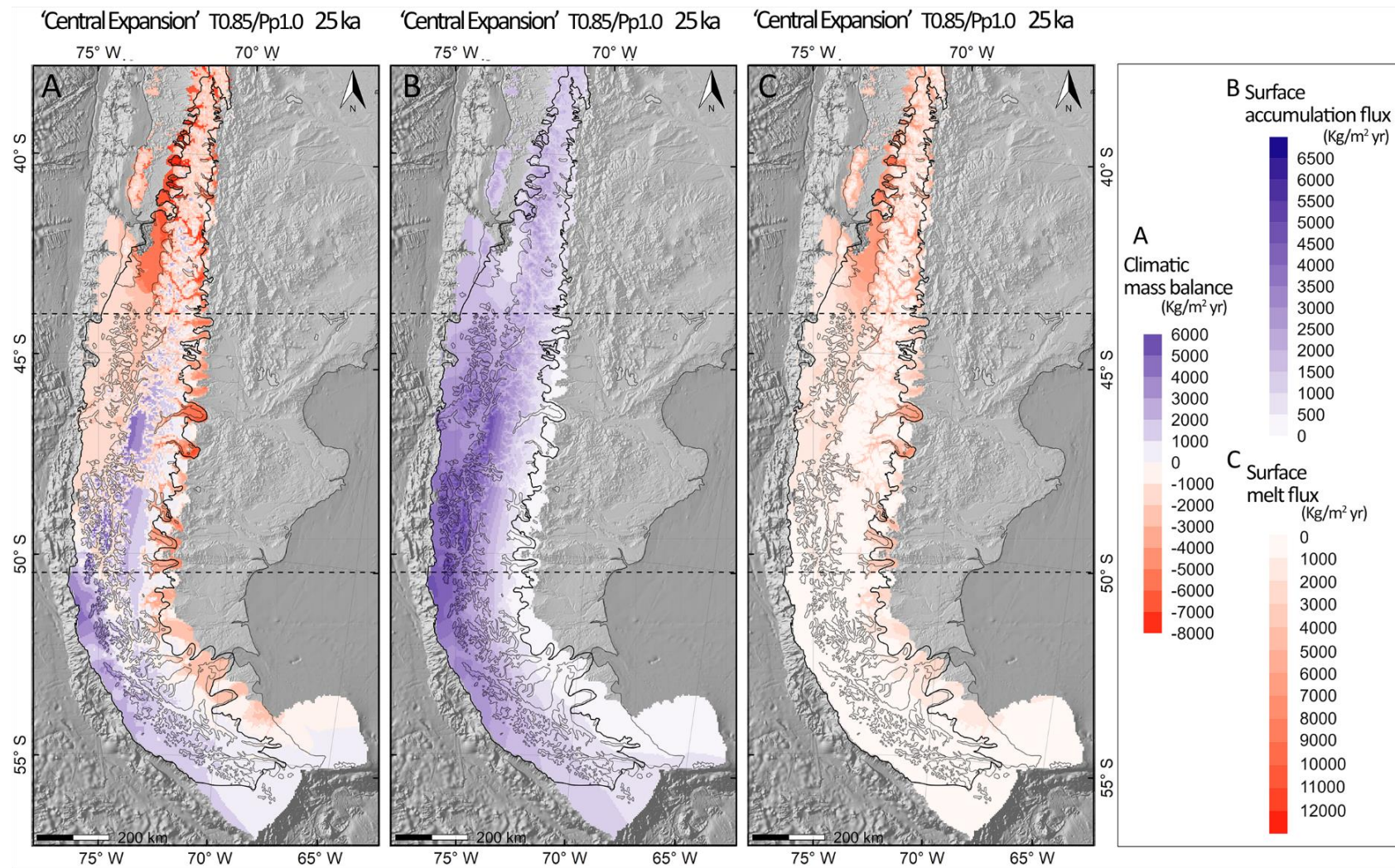
Figure 4.13. Maps of mass balance at 25 ka, produced by model #38. A) Overall mass balance. B) Surface accumulation flux. C) Surface melt flux. Black line corresponds to the geochronology constraint at 25 ka (Davies et al., 2020). Dashed lines divide the model domain in northern, central and south.
