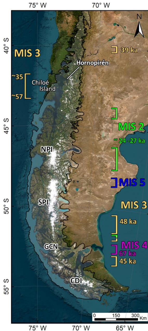
Figure 3.1. Timings for the ice maxima of the former Patagonian Ice Sheet during the last glacial period. The black line corresponds to the Patagonian Ice Sheet extent at the global Last Glacial Maximum (c. 24 ka; Davies et al., 2020). The brackets show the latitudinal extent of the ice maxima for a certain period. The brackets are opened towards the dated ice lobes, either on the western or eastern side of the Andes. A regional tendency can be appreciated, where Northern and Southern Patagonia reached their maximum extensions between 30-50 ka during MIS 3, except for an earlier occurrence at MIS 4 in Southernmost Patagonia. On the other hand, in Central Patagonia, the ice maxima occur in a close agreement between 27 – 24 ka (MIS 2), relatively contemporaneous to the global Last Glacial Maximum. NPI: Northern Patagonian Icefield, SPI: Southern Patagonian Icefield, GCN: Gran Campo Nevado Ice Cap, CDI: Cordillera de Darwin Icefield.
