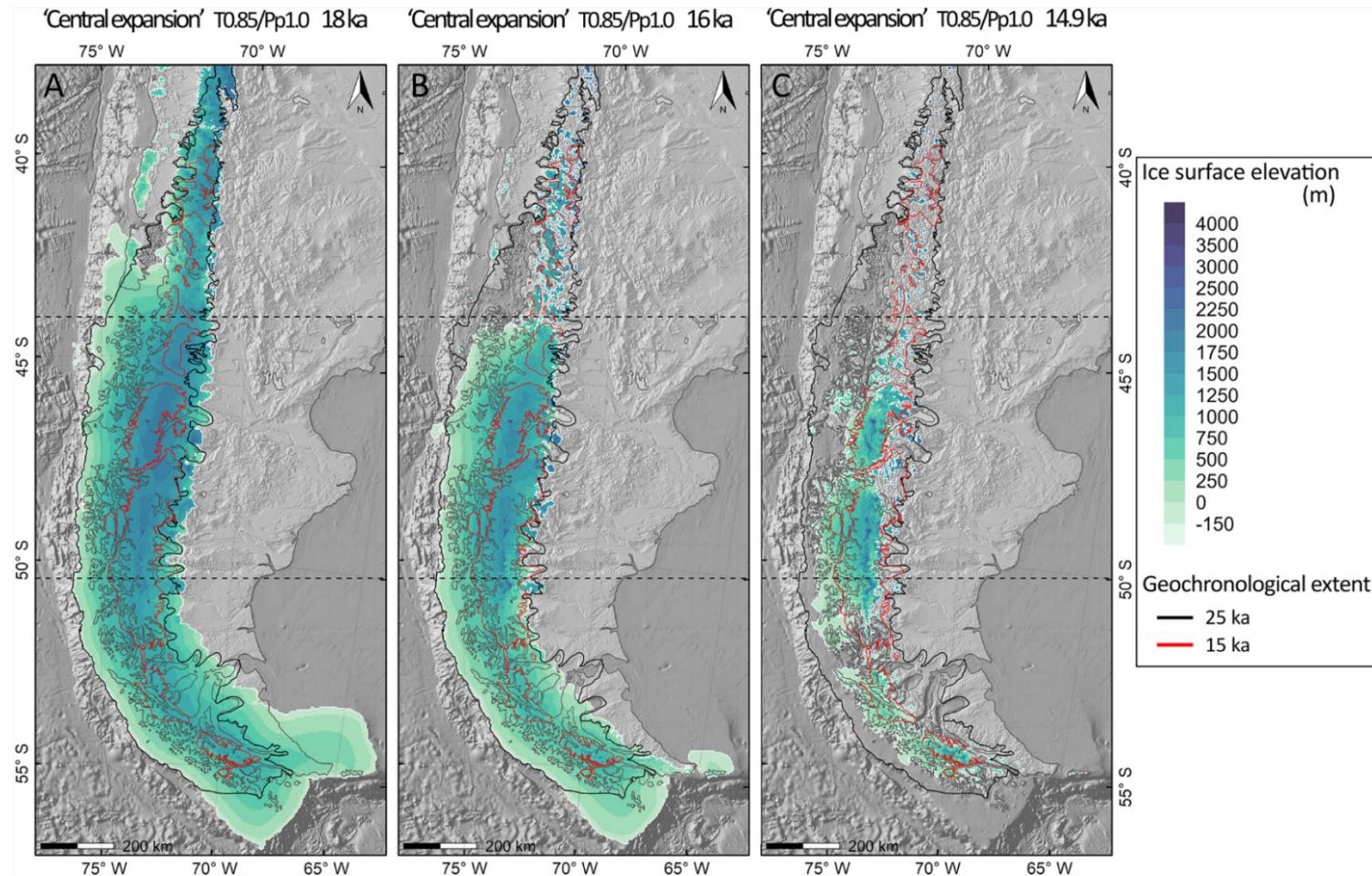
Figure 4.9. Ice extent of the model #38 during the late glacial and deglaciation. Model #38 is forced with Central expansion precipitation scenario and it is the model that best fits the geochronology at 25 ka. Snapshots of the model are taken at 18 ka (A), 16 ka (B) and 14.9 ka (C.) The Geochronology extent at 15 ka is from the PATICE project (Davies et al., 2020), and at 25 ka is modified from PATICE by including Seno Skyring (Lira et al., 2022) and Magallanes ice lobes (Peltier et al., 2021). This figure shows that after the 18 ka the deglaciation is more rapid in northern Patagonia than the rest, and the model does not fit the 15 ka PATICE margin in this area.
