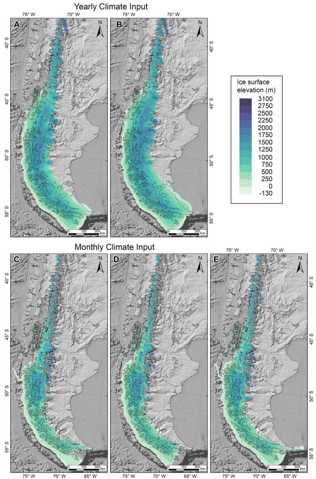
Figure 3.10. Sensitivity tests to evaluate the temporal resolution of the climatic input, yearly (top) vs monthly (bottom), and different methods of temperature standard deviation (SD). All these simulations are run until equilibrium, with the decrease in temperature to -6^{\circ} , with the modern precipitation configuration and a gradual decrease of the sea level to -134 m. Top, simulations use yearly-mean climatic inputs. A) the temperature SD has a constant value of 3. B) uses the linear temperature SD method. Bottom, monthly-mean climatic input. C) constant temperature SD of 3. D) linear temperature SD method. E) Seasonal and spatial variation of the temperature SD. This figure demonstrates how the selection of the different climatic approaches affects the extent of the resulting ice sheet. For instance, using monthly climate forcings (bottom) gives more restricted ice extent than using yearly (top). The different methods to simulate the air temperature SD yield similar ice extent for the region of Patagonia (compare C-E).
