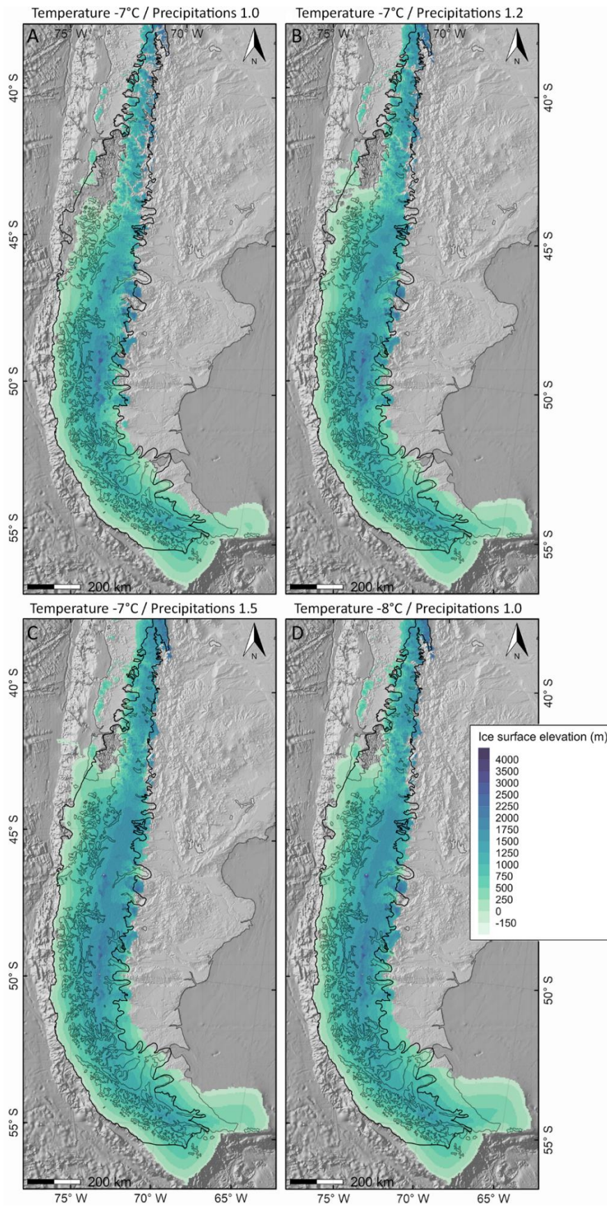
Figure 3.12. Models from the climatic forcing sensitivity test that their ice extent fit the best to the geochronology extent for the LGM. The modern temperature and precipitation configuration has been scaled by different factors and they are indicated on top of each panel. A-B) Better fit for the central south of Patagonia. C-D) Better fit for northern Patagonia. The glaciological and climatic parameters for each model are indicated in Table 3.2, and the results correspond to A) Model #13, B) Model #14, C) Model #15, D) Model #16. The coarse black line corresponds to the ice extent during the LGM (Davies et al., 2020).
