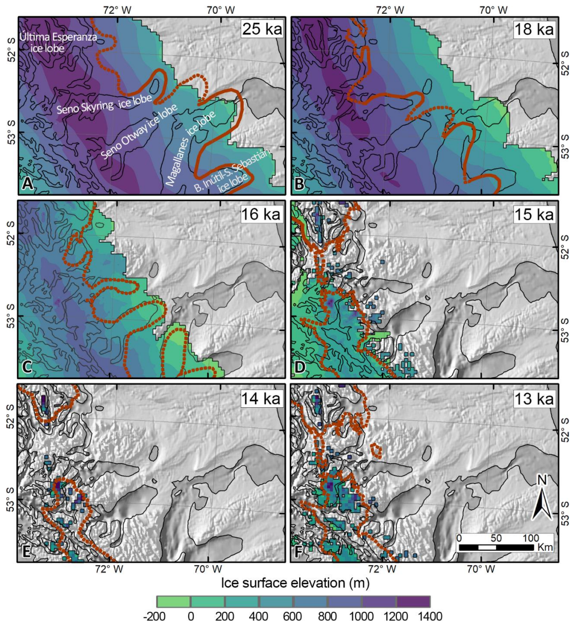
Figure 4.16. Comparison between the modelled ice extent and the geomorphology constrained by the geochronology of southeastern Patagonia, during the LGM and deglaciation. Model #38 is forced with ‘central expansion’ precipitation scenario and it is the model that best fits the geochronology at 25 ka. Continuous brown lines correspond to a direct geochronological constraint of glacial positions. Dashed lines correspond to inferred glacial position from minimum ages for glacial abandonment. A) 25 ka, B) 18 ka, C) 16 ka, D) 15 ka, E) 14 ka and F) 13 ka.
