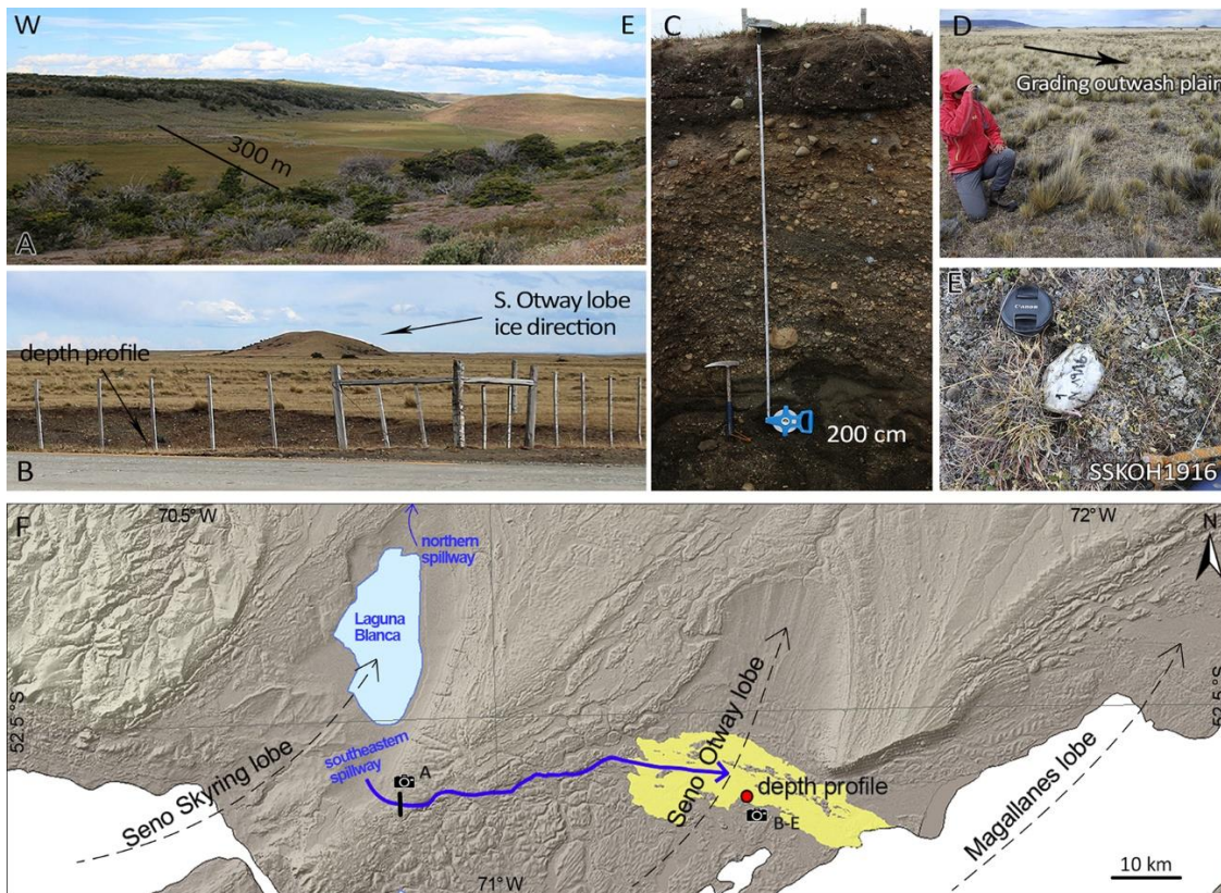
Figure 2.7. Geomorphological record of drainage of Laguna Blanca through the southeastern spillway. A) Southeastern drainage spillway viewed from the south. B) Moraines of the Otway lobe surrounded and partly-buried by a later outwash deposit on both distal and proximal sides. C) Depth profile of the outwash that buries the Otway moraines. D–E) Cobbles sampled for cosmogenic analysis on the surface of the outwash. F) Map showing the mapped drainage route from the southeastern spillway of the Seno Skyring basin towards the Otway lobe basin.
