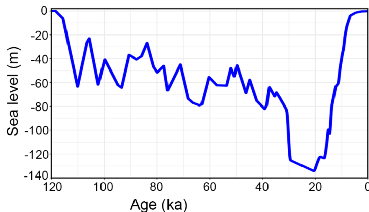
Figure 3.3. Key boundary conditions for the modelling. Sea level changes during the last glacial cycle, from 120 ka to the present (Yokoyama et al., 2018).
