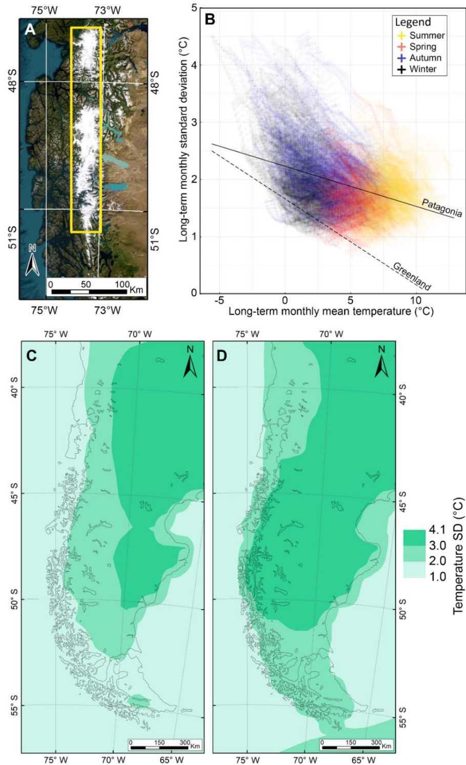
Figure 3.9. Air-temperature standard deviation (SD) methods to simulate diurnal air temperature variabilities. In the top panels a linear temperature SD approach in relation to the surface air temperature is illustrated. A) Long-term monthly mean temperature vs long-term monthly SD data has been obtained from the yellow polygon (ERA-40 reanalysis data) to calculate a linear relationship for the air temperature SD. B) Plot of the data collected from the area of polygon in A, which shows the long-term monthly mean air temperature vs long-term monthly SD data, sorted seasonally. The continuous black line corresponds to the slope that best fits the relationship between the air temperature SD and the air temperature in Patagonia. This linear relationship indicates that the higher the temperature, the smaller the air temperature SD, and vice versa, and this is directly related to the seasons of the year. The dashed line corresponds to the slope that best fits the data in Greenland (Seguinot & Rogozhina, 2014). The bottom panels show the spatial and seasonal air temperature SD approach, which uses a spatial variation for each month. C) January (C) and (D) July temperature SD obtained from Seguinot (2013).
