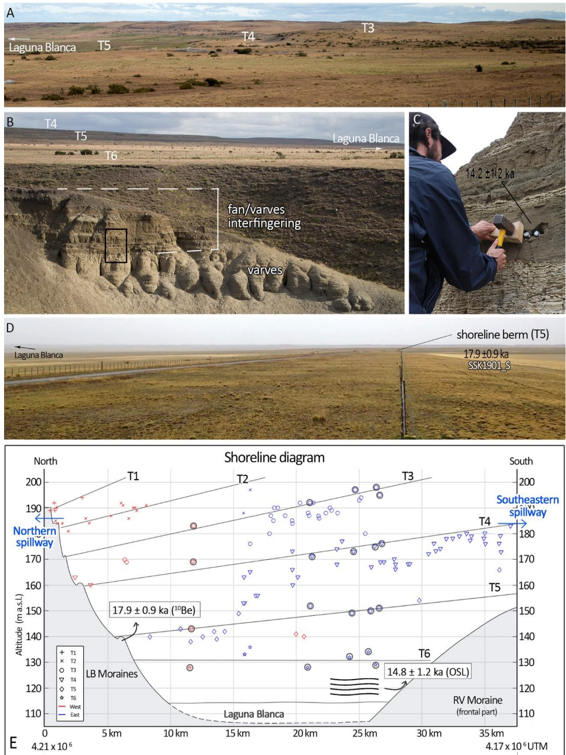
Figure 2.6. Palaeo shorelines of Laguna Blanca. A) Three terrace levels seen at the eastern side of Laguna Blanca. B) Incision of the lowest terrace, T6, exposes glaciolacustrine and alluvial fan sediments. C) OSL sample from a sand layer of the lacustrine profile (see panel b for location). D) Palaeo shoreline berm located at the north part of Laguna Blanca, this berm is related to T5. E) Shoreline Diagram of the former levels of Laguna Blanca. The symbols surrounded by a black circle correspond to the measurements done on the scarp base. The locations are marked of a 10 Be age of the shoreline berm on T5, and an OSL sample of a subaqueous alluvial fan taken from a raised shoreline forming part of terrace T6. Data from west (red) and east (blue) are differentiated. The elevations and positions of the northern and southeastern drainage spillways are marked. See legend for shoreline/terrace numbering.
