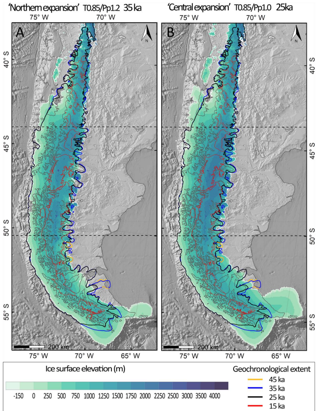
Figure 4.6. Models that have the best fitting ice extent at 35 and 25 ka; the model domain is divided in northern, central and southern Patagonia (boundaries shown by dashed lines). A) Model #21, which is forced with a Northern expansion precipitation with temperature and precipitation scaled by 0.85 and 1.2, respectively. B) Model #38, which is forced with a Central expansion scenario with temperature and precipitation scaled by 0.85 and 1.0, respectively. The Geochronology extent at 35 and 15 ka is from the PATICE project (Davies et al., 2020), and at 25 ka is modified from PATICE by including Seno Skyring (Lira et al., 2022) and Magallanes ice lobes (Peltier et al., 2021). The ice extent at 45 ka is from Darvill et al. (2015) and García et al. (2018).
