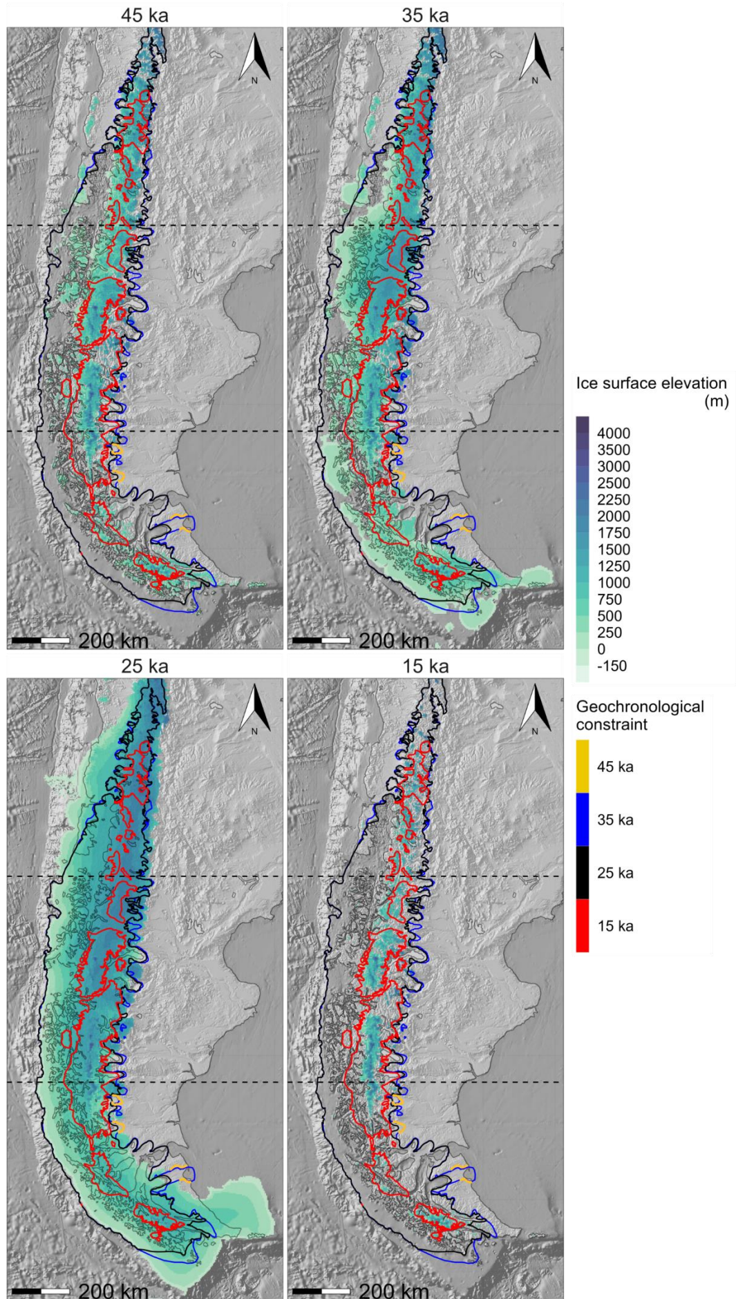
Model #11: 'Northern migration' T0.85/Pp1.0
