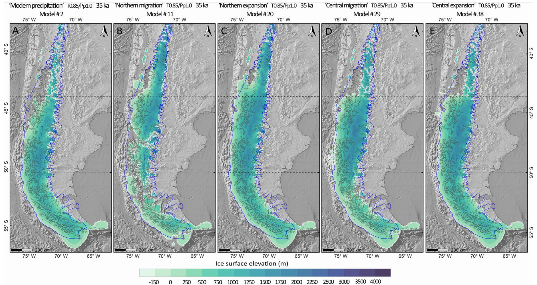
Figure 4.4. Ice surface elevation at 35 ka, resulting from models forced by the five different precipitation scenarios proposed in this work and the temperatures forced by the EPICA curve. In all of them, the precipitation is scaled by a factor of 1.0 and the temperatures by a factor of 0.85. A) Modern precipitation scenario. B) Northern migration scenario. C) Northern expansion scenario. D) Central migration scenario. E) Central expansion scenario. The blue line corresponds to the ice extent constrained at the 35 ka timeslice (Davies et al., 2020).
