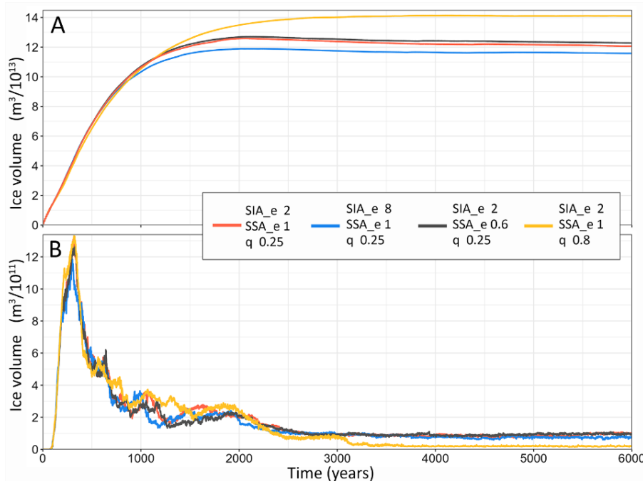
Figure 3.6. Ice volume sensitivity tests to evaluate the influence of the SIA/SSA enhancement factors and the plasticity component ( q ). All these simulations are run until equilibrium, with decrease in air temperature to -6^\circ , with modern precipitation configuration and a gradual decrease of the sea level to -134 m. A) Corresponds to the ice volume for grounded ice. B) Corresponds to the ice volume for the floating ice. The red curve shows the results from the parameters used in this work, which are elected according to the literature that best fits the Patagonian glacial environment.
