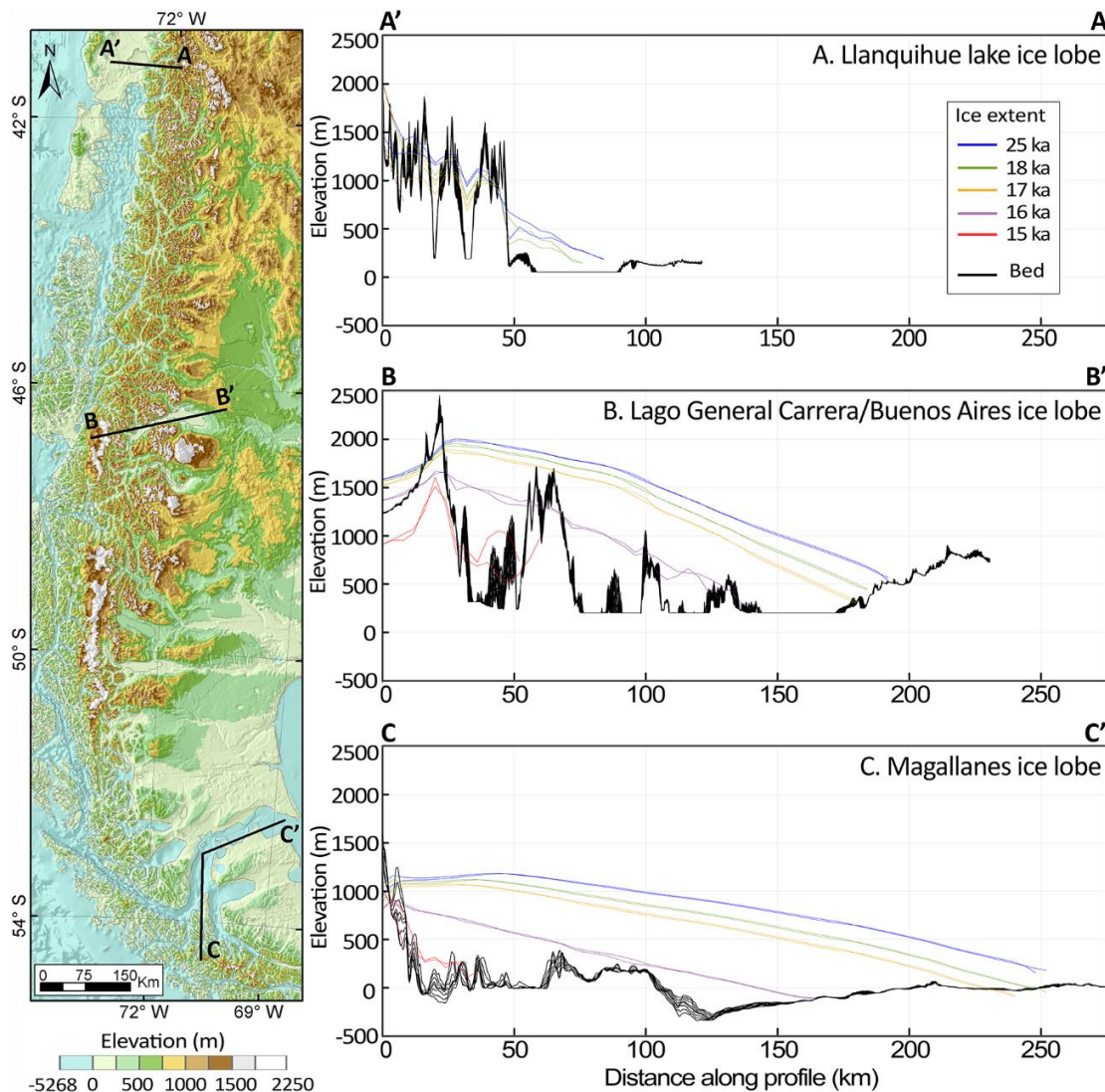
Figure 4.15. Ice lobes' long profile from different regions in Patagonia, showing the characteristic topography of each region, and the ice extent at different time intervals from the LGM to deglaciation. Left, shows the elevation changes along Patagonia and the location of the profiles. Right, shows the A) Llanquihue ice lobe located in northern Patagonia. B) Lago General Carrera/Buenos Aires ice lobe, located in central Patagonia. C) Magallanes ice lobe, located in southern Patagonia. The swath width is 2 km for the topography of all the profiles and 4 km for the ice surface. The topography for A and B is from SRTM (30m resolution); note that in the Llanquihue and General Carrera/Buenos Aires lakes, the bathymetry is absent. For C the bed topography is from GEBCO (450 m resolution), as it considers the bathymetry of the fjords. The ice profiles are obtained from model #38 (Central expansion T0.85/Pp1.0; 4 km resolution).
