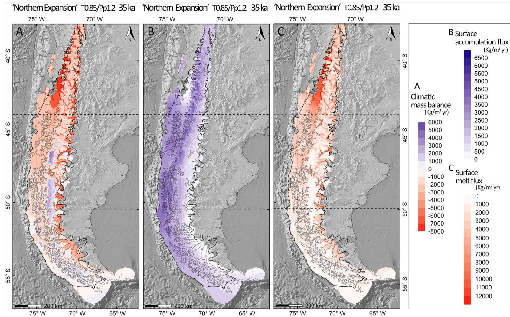
Figure 4.12. Maps of mass balance at 35 ka, produced by model #21. A) Overall mass balance. B) Surface accumulation flux. C) Surface melt flux. Black line corresponds to the geochronology constraint at 25 ka (Davies et al., 2020). Dashed lines divide the model domain in northern, central and south.
