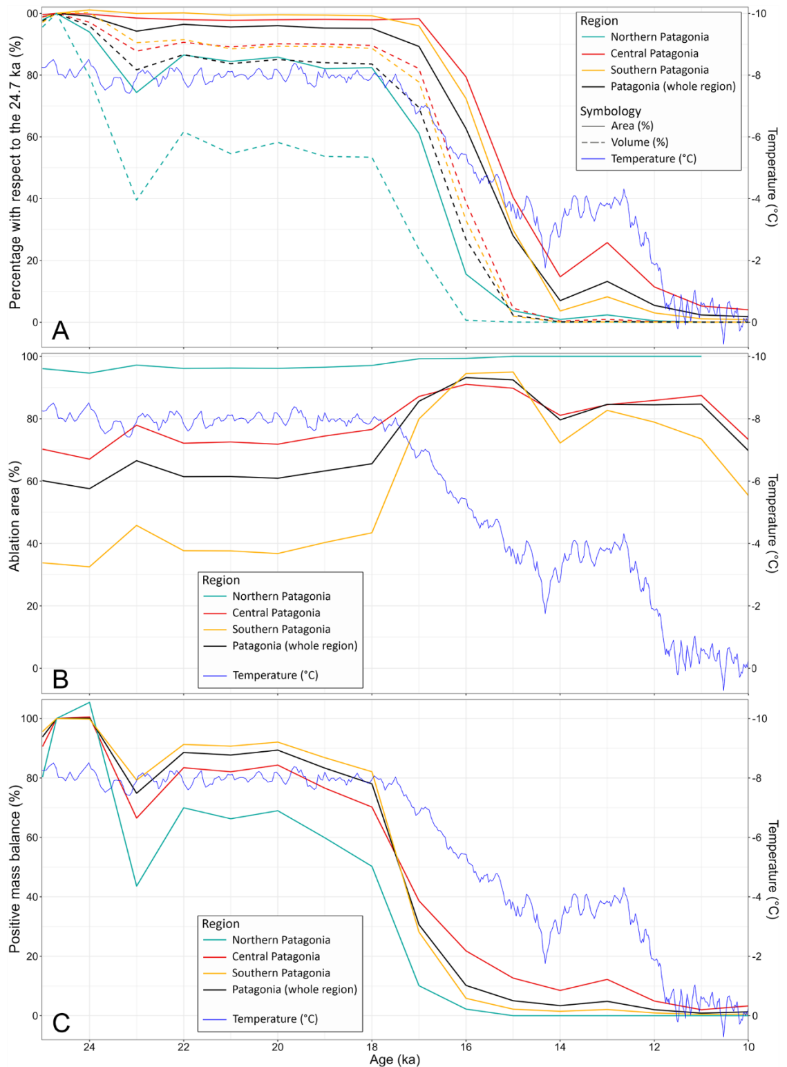
Figure 4.8. Ice sheet deglaciation pattern from 25 to 10 ka. A) Percentage of the ice extent and ice volume, with respect to the maximum ice extent and volume at 24.7 ka (100%). B) Percentage of the ablation area, marked by the area with negative mass balance at each time in percentage. C) Positive mass balance reduction in percentage, from the peak of the glaciation at 24.7 ka. Data are from model #38, which is the simulation that best reproduces the ice extent at 25 ka. The graphs show data for individual regions (northern, central and southern Patagonia) and for the whole of Patagonia. The temperature data (blue line) is obtained from EPICA, and is the record used to force these models. Note that the temperature scale is reversed (coldest at top).
