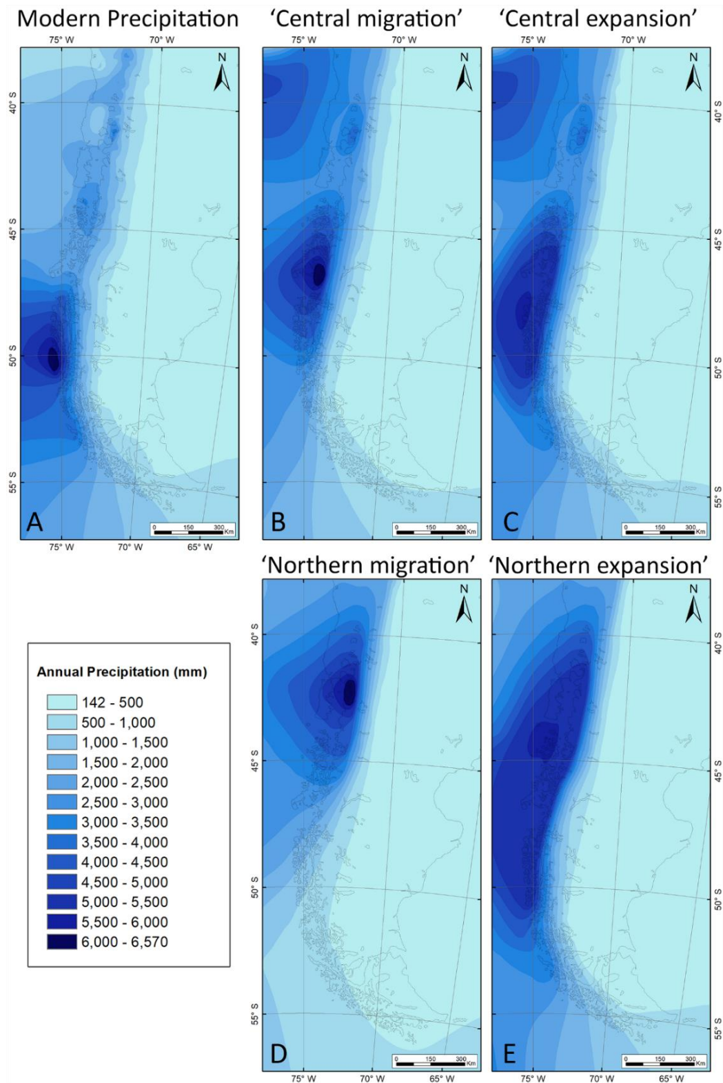
Figure 4.3. Precipitation scenarios used to force the different models. A) Modern precipitation scenario, corresponds to the present day precipitation distribution, where the precipitation is concentrated in a core between 50-51°S. B) 'Central migration' scenario, we transport the core to central Patagonia at ~47°S, creating a wetter Central Patagonia and a drier Southern Patagonia. C) 'Central expansion' scenario, we expand the SWWs core to central Patagonia, but the intensity of the core weakens. The amount of precipitation in the South slightly less than today. D) 'Northern migration' scenario, we transport the core to northern Patagonia at ~42°S, creating a wetter Northern Patagonia, and a drier Southern Patagonia. E) 'Northern expansion' scenario, we expand the SWWs core to northern Patagonia, but the intensity of the core weakens. This scenario keeps slightly less precipitation in Southern Patagonia than today.
