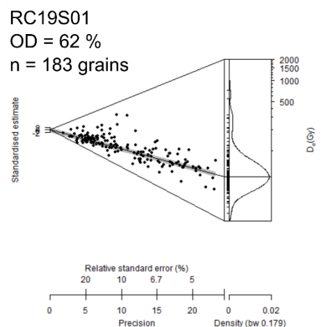
Figure SC2.1. Abanico plots of the De values determined for OSL dating, where the grey shading shows the MAM De for each distribution.
