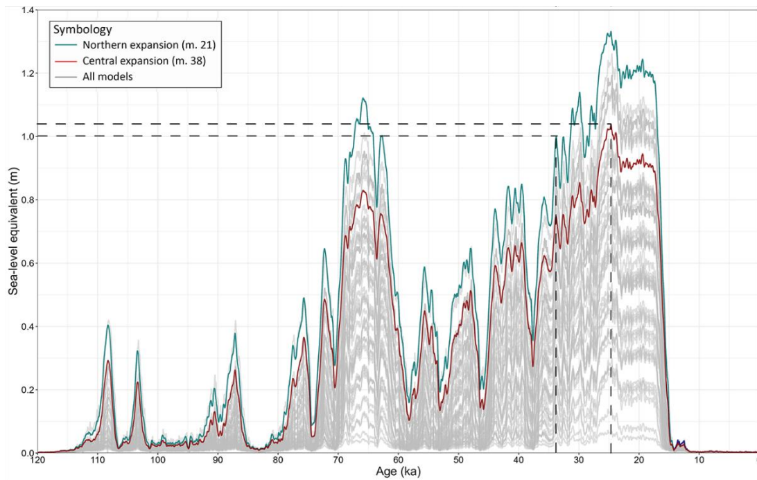
Figure 4.7. Sea-level equivalent of the modelled PIS in the forty-five simulations produced in this work (grey) through the last glacial cycle. The two models that fit the best at 34 ka (model #21) and 24.7 ka (model #38) are highlighted in green and red, respectively. Dash lines guide the x and y axis intersection.
