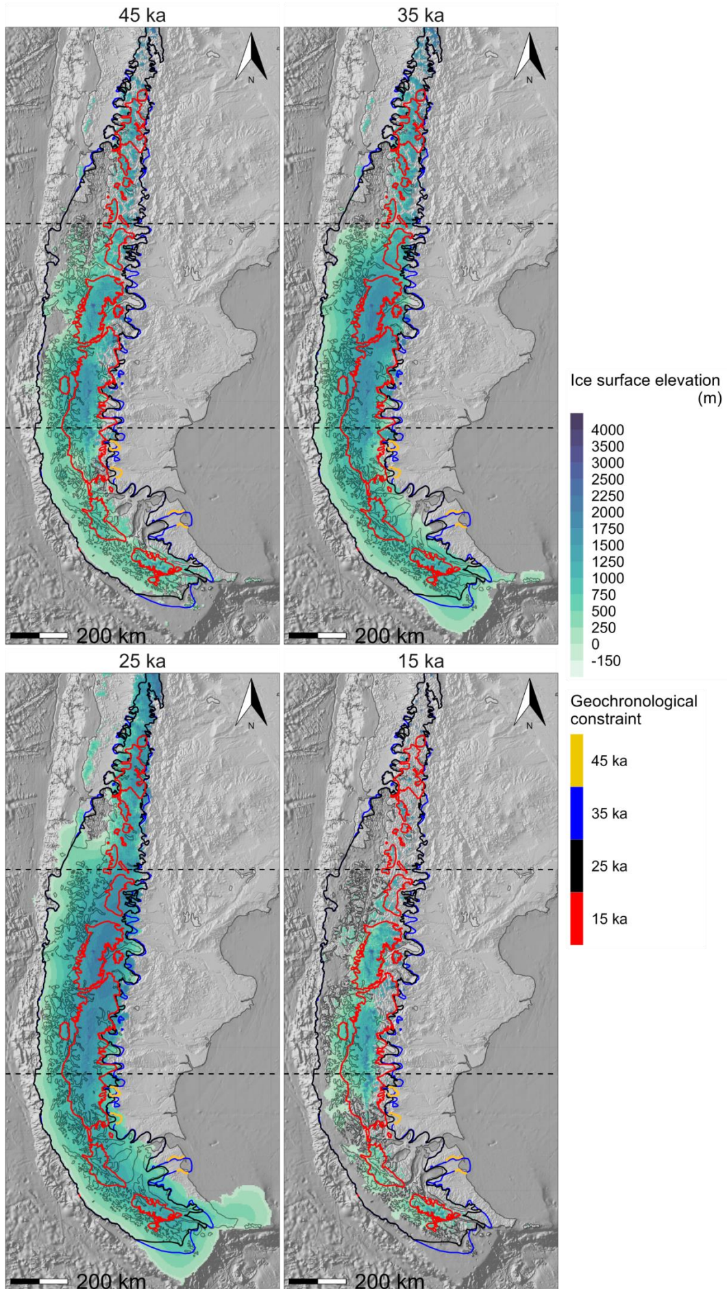
Model #42: 'Central expansion' T0.75/Pp1.2
