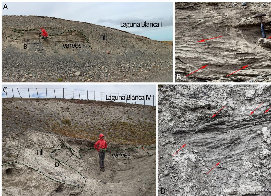
Figure 2.5. Cut profile from LB moraines, showing lacustrine sediments overlain by till. A,B). LB I. C,D). LB IV. The sediments have climbing ripple crosslamination structure. The sediments show evidence of brittle deformation indicated by red arrows.
