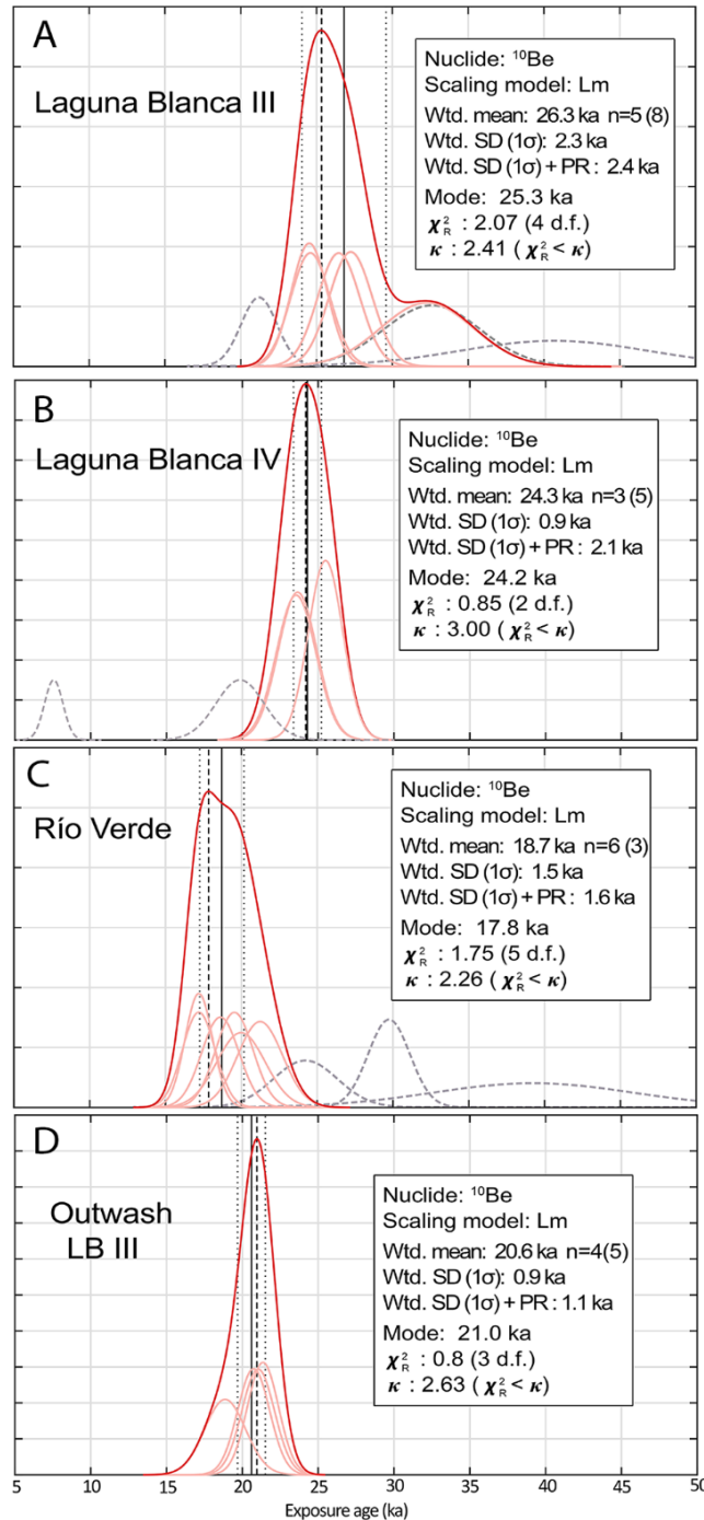
Figure 2.8. Probability density functions (“camel plots”) of the ages for moraines and outwash of the former Skyring ice lobe. All ages are calculated with the Patagonian production rate from Lago Argentino (Kaplan et al., 2011) and considering zero erosion. A) Laguna Blanca III. B) Laguna Blanca IV. C) Río Verde moraine. D) Outwash Laguna Blanca III. n corresponds to the number of samples used to calculate the weighted ages. Bracket numbers are all the samples processed, including outliers. The diagrams were plotted using IceTea (Jones et al., 2019), where the mode (black dashed line), weighted mean (solid black line) and weighted standard deviation (SD; black dotted lines) of the dataset are shown. The application also calculates the reduced chi-squared ( \chi^2_R ) and the associated criterion ( \kappa ). The outliers are shown as grey dashed lines; they were calculated following reduced chi-squared statistics.
