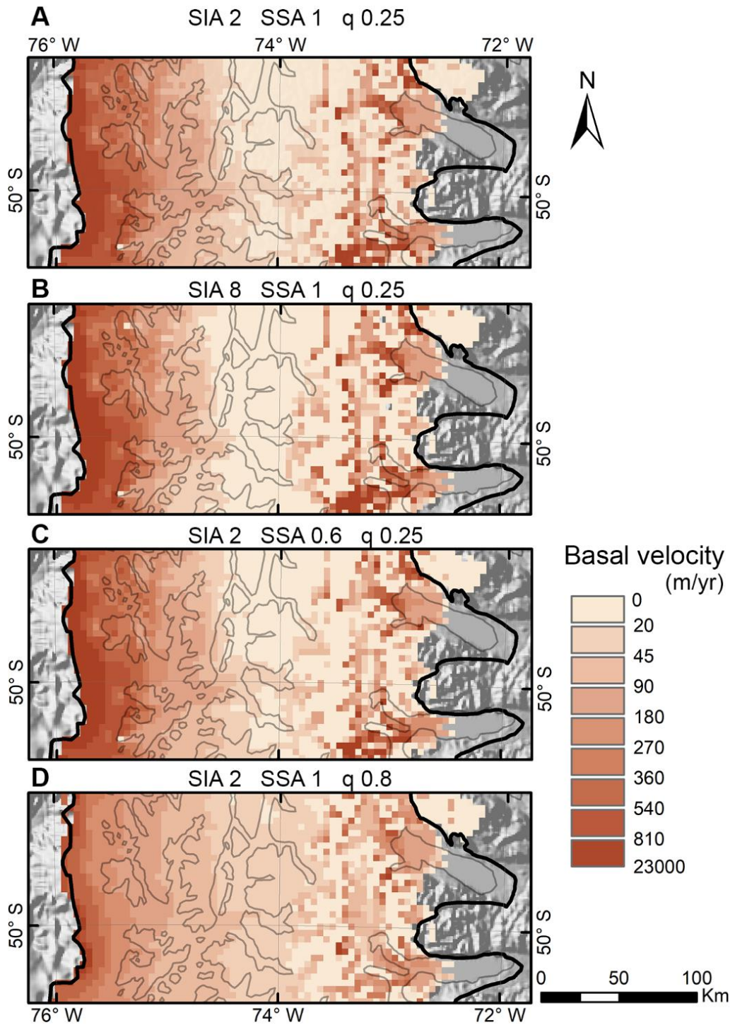
Figure 3.7. Basal sliding sensitivity tests to evaluate the influence of the SIA/SSA enhancement factors and the plasticity component (q). A) Corresponds to model #1. B) Corresponds to model #2. C) Corresponds to model #3. D) Corresponds to model #4. All these simulations are run until equilibrium, with decrease in air-temperature to -6^{\circ} , with modern precipitation configuration and a gradual decrease of the sea level to -134 m. The black line corresponds to the ice extent during the LGM (Davies et al., 2020).
