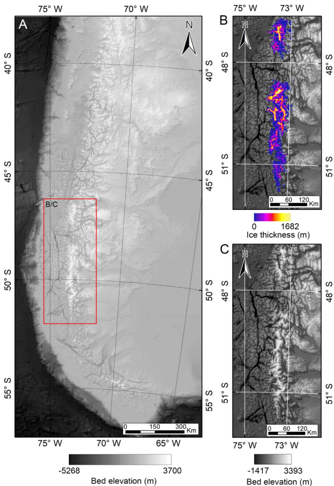
Figure 3.2. Basal boundary conditions for the modelling. Bed topography input model. A) Topography and bathymetry from GEBCO. B) Ice thickness of the Northern and Southern Patagonian Ice Fields (Millan et al., 2019). C) Bed elevation with the ice thickness subtracted (compare the topography with A).
