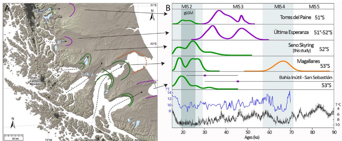
Figure 2.12. Southern Patagonia ice lobe extents and timing of occurrence of the moraine belts during the last glacial period from 15–90 ka. A) Map of major moraine belts which are coloured to match the geochronology in panel (B). Orange corresponds to MIS 4, purple to MIS 3 and green to MIS 2. B) Density functions (probability plots) of exposure ages of moraine boulders in Southern Patagonia moraine belts (this study; McCulloch et al., 2005b; Kaplan et al., 2008; Sagredo et al., 2011; García et al., 2018; Peltier et al., 2021). For the Bahía Inútil-San Sebastián ice lobe, the outer glacial margins were geochronological constrained through a cosmogenic nuclide depth profile approach performed on the outwash plain associated with their respective moraine (Darvill et al., 2015). These ages are indicated by a solid circle (purple) and their uncertainty by a horizontal line. The Sea Surface Temperature (SST) curve (blue) is from an off-shore core in northwestern Patagonia at 41°S (Kaiser et al., 2005) and the east Antarctic temperature record (black) from EPICA Dome C (Jouzel et al., 2007).
