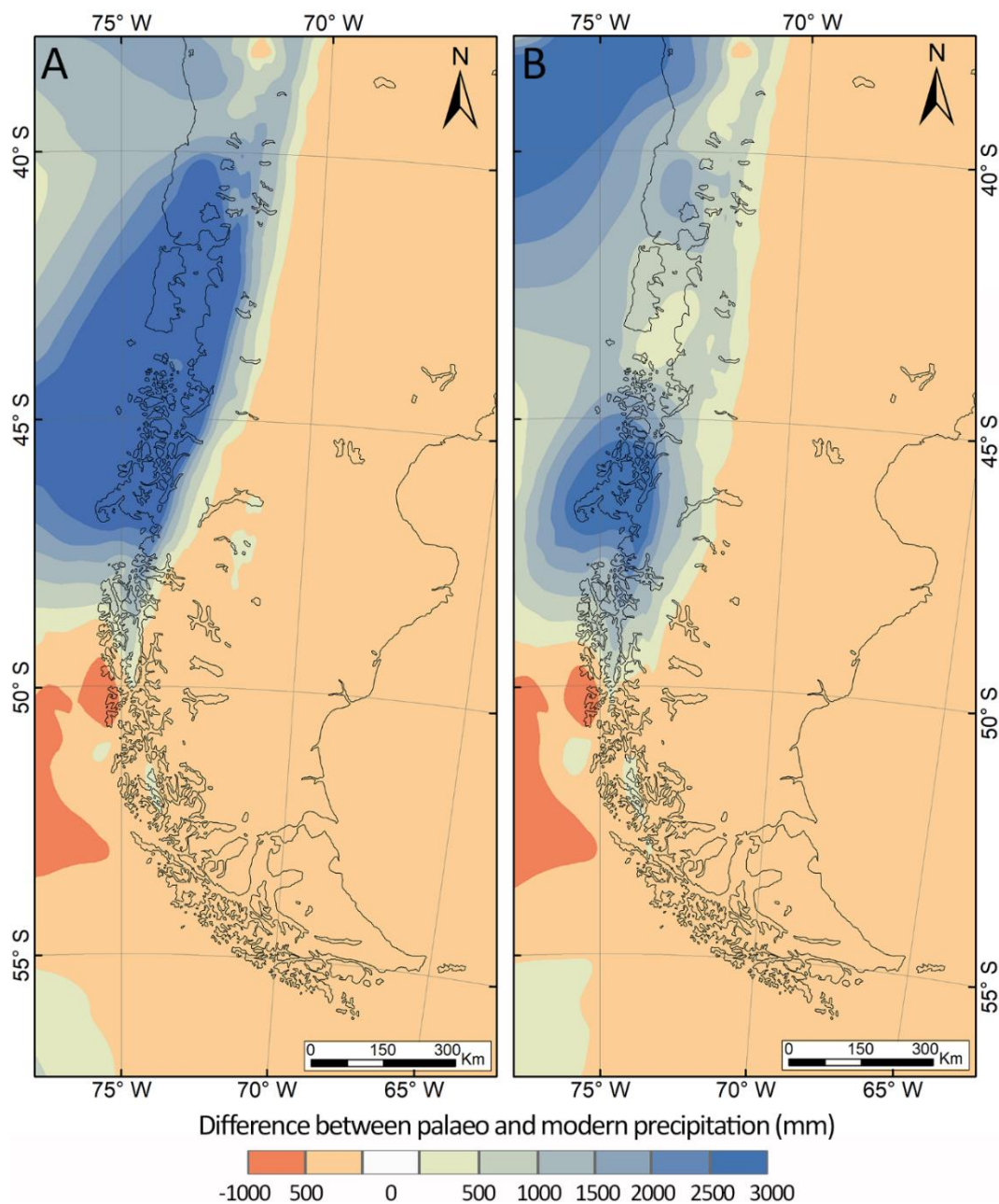
Figure 4.14. Precipitation differences (mm) between palaeo precipitations scenarios with modern annual precipitation. A) Northern expansion scenario. B) Central expansion scenario.
