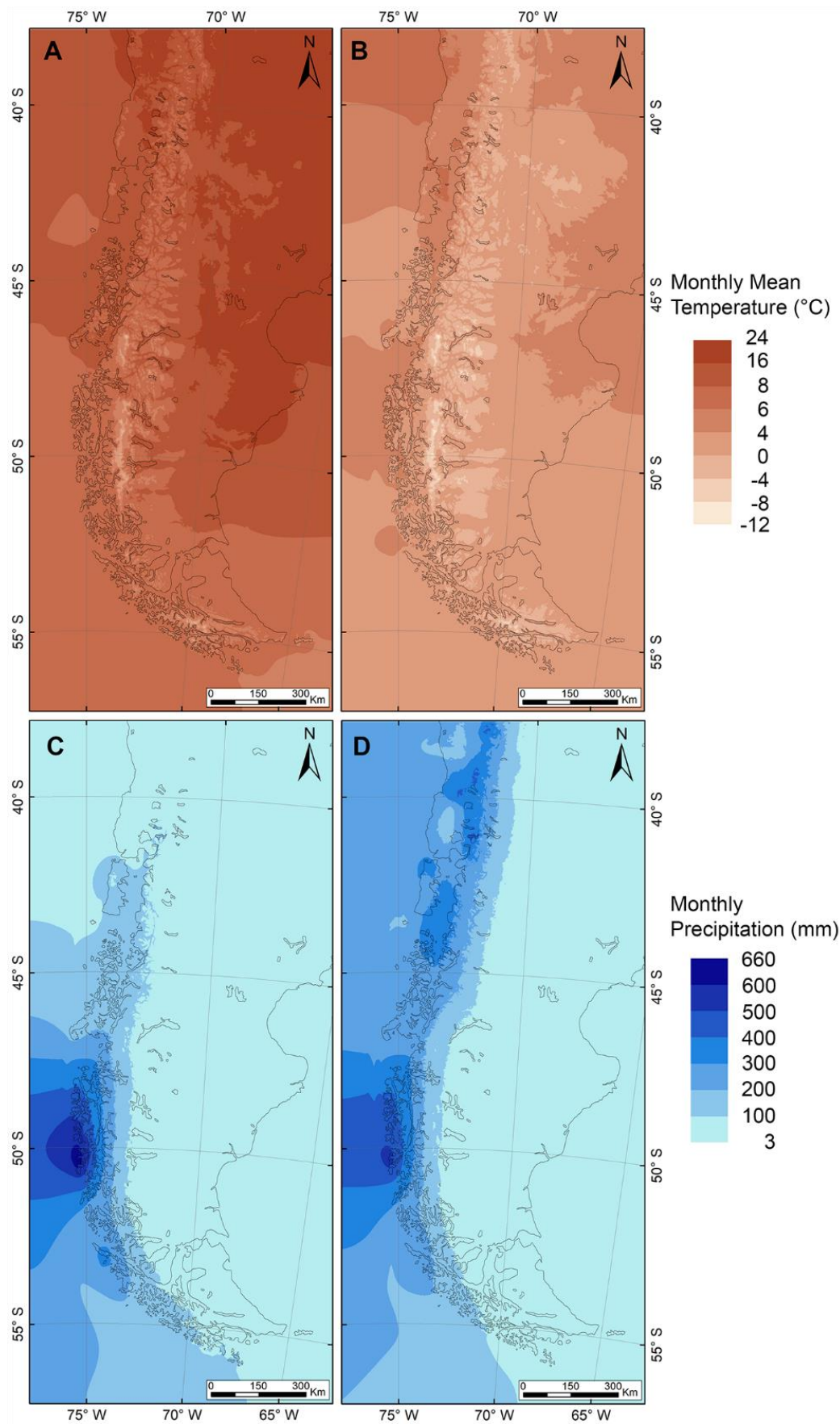
Figure 3.5. Monthly mean climatic inputs. Only January and July are plotted. Top, January (A) and July (B) mean temperature. Bottom, January (C) and July (D) Precipitations. Data obtained from WorldClimate2 (Fick and Hijmans, 2017), the offshore area is interpolated from the data on the continent.
