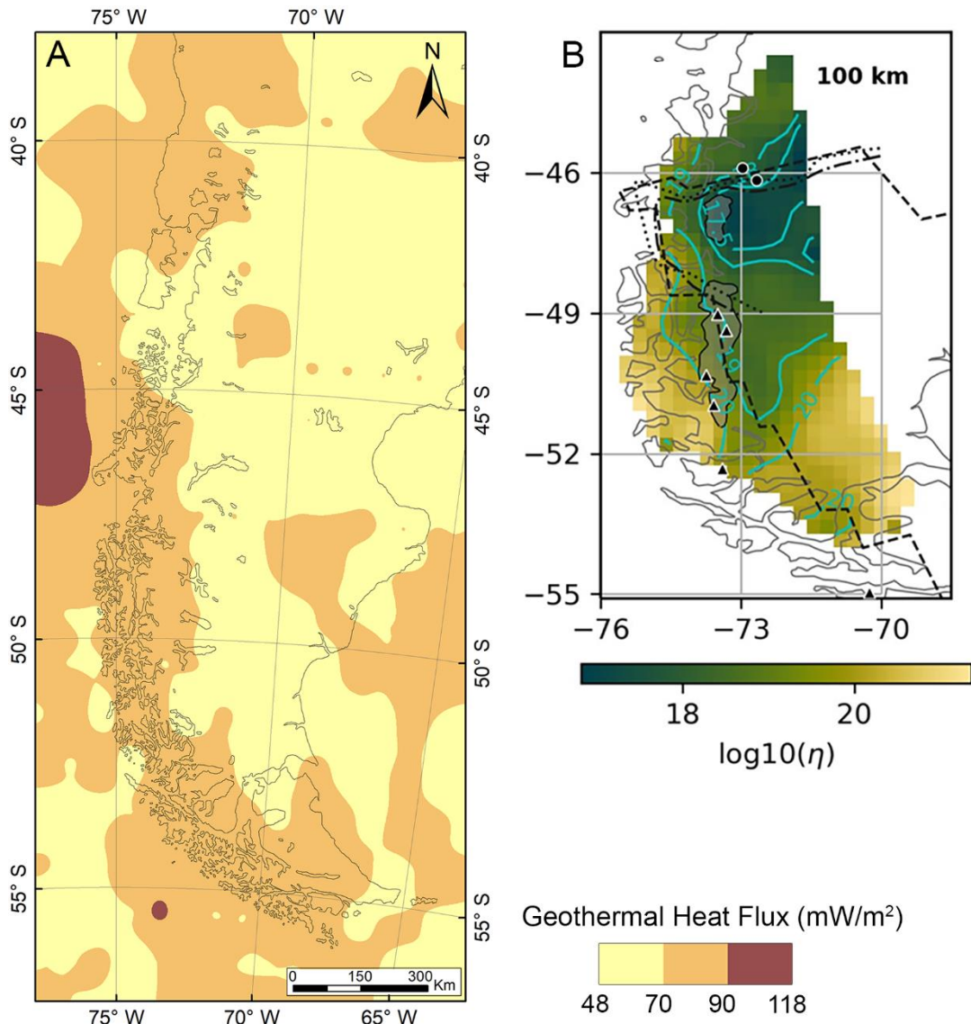
Figure 3.4. Key boundary conditions for the modelling. A) Geothermal heat flux (Goutorbe et al., 2011). B) Mantle viscosity of southwest Patagonia at 100 km depth, units are Pa s (Mark et al., 2022).
