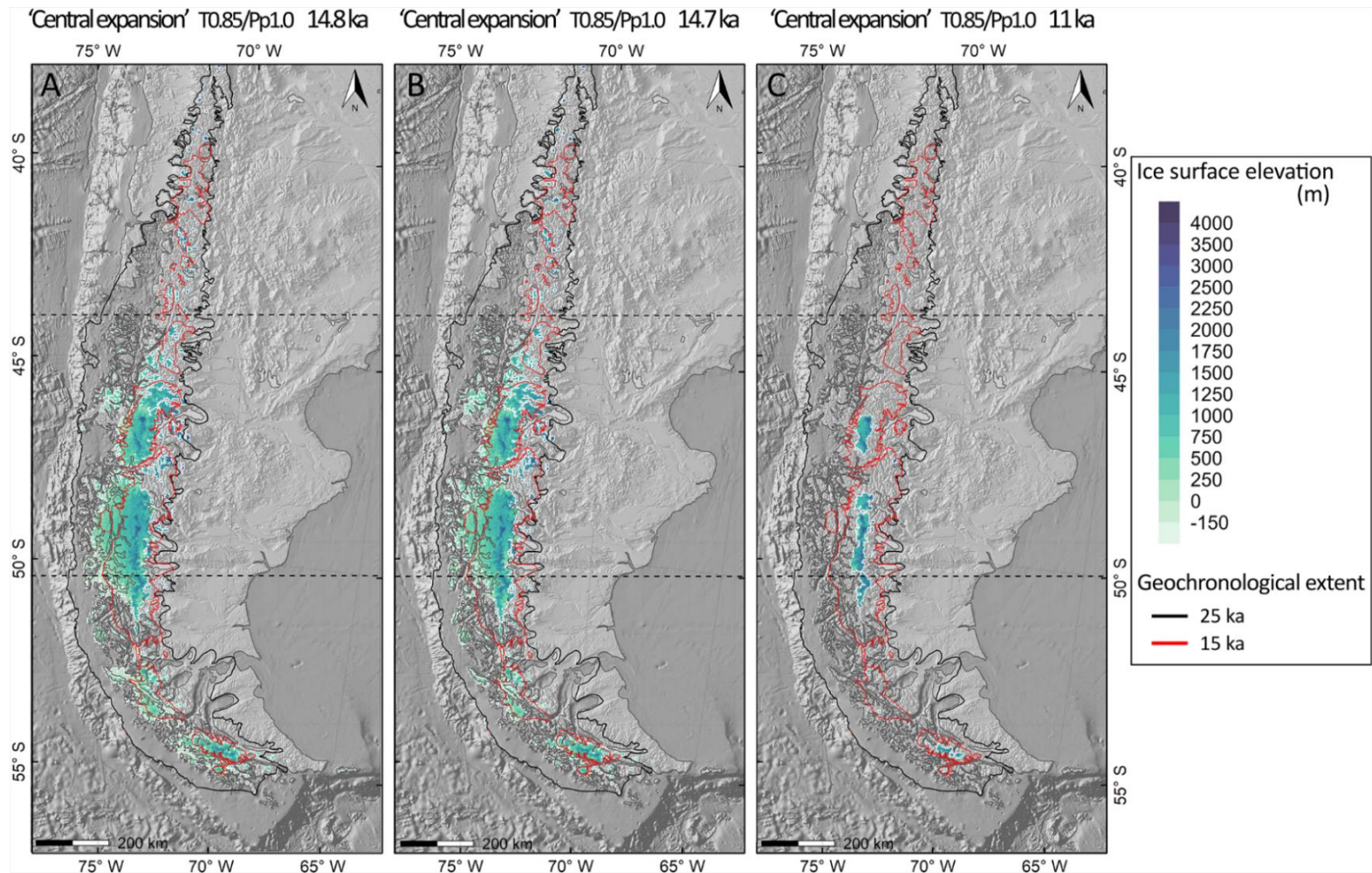
Figure 4.10. Ice extent of the model #38 during the late glacial and deglaciation. Model #38 is forced with Central expansion precipitation scenario and it is the model that best fits the geochronology at 25 ka. Snapshots of the model are taken at 14.8 ka (A), 14.7 ka (B) and 11 ka (C.) The Geochronology extent at 15 ka is from the PATICE project (Davies et al., 2020), and at 25 ka is modified from PATICE by including Seno Skyring (Lira et al., 2022) and Magallanes ice lobes (Peltier et al., 2021). This figure shows that central Patagonia is less sensitive to deglacial conditions than the northern and southern regions.
