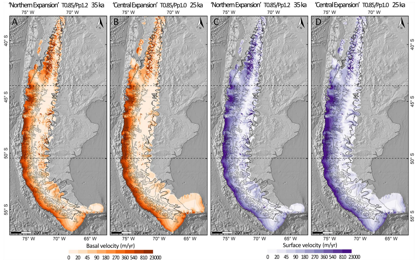
Figure 4.11. Ice velocities of the Patagonian Ice Sheet for the model that best fits the ice extent according to the geochronology records. A) Basal ice velocity of model #21 at 35 ka. B) Basal ice velocity of model #38 at 25 ka. C) Surface ice velocity of model #21 at 35 ka. D) Surface ice velocity of model #38 at 25 ka. The black line corresponds to the geochronology constraint at 25 ka (Davies et al., 2020). Dashed lines divide the model domain in northern, central and south.
