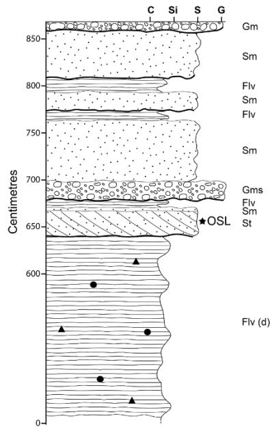
Figure SC2.2. Stratigraphic log from an exposure into T6. Codes for horizontal scale are C, Si, S and G for clay, silt, sand and gravel respectively. Lithofacies codes, Gm (clast-supported gravel), Sm (massive sand), Flv (fine lamination with varves), Gms (matrix-supported gravel), St (medium to very coarse sand with trough cross-bedding), d (dropstones), thicker contact is erosive, from Evans and Benn (2021). Star indicates the location of the OSL sample shown in Figs 6 and 7 (main text).
