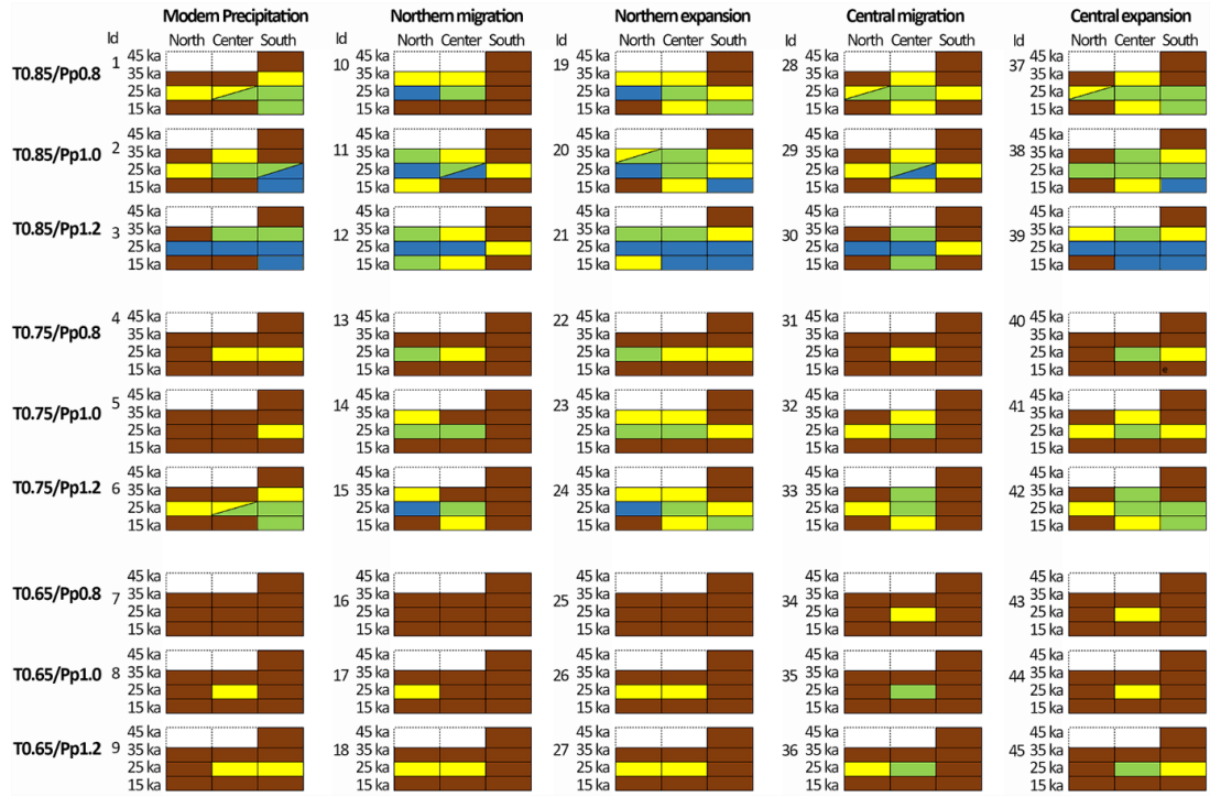
Figure 4.5. Assessment of fit of the 45 models with the geomorphology records constraint by the geochronology, at 45 ka, 35 ka, 25 ka and 15 ka. Each column corresponds to a precipitation scenario, and the rows represent the scaling factor for the temperatures and precipitation. Colour categories: brown: poor; yellow: fair; green: good; and blue: excess. See text for definitions of quality of fit. This figure shows that better fits occur with colder temperatures (e.g. when scaling the temperature by a factor of 0.85). Moreover, the better fit along northern, central, and southern Patagonia at a specific time is reproduced better with expansion precipitation scenarios (northern and central), than the other scenarios.
