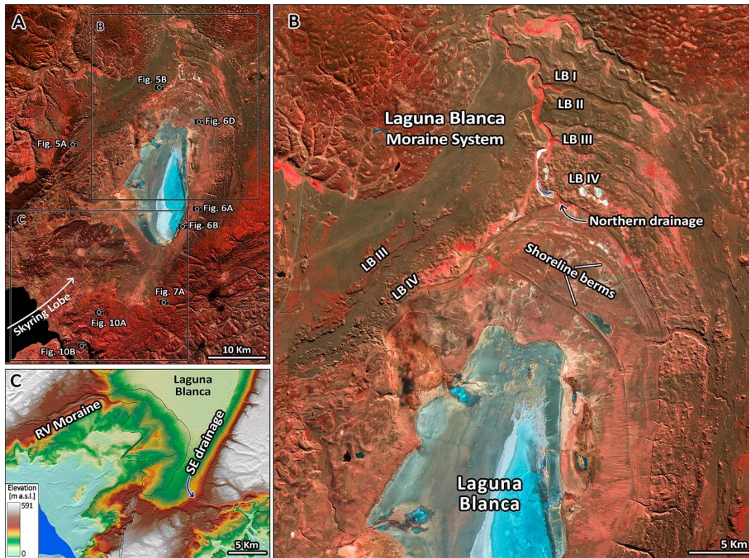
Figure 2.2. A) Sentinel 2 (band combination 843) image of the Seno Skyring ice lobe area. Former ice flow of the Skyring lobe was directed from Seno Skyring north-east to the Río Verde (RV) and Laguna Blanca (LB) moraine systems. B) Detailed image with focus on LB moraine system, showing its four different moraine belts, from older to younger LB I, LB II, LB III and LB IV respectively. Former shoreline berms and a northern drainage spillway of the palaeo Laguna Blanca are indicated. C) Hillshade and elevation colour ramp (SRTM) of the area around RV moraine system, black lines indicate the RV moraine extension. The south-eastern drainage spillway of the palaeo Laguna Blanca is marked. Note that the altitude of this drainage spillway is higher than the central (front) parts of the RV moraine, implying an ice dam must have been present.
