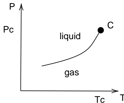
Figure 1.1: A generic liquid-gas phase diagram.
