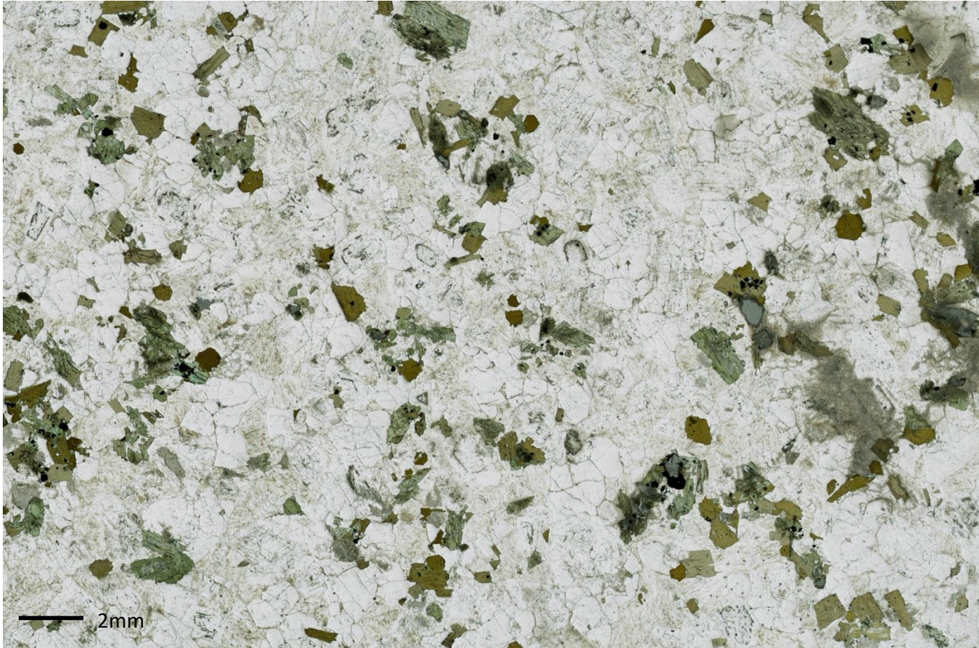
BP28 - Granite
