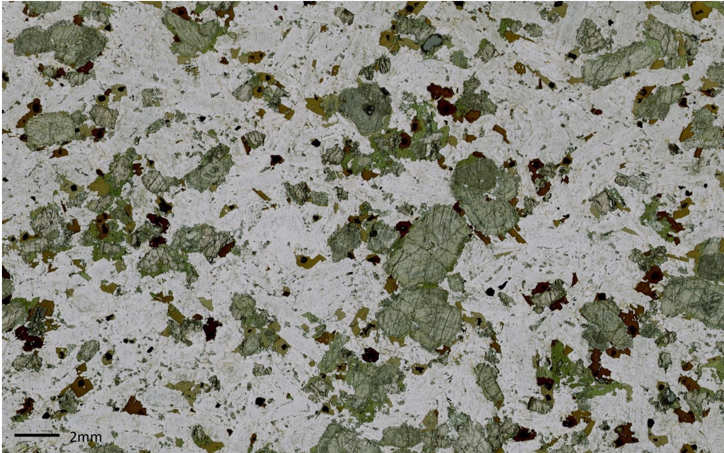
BP1 - Diorite
