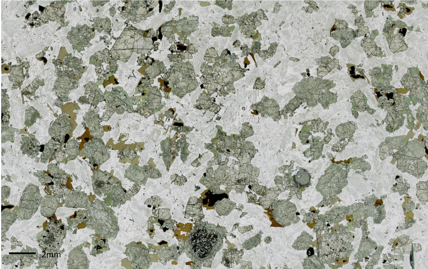
BP39 - Diorite
