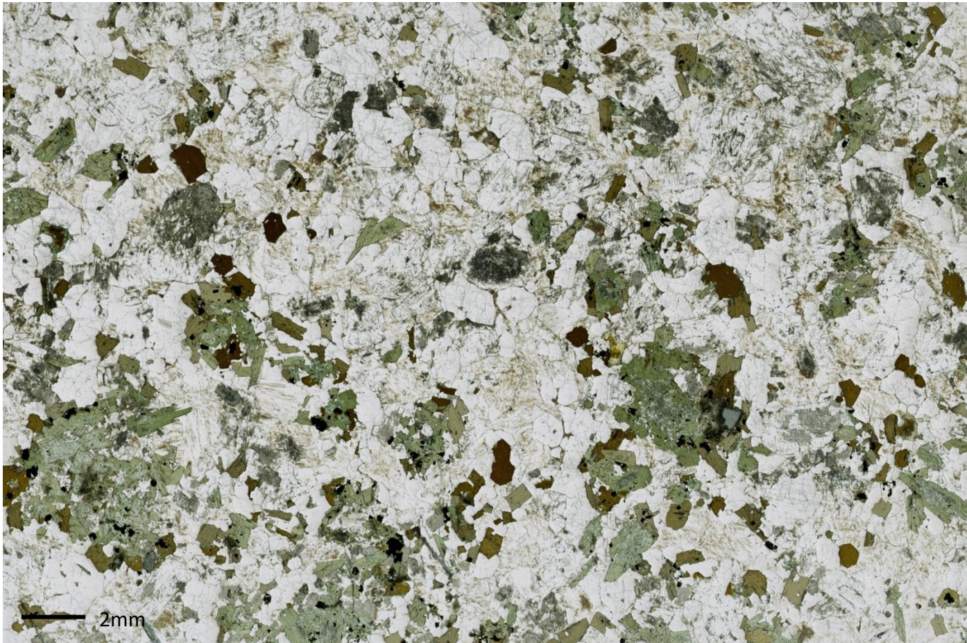
BP22 - Granite
