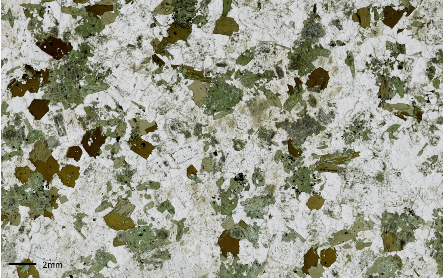
BP29 - Granite
