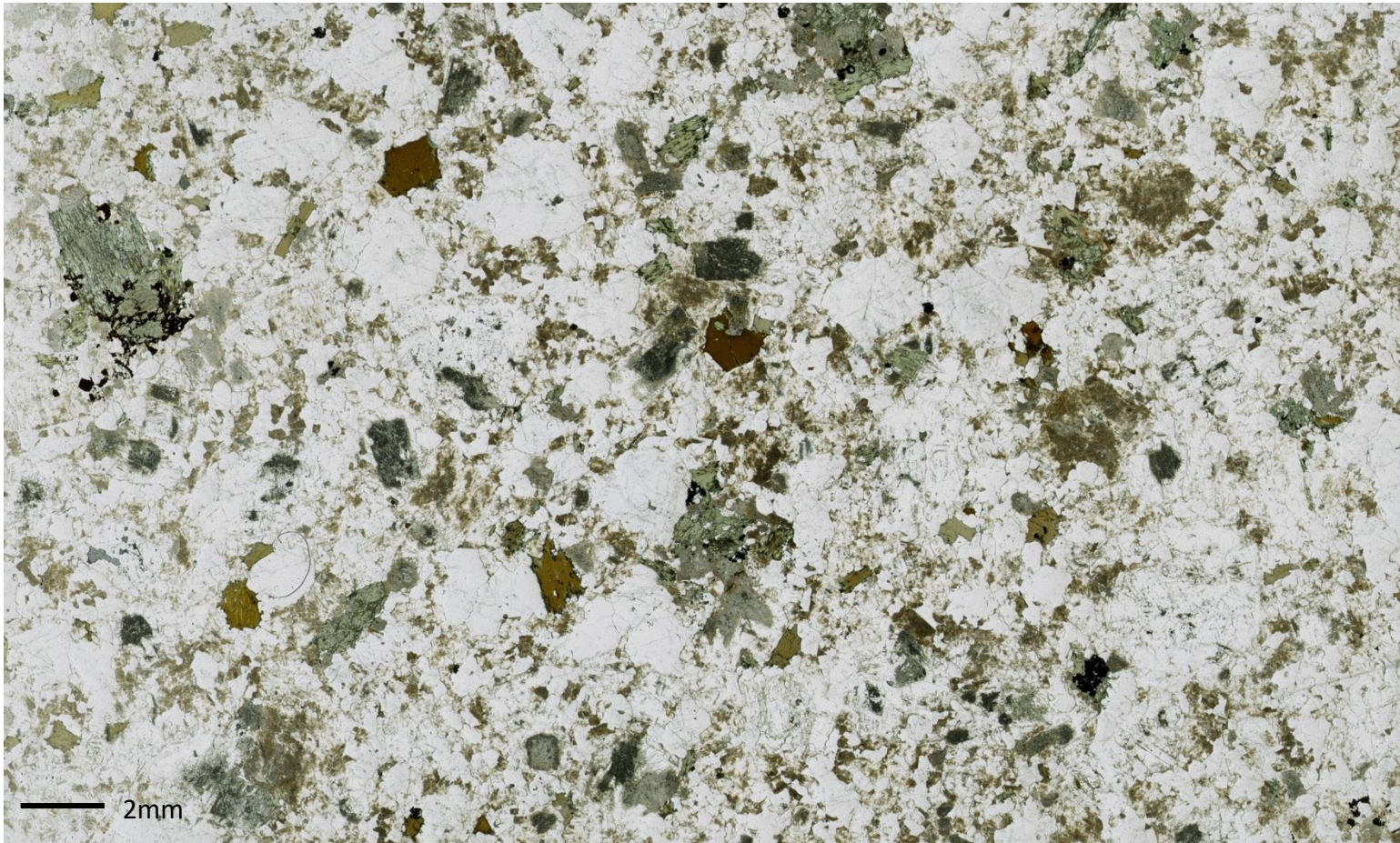
BP11 - Granite
