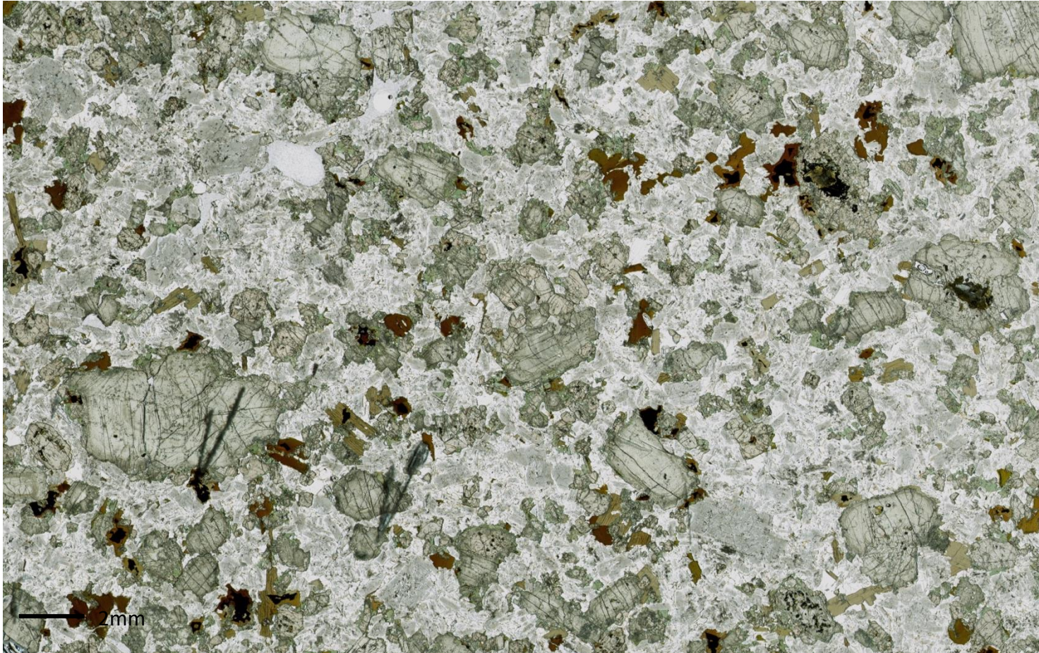
BP34 - Diorite
