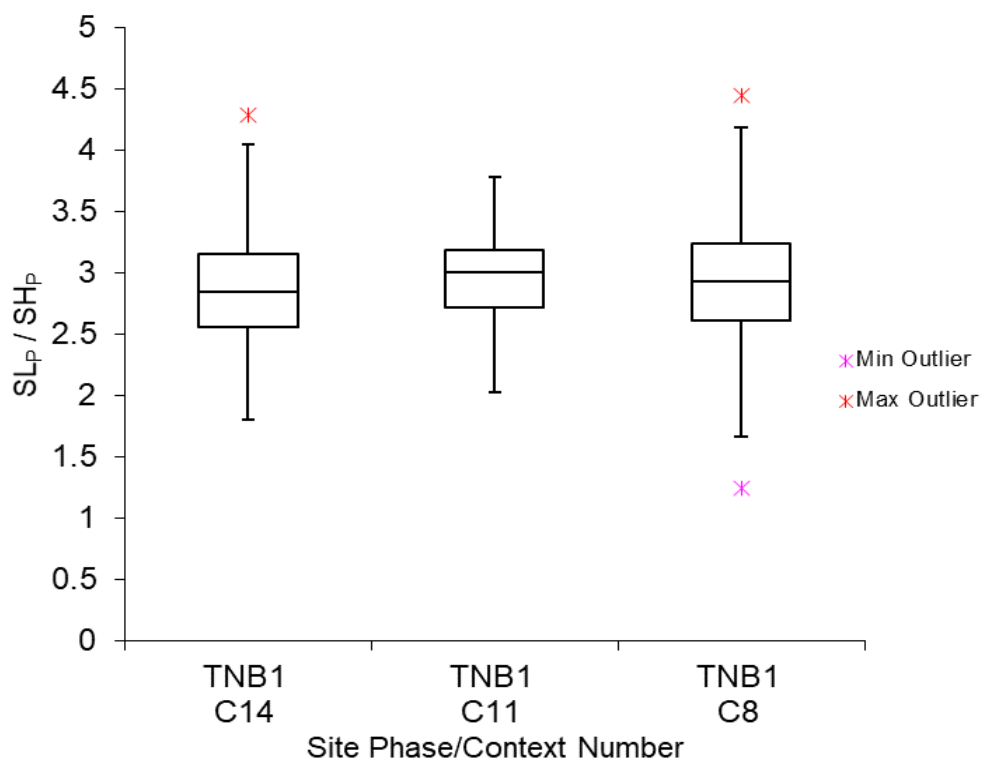
Figure C6-58: The population structures in terms of conicity from section C-D. Samples sizes as per figure C6-56.
