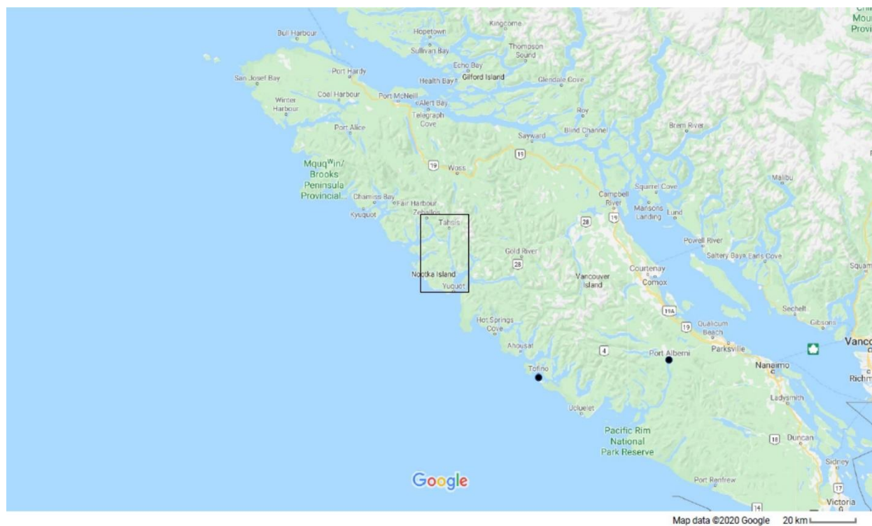
Figure C3-2B: The location of Friendly Cove on Vancouver Island. The black dots show the locations for which modern SST data was obtained.
