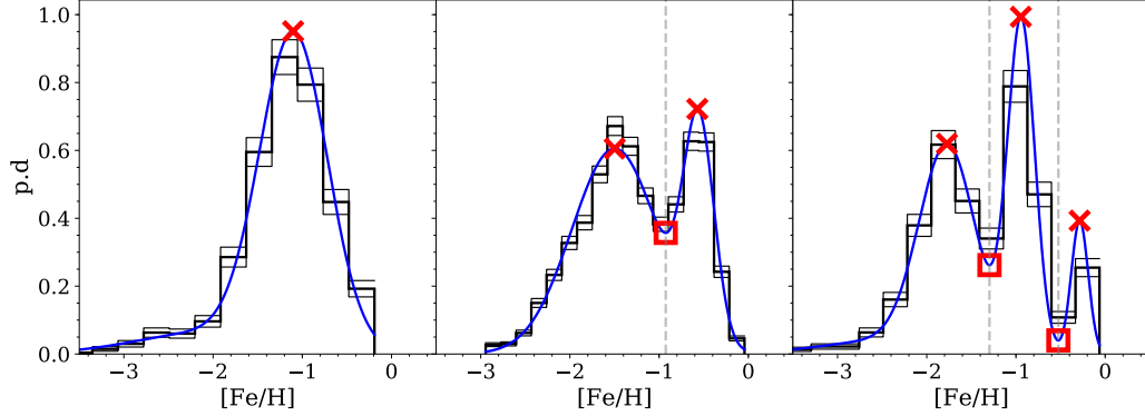
Figure 2.1: Metallicity probability density (p.d.) for examples of galaxies with one (left), two (middle) and three (right) distinct stellar populations as determined by the method described in Section 2.2.4. The black lines show binned data and corresponding Poisson errors. The blue line shows the best fitting Gaussian Mixture Model. The red crosses show the location of peaks; their number is equal to the number of identified populations. The red squares show the local minima and mark the locations where populations are split (also shown with a vertical dashed grey line).
