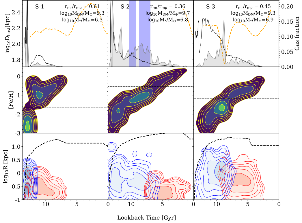
Figure 2.9: Properties of three example satellites in order of increasing stellar mass. Top: grey shaded areas show the SFH of the dwarfs in arbitrary units. The black solid lines show the gas fraction of the satellites (the bound gas mass divided by the dark matter mass), with the corresponding scale displayed on the right. The yellow dashed lines show distance to the host galaxy. For dwarf S-2, the blue bands show the times of interaction with cosmic filaments, as will be illustrated in Fig. 2.10. Middle: the metallicity-age distribution for the three galaxies. The dashed line shows the metallicity value at which our method splits the two populations. The probability density contours are geometrically spaced with a ratio of 2 and are consistent for the three dwarfs. Bottom: the radii at which the metal-rich (red) and the metal-poor (blue) particles form. The black dashed line is the evolution of the virial radius, which becomes the tidal radius after infall. The width of the smoothing kernel of the density estimate is consistent for the three galaxies across the middle and bottom panels.
