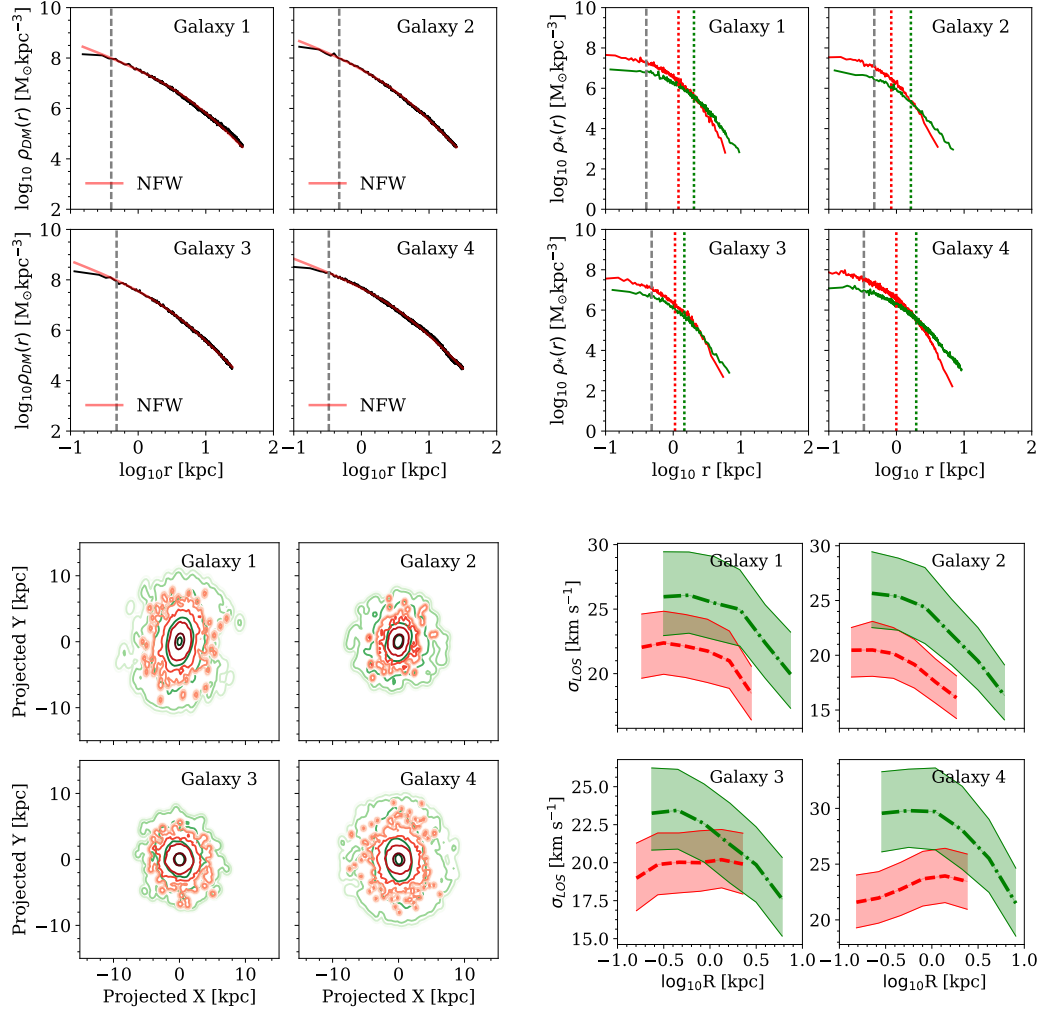
Figure 3.5: Upper left : dark matter profiles for the four illustrative examples discussed in this section. As for all galaxies in our sample, the inner density slope has a cusp; the best fitting NFW profile is shown in red. The grey dashed line marks the convergence radius defined by Power et al. (2003). Upper right : stellar density profiles for the metal-rich (red) and metal-poor subpopulations (green) for the four examples. The grey dashed line marks the convergence radius and the red and green dotted lines show the 3D half-mass radii of the metal-rich and metal-poor subpopulations respectively. The metal-poor component is more extended, with the metal-rich population concentrated near the centre. Lower left : probability density contours of the spatial distribution of stars in the four galaxies. The red and green contours represent the metal-rich and metal-poor subpopulations, respectively, with the highest contour enclosing p(x, y) = 0.1 and lower ones decreasing in probability density by factors of 10. The galaxies are viewed along the direction of the intermediate axis of the metal-poor subpopulation. Lower right : velocity dispersion profiles for the four examples, projected over 100 lines of sight, as a function of projected distance from the centre. The red dashed line and the green dash-dotted line show the medians of the metal-rich and the metal-poor subpopulations, respectively. The bands show the 1\sigma scatter. The metal-rich subpopulation is kinematically colder than the metal-poor subpopulation at small radii.
