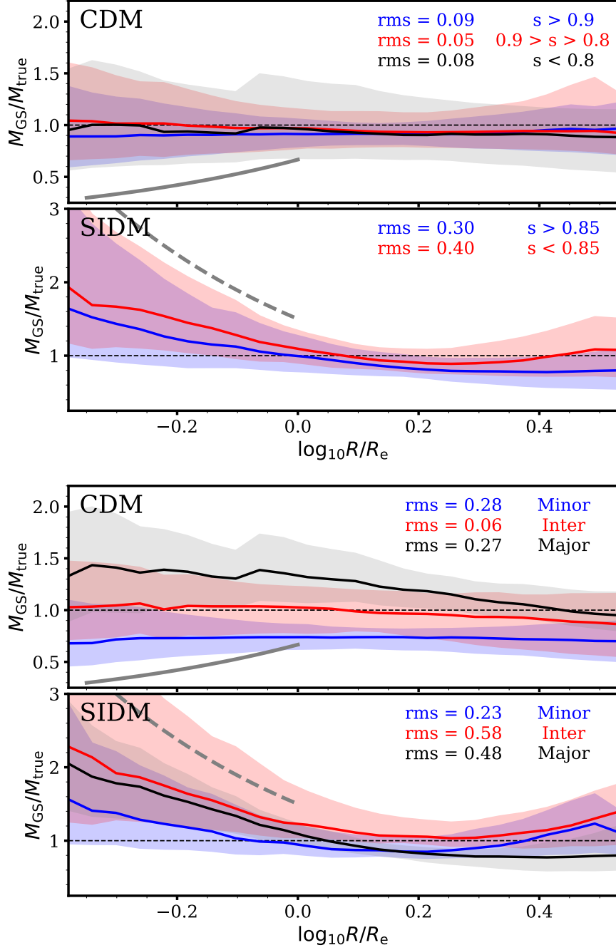
Figure 4.11: Top : bias in mass profiles returned by GRAVSPHERE for dwarfs, grouped by their minor-to-major axis ratio c/a . The top panel shows the CDM sample and the bottom panel shows the SIDM sample. Bottom : line-of-sight effects on the accuracy of the mass profile recovery by GRAVSPHERE. The sample of galaxies is split into those viewed along the minor (blue line and bands), intermediate (red) and major (black) axis. Only dwarfs with s < 0.8 for CDM and s < 0.85 for SIDM are shown. The dotted black line in each plot represents unbiased results. The solid grey line corresponds to the bias expected in order to incorrectly infer a core within the half-light radius of a cuspy dark matter halo. The dashed grey line corresponds to the bias expected to incorrectly infer an NFW cusp, when in reality there is a core.
