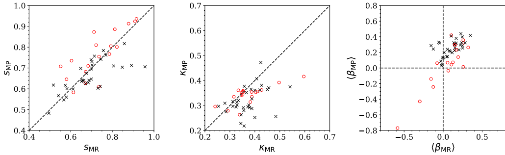
Figure 3.4: Left : the correlation of the sphericities of the metal-poor and the metal-rich subpopulations for satellites (red circles) and field galaxies (black crosses) in our sample. The dashed line indicates the one-to-one relation. Middle : \kappa_{\text{rot}} of the metal-poor and metal-rich subpopulations. Right : the correlation between the average velocity anisotropy of the metal-poor and metal-rich subpopulations. The dashed lines indicate isotropy, \beta=0 .
