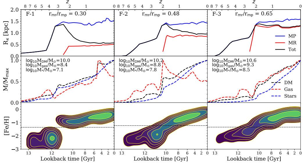
Figure 2.5: Top : the evolution of the half-mass radius of the metal-poor stars formed in-situ (blue), the metal-rich stars (red) and the entire set of stellar particles formed in-situ (black). The lookback time is shown on the bottom axis and the redshift on the top. The subpopulations are tracked from the time when they first contain at least 50 stellar particles. From left to right are three examples of galaxies with progressively poorer spatial segregation. Middle : the evolution of mass for the dark matter (black), gas (red) and stars (blue). Sudden increases in dark matter mass correspond to mergers. The mass is normalised by the maximum component mass, shown by the labels in the upper left corners. Note that galaxy F-2 merges with two haloes at approximately the same time. Bottom : the metallicity-age relation for the three example galaxies. The rise in metallicity is seen to occur following a merger. The contours in probability density are spaced geometrically by factors of 2 and are consistent for the three galaxies.
