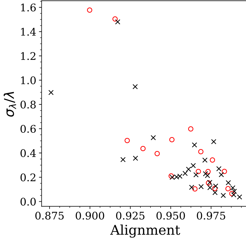
Figure 3.8: Relative upper error (the difference between the 84 th and the 50 th percentile divided by the median value) on the mass slope accuracy, \lambda , as a function of the alignment of the metal-rich and the metal-poor subpopulations, as defined in Section 3.3.1. Satellites and field galaxies are shown with red circles and black crosses respectively. Measurements in galaxies with more misaligned subpopulations are more likely to return larger values of \Gamma .
