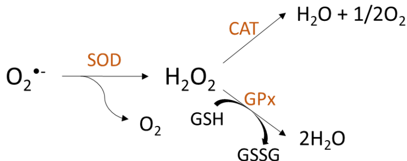
Figure 8.2: Diagram of the activity of enzymatic anti-oxidants activity in the lens. SOD catalyses the conversion of O_2^{\bullet -} into H_2O_2 . Subsequently H_2O_2 can be neutralised by conversion into H_2O , this is catalysed by CAT or GPx. SOD: superoxide dismutase, CAT: catalase, GPx: glutathione peroxidase, GSH: glutathione, GSSG: glutathione disulphide
