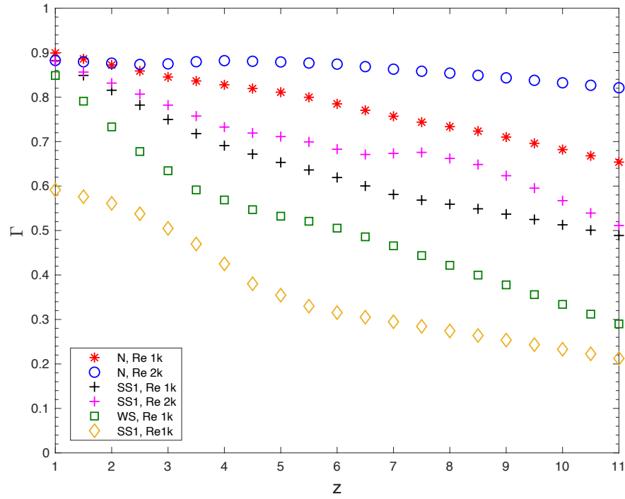
Figure 4.34: The decay of the vortex core circulation, \Gamma of the first plane, \theta = 1 for all cases.
