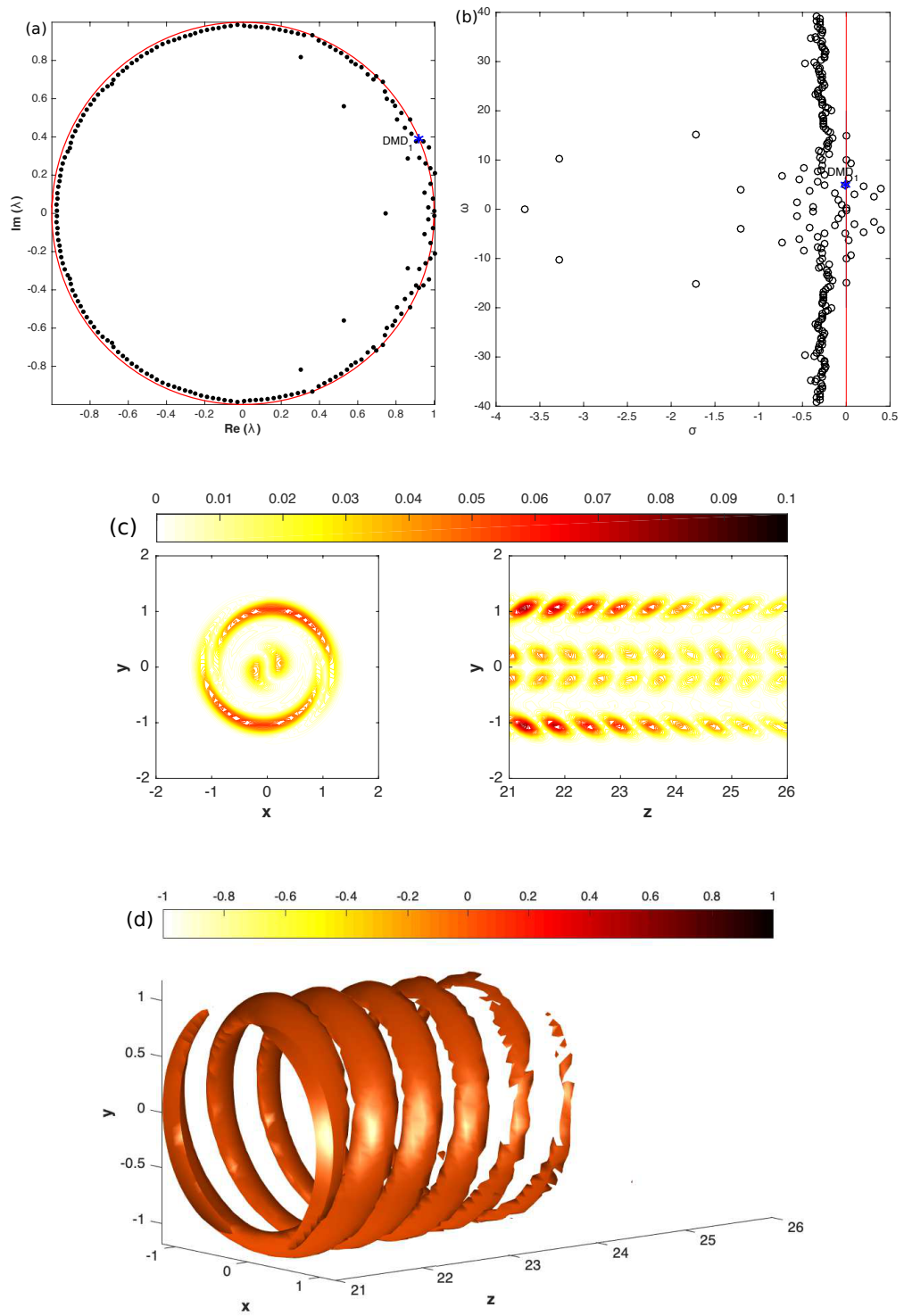
Figure 6.34: Dynamic eigenvalue characteristics of N , Re1k. (a) Ritz values and (b) DMD spectra of temporal DMD 1 . (c) |\omega| contour plot in xy -cut at z = 23.5 (left) and zy -cut at x = 0 (right). (d) Isosurface plot of |\omega| = 0.05 corresponding to DMD 1 ( \lambda = 0.9201 + 0.3893i ).
