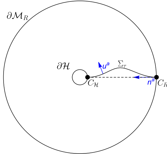
Figure 3.5: An illustration of the foliation of the Euclidean \{\tau, r\} section of the brane black hole. The normals u^a and n^a of, respectively, the foliation \Sigma_\tau and manifold boundaries are shown, together with the codimension two surfaces C_R and C_H , which may be regarded as codimension one submanifolds of the \Sigma_\tau surfaces. Since \Sigma_\tau is not necessarily a ray (dashed line), in general (\partial_\tau)^a and u^a are not always pointing in the same direction.
