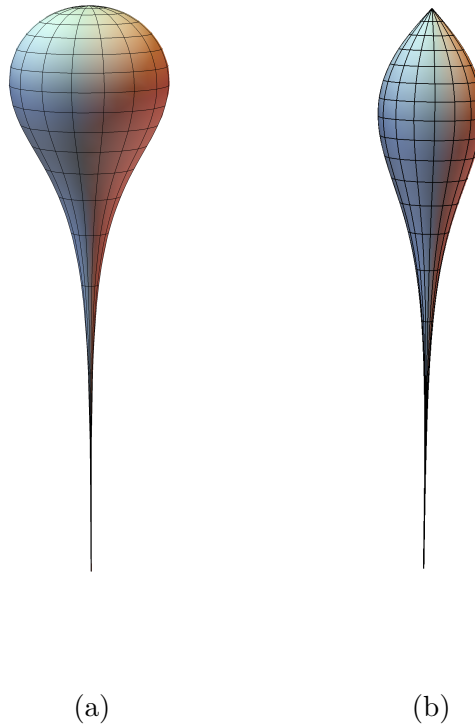
Figure 4.6: Horizon embeddings in \mathbb{R}^3 of critical black holes. We display the horizon embeddings of the critical C-metric for (a) K = 2\Xi and (b) K = 3\Xi . These are the equivalent horizons of fig. 4.4 in the critical limit 2\tilde{m} = \Xi .
