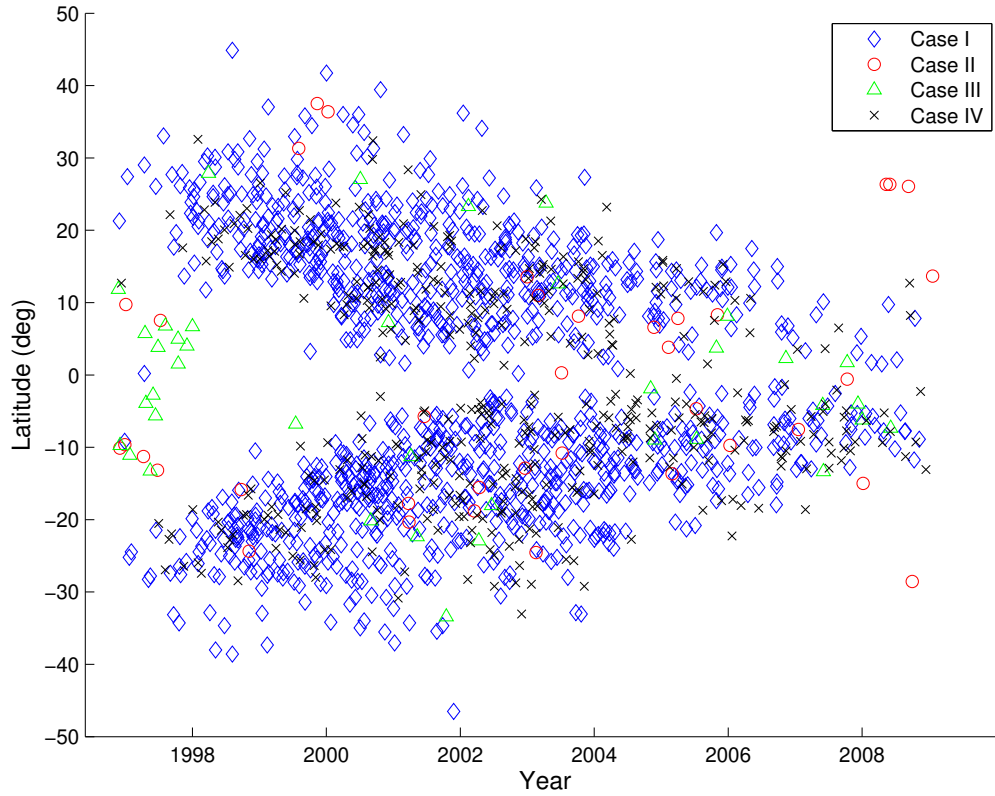
Figure 2.5: Scatterplot of the four cases of BMR alignment. Case I is positive tilt and normal polarity, Case II is positive tilt and abnormal polarity, Case III is negative tilt and abnormal polarity, and Case IV is negative tilt and normal polarity. Normal (abnormal) refers to when the leading polarity matches (opposes) the typical leading polarity of the cycle in question. Positive (negative) tilt refers to when the leading polarity is closer to (further from) the equator than the trailing polarity.
