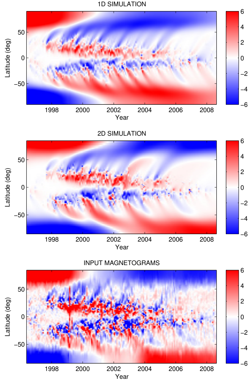
Figure 2.15: Top: Butterfly diagram for the optimal parameter 5-set for the 1D model in Table 2.5(a). Middle: Butterfly diagram for the optimal parameter 5-set for the 2D model with varying B_{\text{par}} in Table 2.5(c). Bottom: Ground truth data for Cycle 23.
