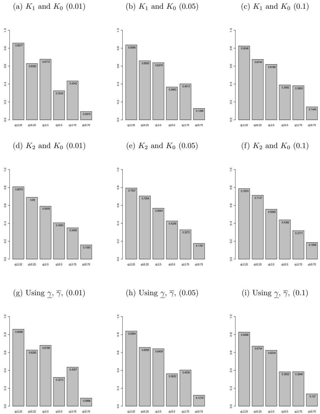
Figure 4.12: Proportion of runs with future observation greater than the quartiles, n = 50 .
