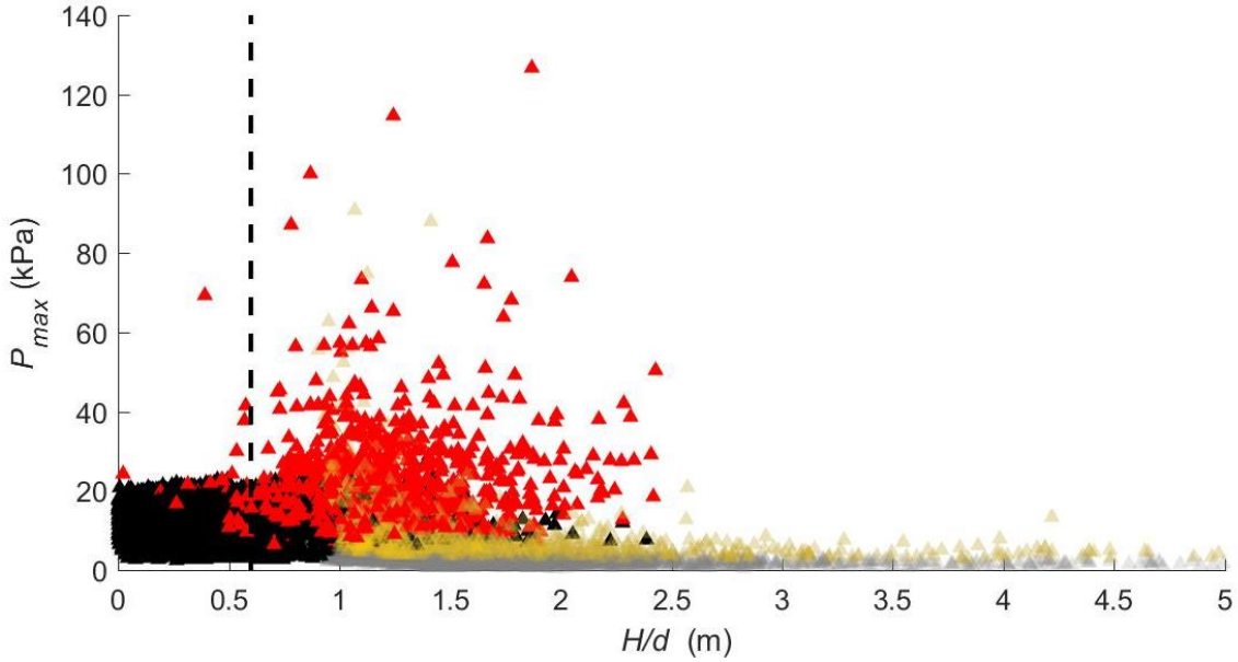
Figure 7.12: Combined wave height / water depth ratio ( H/d ) for each wave in all datasets and their corresponding maximum pressure values ( P_{max} ). Impulsive (red) and pulsating (black) loads are shown. H/d estimates, based on extrapolating d to zero and using the breaker criterion to find the maximum H , are shown in faded yellow and grey data points for impulsive and pulsating loads respectively. The breaker criterion ( \gamma = 0.6 ) is shown (black dashed line).
