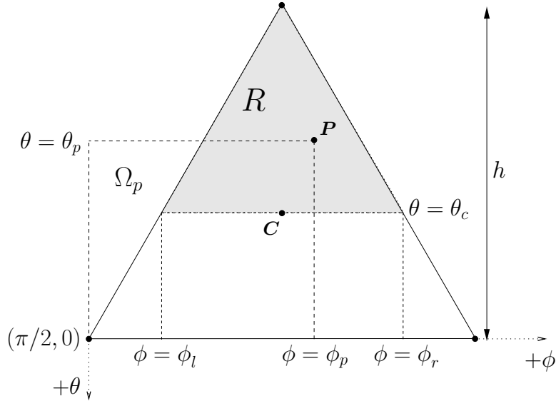
Figure 6.2: Illustration of R and \Omega_p for some \Delta_* .
