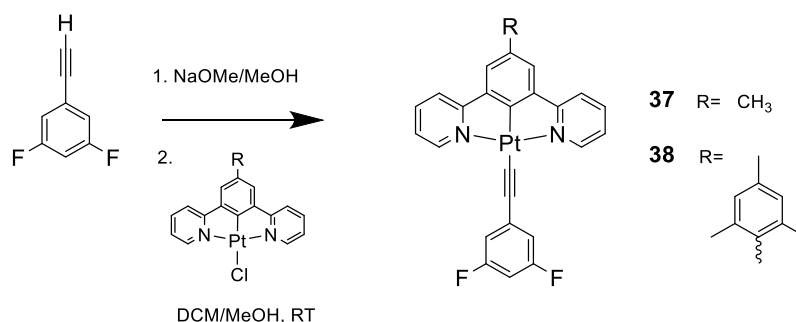
Scheme 3.2: Synthesis of Pt(N^{\wedge}C^{\wedge}N) acetylide complexes 37 and 38 .
