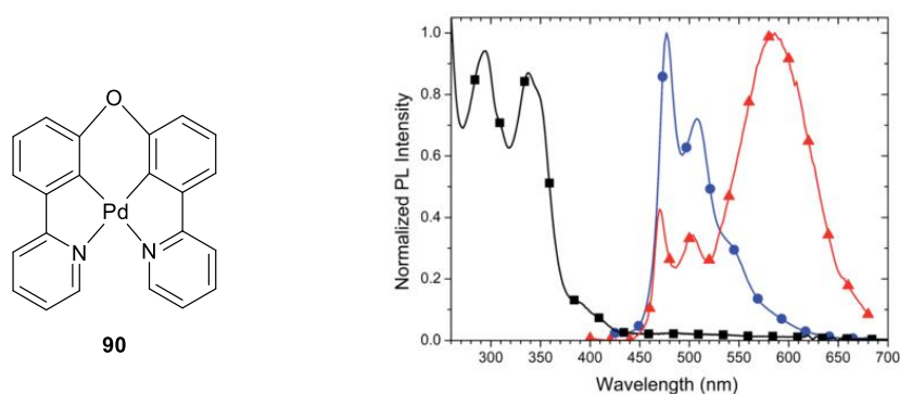
Figure 4.14: The structure of 90 and its absorption and emission in a 1 wt. % 26mCPy film (blue) and in degassed DCM solution (red). Reproduced from Fleetham et al. by permission of the Royal Society of Chemistry. 167
