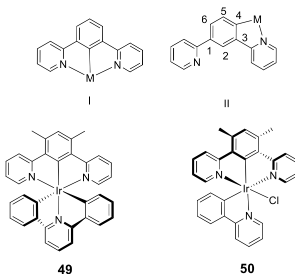
Figure 3.15: Different possible binding modes of dipyridylbenzene (I and II, top) and structures of the bis-tridentate complex 49 and 3+2+1 complex 50 (bottom).
