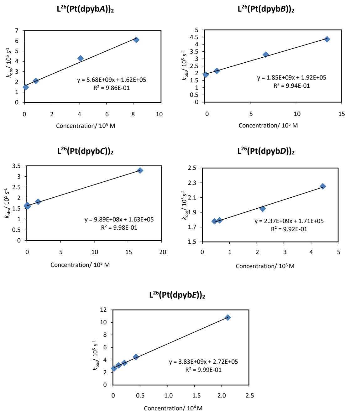
Figure 5.19: Stern-Volmer plots for class 2 complexes showing self-quenching parameters.
