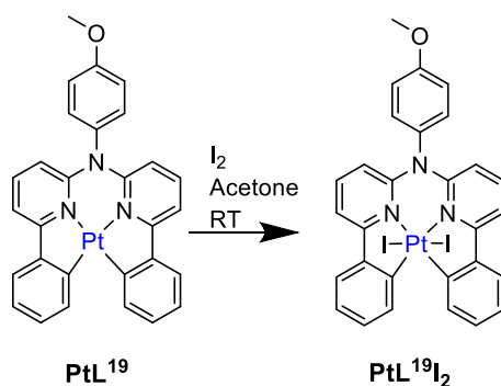
Scheme 4.4: Oxidation of \text{PtL}^{19} to \text{PtL}^{19}\text{I}_2 .
