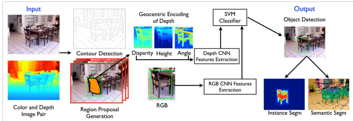
Figure 4.2 An overview of the object detection and segmentation approach of Gupta et al [63]. Colour and depth information are input to separate CNNs to extract relevant features which are then classified by SVM.
