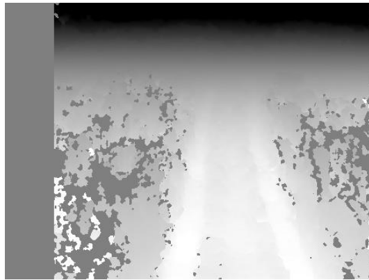
Figure 4.6 An example of a height map, H . Darker pixels are further from the assumed ground plane.
