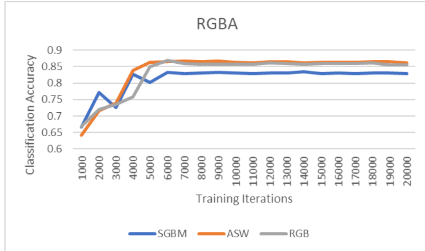
Figure 4.19 Training progress of the network models using RGB-A images, with angle with gravity derived from both SGBM and ASW algorithms. RGB results are also shown for comparison.
