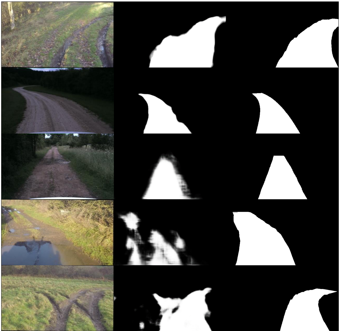
Figure 5.11 Example images from our test data set. Left: input, centre: raw CNN output prior to post-processing, right: ground truth
