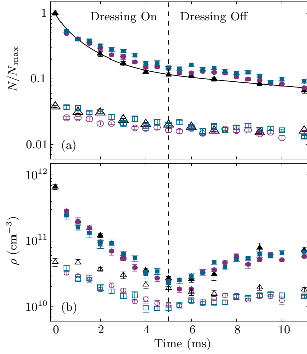
Figure 6.9: (a) Atom number as a function of time for three different states: 5s34d\ ^3D_2 (blue squares), 5s36d\ ^3D_2 (black triangles) and 5s37d\ ^3D_2 (purple circles). Different initial densities of 1 \times 10^{12}\text{ cm}^{-3} (filled data points) and 5 \times 10^{10}\text{ cm}^{-3} (hollow data points) are shown. The vertical dashed line indicates where the UV beam is turned off (after 5 ms). (b) Density as a function of time for the same states.
