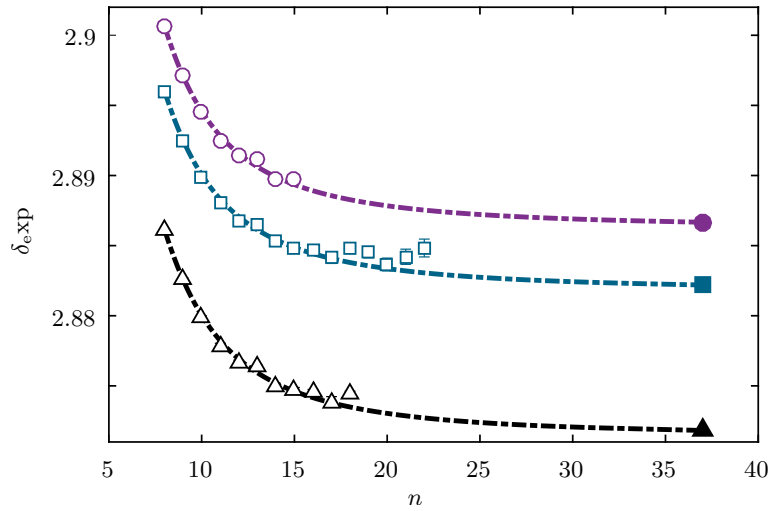
Figure 5.14: Quantum defects, \delta_{\text{exp}} , for the 5snp ^3P_0 (purple circles), ^3P_1 (blue squares) and ^3P_2 (black triangles) Rydberg series. The hollow markers are previously measured values from other groups [48] while the filled markers show the results from our measurements. The solid lines are fits to the data using the Rydberg-Ritz formula.
