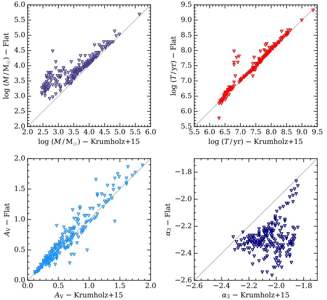
Figure 3.7: Comparison between the median values for each parameter returned by CLUSTER_SLUG for flat priors and the physically motivated priors by Krumholz et al. (2015b). The grey line marks the one-to-one correspondence. While extinction and age are insensitive to the choice of priors, mass and \alpha_3 depend on the assumed prior, owing to a degeneracy between these two parameters.
